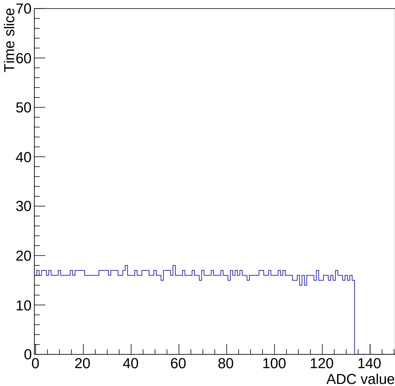
Evt 10 Time mcm 2000 chip 0 chan 6 34625-gain0-shaper0
