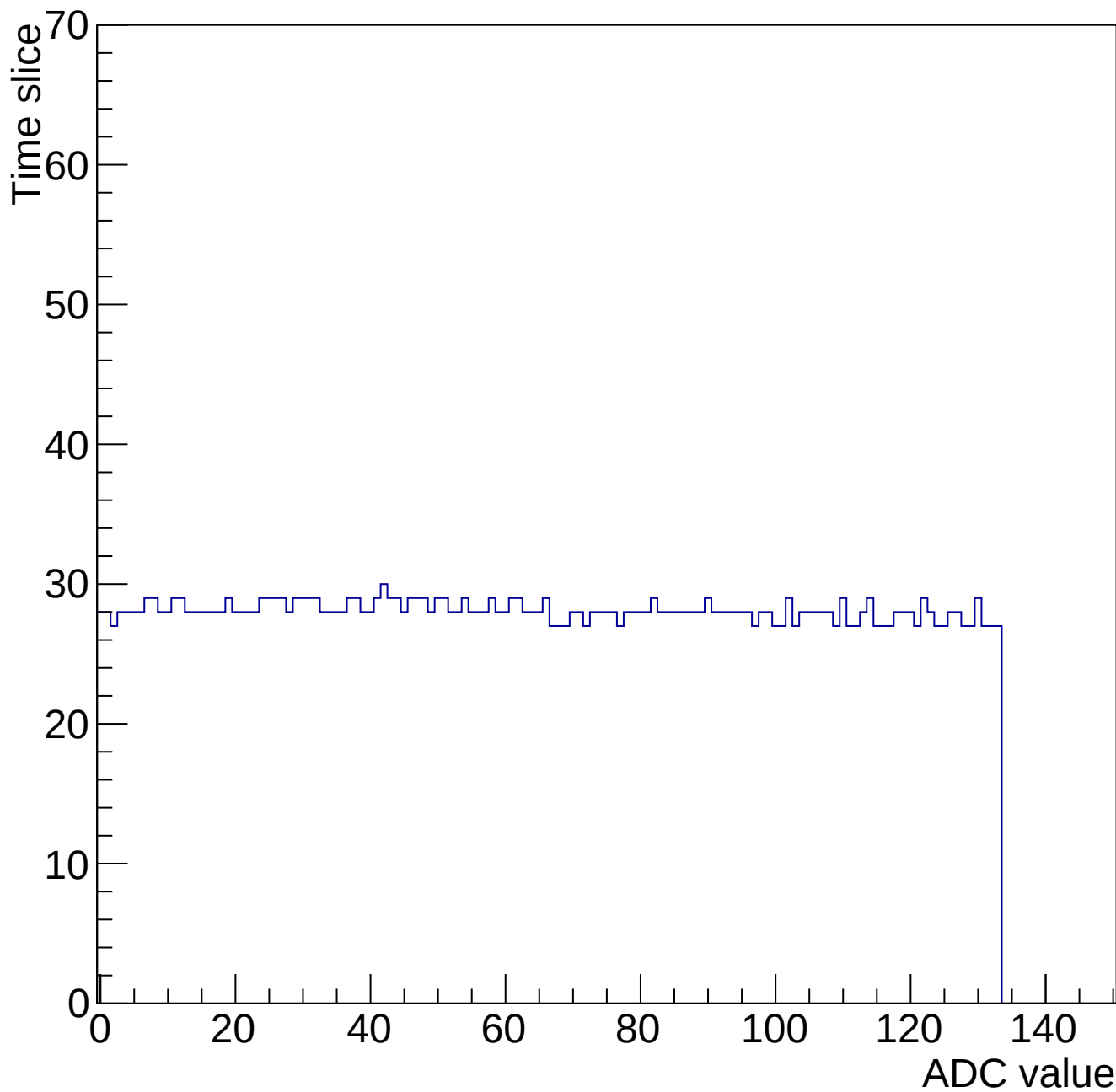
Evt 10 Time mcm 2000 chip 0 chan 8 34625-gain0-shaper0
