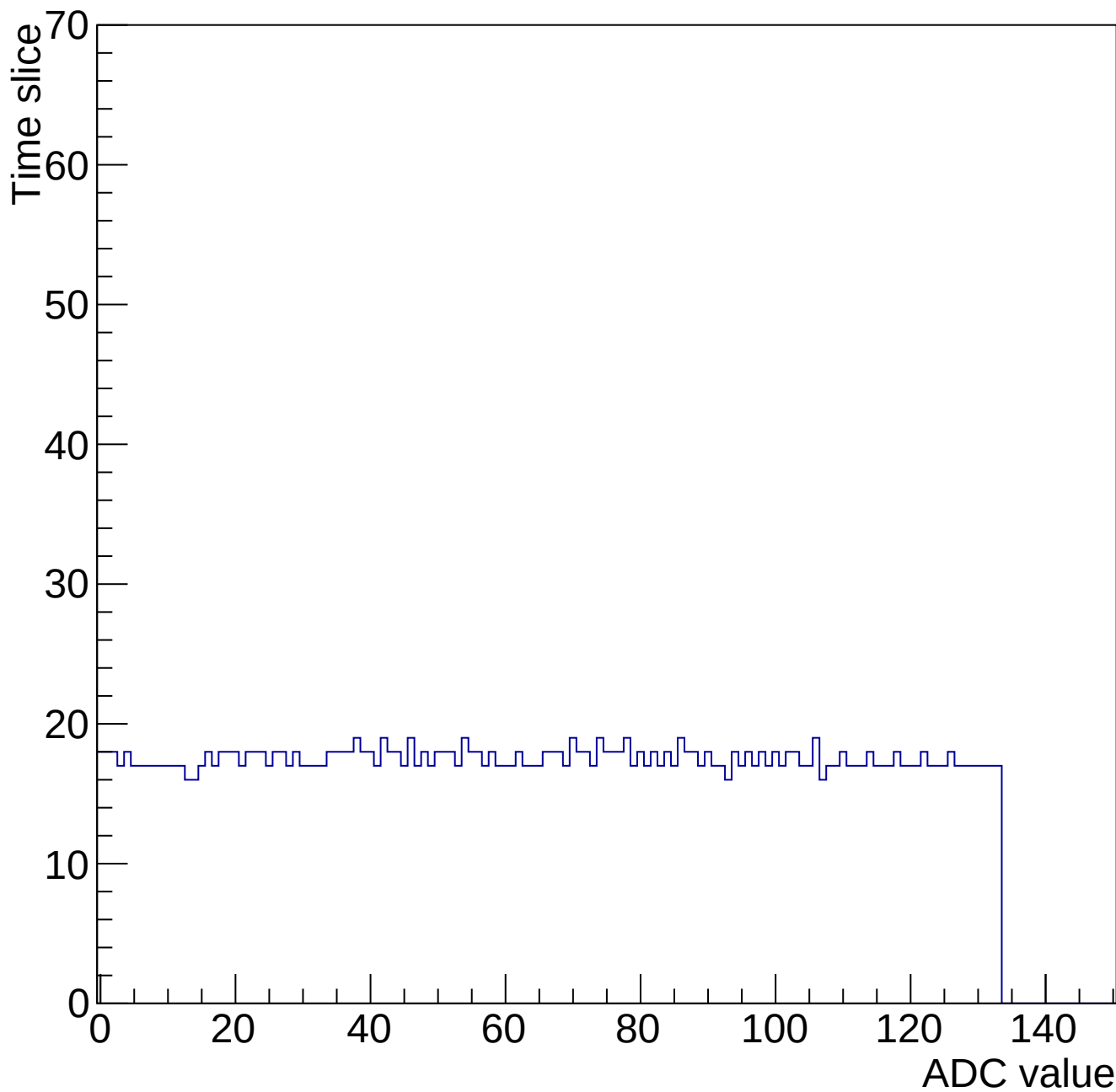
Evt 10 Time mcm 2000 chip 0 chan 9 34625-gain0-shaper0
