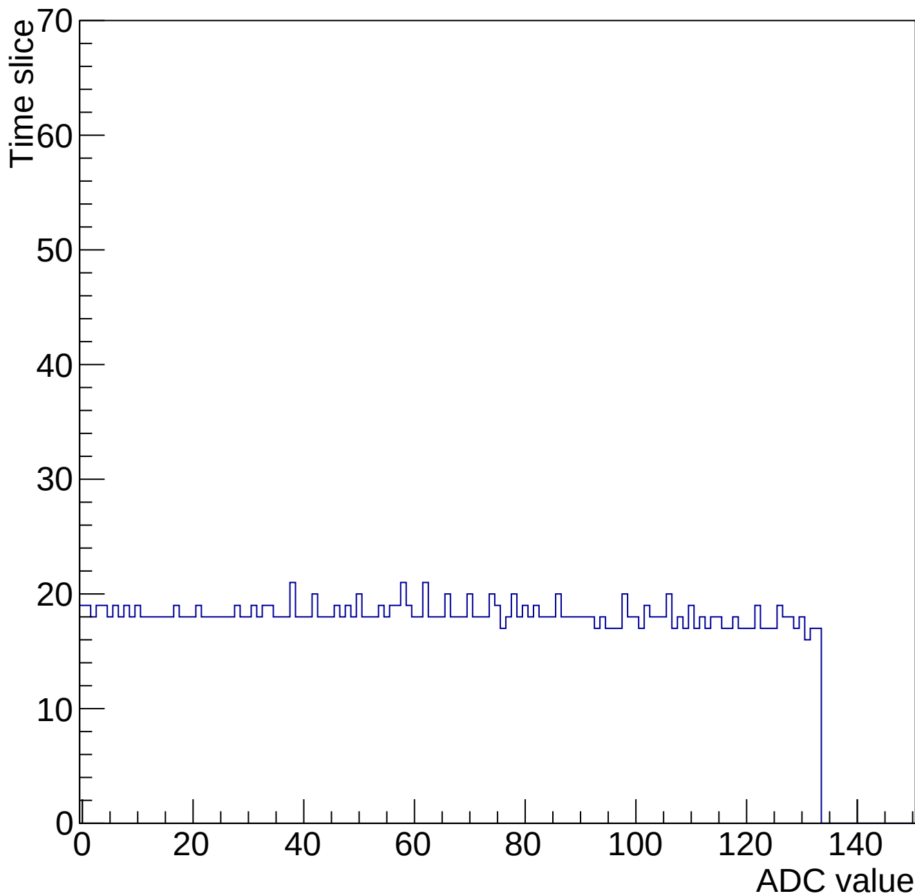
Evt 10 Time mcm 2000 chip 0 chan 0 34625-gain0-shaper0
