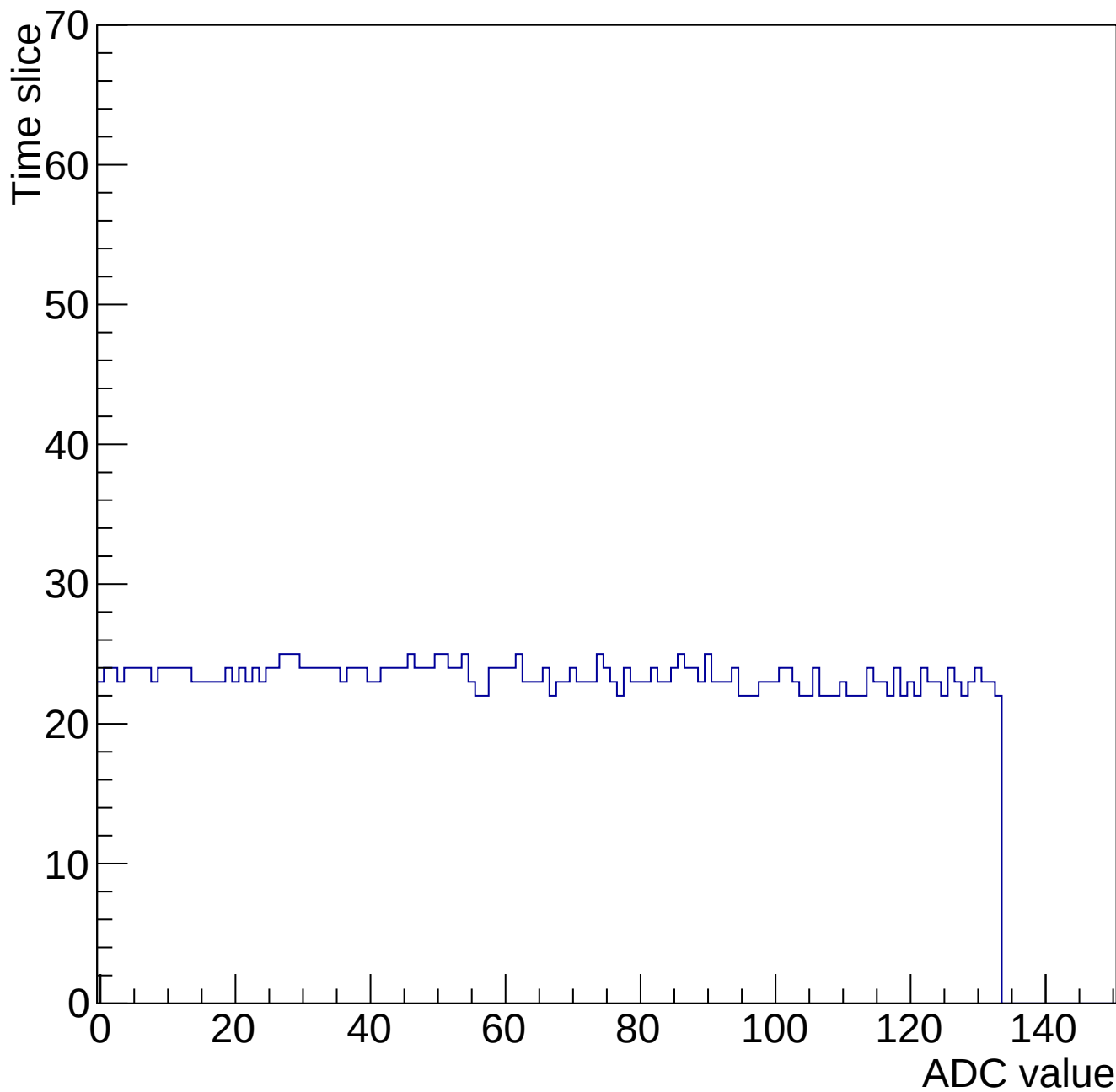
Evt 10 Time mcm 2000 chip 0 chan 3 34625-gain0-shaper0
