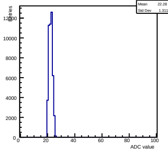
Pedestals ch 13 chip 2000 gain0-shaper6
