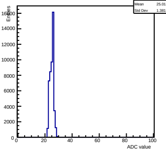
Pedestals ch 12 chip 2000 gain0-shaper6
