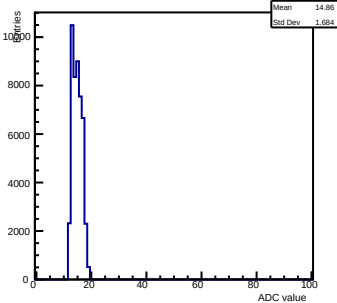
Pedestals ch 0 chip 2000 gain0-shaper6
