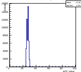
Pedestals ch 5 chip 2000 gain0-shaper6
