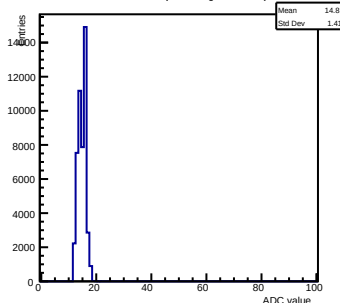
Pedestals ch 6 chip 2000 gain0-shaper6
