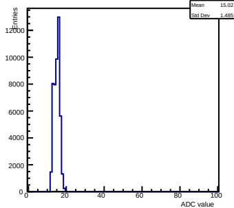
Pedestals ch 10 chip 2000 gain0-shaper6
