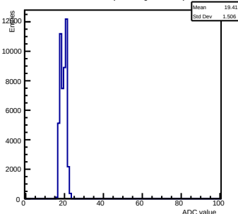
Pedestals ch 4 chip 2000 gain0-shaper6
