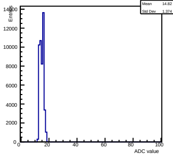
Pedestals ch 9 chip 2000 gain0-shaper6
