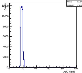
Pedestals ch 2 chip 2000 gain0-shaper6
