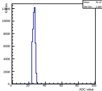
Pedestals ch 1 chip 2000 gain0-shaper6
