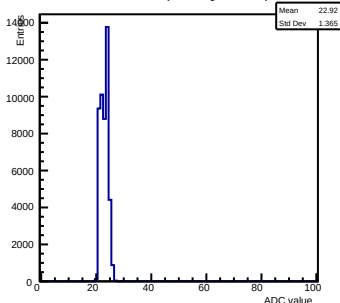
Pedestals ch 7 chip 2000 gain0-shaper6
