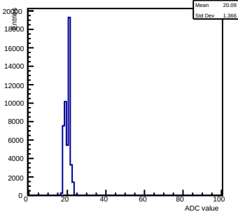
Pedestals ch 11 chip 2000 gain0-shaper6
