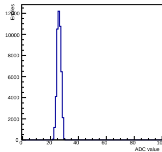
Pedestals ch 10 chip 2001 gain0-shaper0
