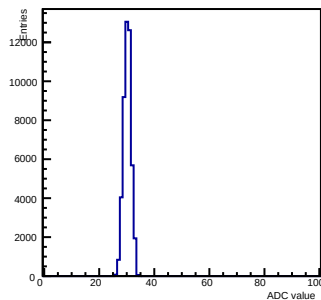
Pedestals ch 15 chip 2001 gain0-shaper0
