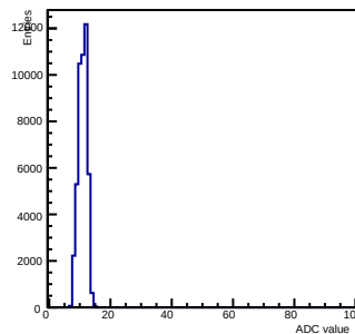
Pedestals ch 14 chip 2001 gain0-shaper0
