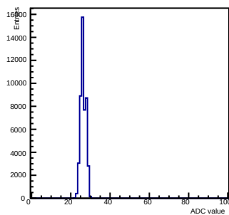
Pedestals ch 3 chip 2001 gain0-shaper0
