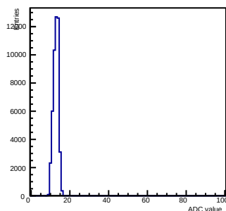
Pedestals ch 7 chip 2001 gain0-shaper0
