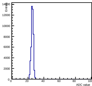
Pedestals ch 13 chip 2001 gain0-shaper0
