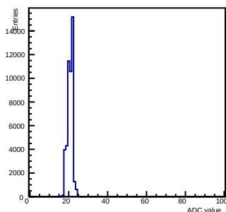
Pedestals ch 5 chip 2001 gain0-shaper0
