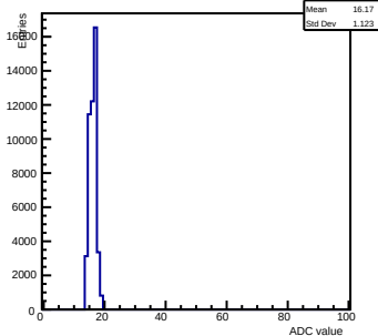
Pedestals ch 12 chip 2001 gain0-shaper6
