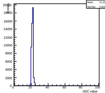
Pedestals ch 11 chip 2001 gain0-shaper6
