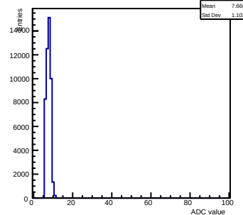
Pedestals ch 14 chip 2001 gain0-shaper6
