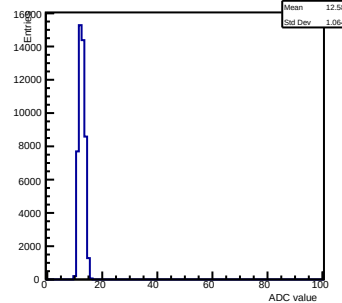
Pedestals ch 2 chip 2001 gain0-shaper6
