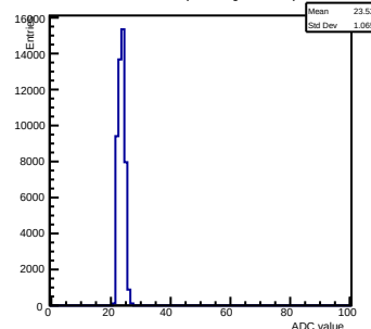
Pedestals ch 6 chip 2001 gain0-shaper6
