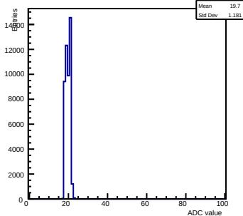
Pedestals ch 13 chip 2001 gain0-shaper6
