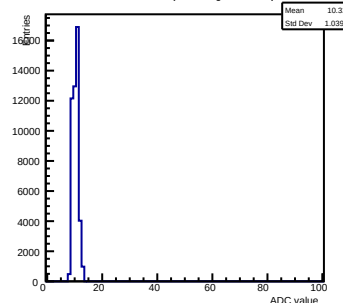
Pedestals ch 7 chip 2001 gain0-shaper6
