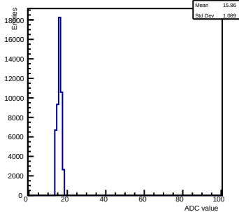
Pedestals ch 9 chip 2001 gain0-shaper6
