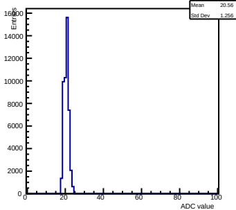
Pedestals ch 0 chip 2001 gain0-shaper6
