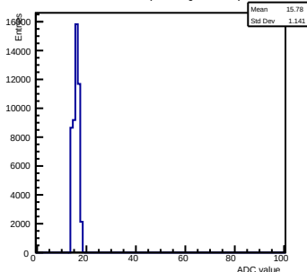
Pedestals ch 5 chip 2001 gain0-shaper6
