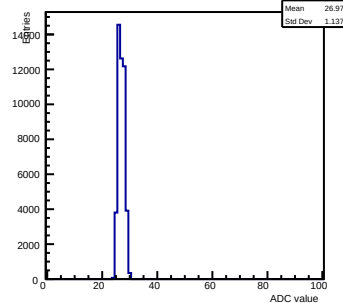
Pedestals ch 15 chip 2001 gain0-shaper6
