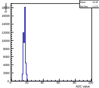
Pedestals ch 8 chip 2001 gain0-shaper6
