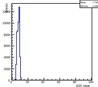
Pedestals ch 14 chip 2002 gain0-shaper0
