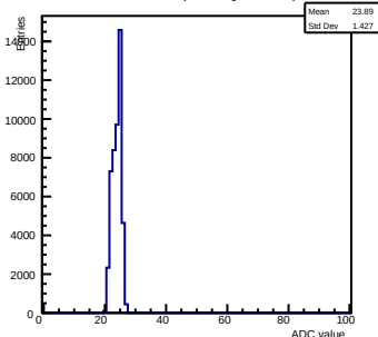
Pedestals ch 5 chip 2002 gain0-shaper0
