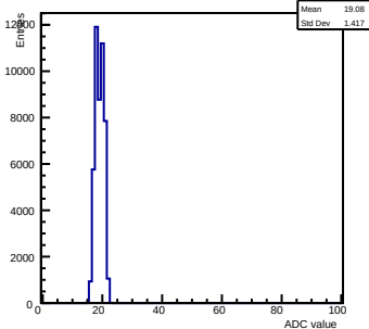
Pedestals ch 13 chip 2002 gain0-shaper0
