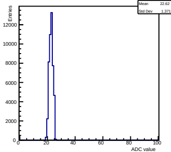
Pedestals ch 0 chip 2002 gain0-shaper0
