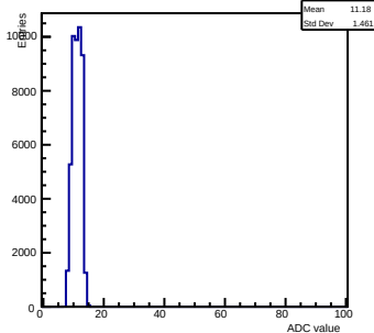
Pedestals ch 12 chip 2002 gain0-shaper0
