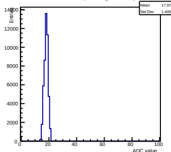
Pedestals ch 6 chip 2002 gain0-shaper0
