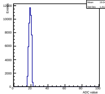
Pedestals ch 11 chip 2002 gain0-shaper0
