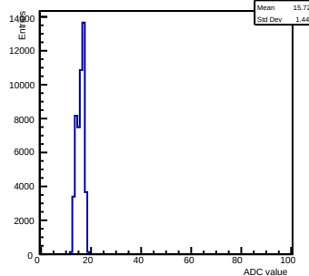
Pedestals ch 15 chip 2002 gain0-shaper0
