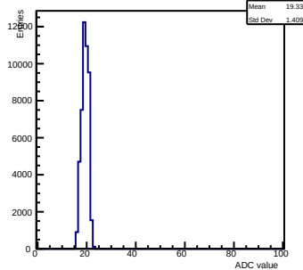
Pedestals ch 10 chip 2002 gain0-shaper0
