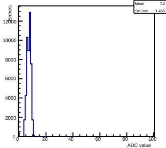
Pedestals ch 8 chip 2002 gain0-shaper0
