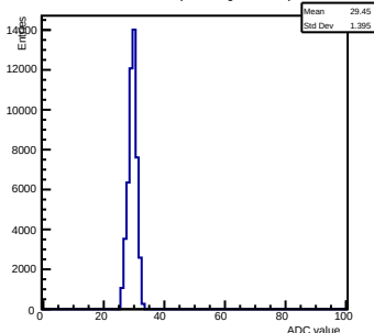
Pedestals ch 4 chip 2002 gain0-shaper0
