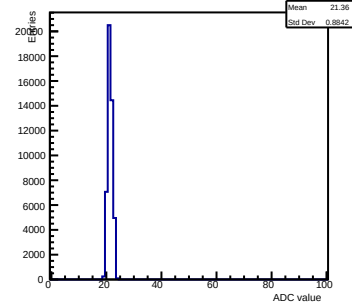
Pedestals ch 0 chip 2002 gain0-shaper6
