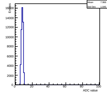
Pedestals ch 8 chip 2002 gain0-shaper6
