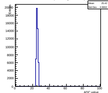
Pedestals ch 4 chip 2002 gain0-shaper6
