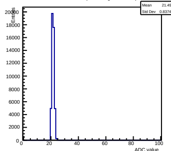
Pedestals ch 7 chip 2002 gain0-shaper6
