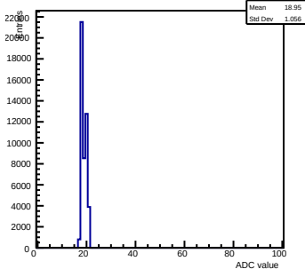
Pedestals ch 13 chip 2002 gain0-shaper6
