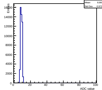
Pedestals ch 14 chip 2002 gain0-shaper6
