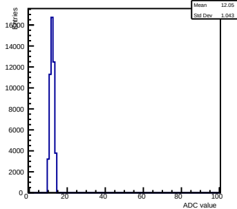
Pedestals ch 1 chip 2002 gain0-shaper6
