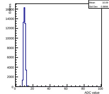
Pedestals ch 12 chip 2002 gain0-shaper6
