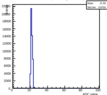
Pedestals ch 5 chip 2002 gain0-shaper6
