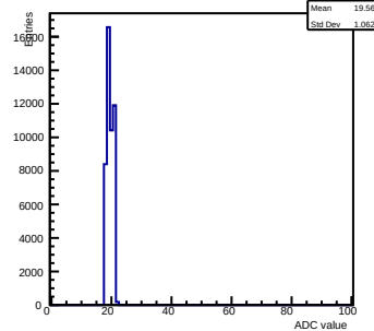
Pedestals ch 11 chip 2002 gain0-shaper6
