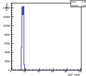
Pedestals ch 3 chip 2003 gain0-shaper6
