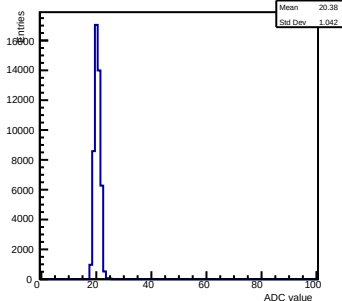
Pedestals ch 9 chip 2003 gain0-shaper6
