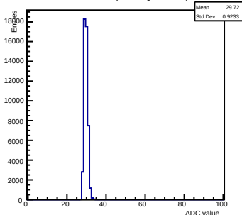
Pedestals ch 4 chip 2003 gain0-shaper6
