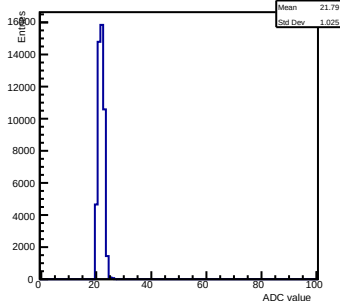
Pedestals ch 10 chip 2003 gain0-shaper6
