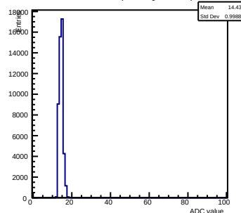
Pedestals ch 7 chip 2003 gain0-shaper6
