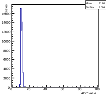
Pedestals ch 12 chip 2003 gain0-shaper6
