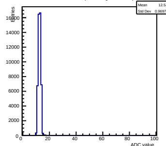
Pedestals ch 15 chip 2003 gain0-shaper6
