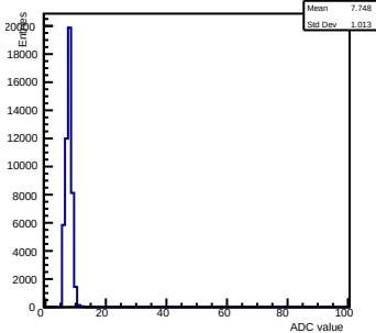
Pedestals ch 1 chip 2003 gain0-shaper6
