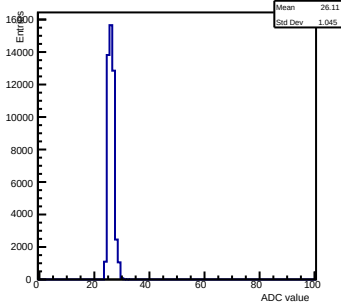
Pedestals ch 0 chip 2003 gain0-shaper6
