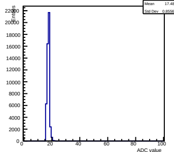
Pedestals ch 11 chip 2003 gain0-shaper6
