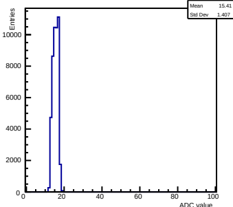
Pedestals ch 13 chip 2004 gain0-shaper0
