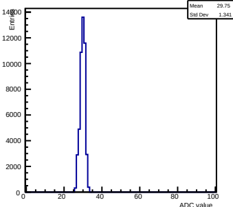
Pedestals ch 7 chip 2004 gain0-shaper0
