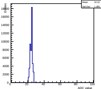
Pedestals ch 9 chip 2004 gain0-shaper0
