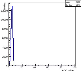
Pedestals ch 6 chip 2004 gain0-shaper0
