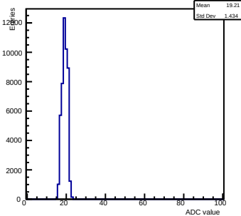
Pedestals ch 3 chip 2004 gain0-shaper0
