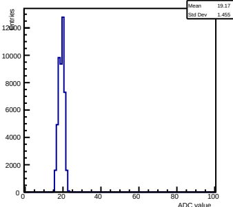
Pedestals ch 4 chip 2004 gain0-shaper0
