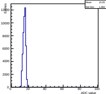
Pedestals ch 8 chip 2004 gain0-shaper0
