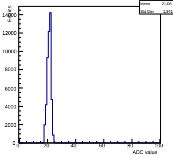
Pedestals ch 2 chip 2004 gain0-shaper0
