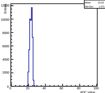
Pedestals ch 12 chip 2004 gain0-shaper0
