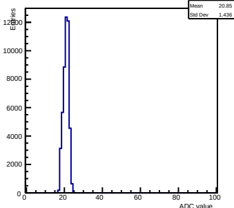
Pedestals ch 14 chip 2004 gain0-shaper0
