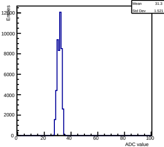
Pedestals ch 0 chip 2004 gain0-shaper0
