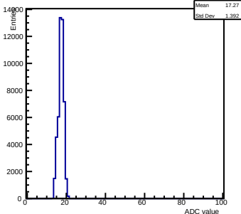
Pedestals ch 10 chip 2004 gain0-shaper0
