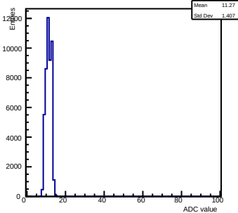
Pedestals ch 1 chip 2004 gain0-shaper0
