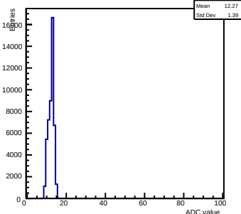
Pedestals ch 15 chip 2004 gain0-shaper0
