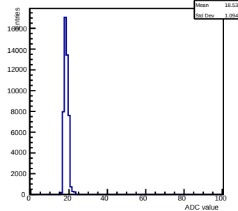
Pedestals ch 10 chip 2004 gain0-shaper6
