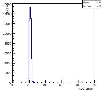
Pedestals ch 14 chip 2004 gain0-shaper6
