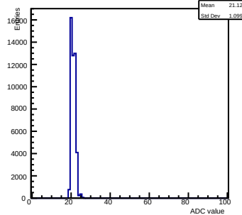
Pedestals ch 11 chip 2004 gain0-shaper6
