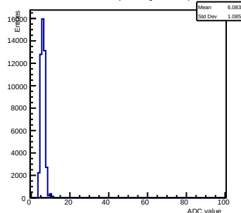
Pedestals ch 6 chip 2004 gain0-shaper6
