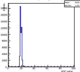
Pedestals ch 4 chip 2004 gain0-shaper6
