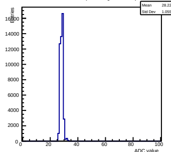
Pedestals ch 7 chip 2004 gain0-shaper6
