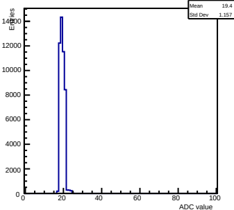
Pedestals ch 12 chip 2004 gain0-shaper6
