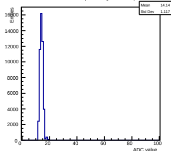
Pedestals ch 5 chip 2004 gain0-shaper6
