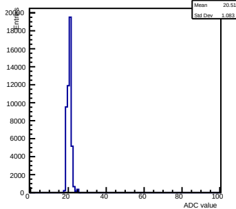
Pedestals ch 9 chip 2004 gain0-shaper6
