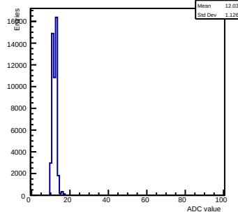
Pedestals ch 15 chip 2004 gain0-shaper6
