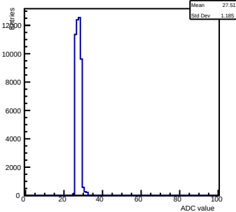
Pedestals ch 0 chip 2004 gain0-shaper6
