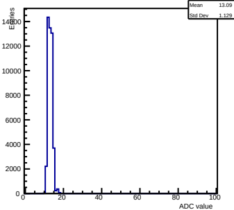
Pedestals ch 8 chip 2004 gain0-shaper6
