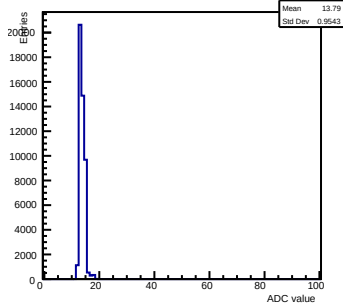
Pedestals ch 13 chip 2004 gain0-shaper6
