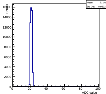
Pedestals ch 6 chip 2005 gain0-shaper6
