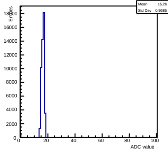
Pedestals ch 5 chip 2005 gain0-shaper6
