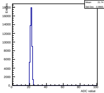
Pedestals ch 1 chip 2005 gain0-shaper6
