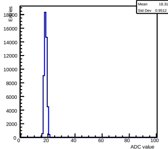
Pedestals ch 7 chip 2005 gain0-shaper6
