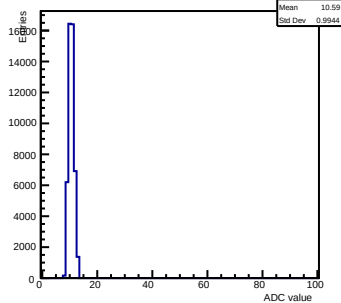
Pedestals ch 14 chip 2005 gain0-shaper6
