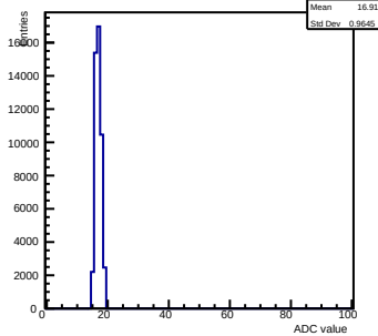
Pedestals ch 11 chip 2005 gain0-shaper6
