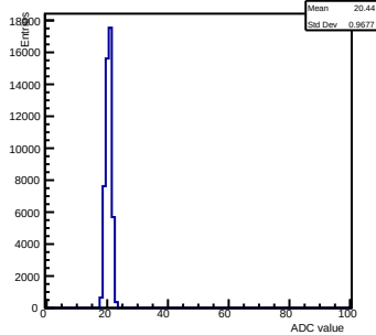
Pedestals ch 2 chip 2005 gain0-shaper6
