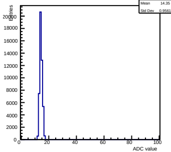
Pedestals ch 9 chip 2005 gain0-shaper6
