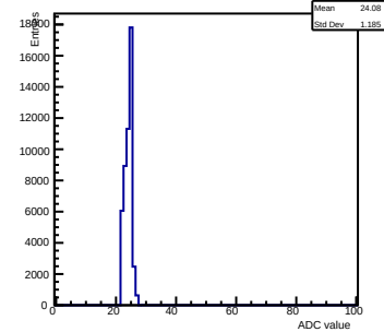
Pedestals ch 0 chip 2005 gain0-shaper6
