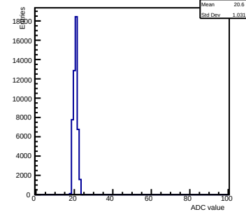
Pedestals ch 8 chip 2005 gain0-shaper6
