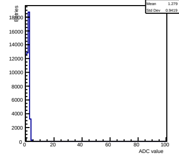
Pedestals ch 12 chip 2005 gain0-shaper6
