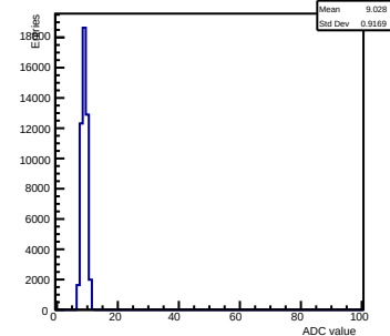
Pedestals ch 4 chip 2005 gain0-shaper6
