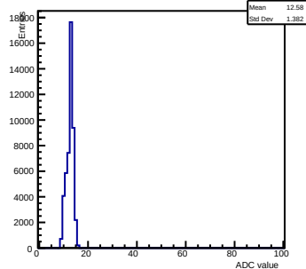
Pedestals ch 6 chip 2006 gain0-shaper0
