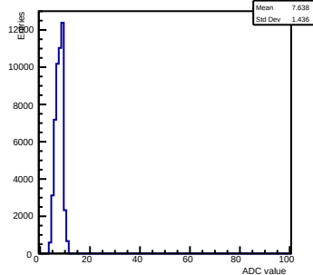
Pedestals ch 7 chip 2006 gain0-shaper0
