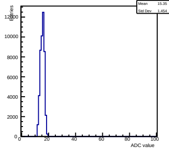
Pedestals ch 3 chip 2006 gain0-shaper0
