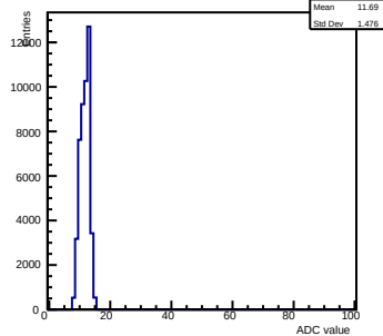
Pedestals ch 9 chip 2006 gain0-shaper0
