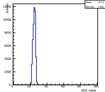
Pedestals ch 1 chip 2006 gain0-shaper0
