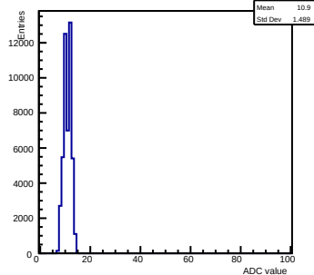
Pedestals ch 15 chip 2006 gain0-shaper0
