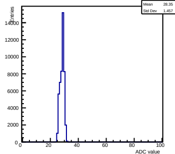
Pedestals ch 5 chip 2006 gain0-shaper0
