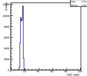
Pedestals ch 10 chip 2006 gain0-shaper0
