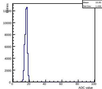
Pedestals ch 14 chip 2006 gain0-shaper0
