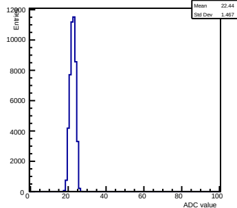
Pedestals ch 13 chip 2006 gain0-shaper0
