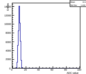
Pedestals ch 4 chip 2006 gain0-shaper0
