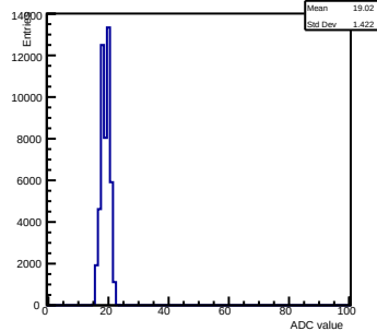
Pedestals ch 2 chip 2006 gain0-shaper0
