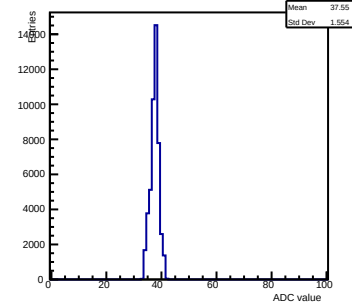
Pedestals ch 0 chip 2006 gain0-shaper0
