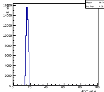
Pedestals ch 14 chip 2006 gain0-shaper6
