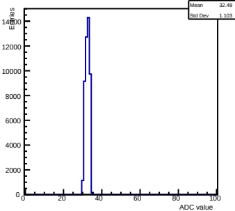
Pedestals ch 0 chip 2006 gain0-shaper6
