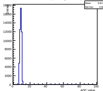
Pedestals ch 6 chip 2006 gain0-shaper6
