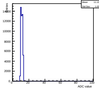
Pedestals ch 3 chip 2006 gain0-shaper6
