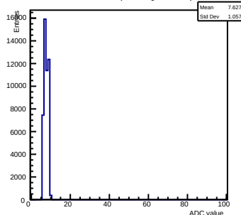
Pedestals ch 7 chip 2006 gain0-shaper6
