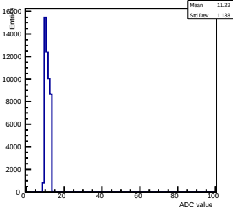
Pedestals ch 9 chip 2006 gain0-shaper6
