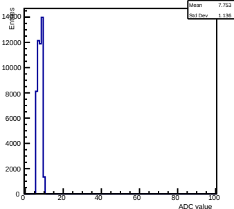
Pedestals ch 8 chip 2006 gain0-shaper6
