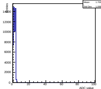
Pedestals ch 11 chip 2006 gain0-shaper6
