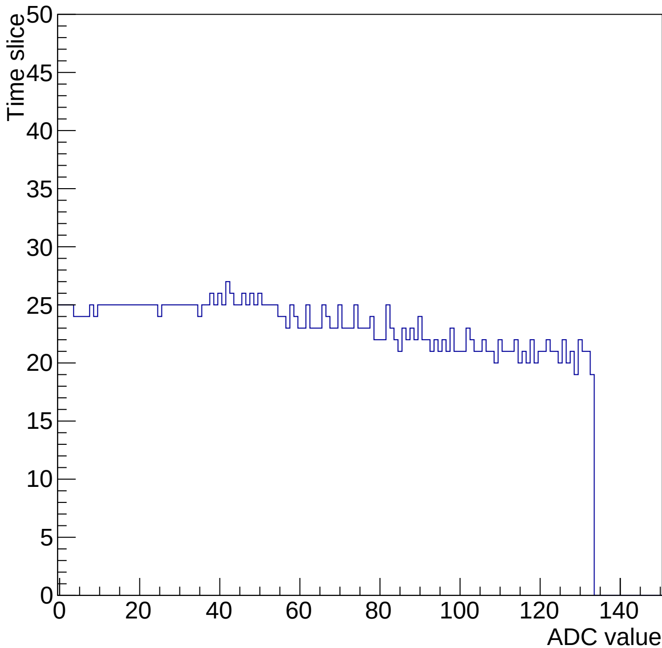
Evt 10 Time mcm 2000 chip 0 chan 14 34643-gain0-shaper0
