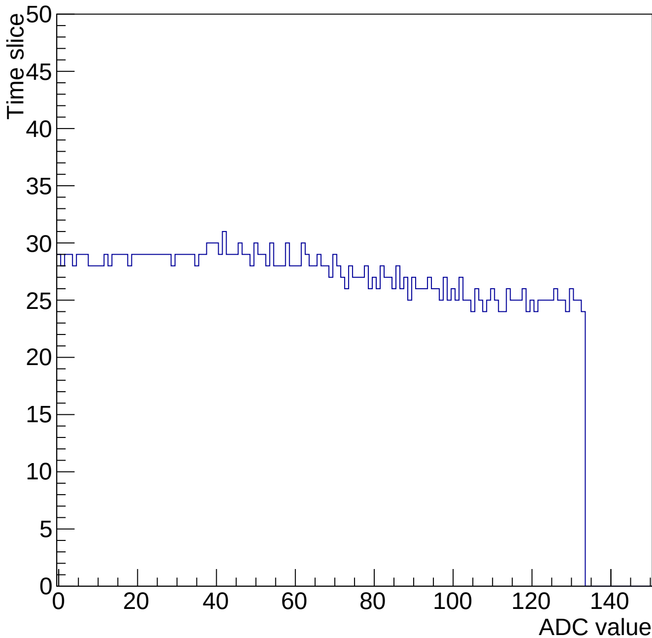
Evt 10 Time mcm 2000 chip 0 chan 12 34643-gain0-shaper0
