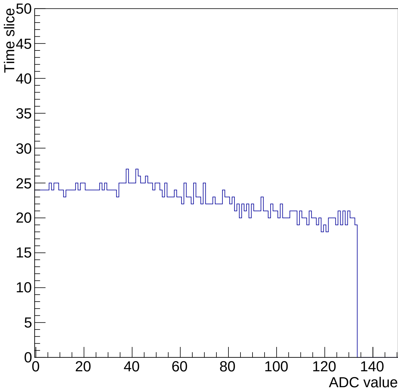
Evt 10 Time mcm 2000 chip 0 chan 4 34643-gain0-shaper0
