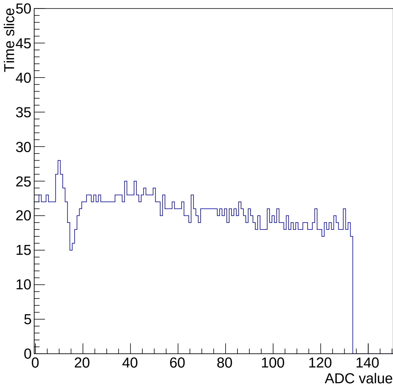
Evt 10 Time mcm 2000 chip 0 chan 2 34643-gain0-shaper0
