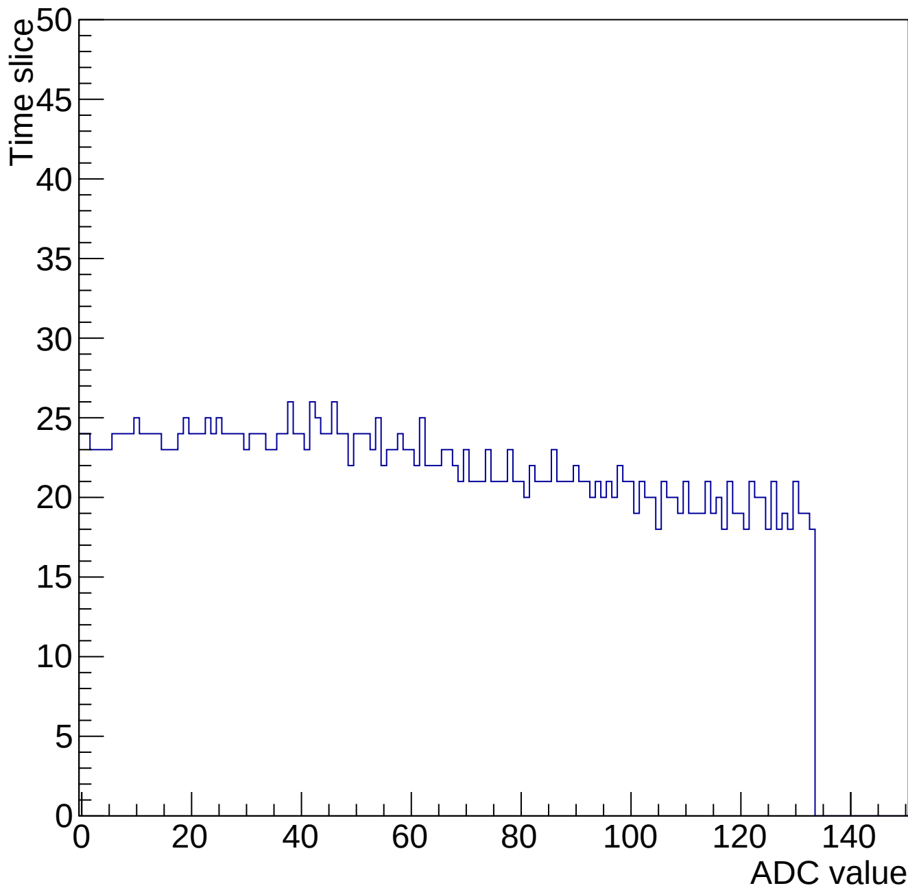
Evt 10 Time mcm 2000 chip 0 chan 3 34643-gain0-shaper0
