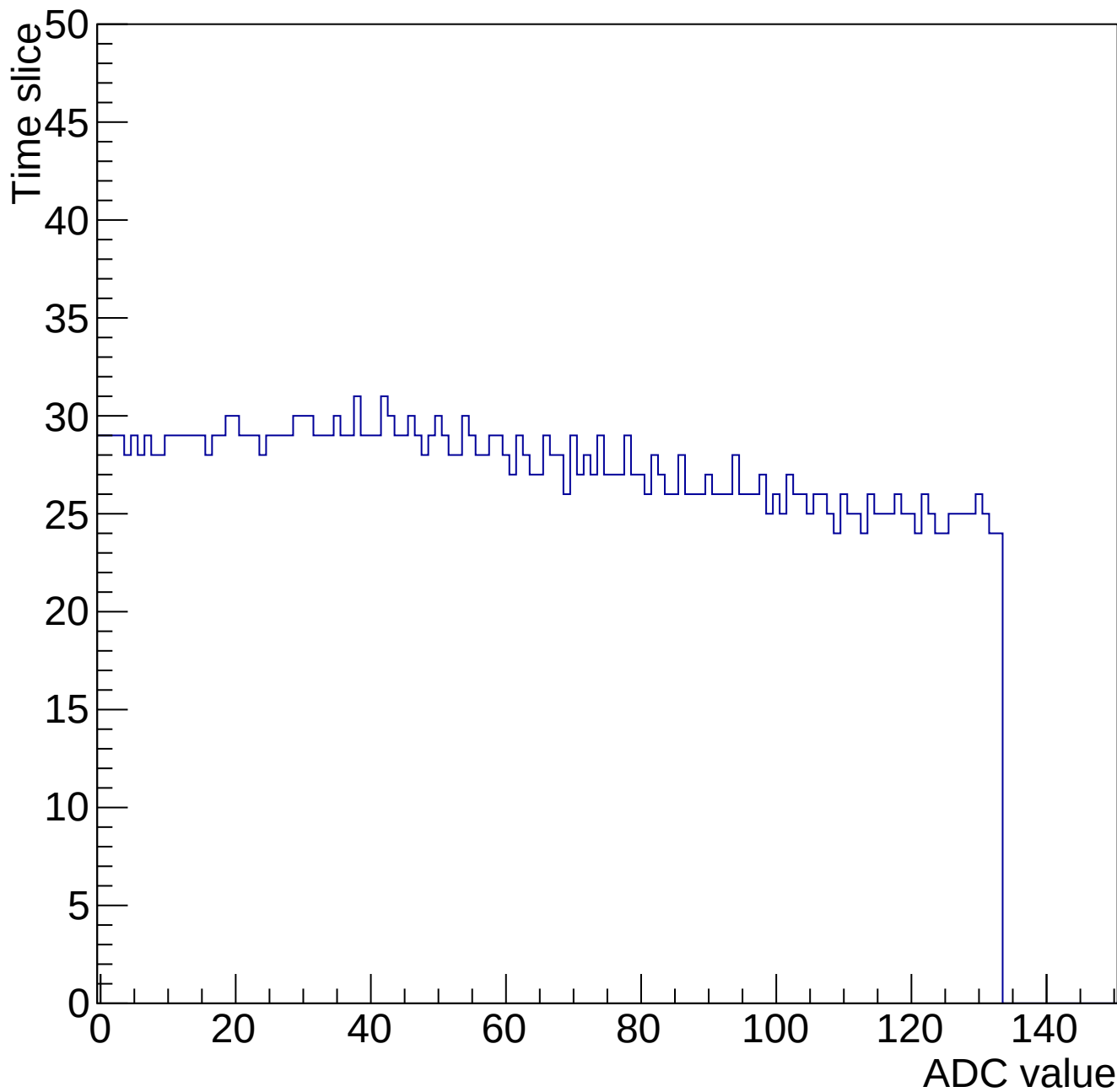
Evt 10 Time mcm 2000 chip 0 chan 13 34643-gain0-shaper0
