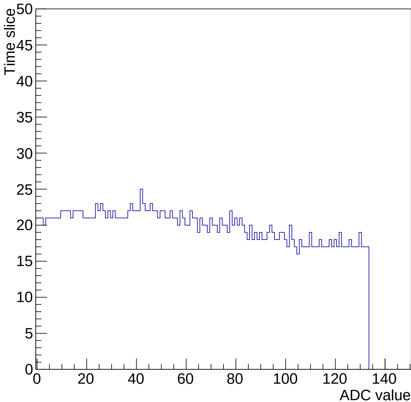
Evt 10 Time mcm 2000 chip 0 chan 11 34643-gain0-shaper0
