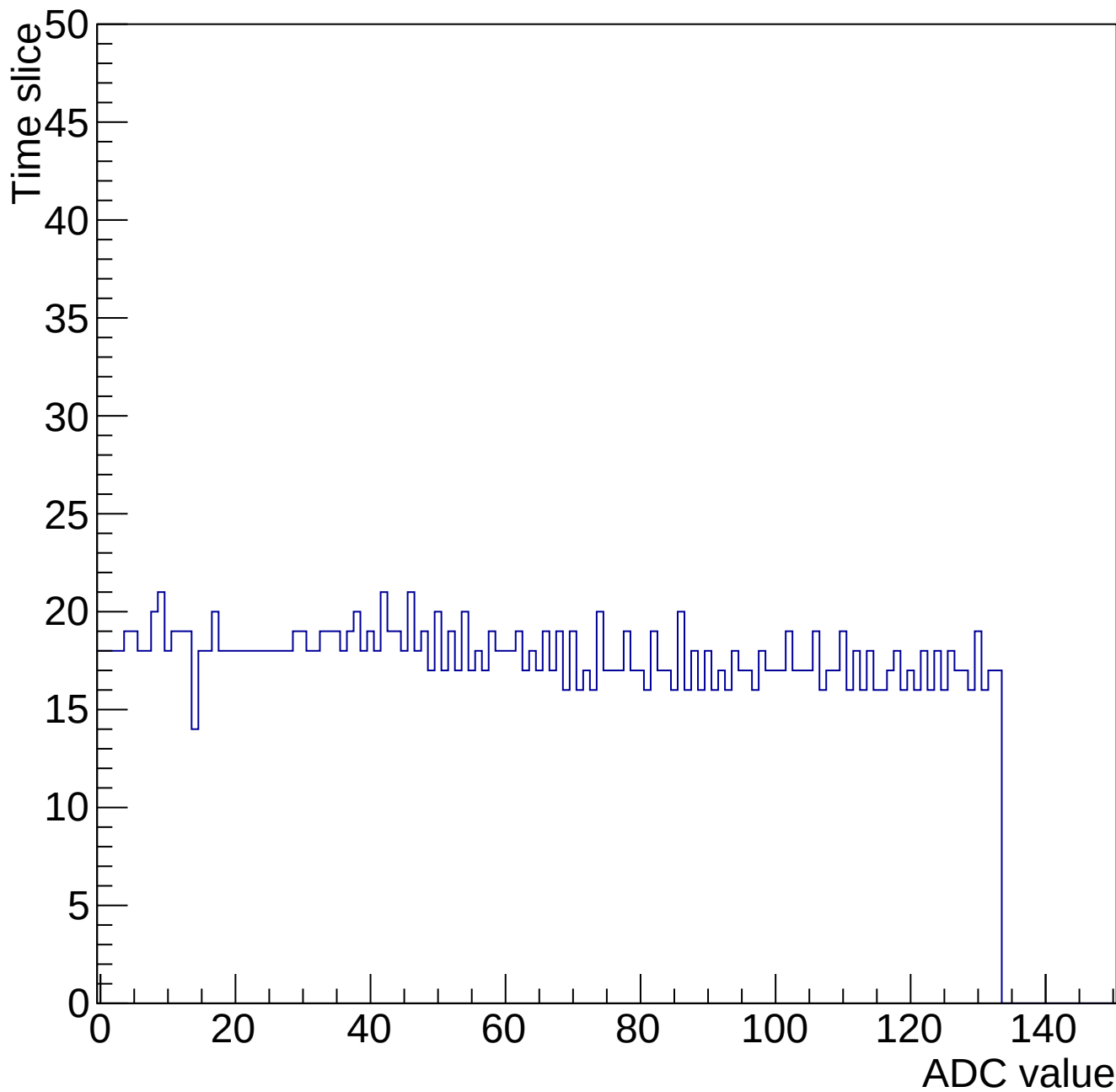
Evt 10 Time mcm 2000 chip 0 chan 2 34667-gain0-shaper6
