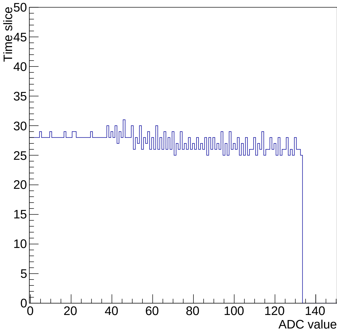
Evt 10 Time mcm 2000 chip 0 chan 5 34667-gain0-shaper6
