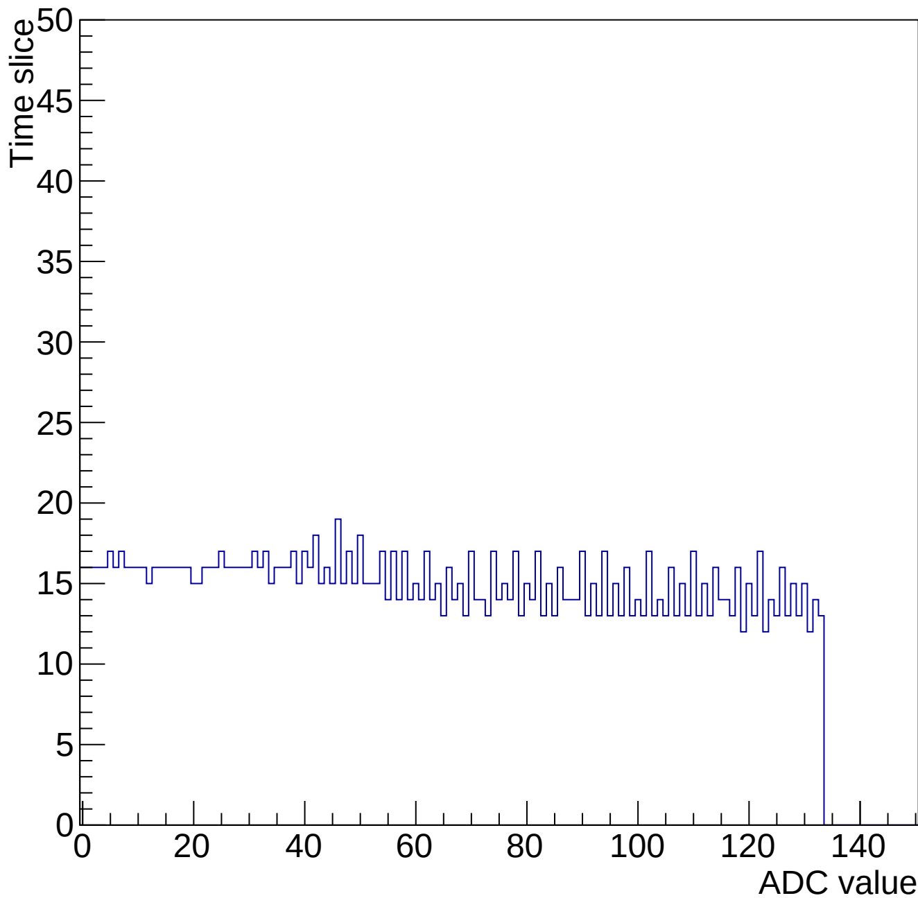
Evt 10 Time mcm 2000 chip 0 chan 10 34667-gain0-shaper6
