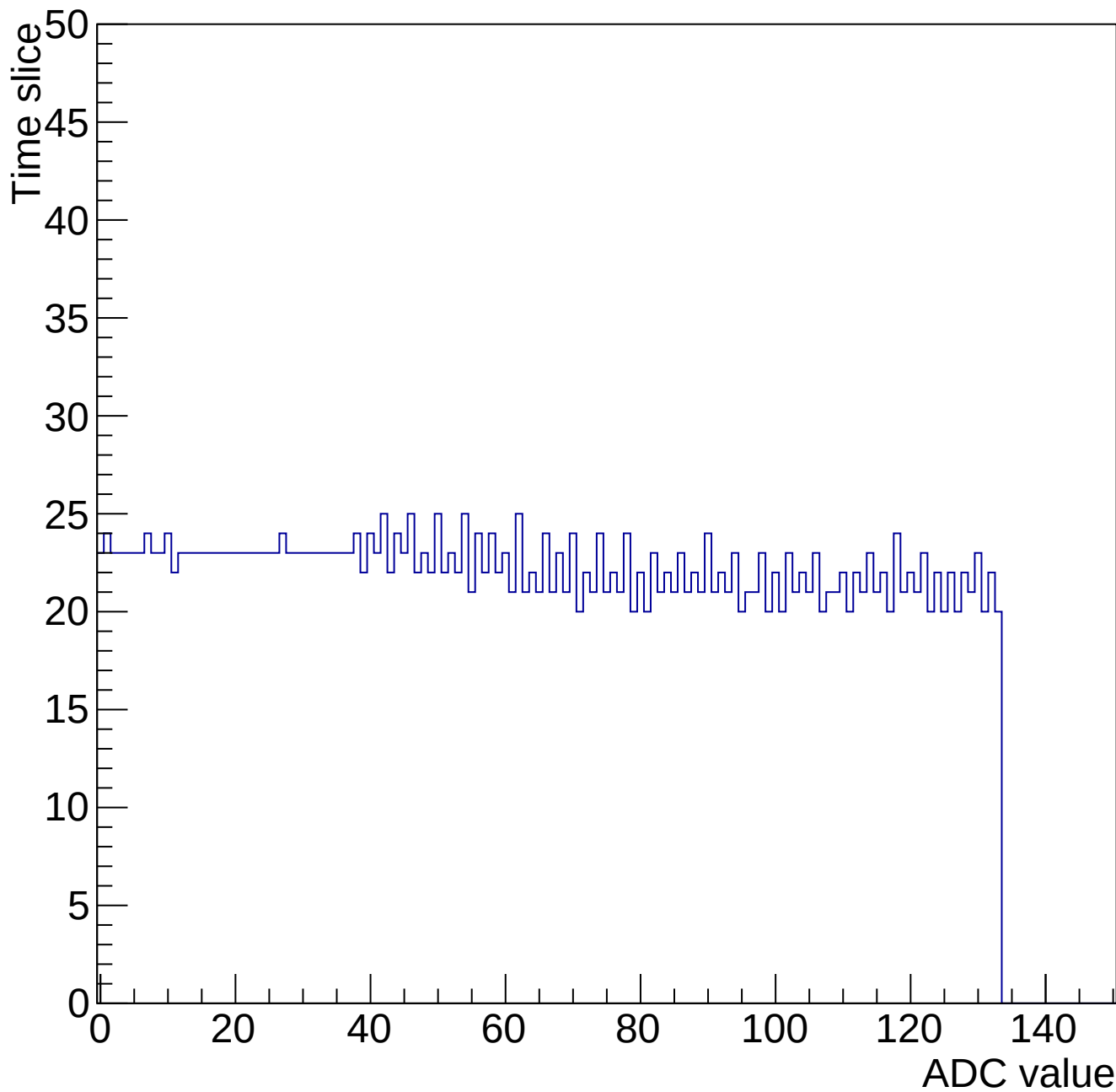
Evt 10 Time mcm 2000 chip 0 chan 13 34667-gain0-shaper6
