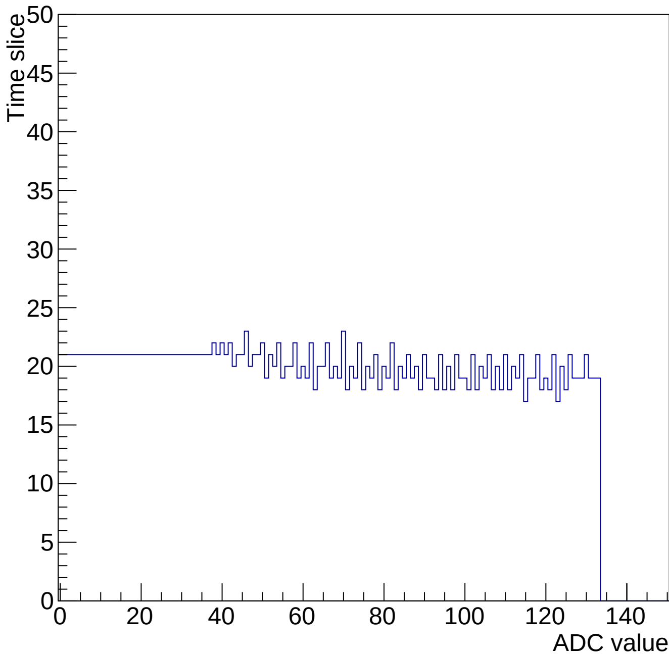
Evt 10 Time mcm 2000 chip 0 chan 11 34667-gain0-shaper6
