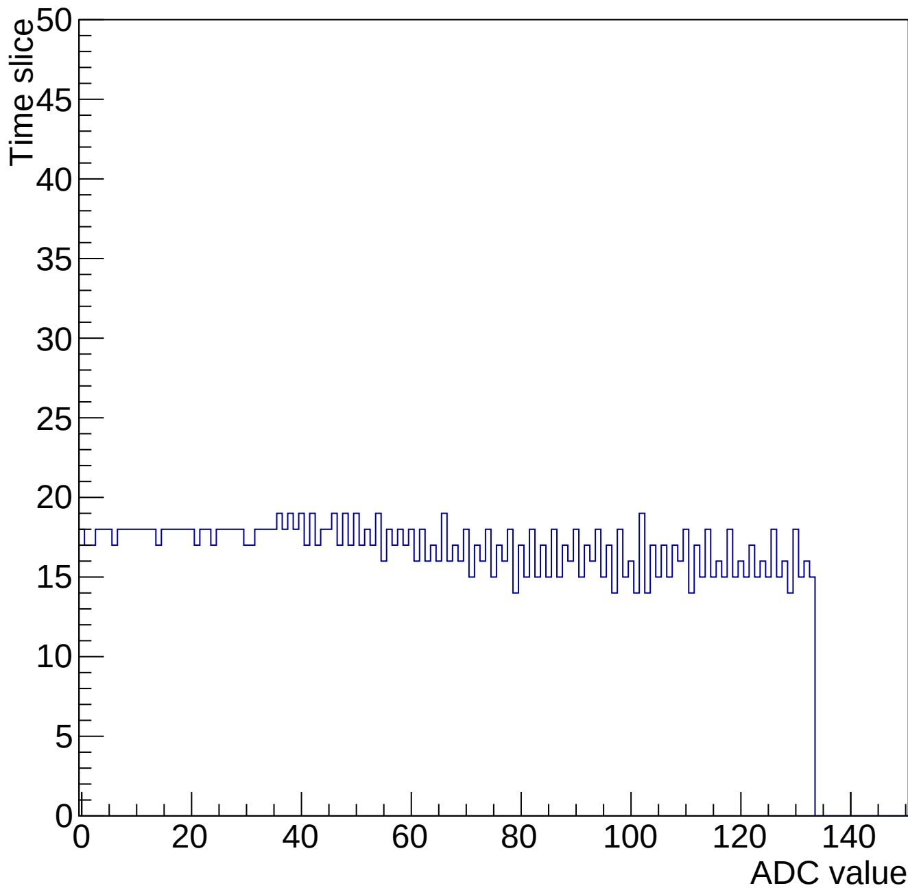
Evt 10 Time mcm 2000 chip 0 chan 15 34667-gain0-shaper6
