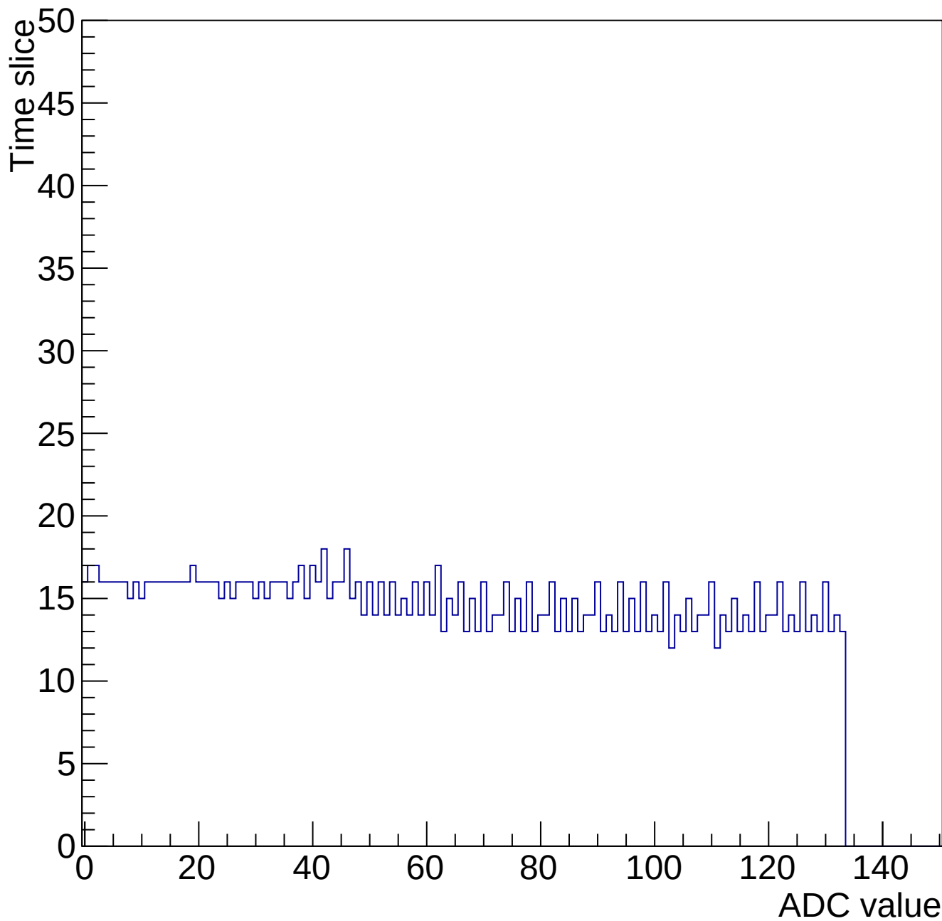
Evt 10 Time mcm 2000 chip 0 chan 6 34667-gain0-shaper6
