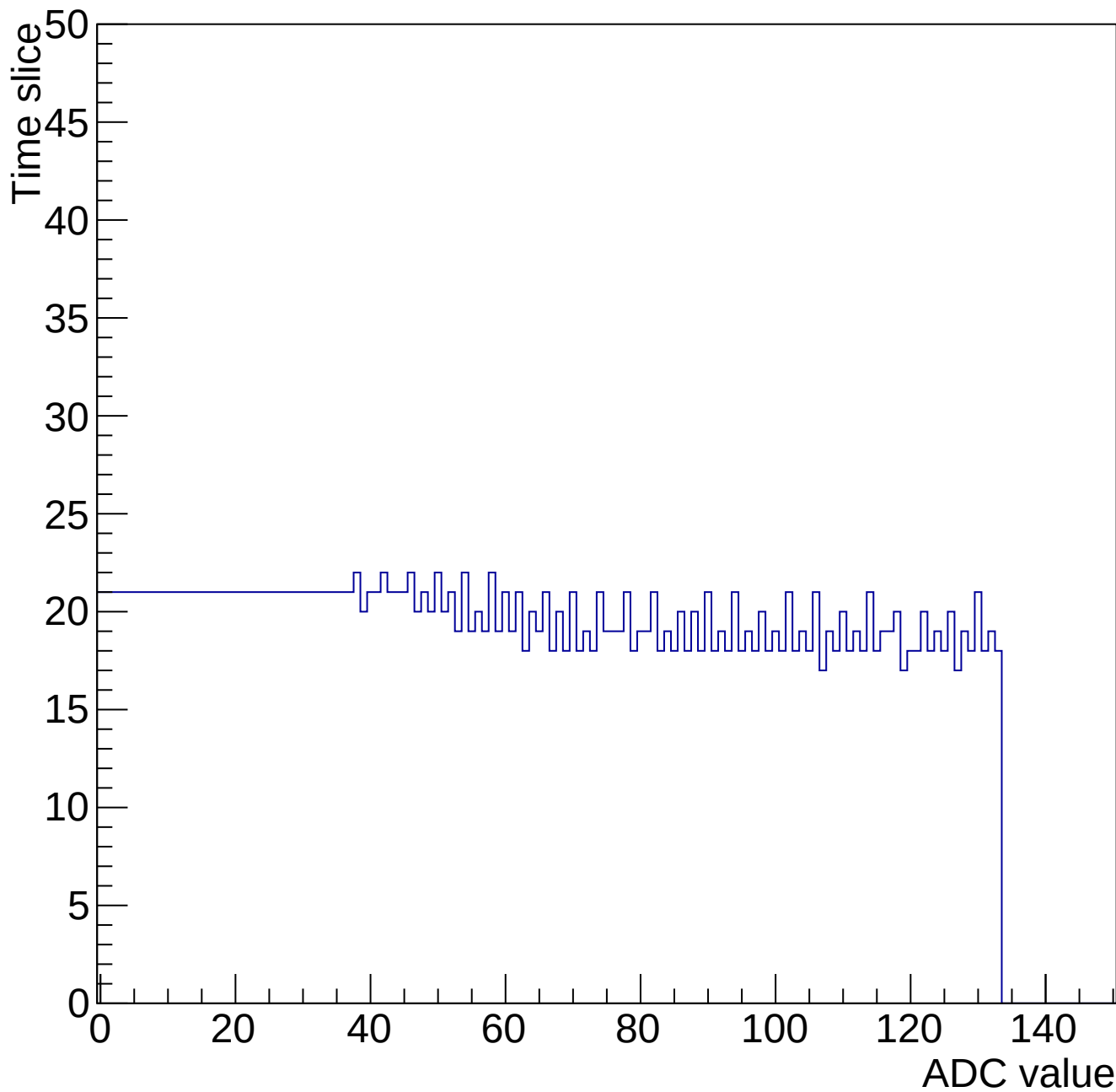
Evt 10 Time mcm 2000 chip 0 chan 14 34667-gain0-shaper6
