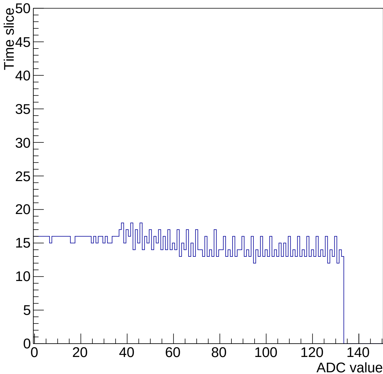
Evt 10 Time mcm 2000 chip 0 chan 9 34667-gain0-shaper6
