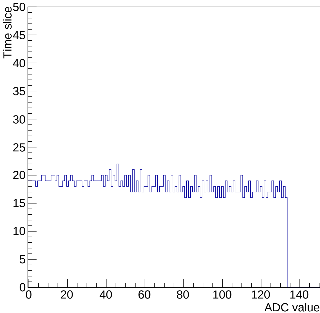
Evt 10 Time mcm 2000 chip 0 chan 3 34667-gain0-shaper6
