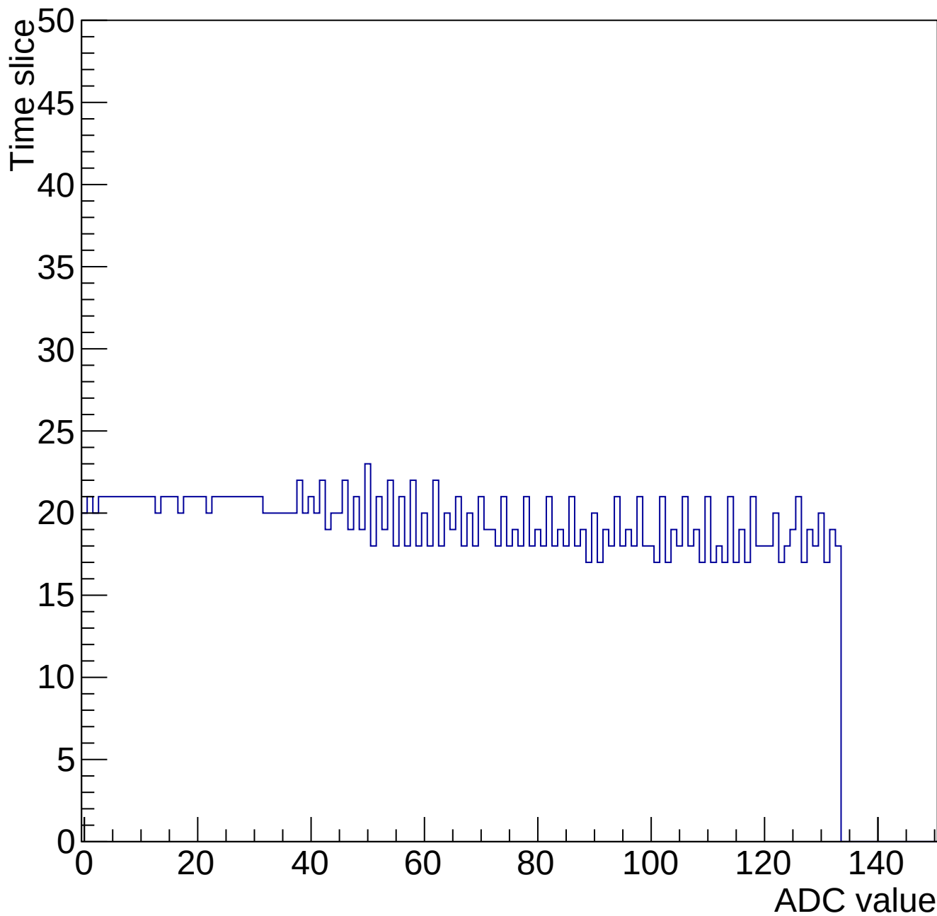
Evt 10 Time mcm 2000 chip 0 chan 4 34667-gain0-shaper6
