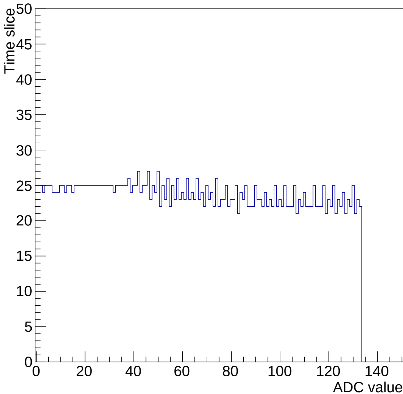
Evt 10 Time mcm 2000 chip 0 chan 8 34667-gain0-shaper6
