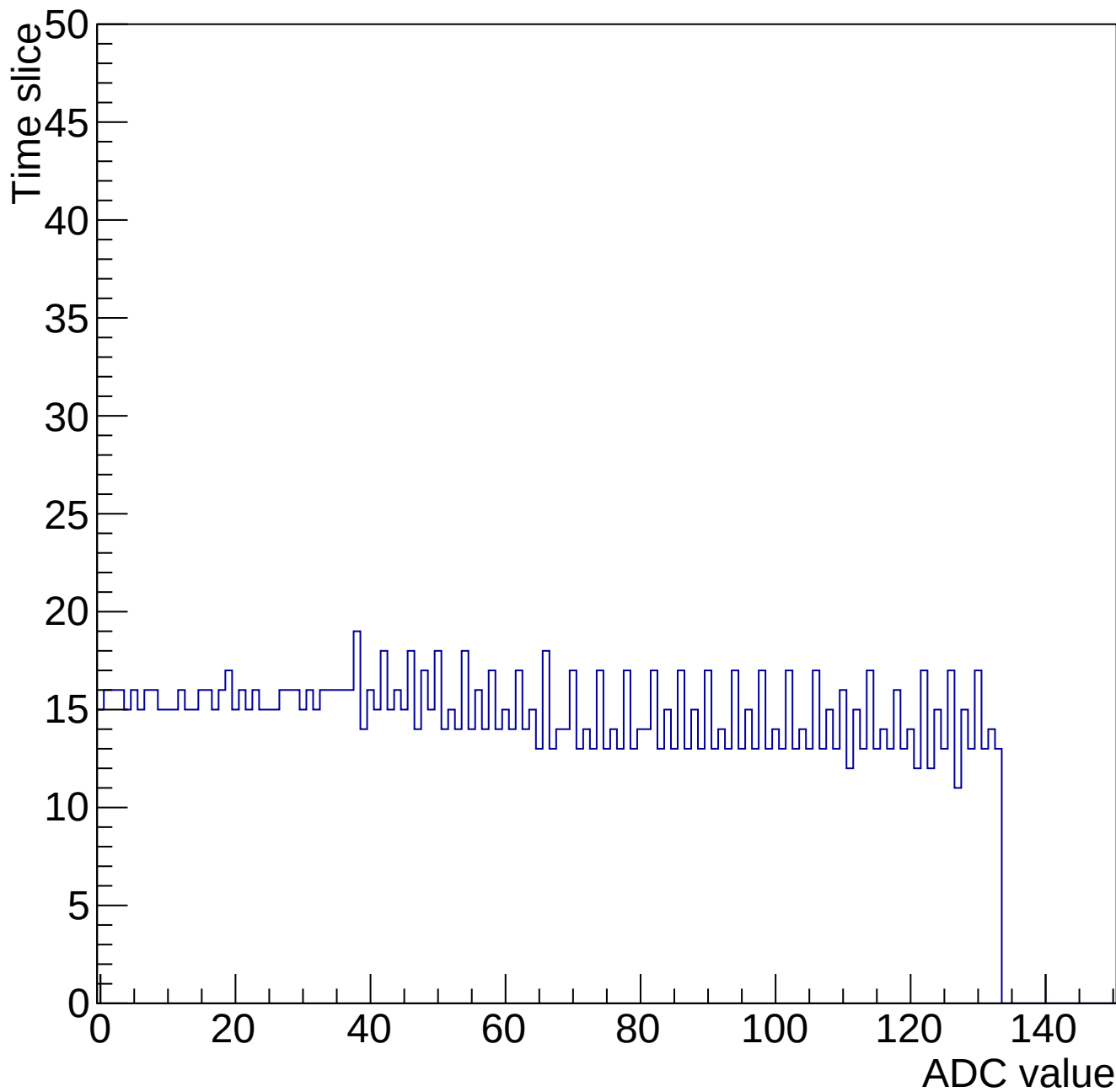
Evt 10 Time mcm 2000 chip 0 chan 0 34667-gain0-shaper6
