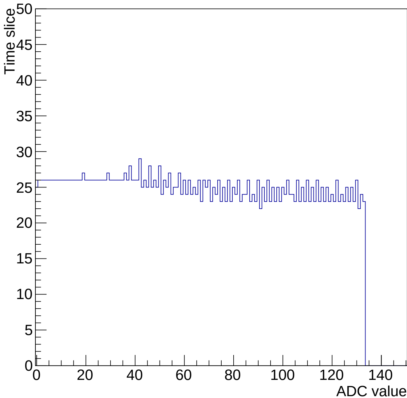
Evt 10 Time mcm 2000 chip 0 chan 12 34667-gain0-shaper6
