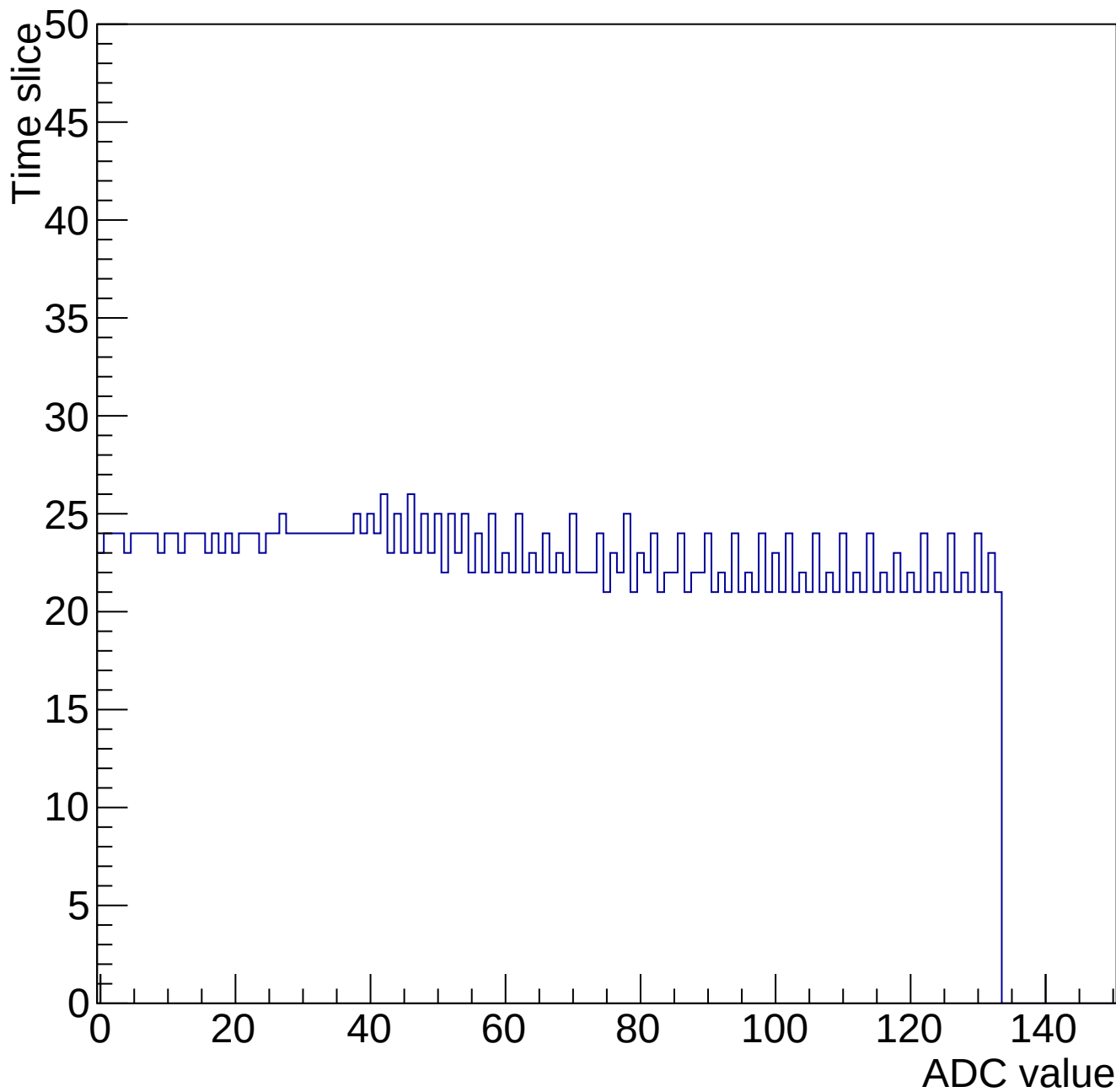
Evt 10 Time mcm 2000 chip 0 chan 7 34667-gain0-shaper6
