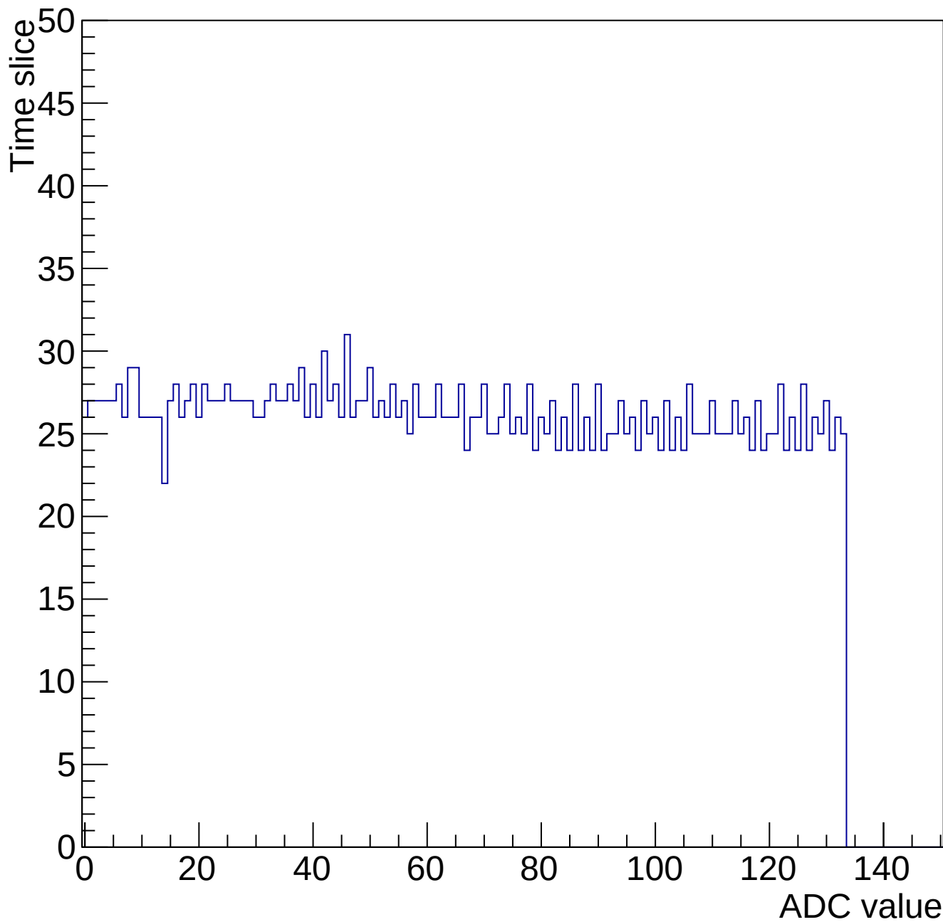
Evt 10 Time mcm 2000 chip 0 chan 1 34667-gain0-shaper6
