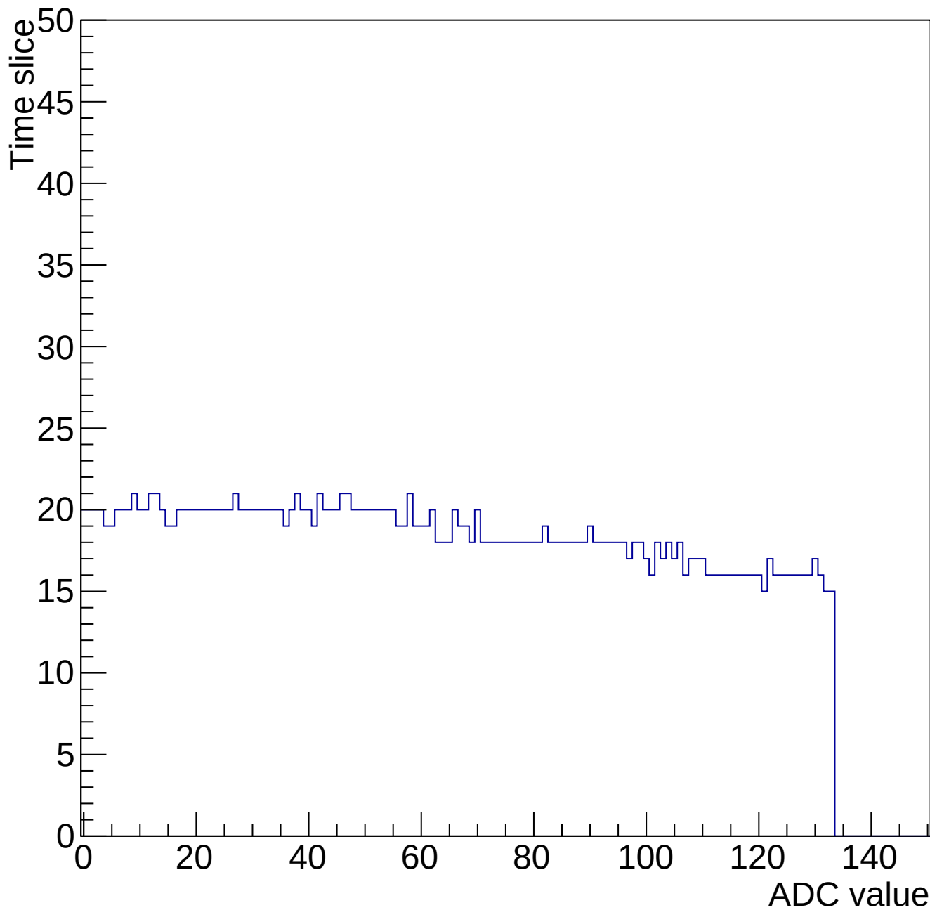
Evt 10 Time mcm 2001 chip 1 chan 9 34645-gain0-shaper0
