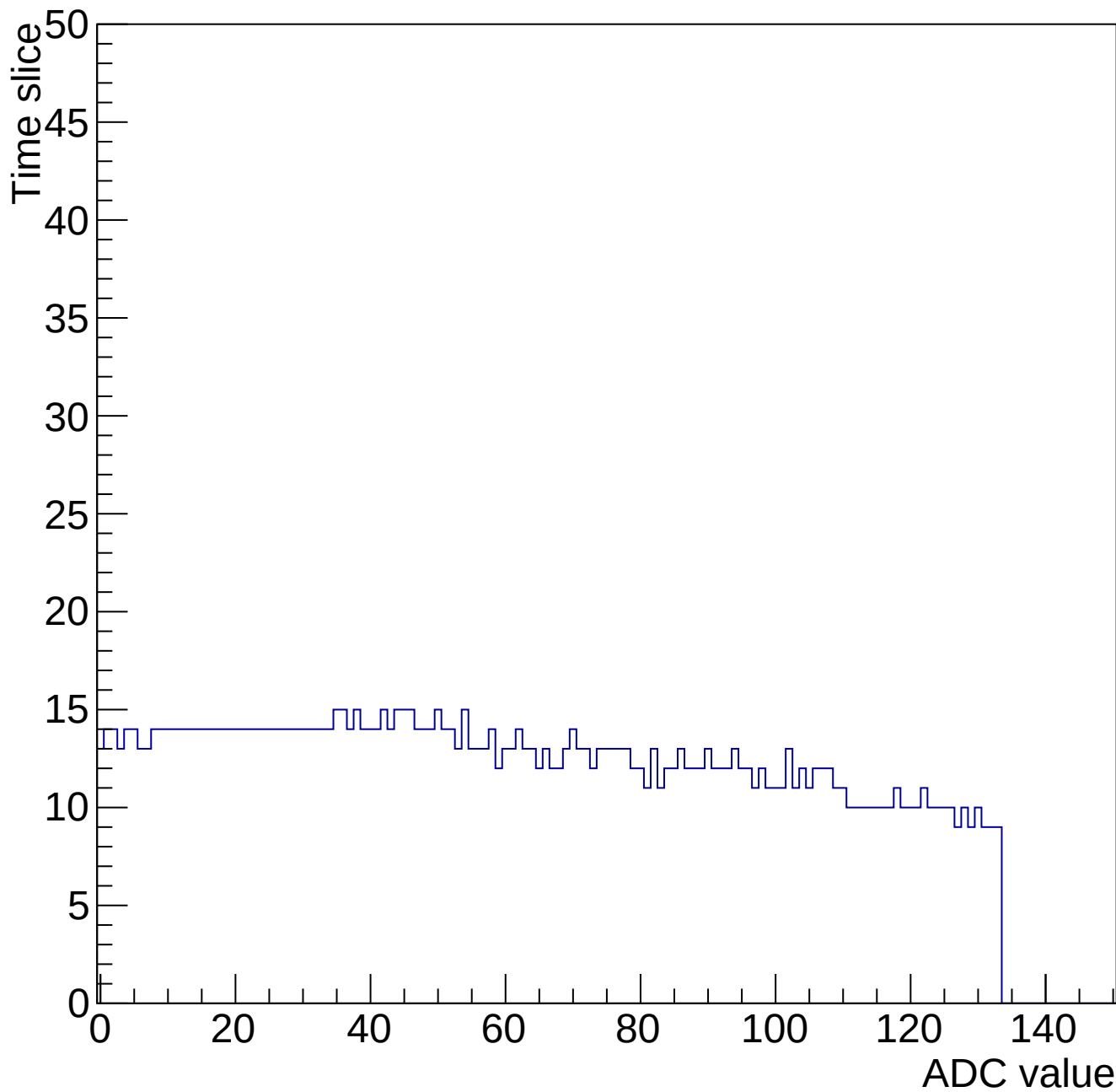
Evt 10 Time mcm 2001 chip 1 chan 7 34645-gain0-shaper0
