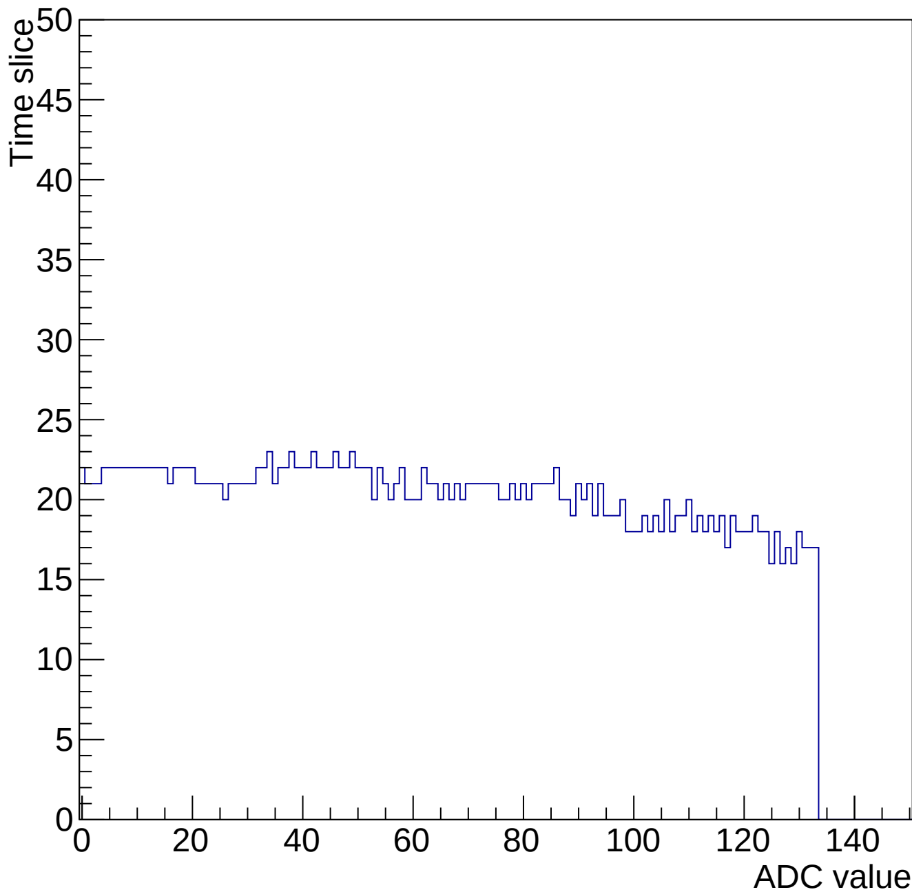
Evt 10 Time mcm 2001 chip 1 chan 12 34645-gain0-shaper0
