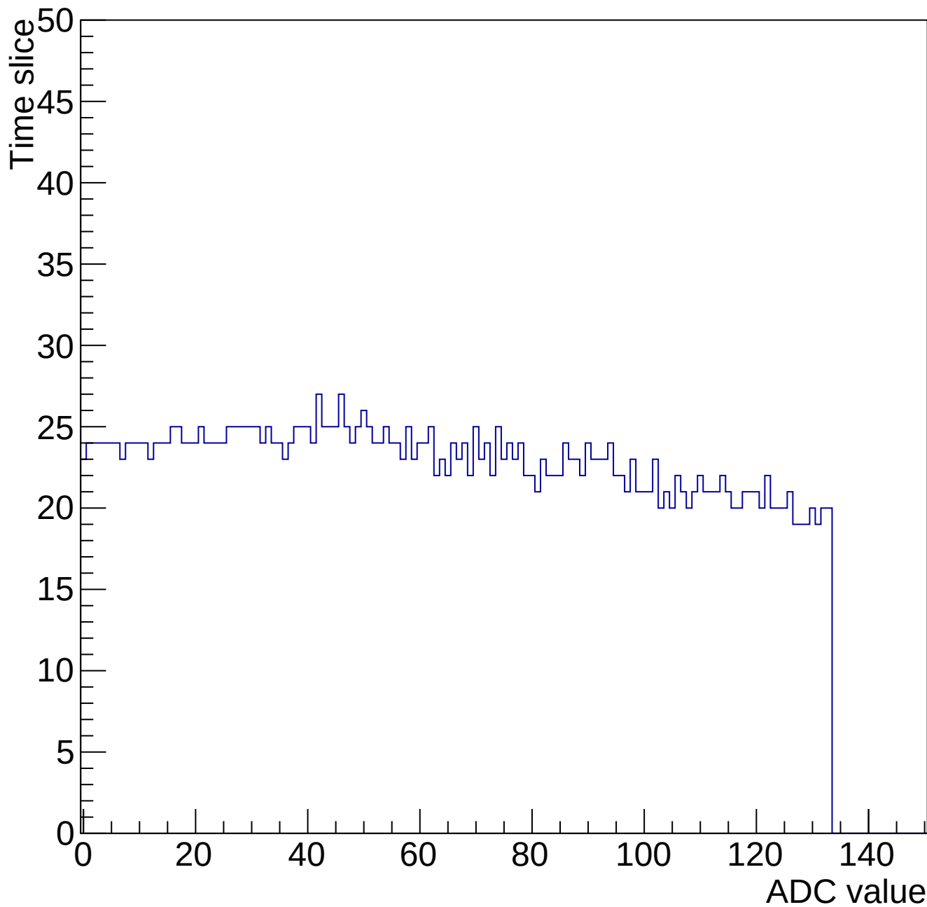
Evt 10 Time mcm 2001 chip 1 chan 0 34645-gain0-shaper0
