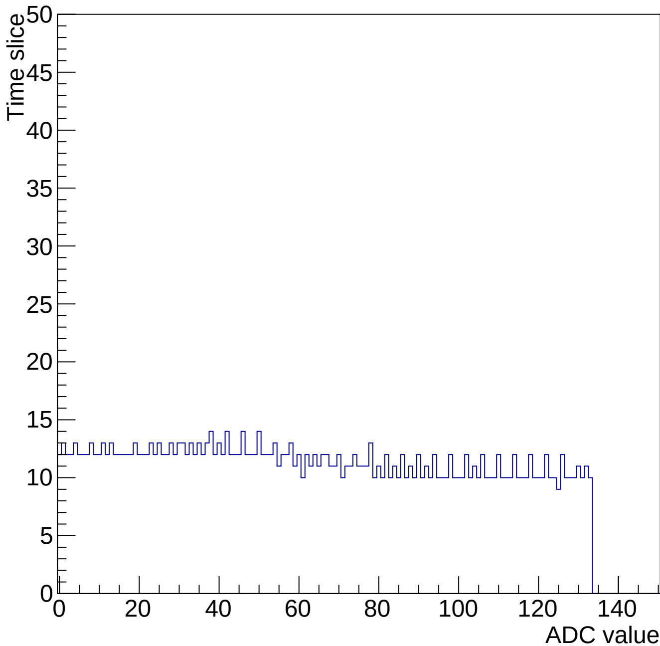
Evt 10 Time mcm 2001 chip 1 chan 1 34660-gain0-shaper6
