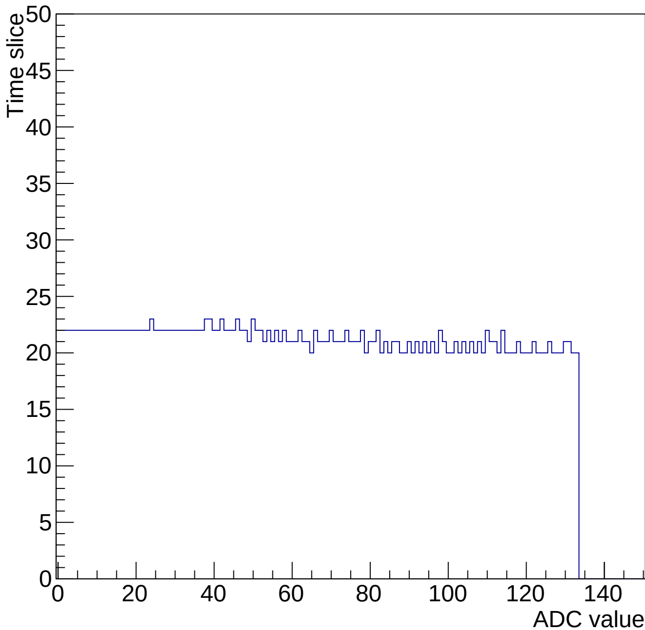
Evt 10 Time mcm 2001 chip 1 chan 11 34660-gain0-shaper6
