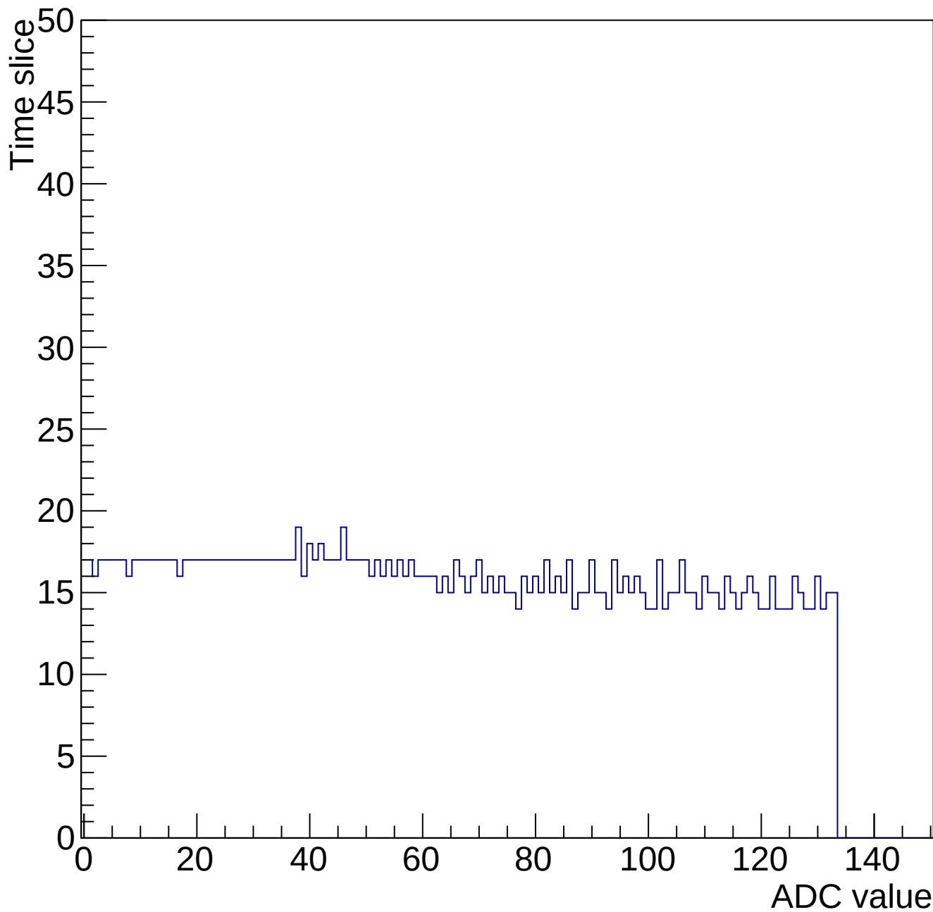
Evt 10 Time mcm 2001 chip 1 chan 12 34660-gain0-shaper6
