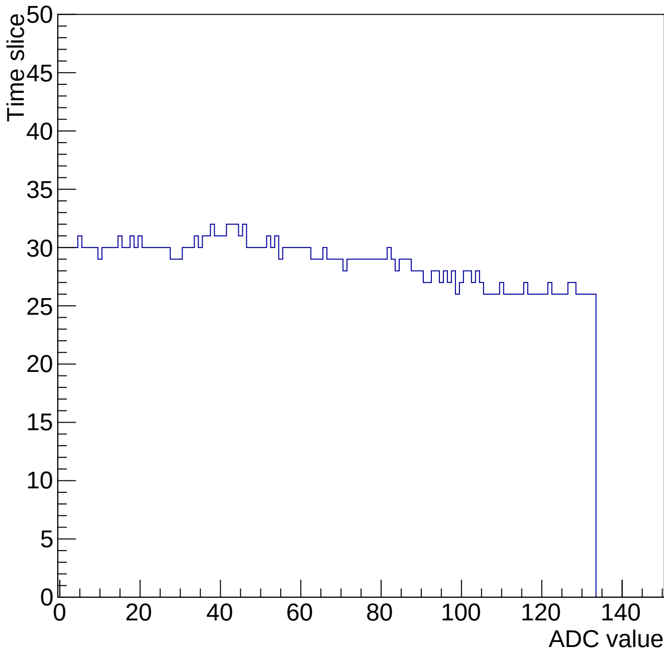
Evt 10 Time mcm 2002 chip 2 chan 4 34647-gain0-shaper0
