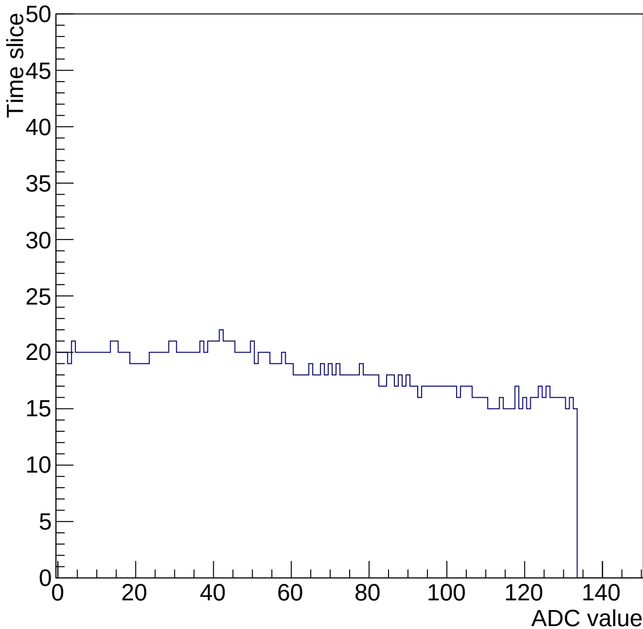
Evt 10 Time mcm 2002 chip 2 chan 9 34647-gain0-shaper0
