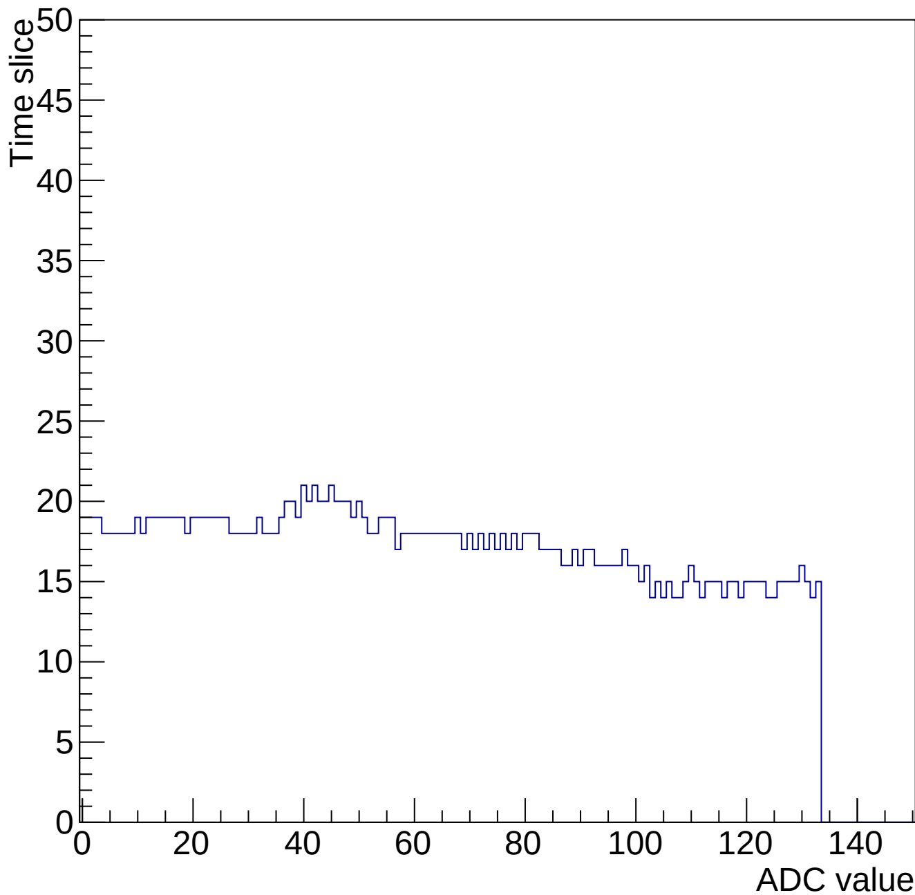
Evt 10 Time mcm 2002 chip 2 chan 6 34647-gain0-shaper0
