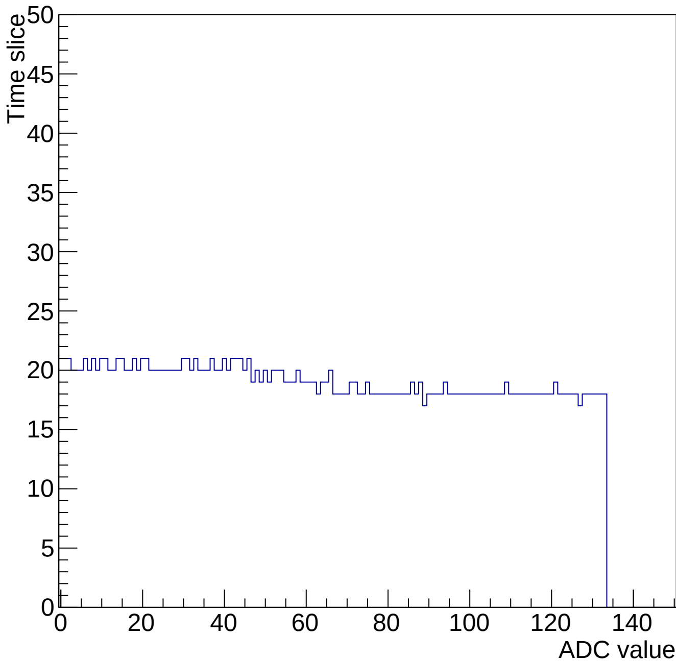
Evt 10 Time mcm 2002 chip 2 chan 13 34661-gain0-shaper6
