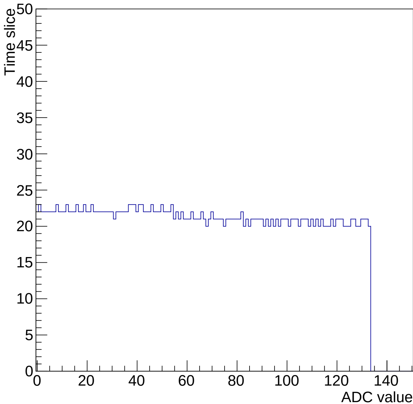
Evt 10 Time mcm 2002 chip 2 chan 0 34661-gain0-shaper6
