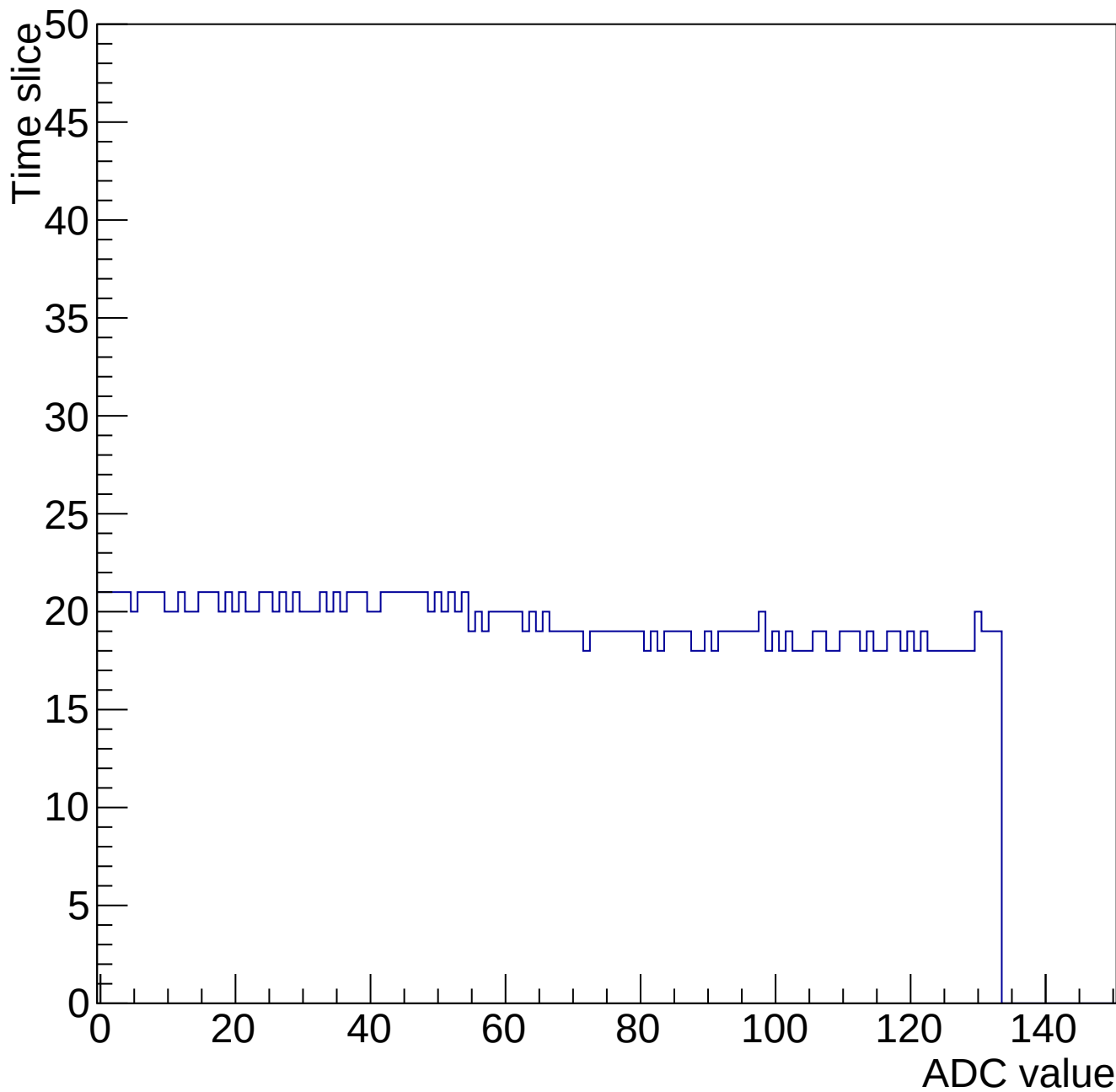
Evt 10 Time mcm 2002 chip 2 chan 11 34661-gain0-shaper6
