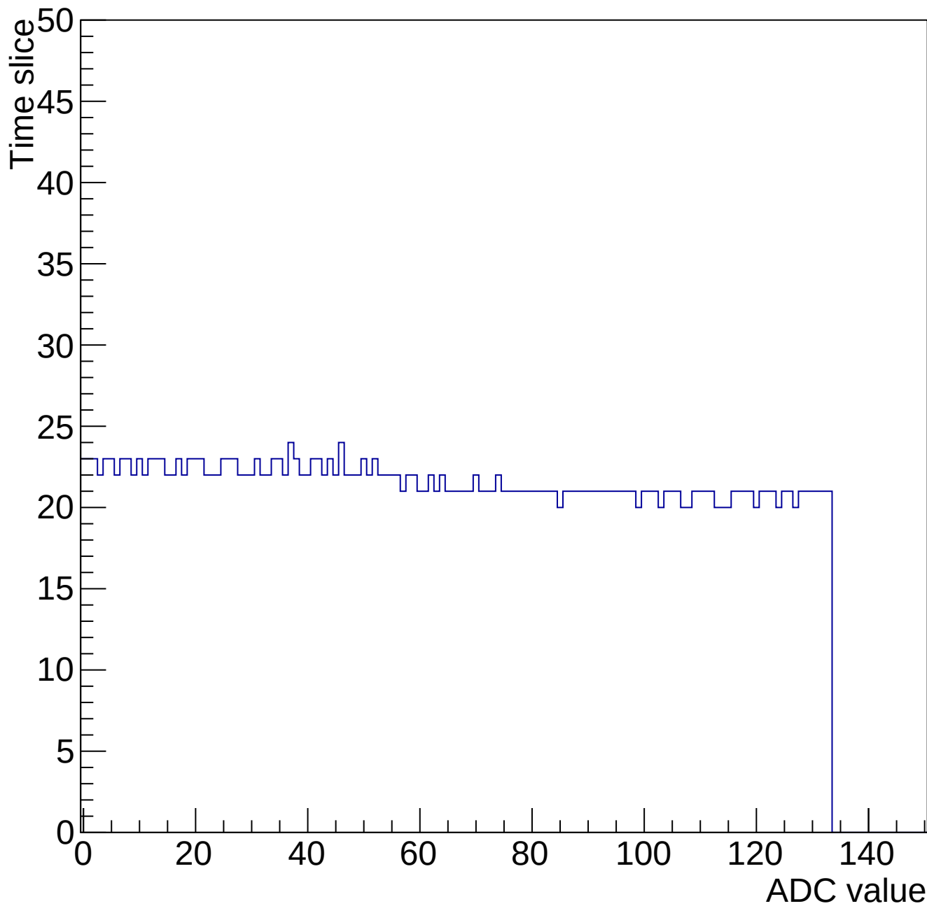
Evt 10 Time mcm 2002 chip 2 chan 5 34661-gain0-shaper6
