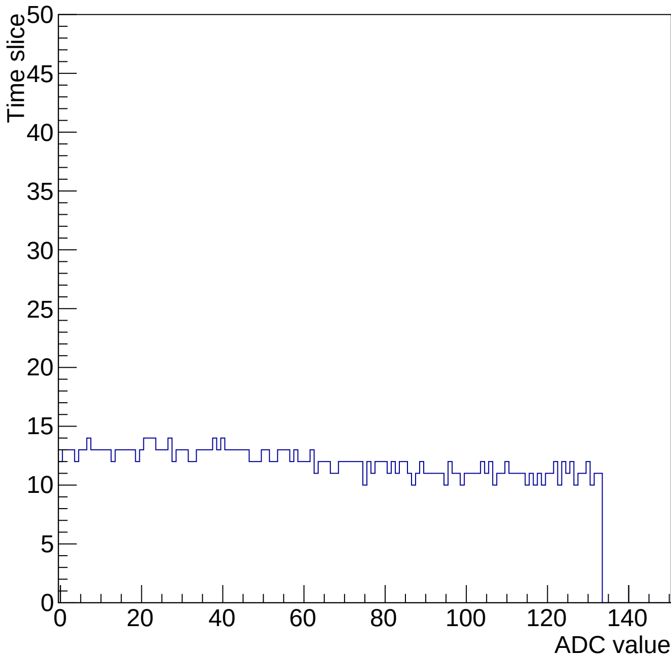
Evt 10 Time mcm 2002 chip 2 chan 1 34661-gain0-shaper6
