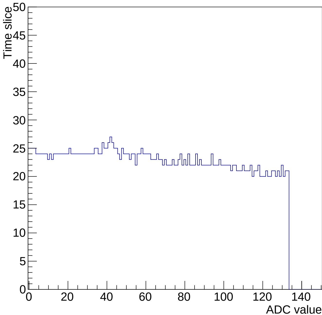
Evt 10 Time mcm 2003 chip 3 chan 2 34649-gain0-shaper0
