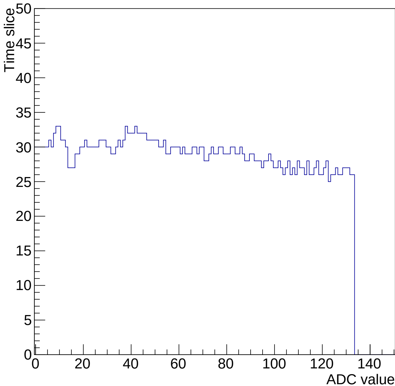
Evt 10 Time mcm 2003 chip 3 chan 0 34649-gain0-shaper0
