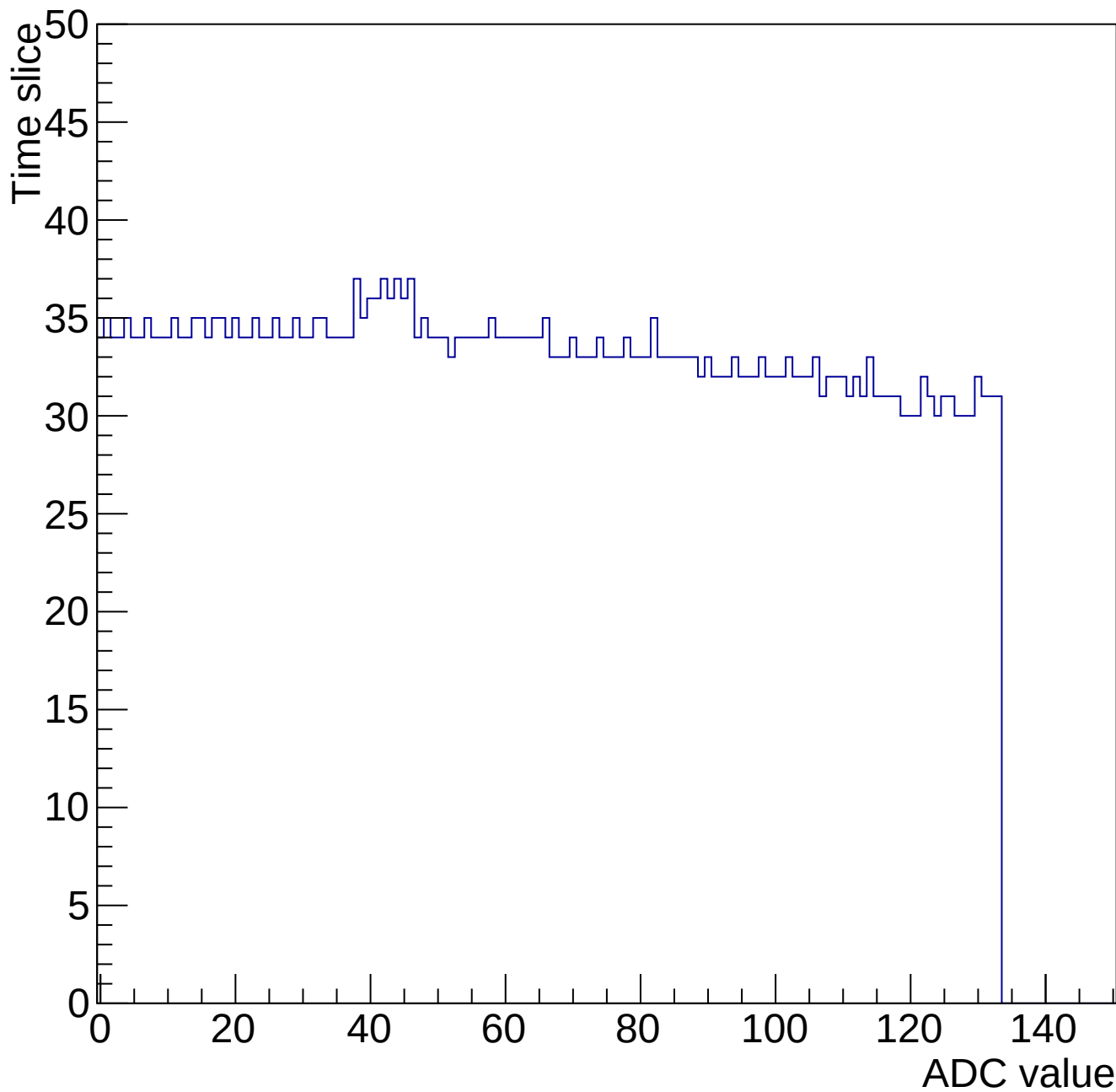
Evt 10 Time mcm 2003 chip 3 chan 4 34649-gain0-shaper0
