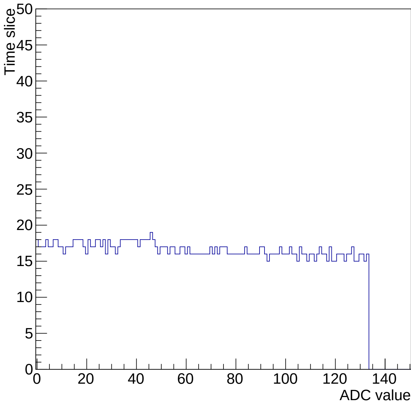
Evt 10 Time mcm 2005 chip 5 chan 10 34664-gain0-shaper6
