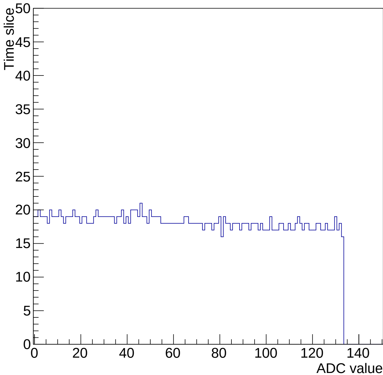
Evt 10 Time mcm 2005 chip 5 chan 7 34664-gain0-shaper6
