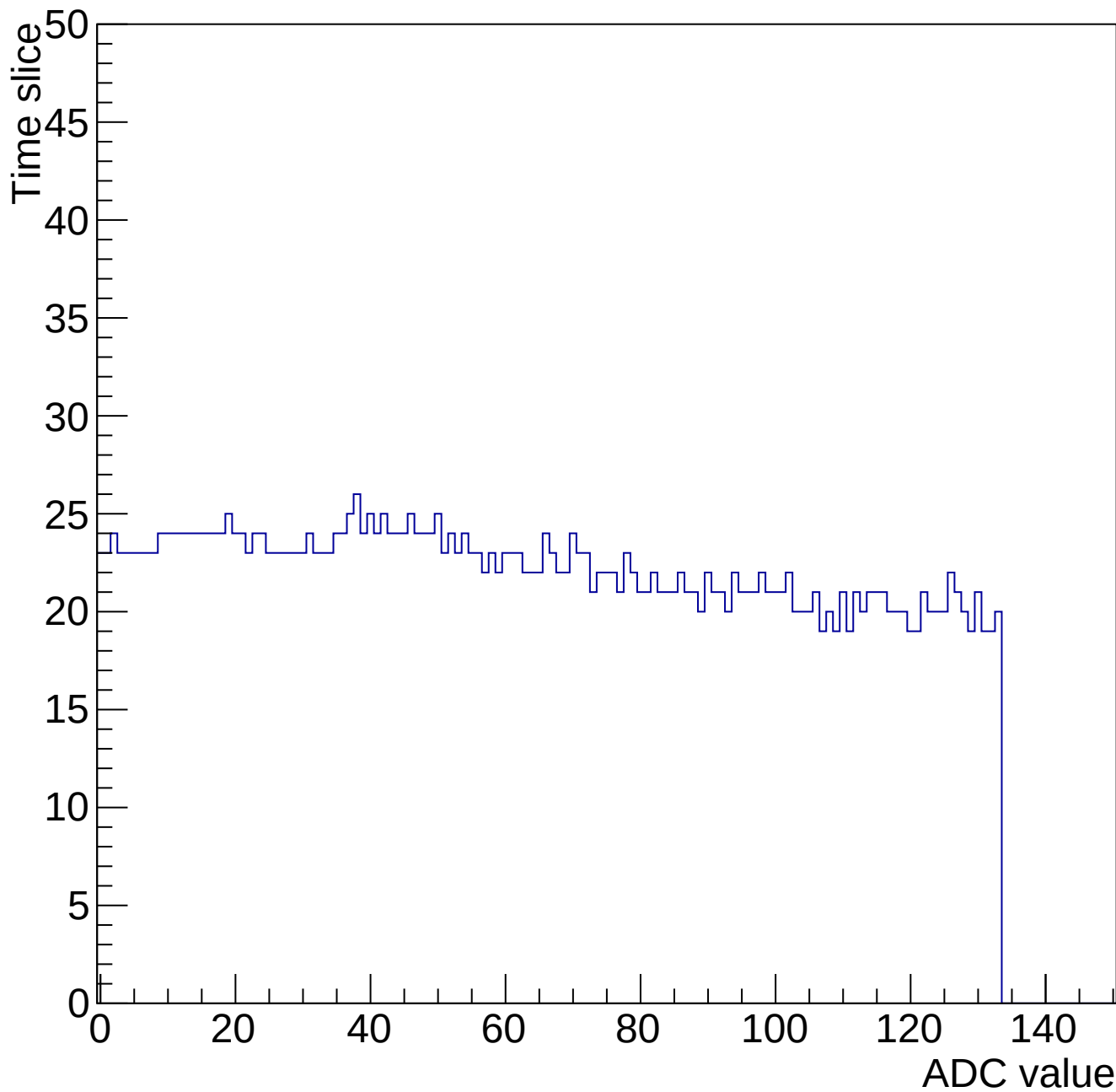
Evt 10 Time mcm 2007 chip 7 chan 3 34656-gain0-shaper0
