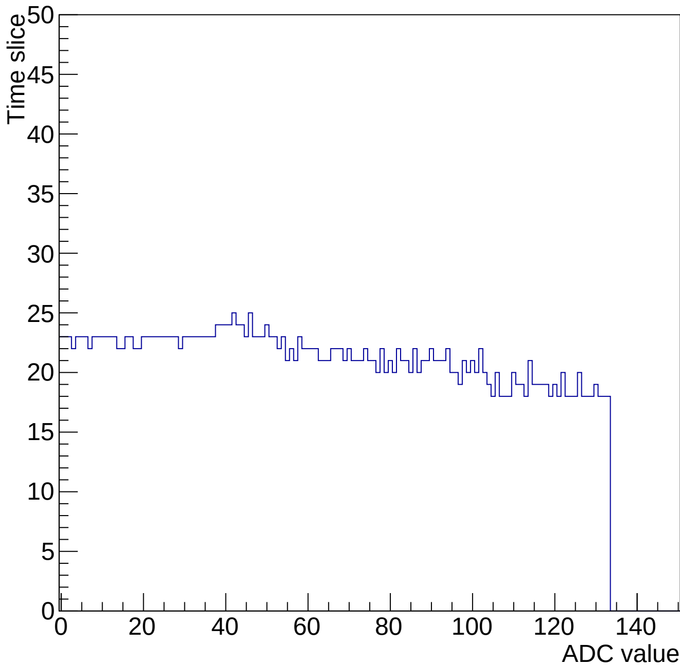
Evt 10 Time mcm 2007 chip 7 chan 10 34656-gain0-shaper0
