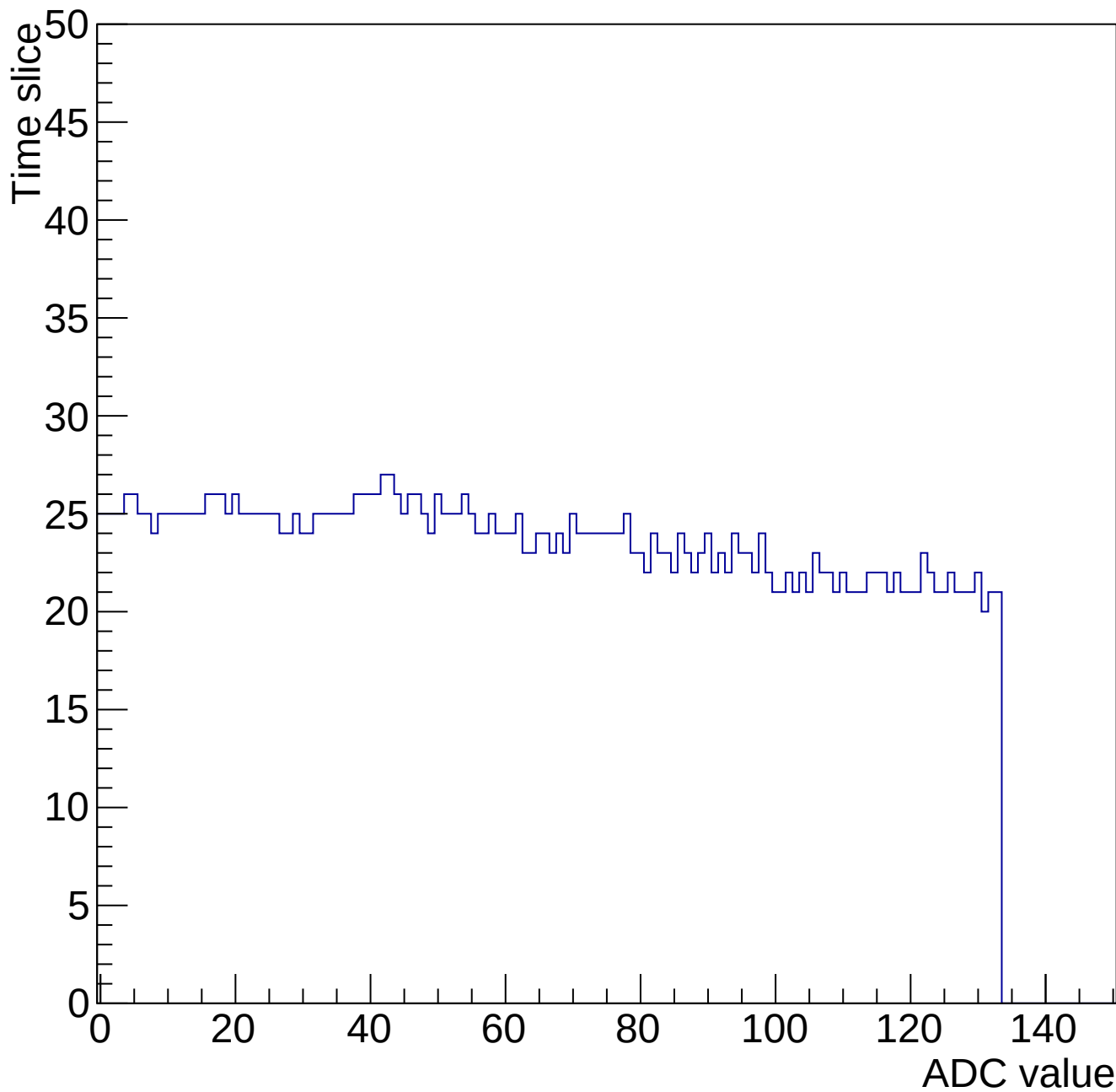
Evt 10 Time mcm 2007 chip 7 chan 6 34656-gain0-shaper0
