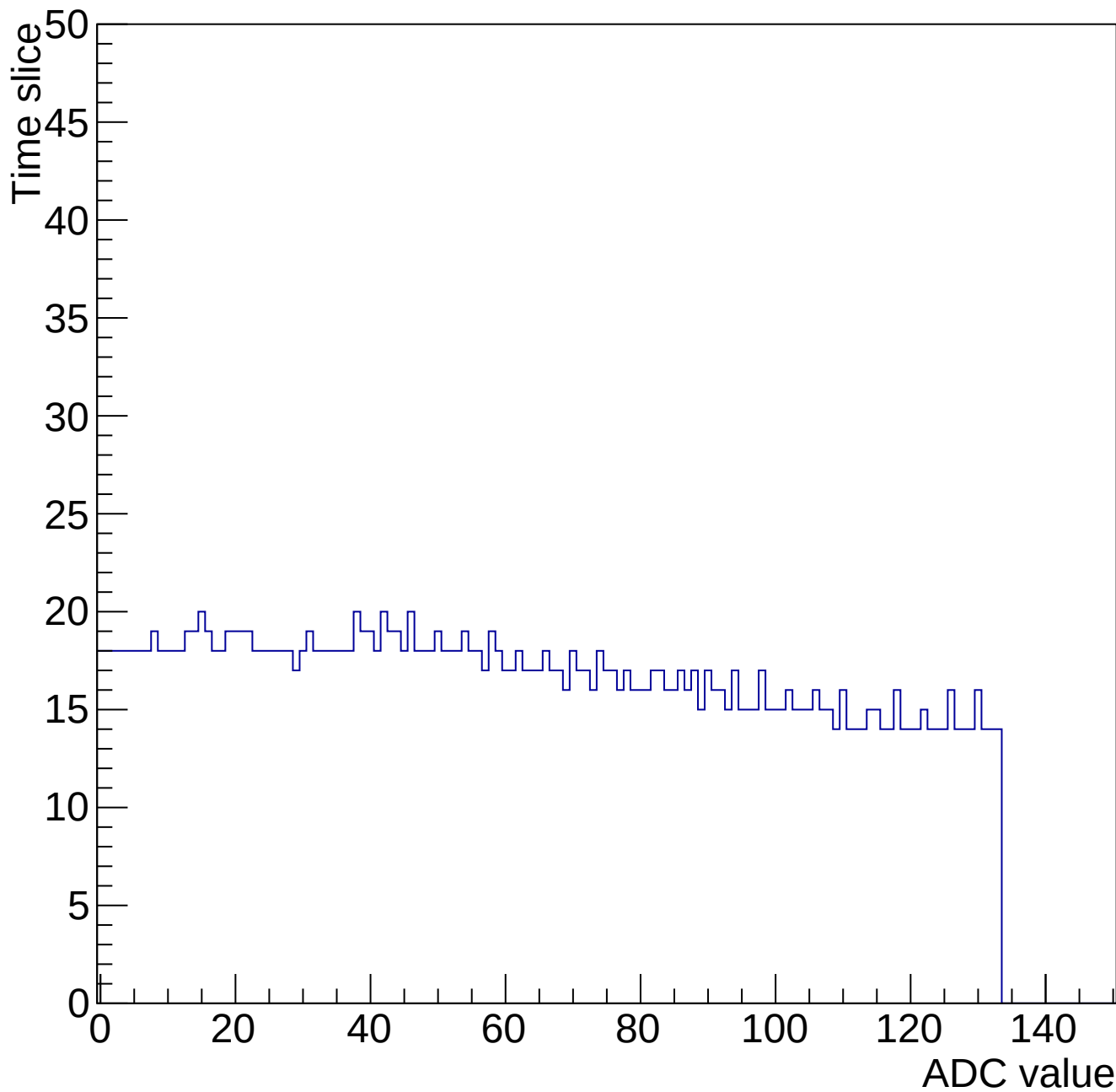
Evt 10 Time mcm 2007 chip 7 chan 15 34656-gain0-shaper0
