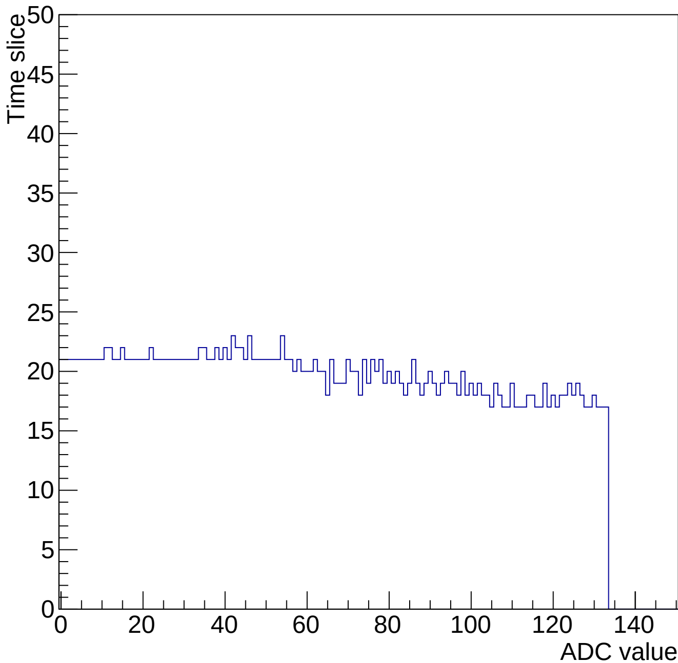
Evt 10 Time mcm 2007 chip 7 chan 11 34656-gain0-shaper0
