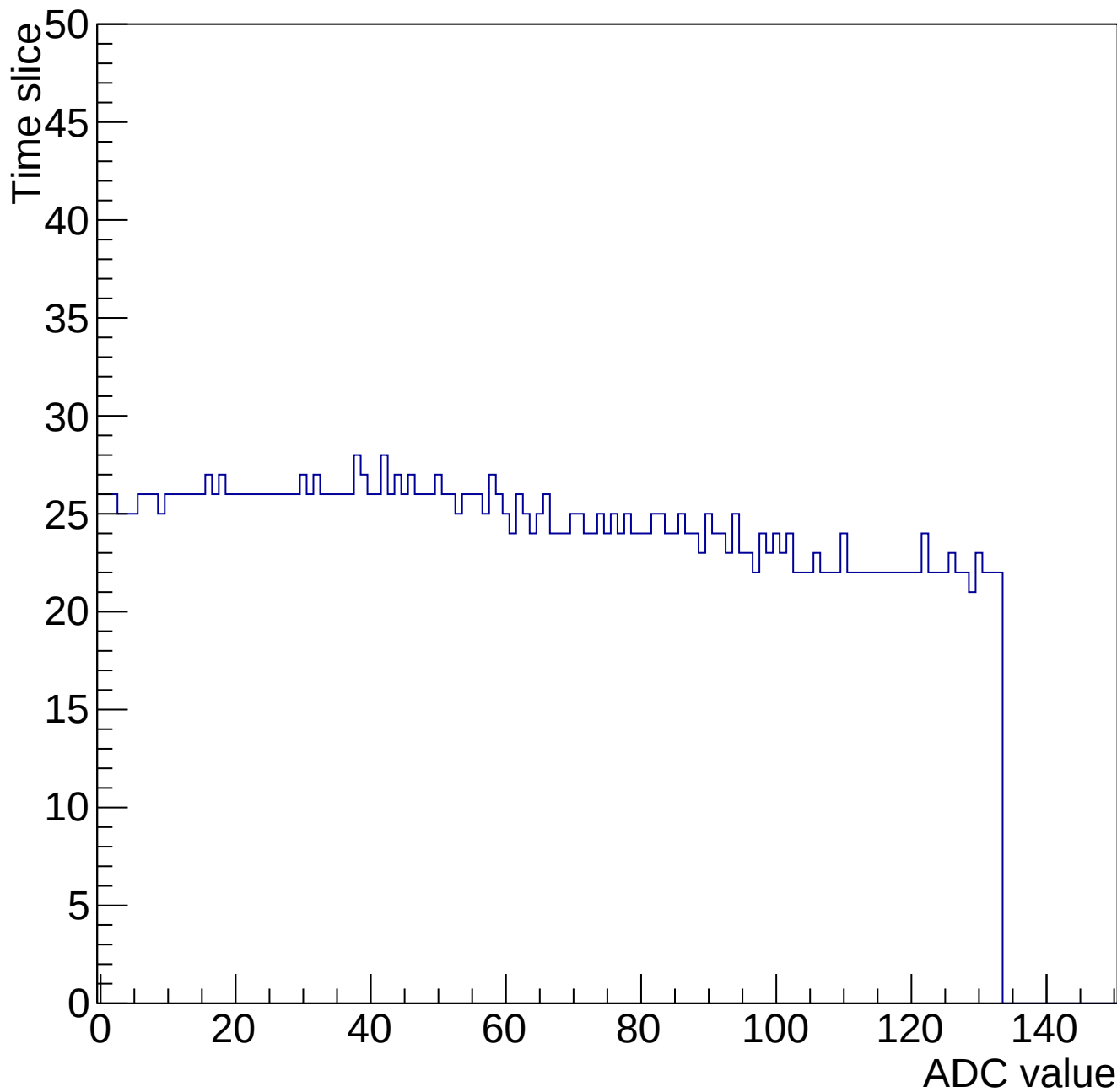
Evt 10 Time mcm 2007 chip 7 chan 13 34656-gain0-shaper0
