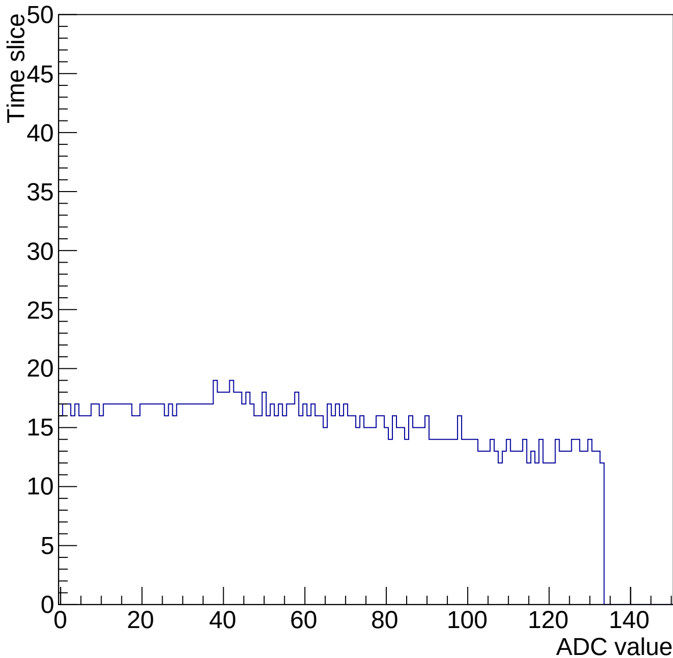
Evt 10 Time mcm 2007 chip 7 chan 2 34656-gain0-shaper0
