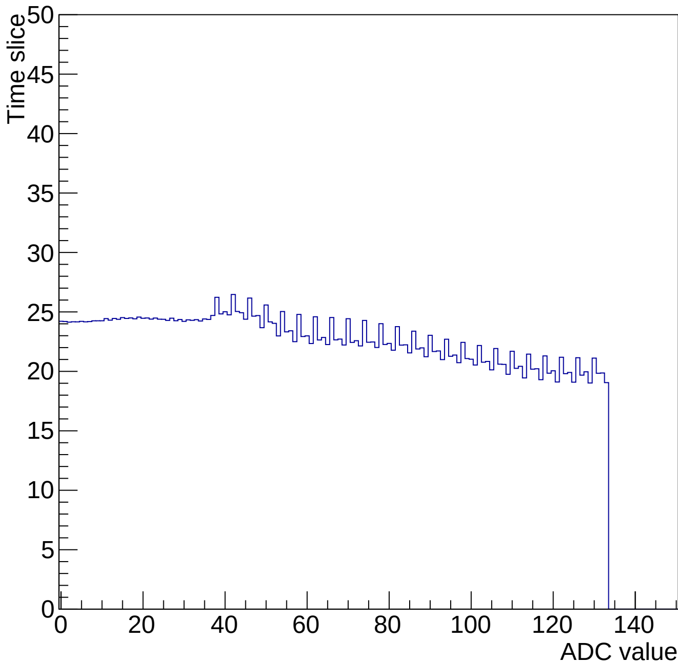
Time mcm 2000 chip 0 chan 4 34643-gain0-shaper0
