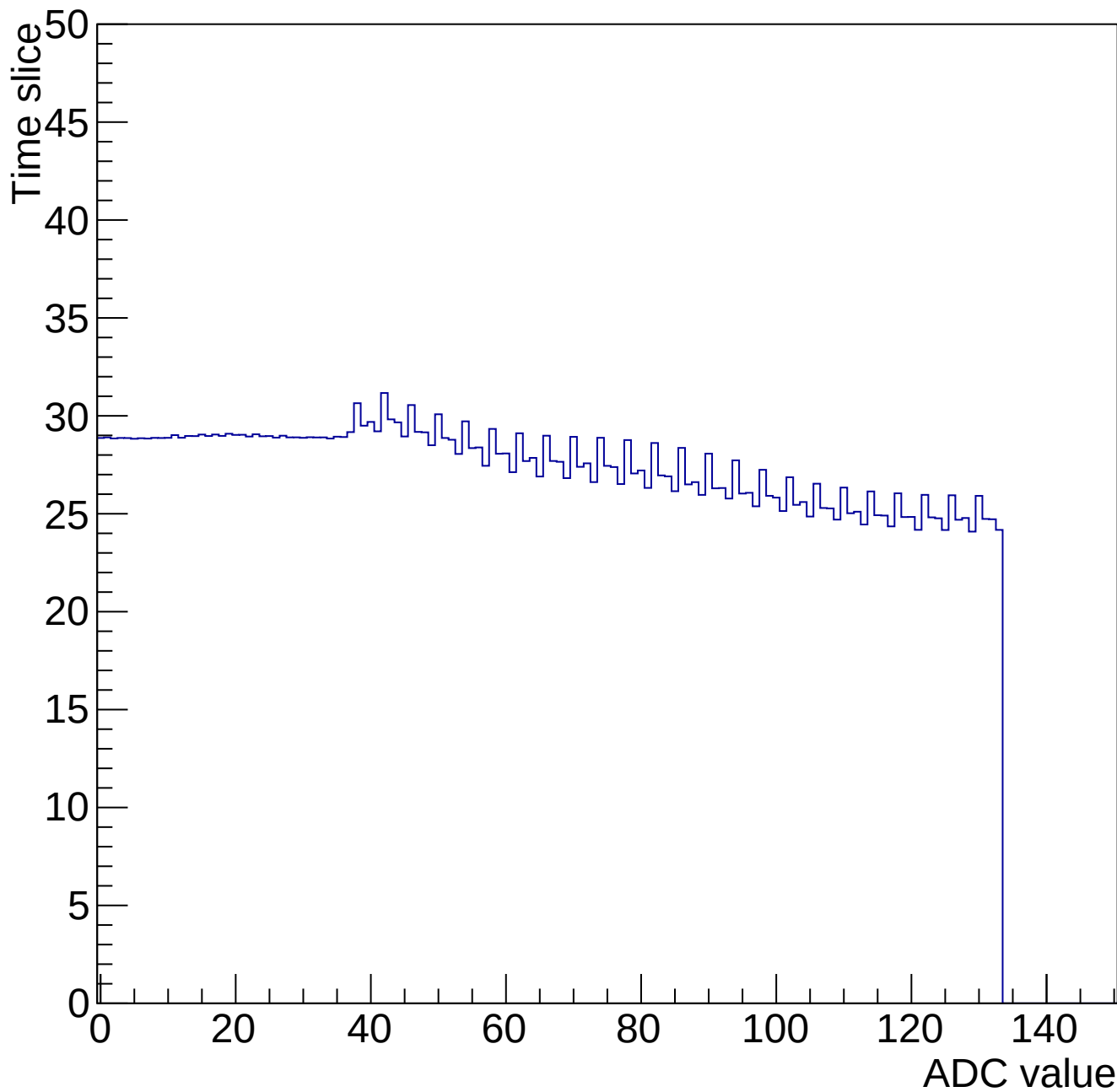
Time mcm 2000 chip 0 chan 13 34643-gain0-shaper0
