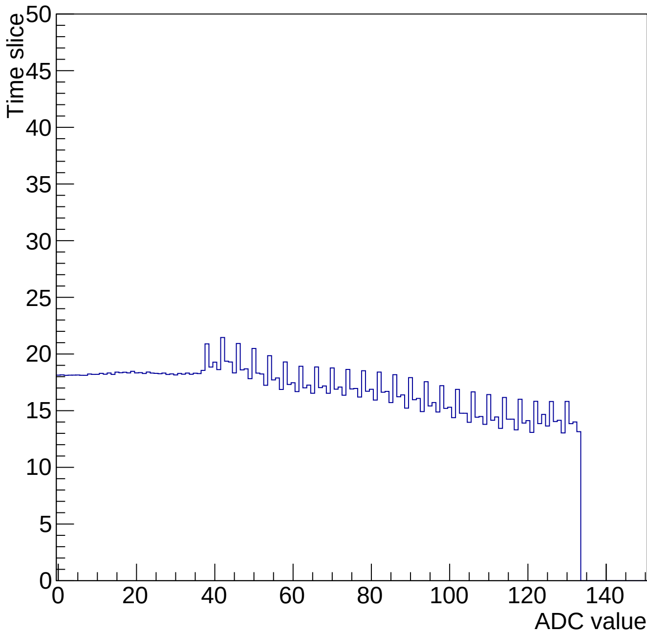
Time mcm 2000 chip 0 chan 0 34643-gain0-shaper0
