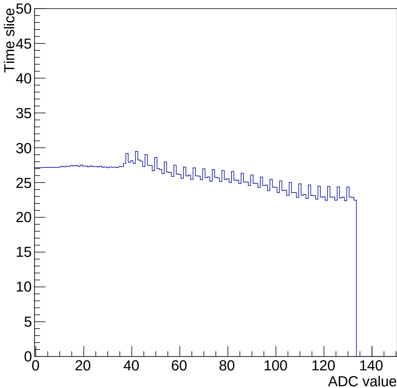
Time mcm 2000 chip 0 chan 7 34643-gain0-shaper0
