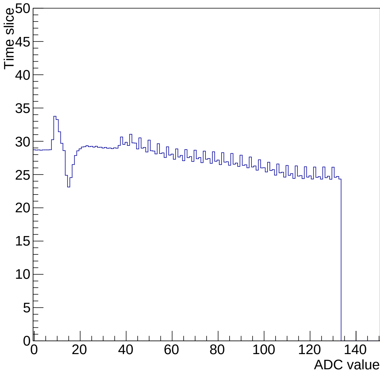
Time mcm 2000 chip 0 chan 1 34643-gain0-shaper0
