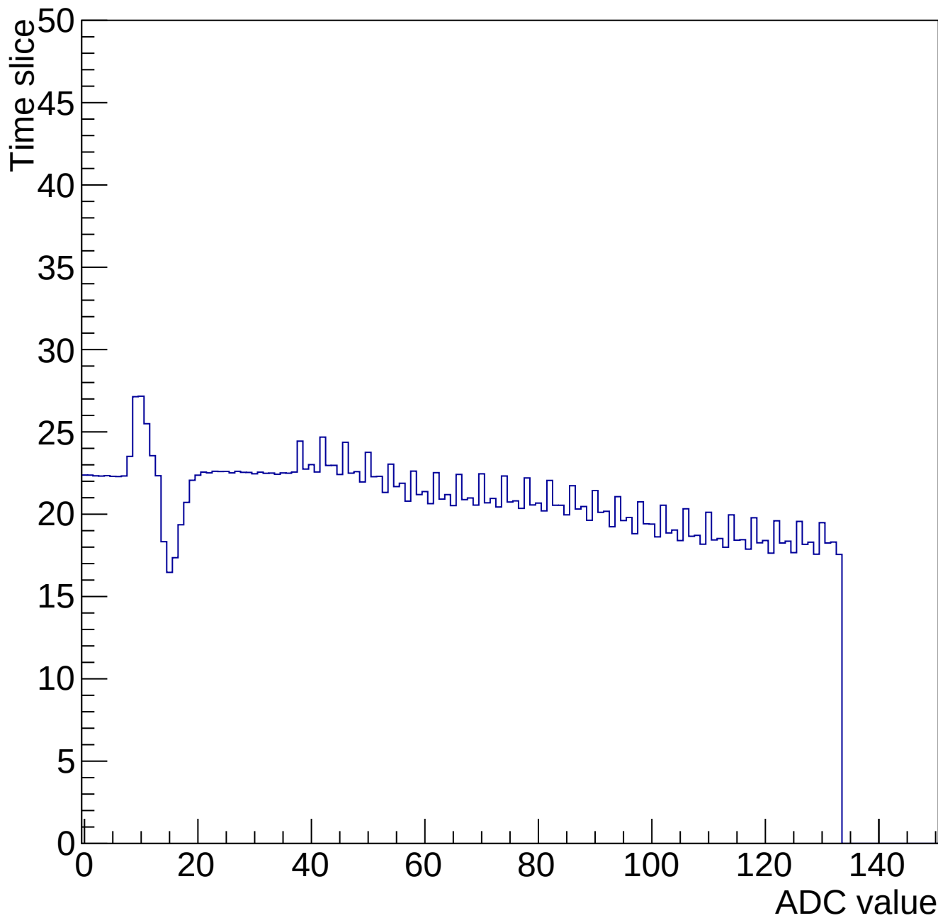
Time mcm 2000 chip 0 chan 2 34643-gain0-shaper0
