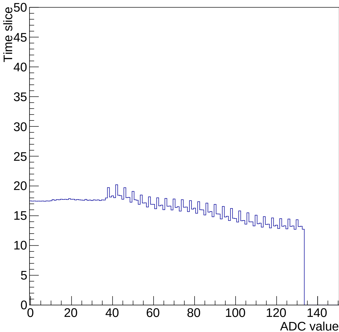
Time mcm 2000 chip 0 chan 9 34643-gain0-shaper0
