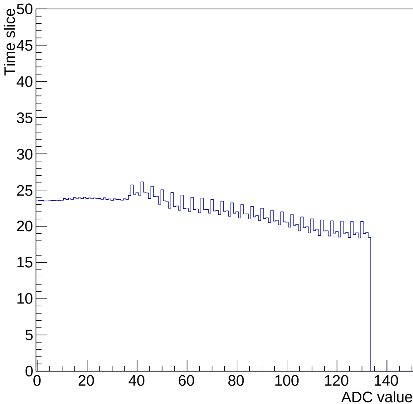
Time mcm 2000 chip 0 chan 3 34643-gain0-shaper0
