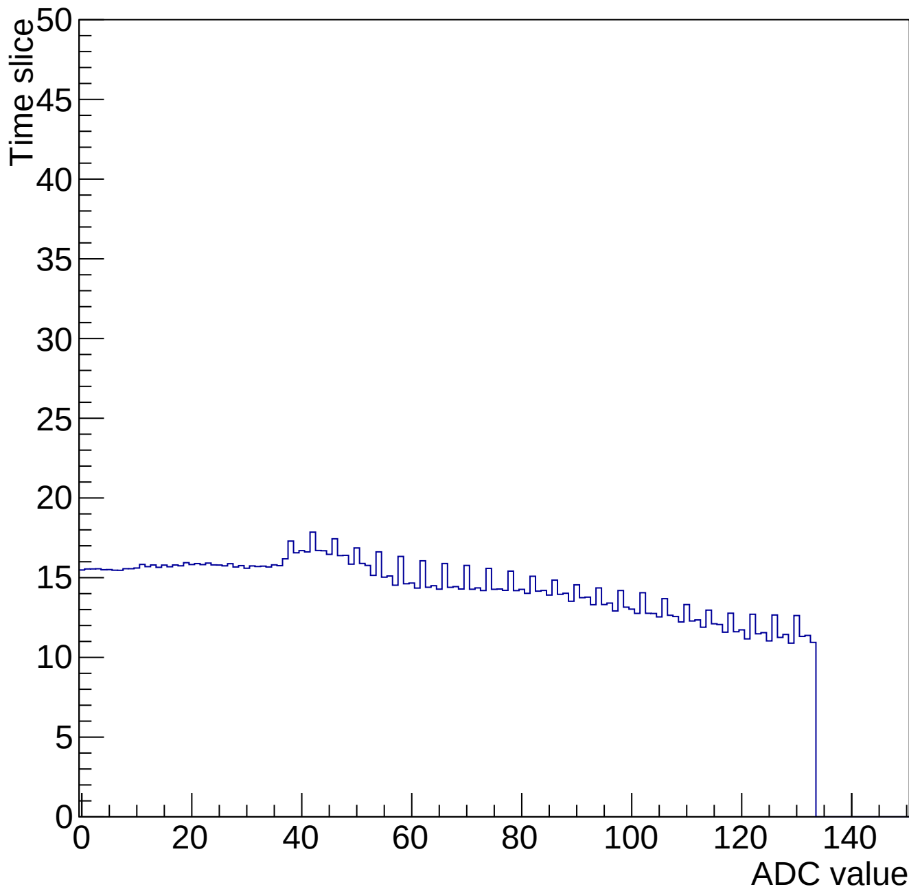
Time mcm 2001 chip 1 chan 4 34645-gain0-shaper0
