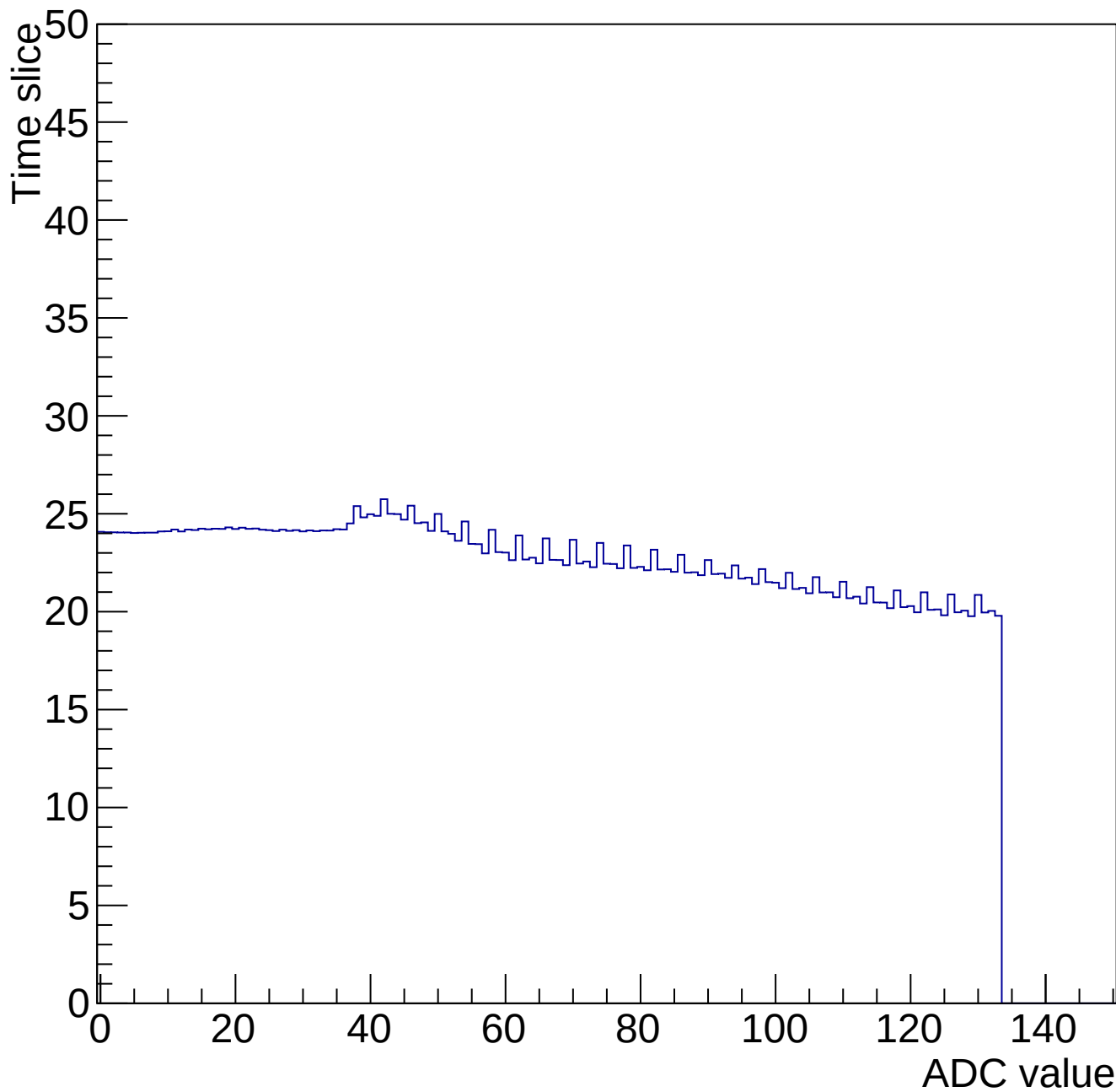
Time mcm 2001 chip 1 chan 11 34645-gain0-shaper0
