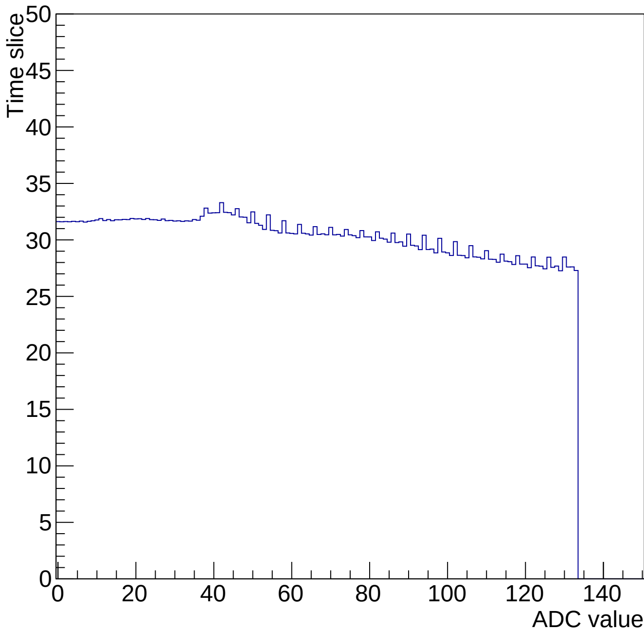
Time mcm 2001 chip 1 chan 6 34645-gain0-shaper0
