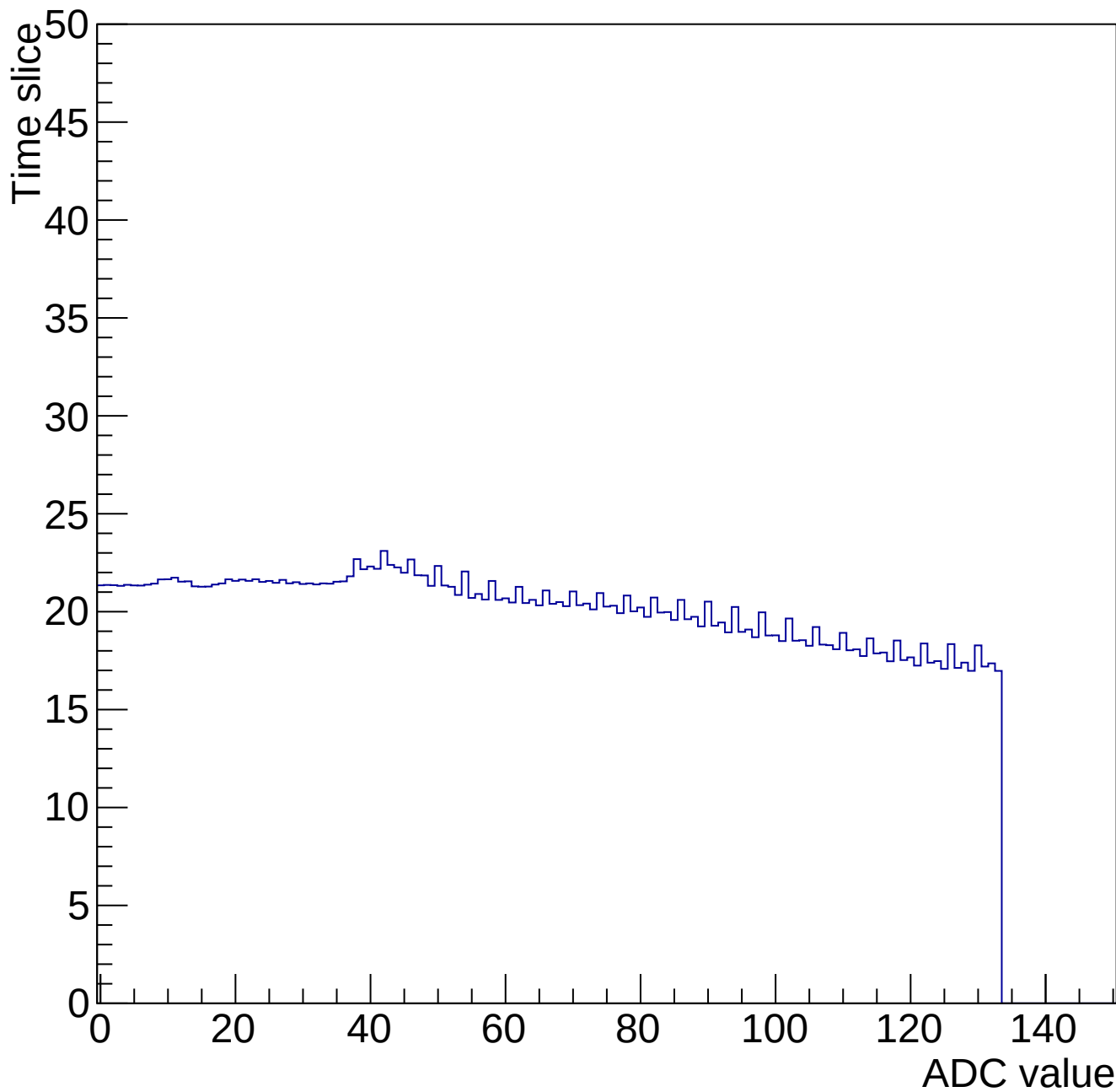
Time mcm 2001 chip 1 chan 12 34645-gain0-shaper0
