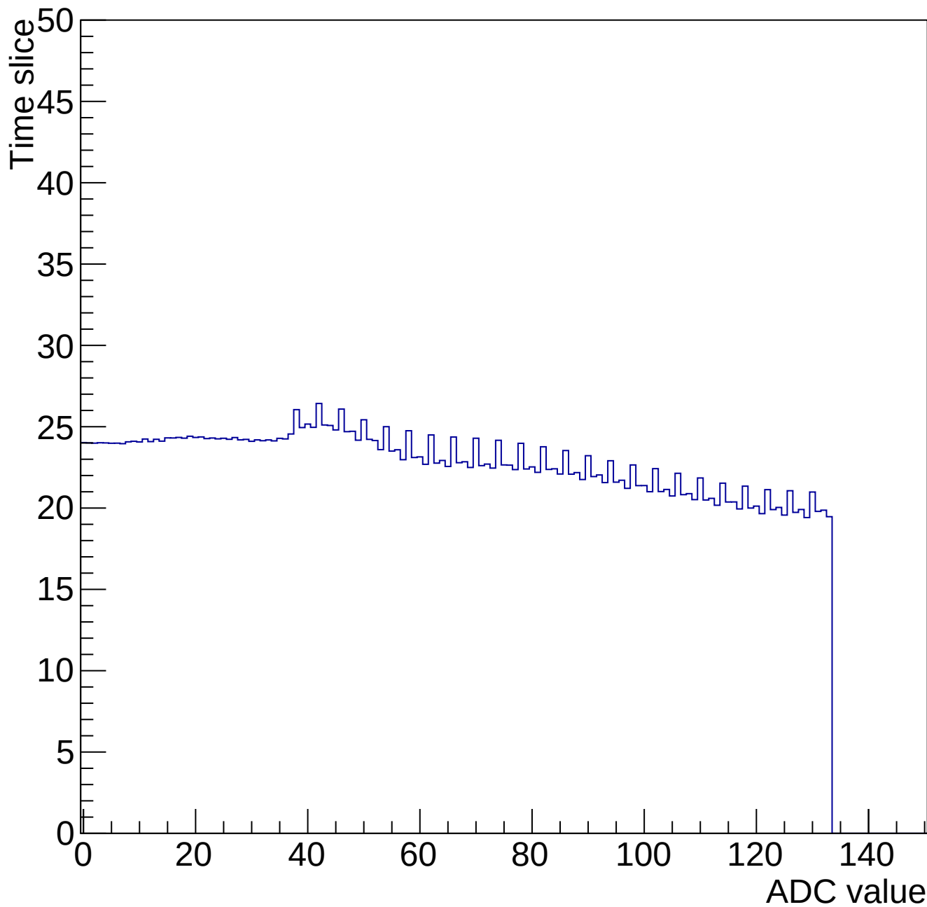
Time mcm 2001 chip 1 chan 0 34645-gain0-shaper0
