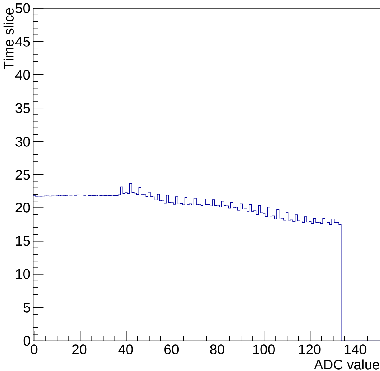
Time mcm 2001 chip 1 chan 5 34645-gain0-shaper0
