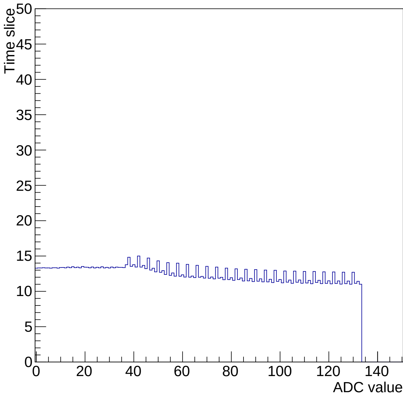
Time mcm 2001 chip 1 chan 2 34660-gain0-shaper6
