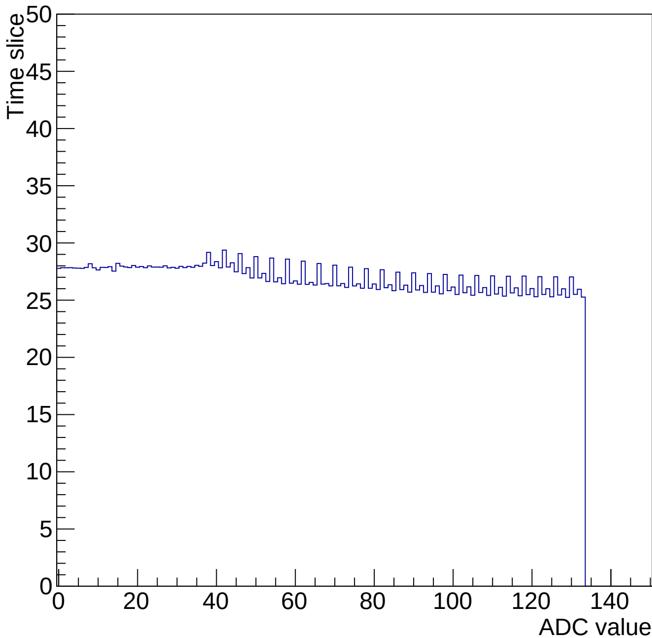
Time mcm 2001 chip 1 chan 15 34660-gain0-shaper6
