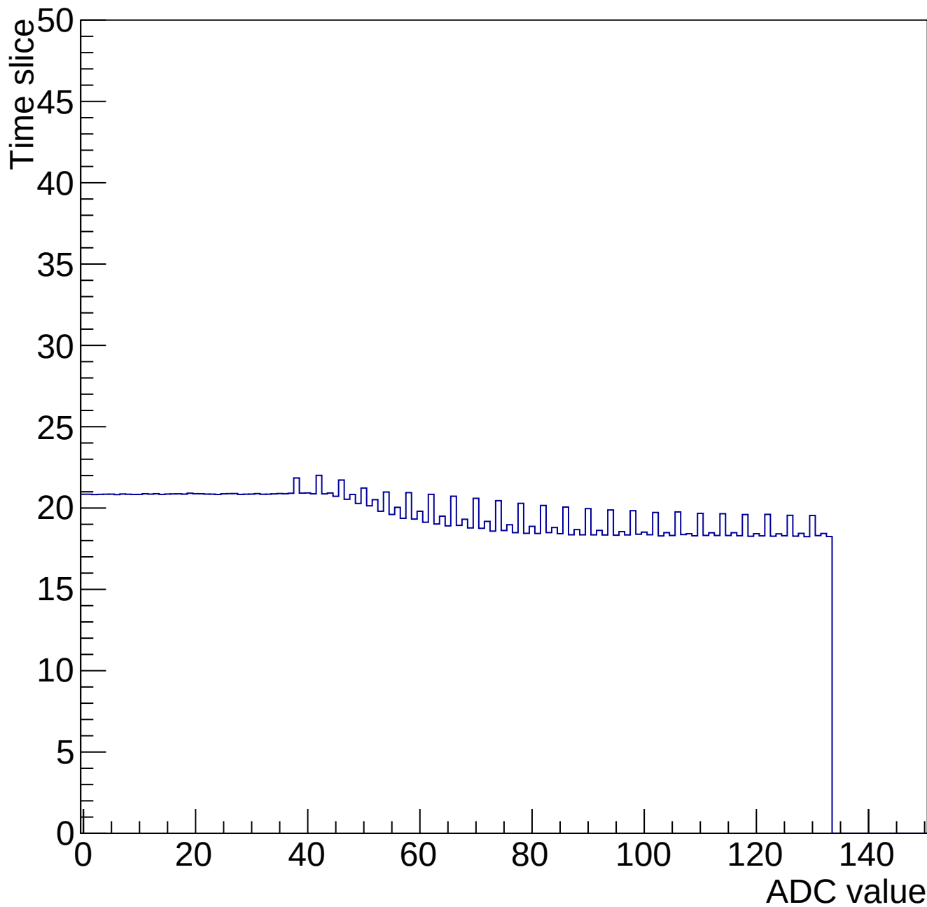
Time mcm 2001 chip 1 chan 13 34660-gain0-shaper6
