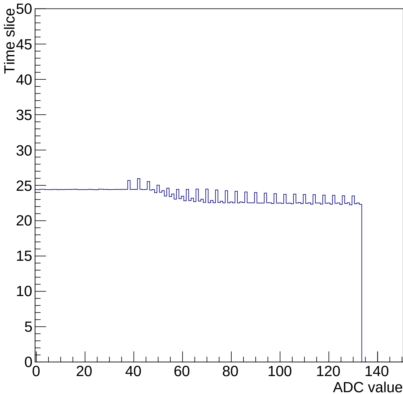
Time mcm 2001 chip 1 chan 6 34660-gain0-shaper6
