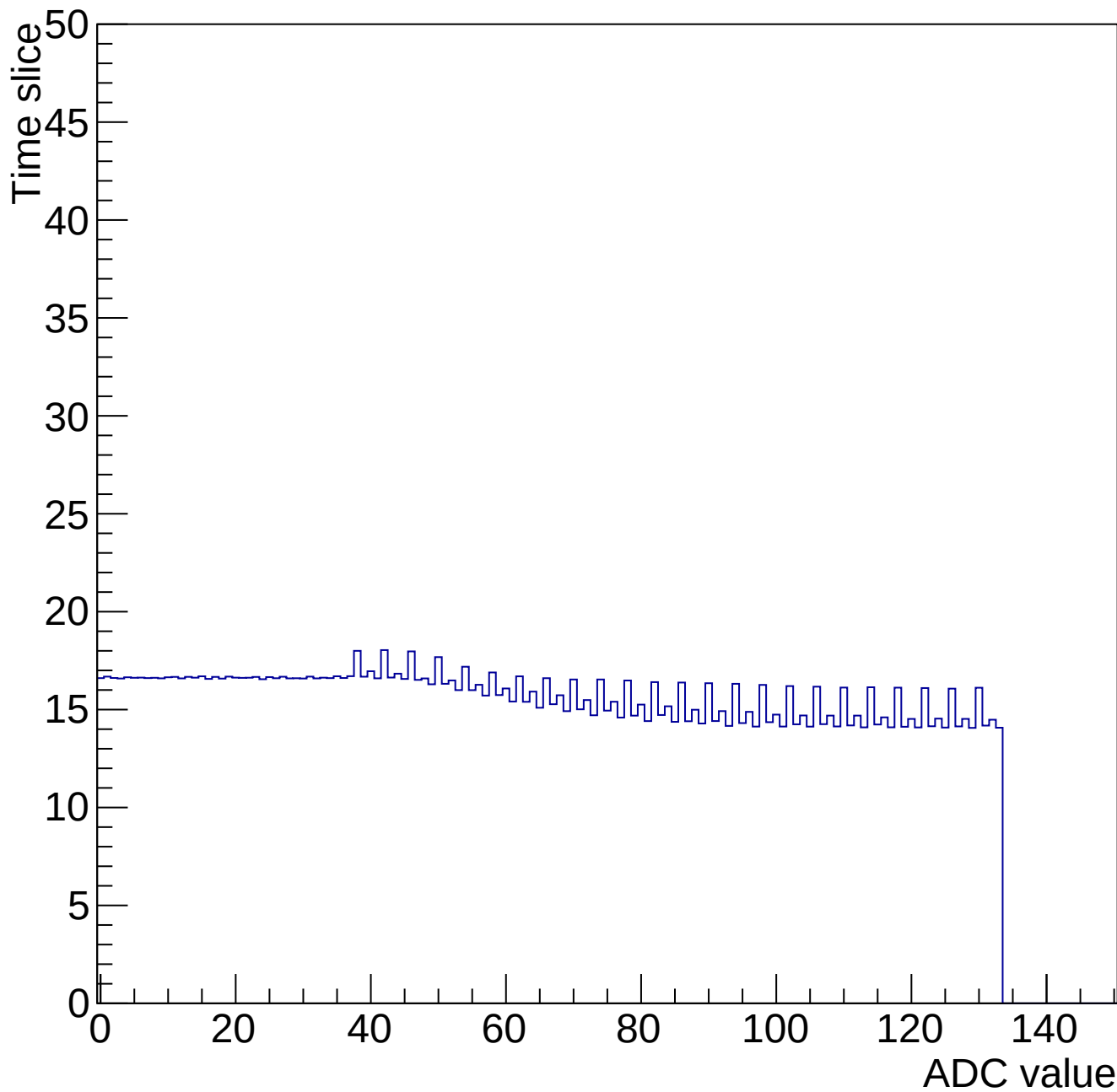
Time mcm 2001 chip 1 chan 5 34660-gain0-shaper6
