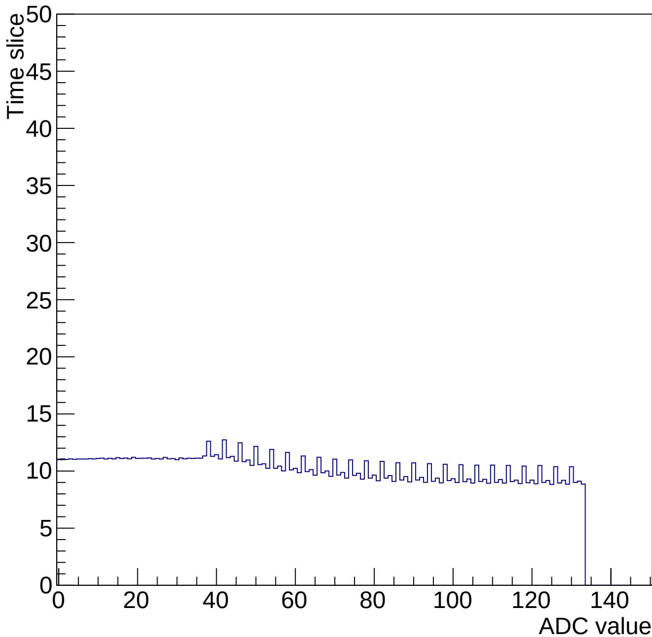
Time mcm 2001 chip 1 chan 7 34660-gain0-shaper6
