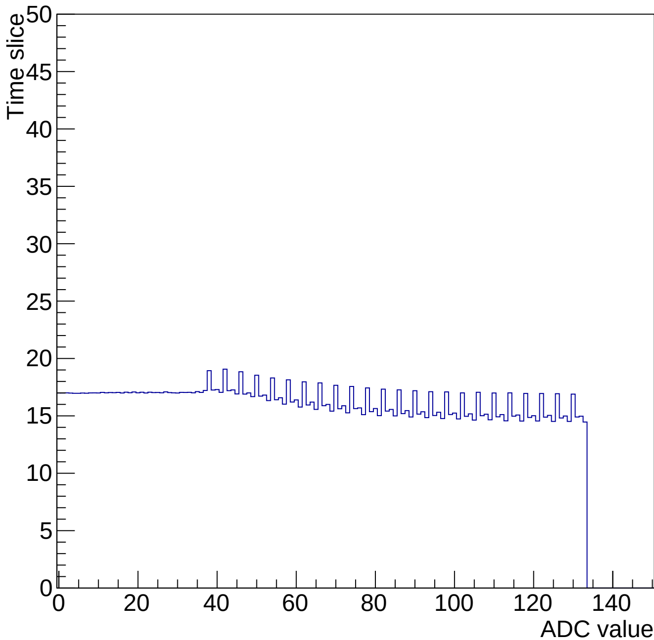
Time mcm 2001 chip 1 chan 8 34660-gain0-shaper6
