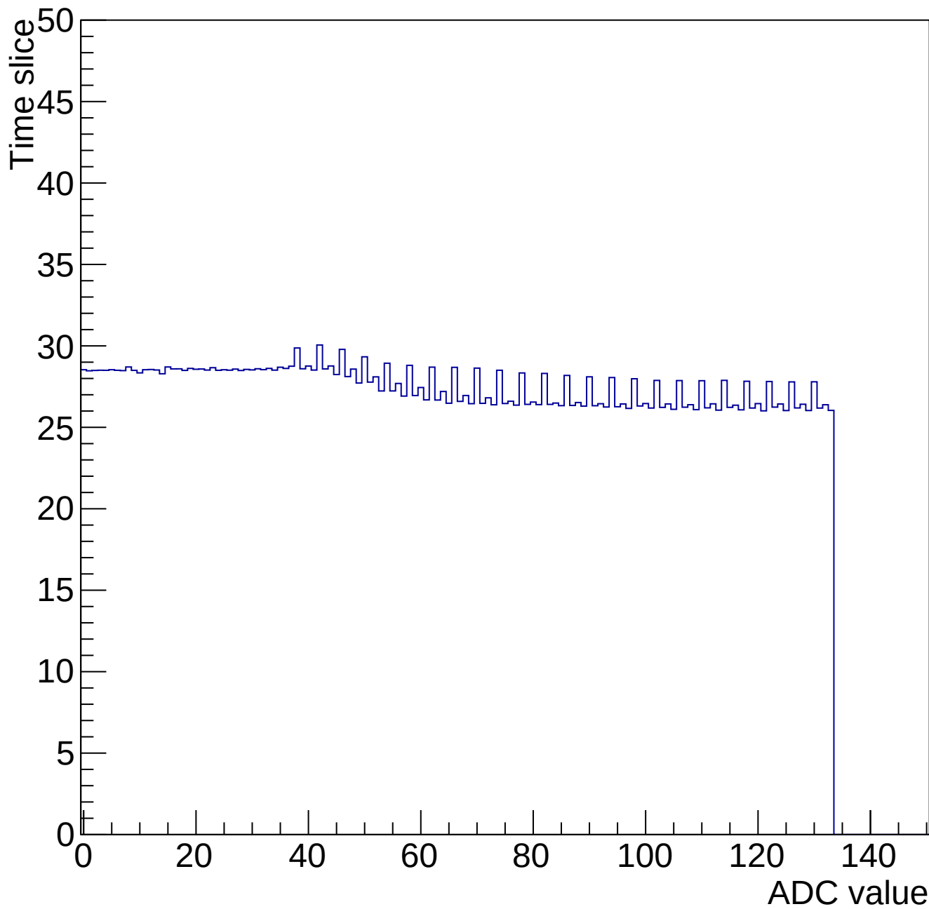
Time mcm 2001 chip 1 chan 15 34668-gain0-shaper6
