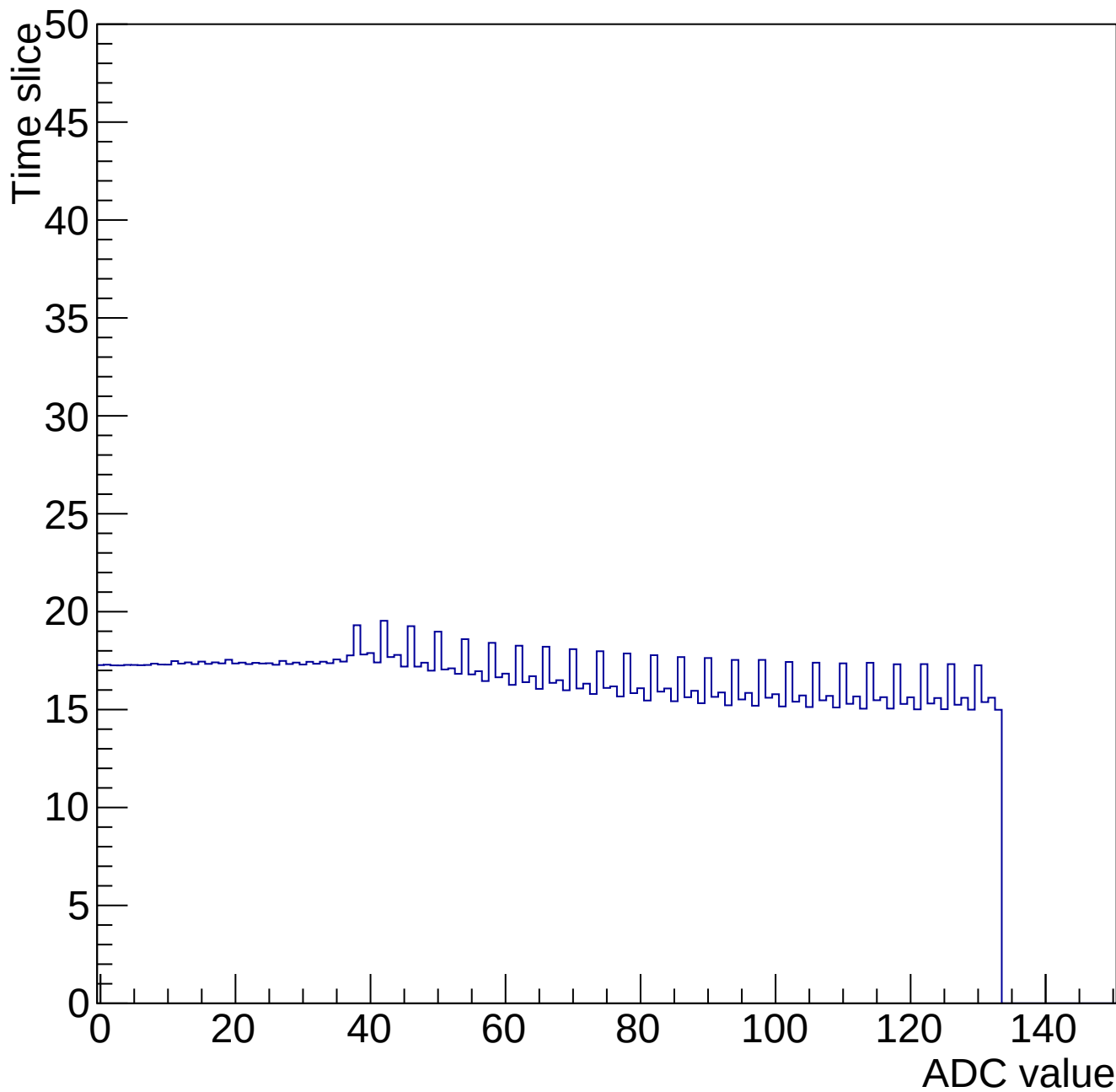
Time mcm 2001 chip 1 chan 8 34668-gain0-shaper6
