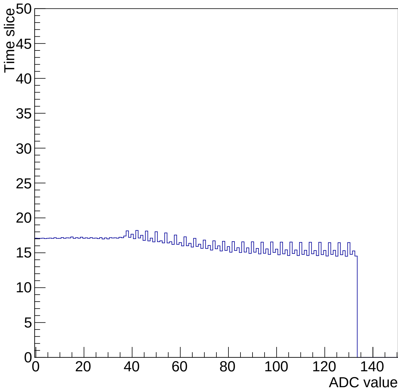
Time mcm 2001 chip 1 chan 5 34668-gain0-shaper6
