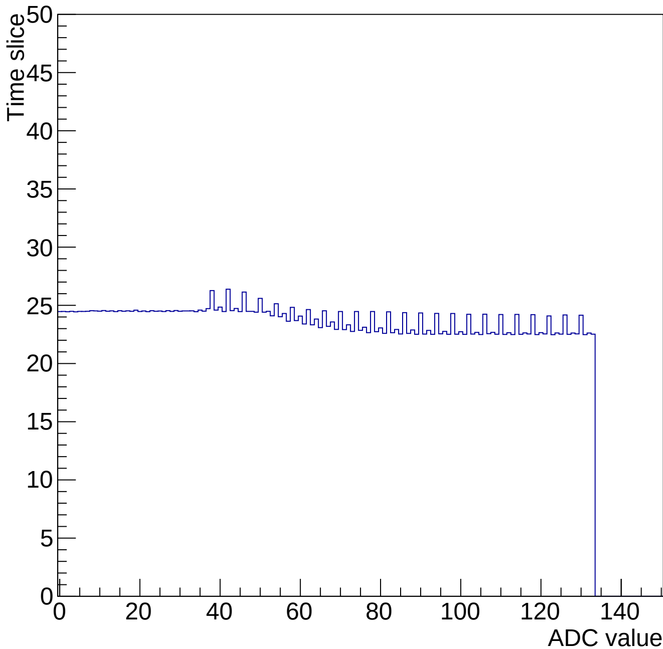
Time mcm 2001 chip 1 chan 6 34668-gain0-shaper6
