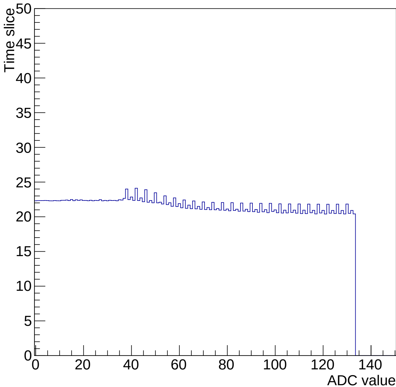
Time mcm 2001 chip 1 chan 11 34668-gain0-shaper6
