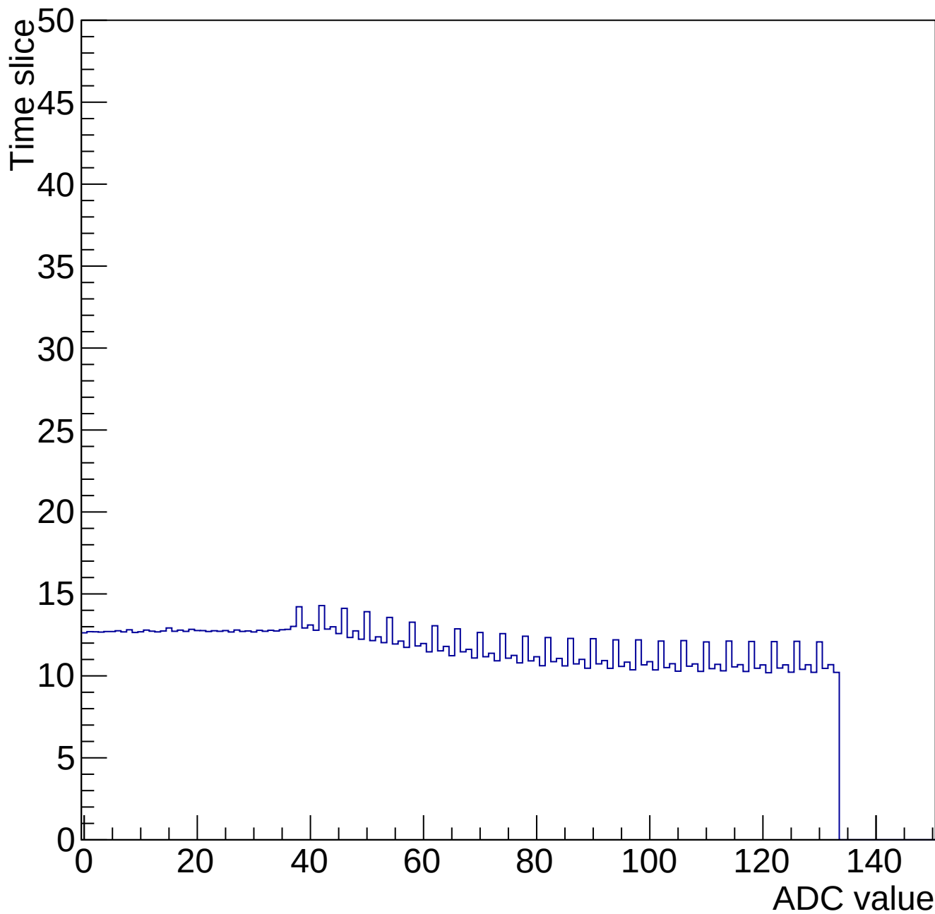
Time mcm 2001 chip 1 chan 1 34668-gain0-shaper6
