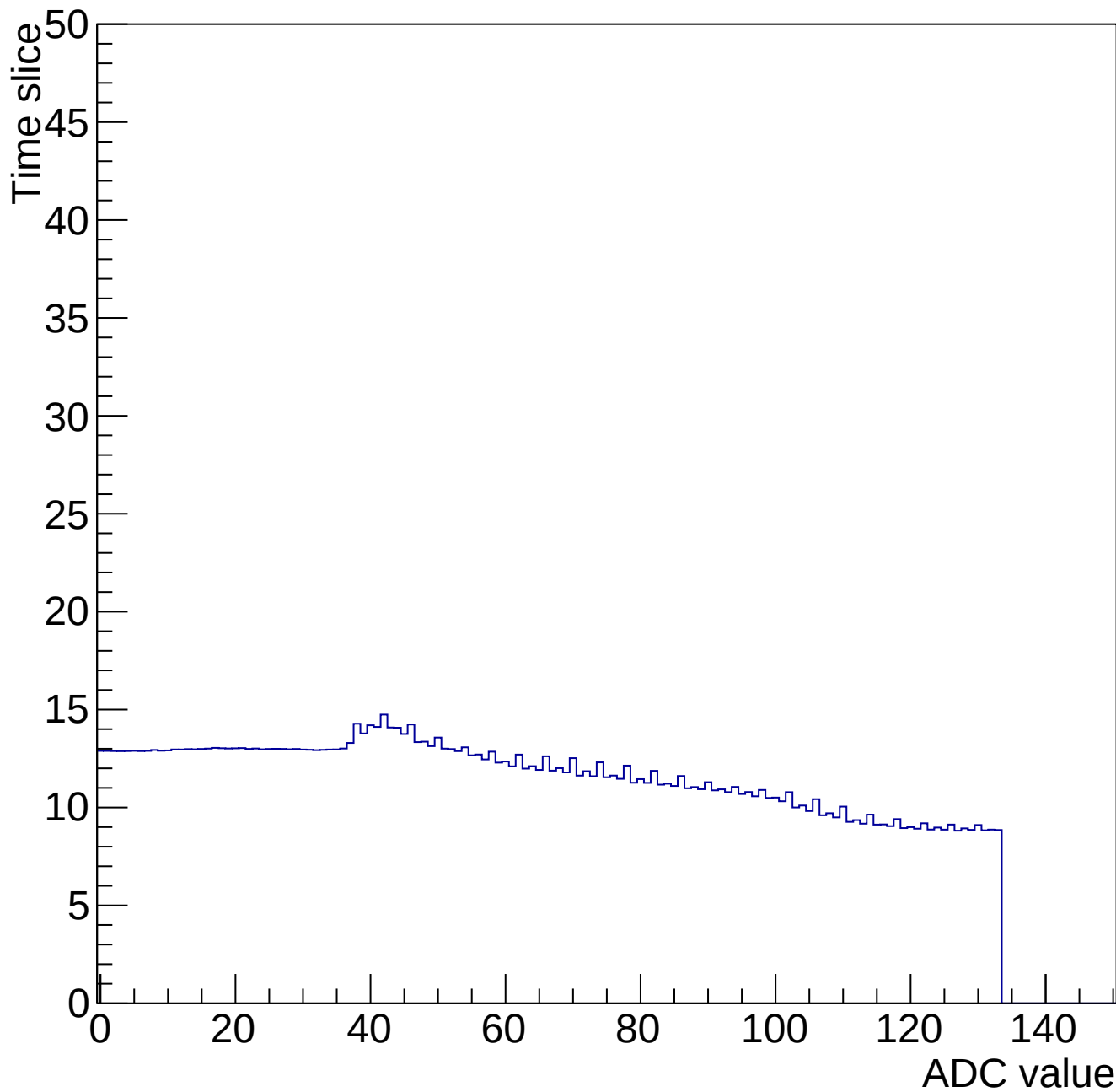
Time mcm 2002 chip 2 chan 3 34647-gain0-shaper0
