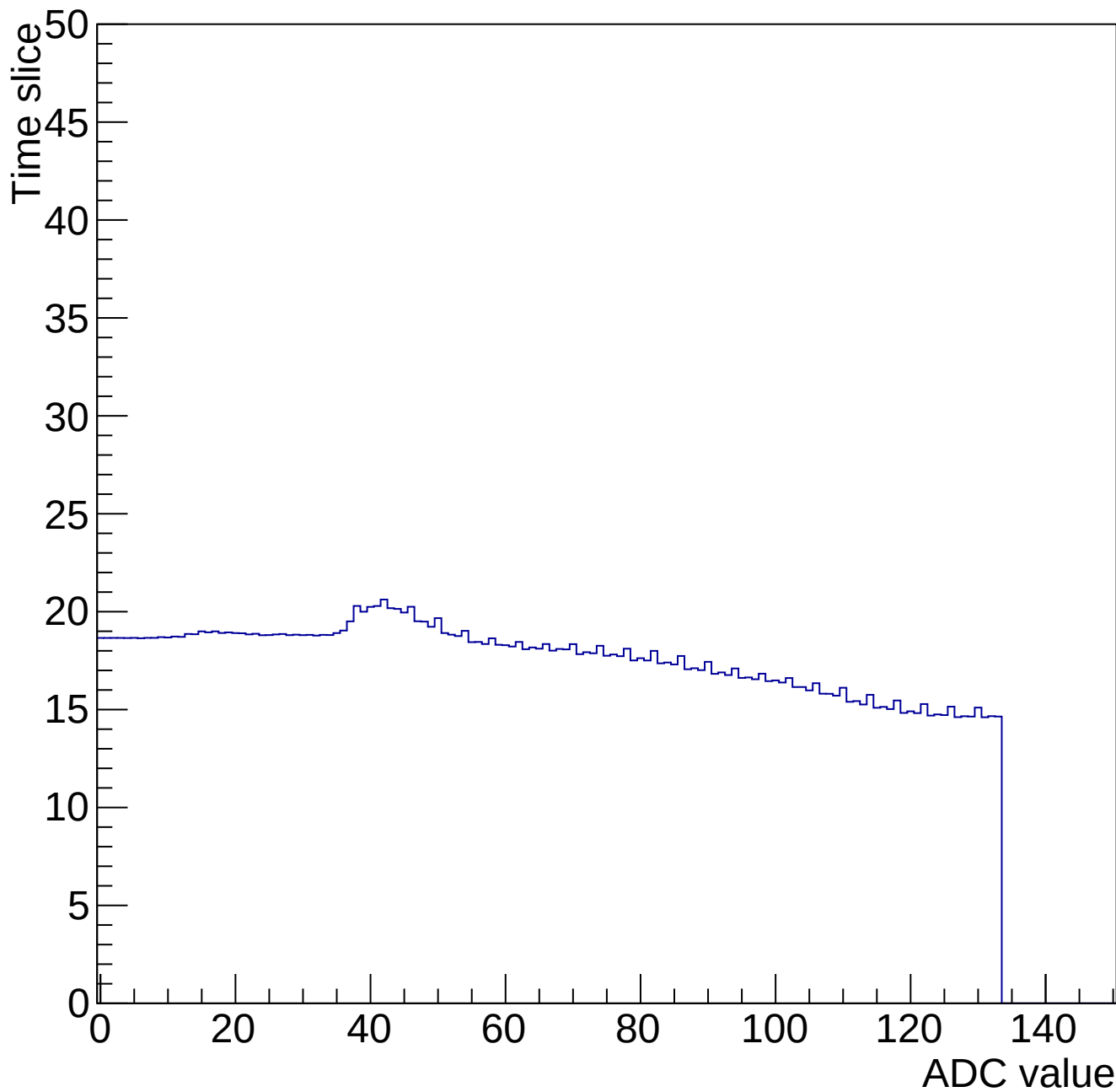
Time mcm 2002 chip 2 chan 6 34647-gain0-shaper0
