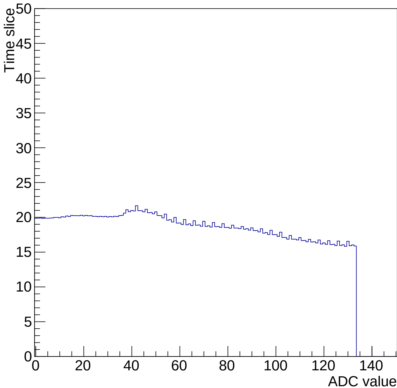
Time mcm 2002 chip 2 chan 11 34647-gain0-shaper0
