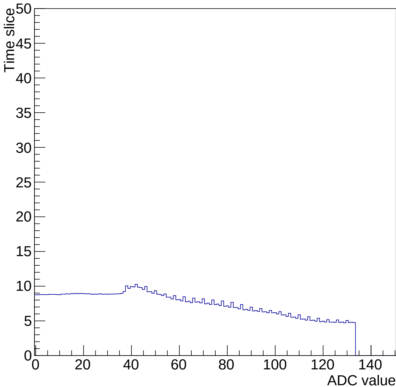
Time mcm 2002 chip 2 chan 14 34647-gain0-shaper0
