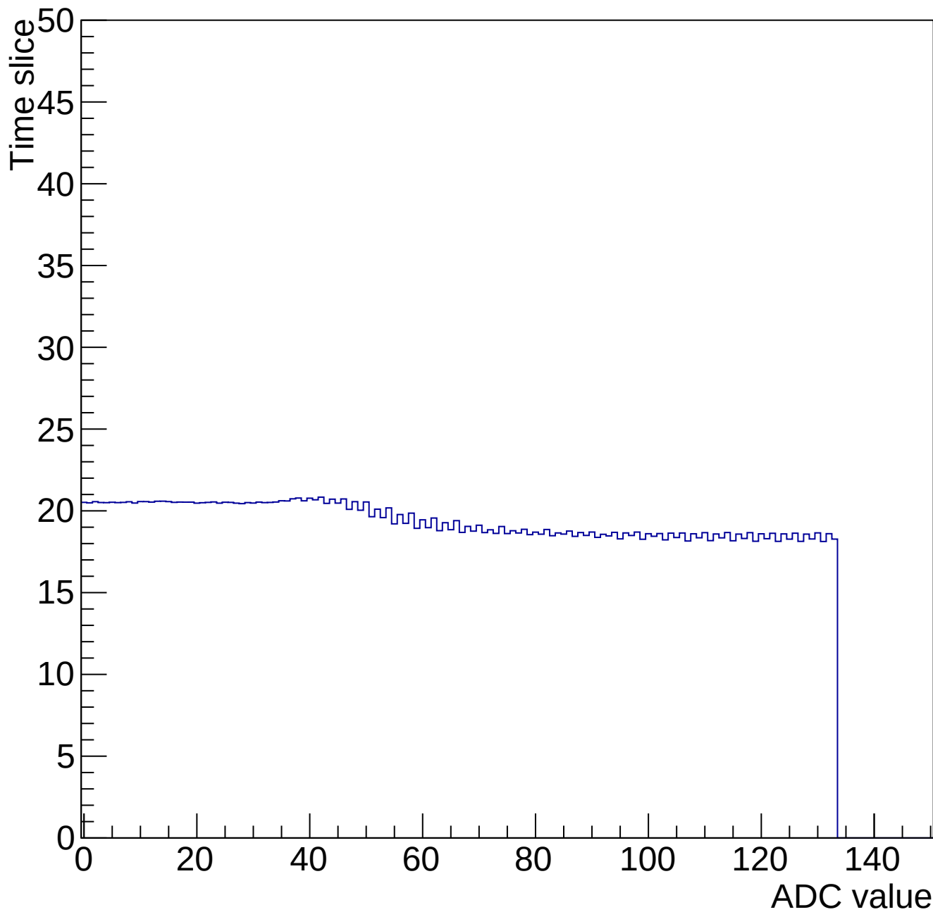
Time mcm 2002 chip 2 chan 10 34661-gain0-shaper6
