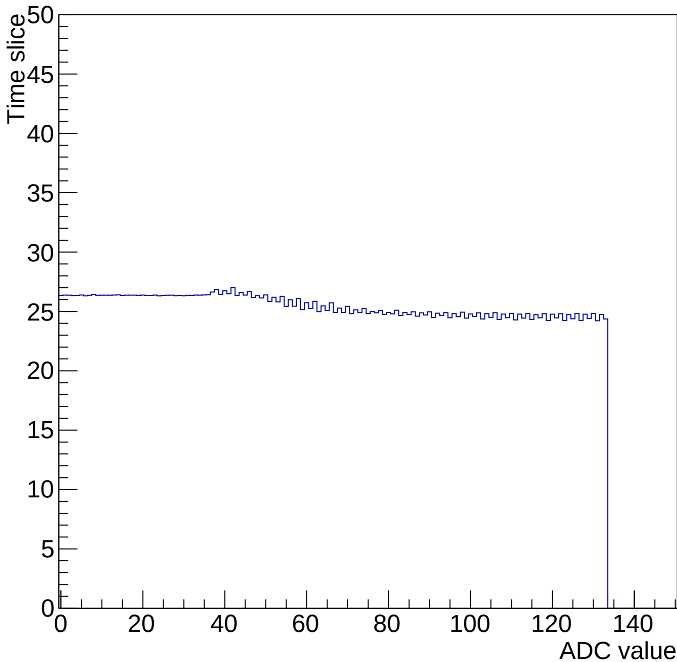
Time mcm 2002 chip 2 chan 4 34661-gain0-shaper6
