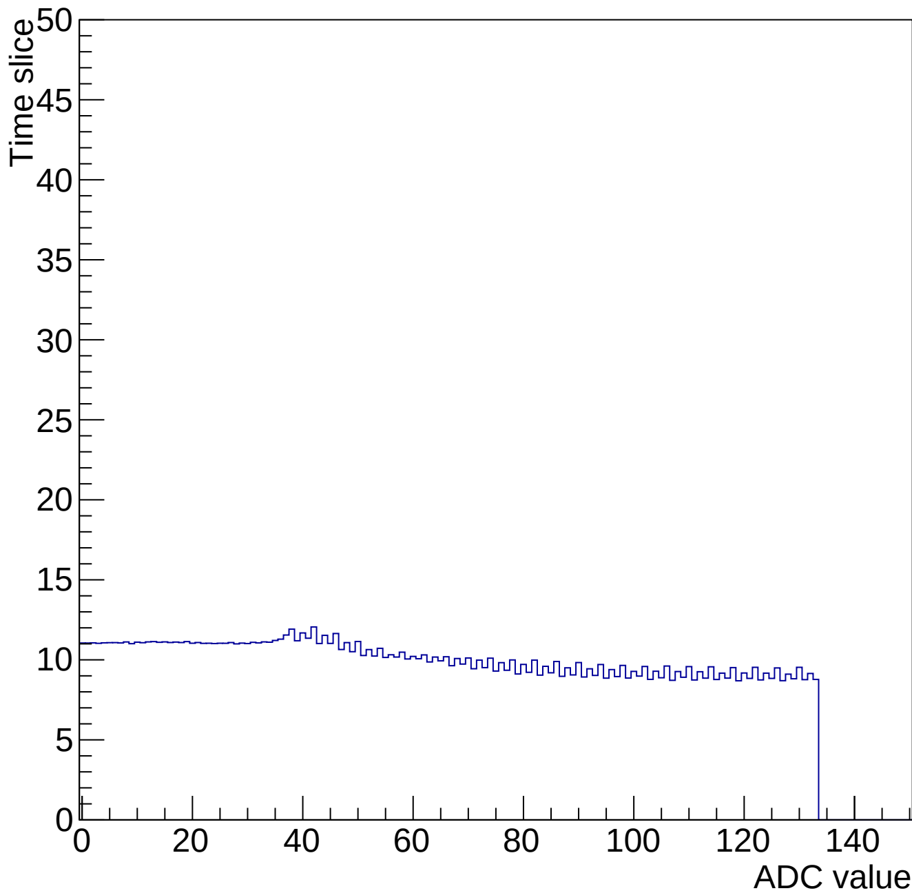
Time mcm 2002 chip 2 chan 12 34661-gain0-shaper6
