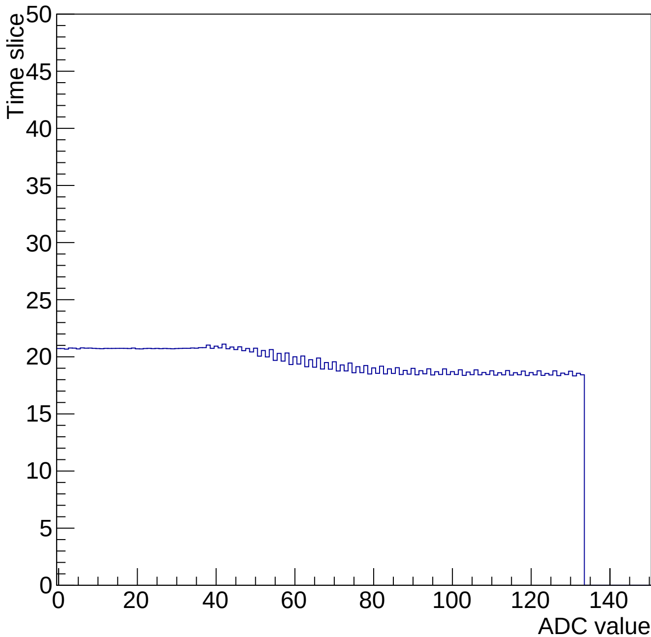
Time mcm 2002 chip 2 chan 11 34661-gain0-shaper6
