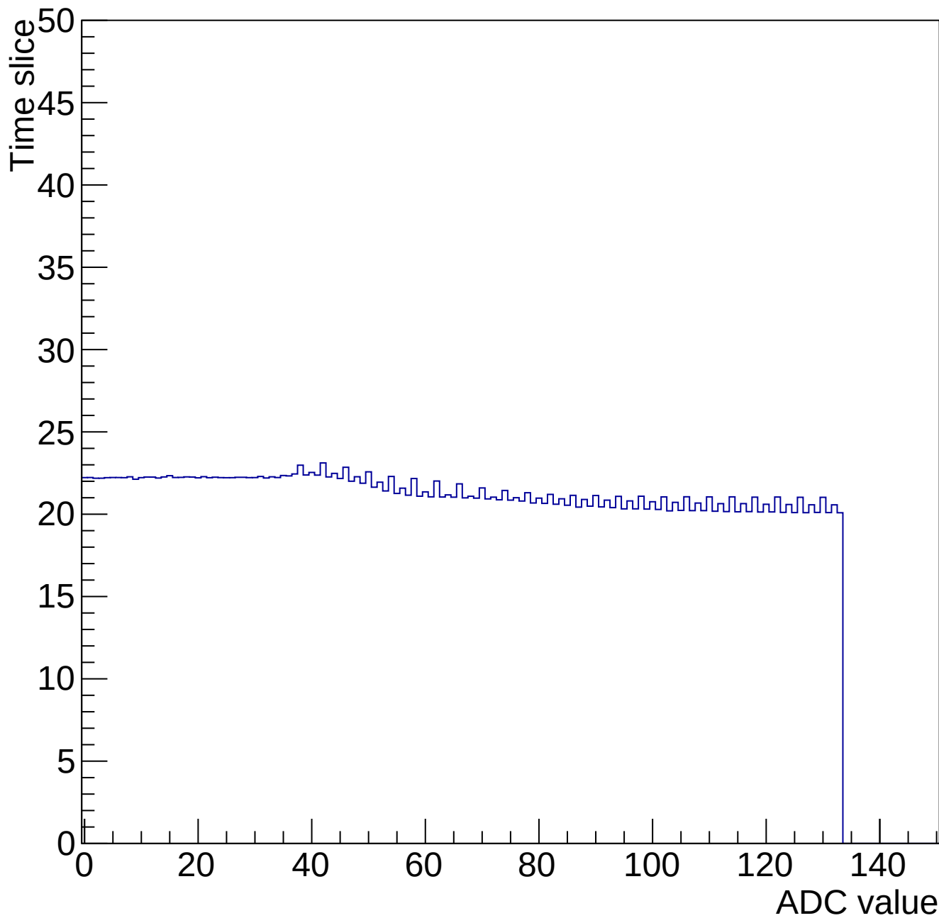
Time mcm 2002 chip 2 chan 0 34661-gain0-shaper6
