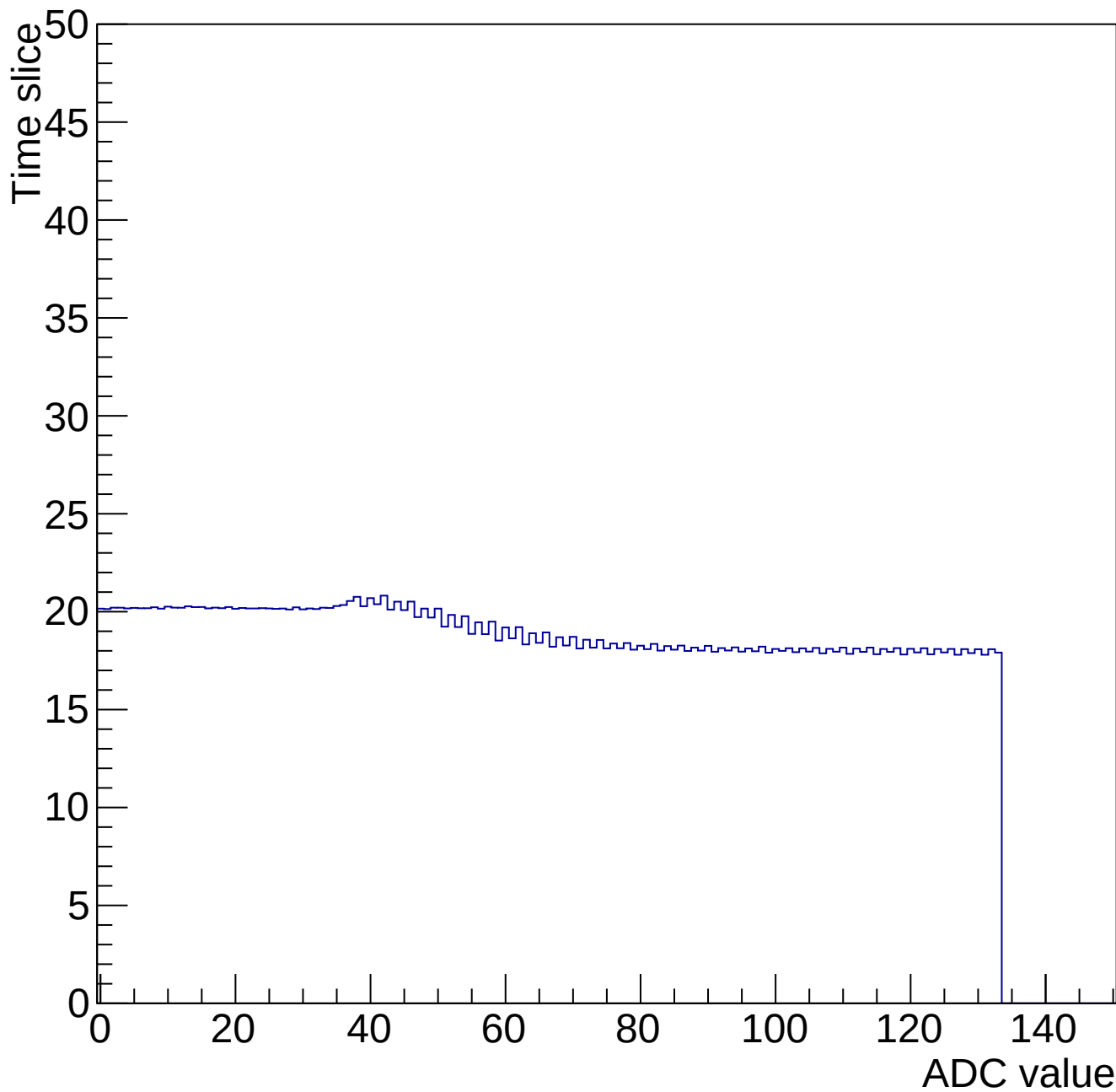
Time mcm 2002 chip 2 chan 13 34661-gain0-shaper6
