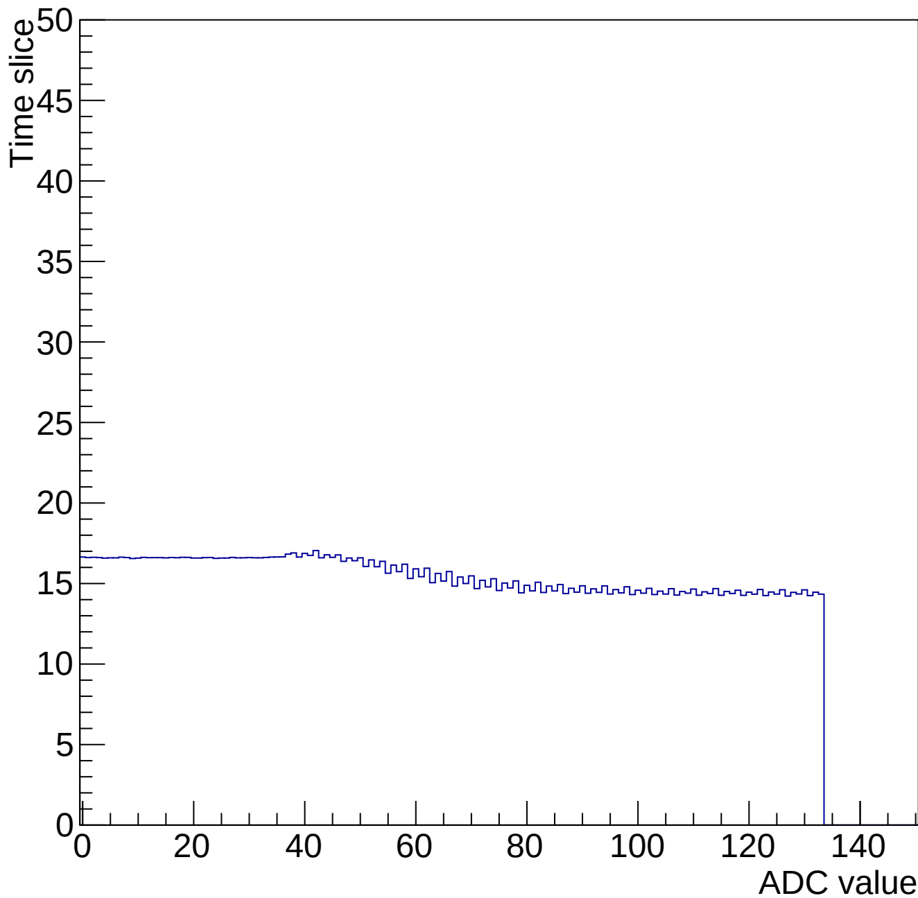
Time mcm 2002 chip 2 chan 6 34661-gain0-shaper6
