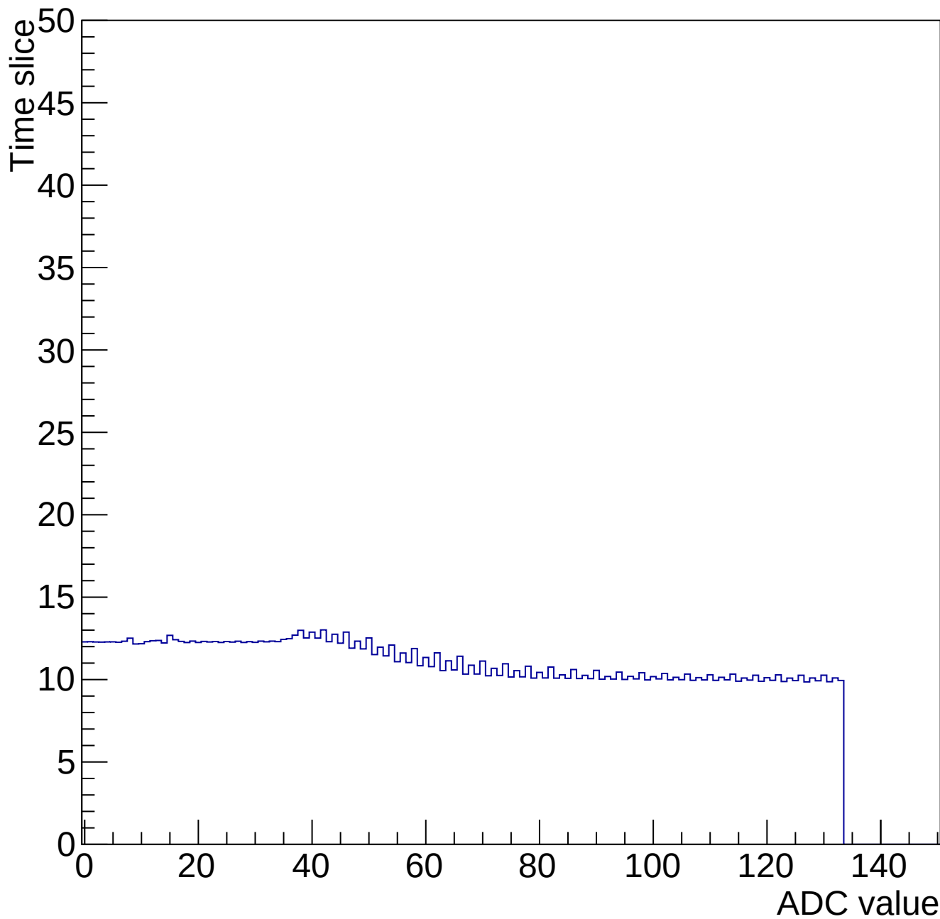
Time mcm 2002 chip 2 chan 15 34661-gain0-shaper6
