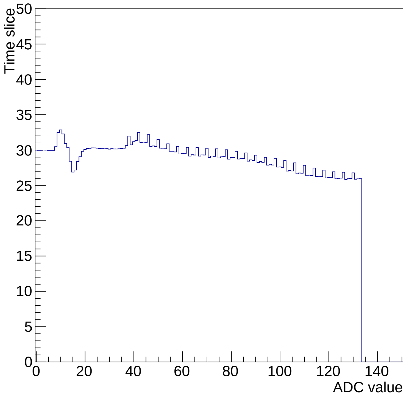
Time mcm 2003 chip 3 chan 0 34649-gain0-shaper0
