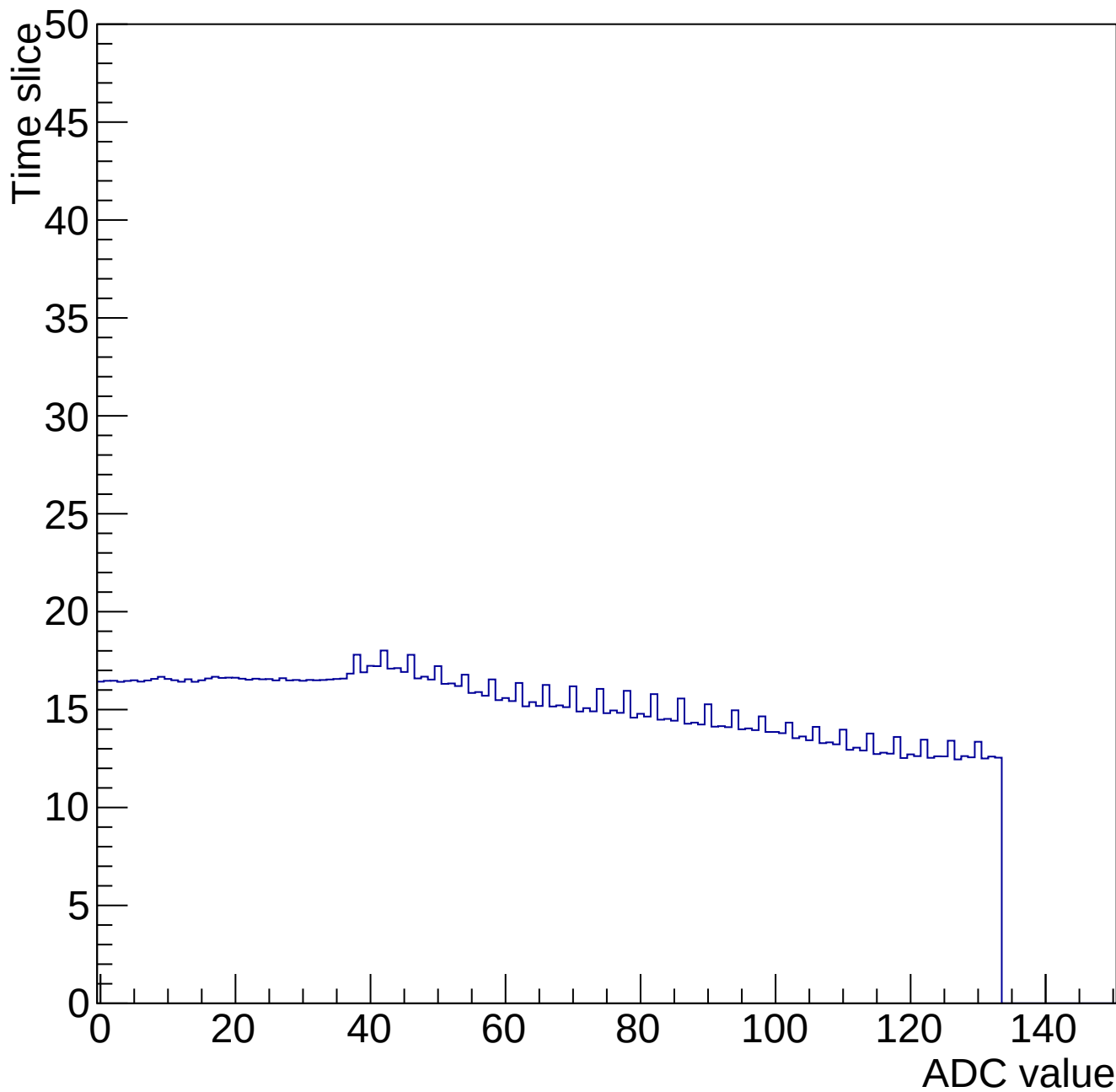
Time mcm 2003 chip 3 chan 15 34649-gain0-shaper0
