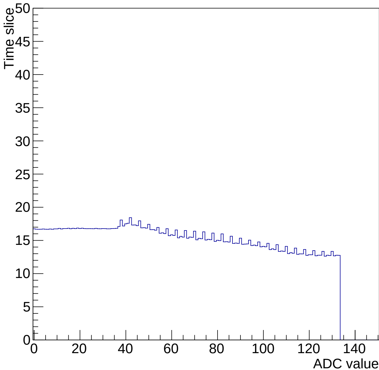
Time mcm 2003 chip 3 chan 3 34649-gain0-shaper0
