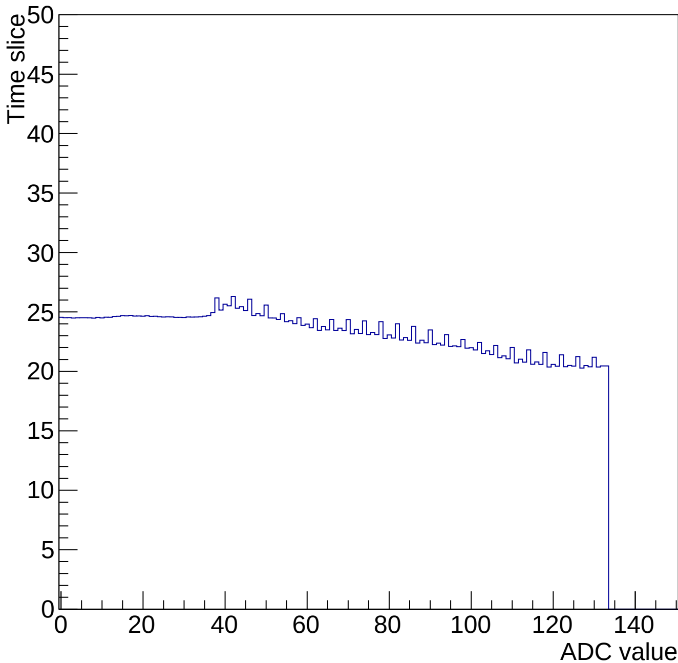
Time mcm 2003 chip 3 chan 9 34649-gain0-shaper0
