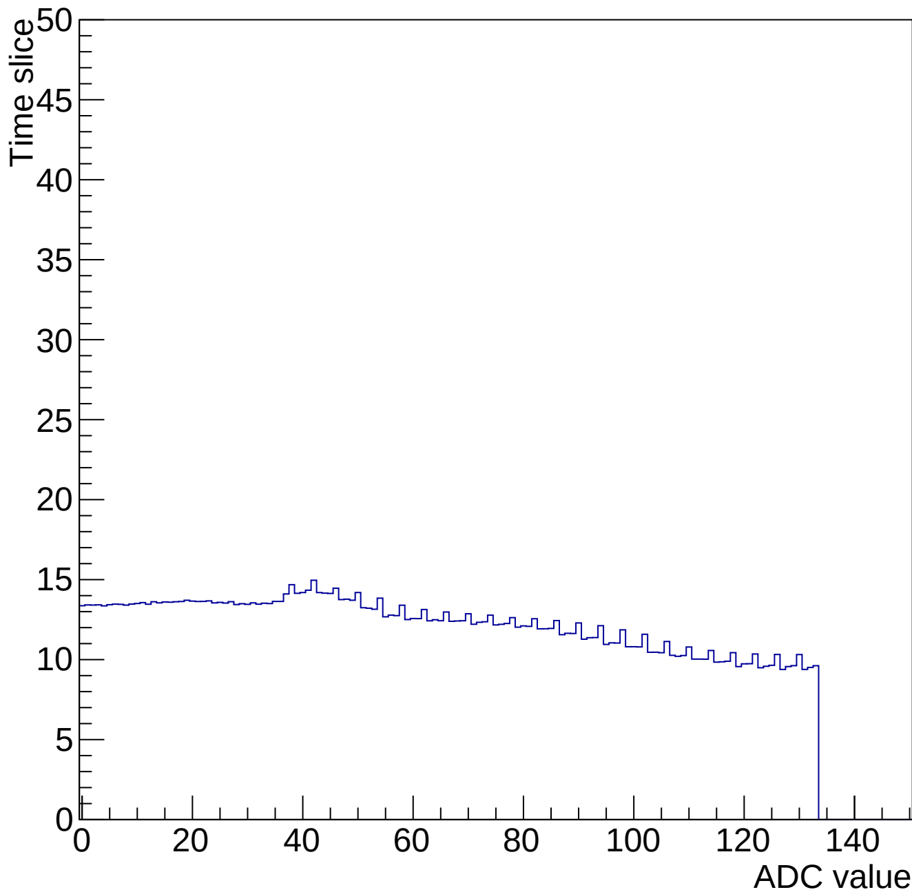
Time mcm 2003 chip 3 chan 12 34649-gain0-shaper0
