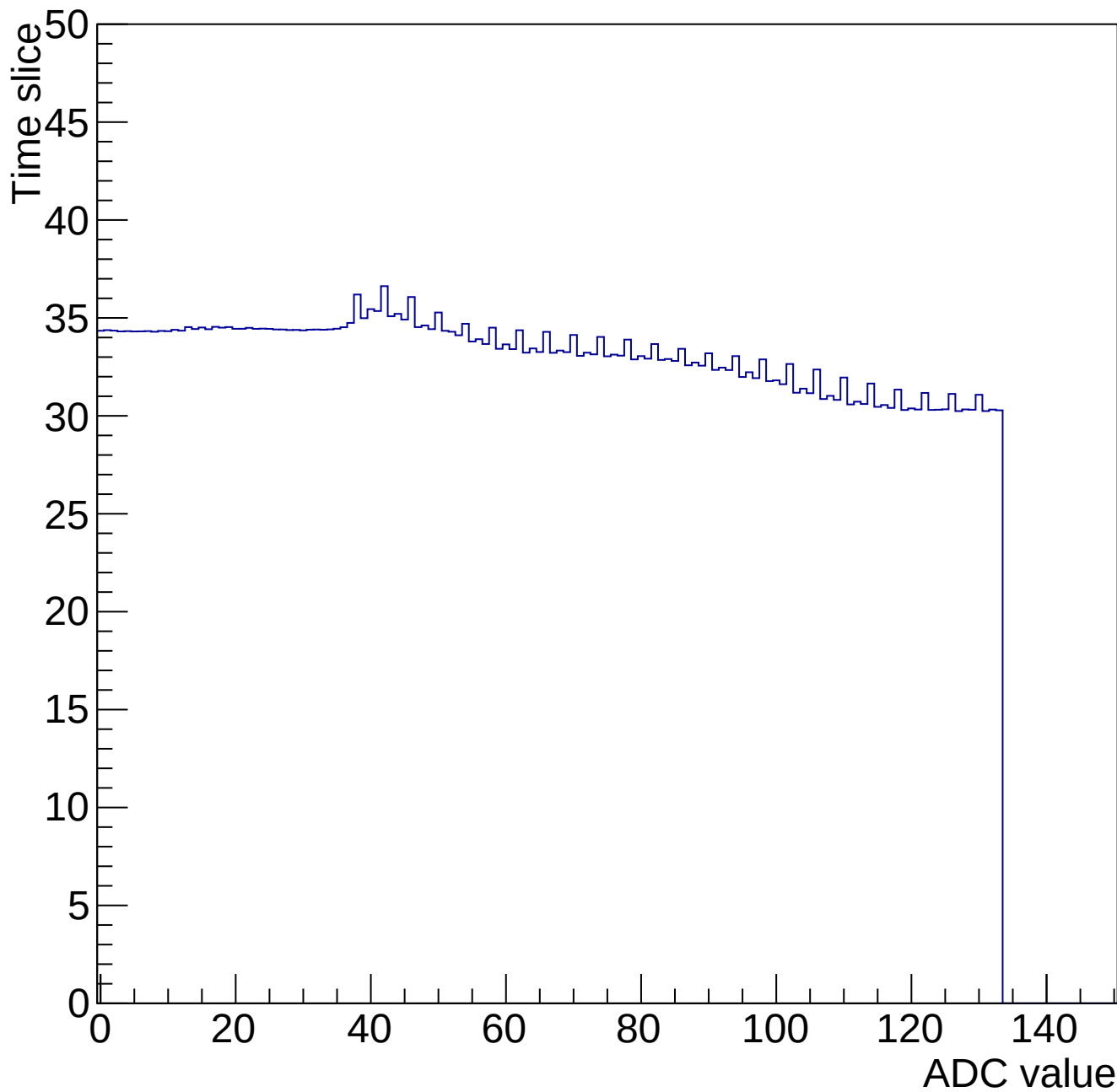
Time mcm 2003 chip 3 chan 4 34649-gain0-shaper0
