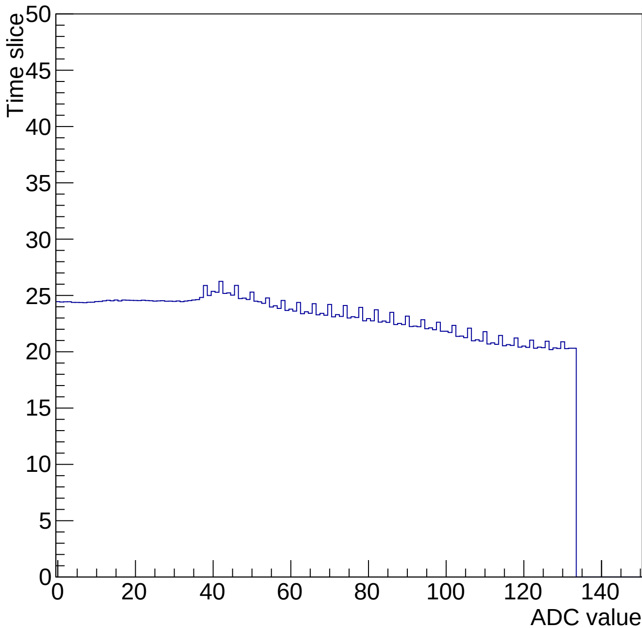
Time mcm 2003 chip 3 chan 10 34649-gain0-shaper0
