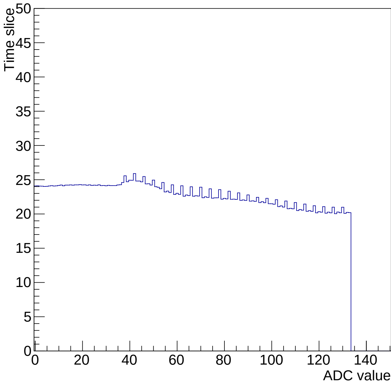
Time mcm 2003 chip 3 chan 2 34649-gain0-shaper0
