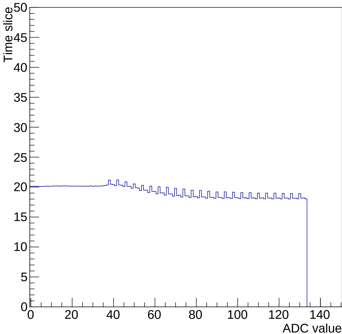
Time mcm 2003 chip 3 chan 5 34662-gain0-shaper6
