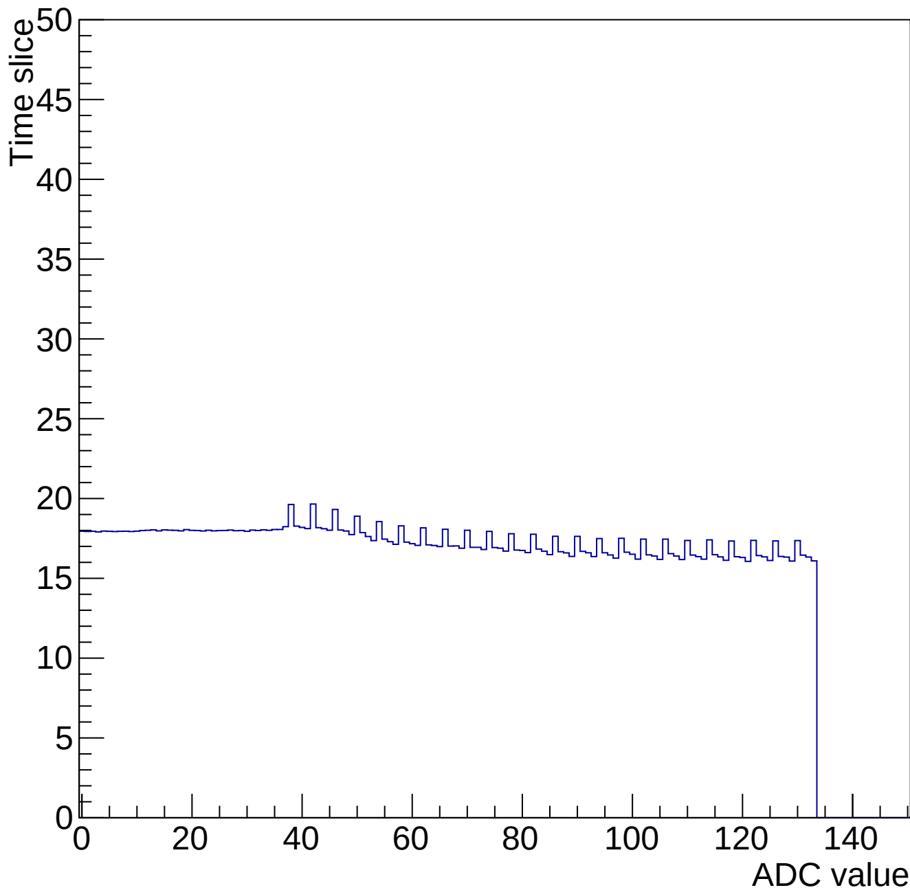
Time mcm 2003 chip 3 chan 8 34662-gain0-shaper6
