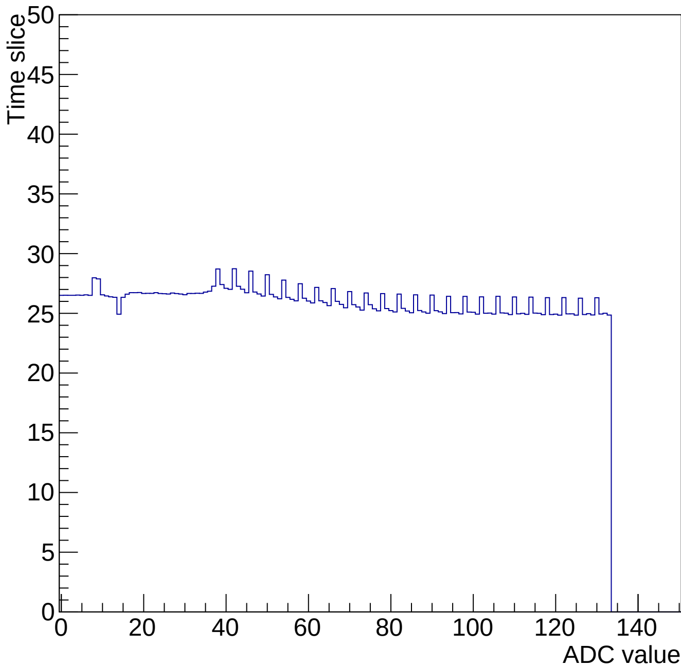
Time mcm 2003 chip 3 chan 0 34662-gain0-shaper6
