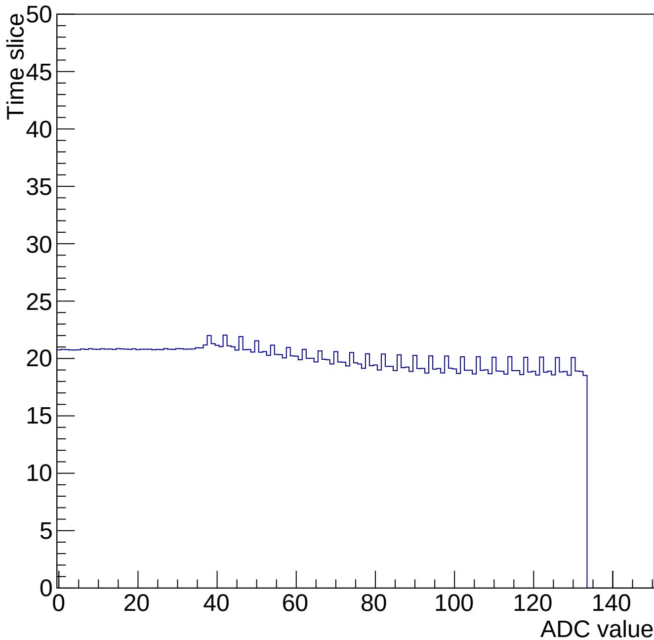
Time mcm 2003 chip 3 chan 2 34662-gain0-shaper6
