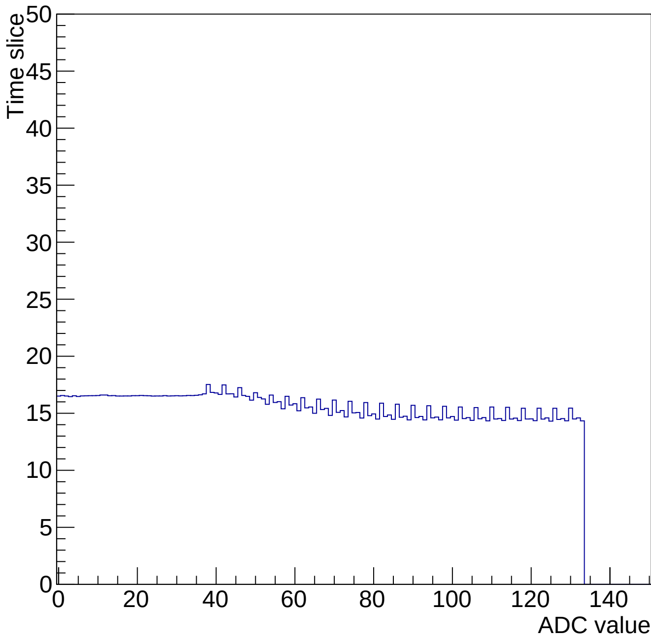
Time mcm 2003 chip 3 chan 13 34662-gain0-shaper6
