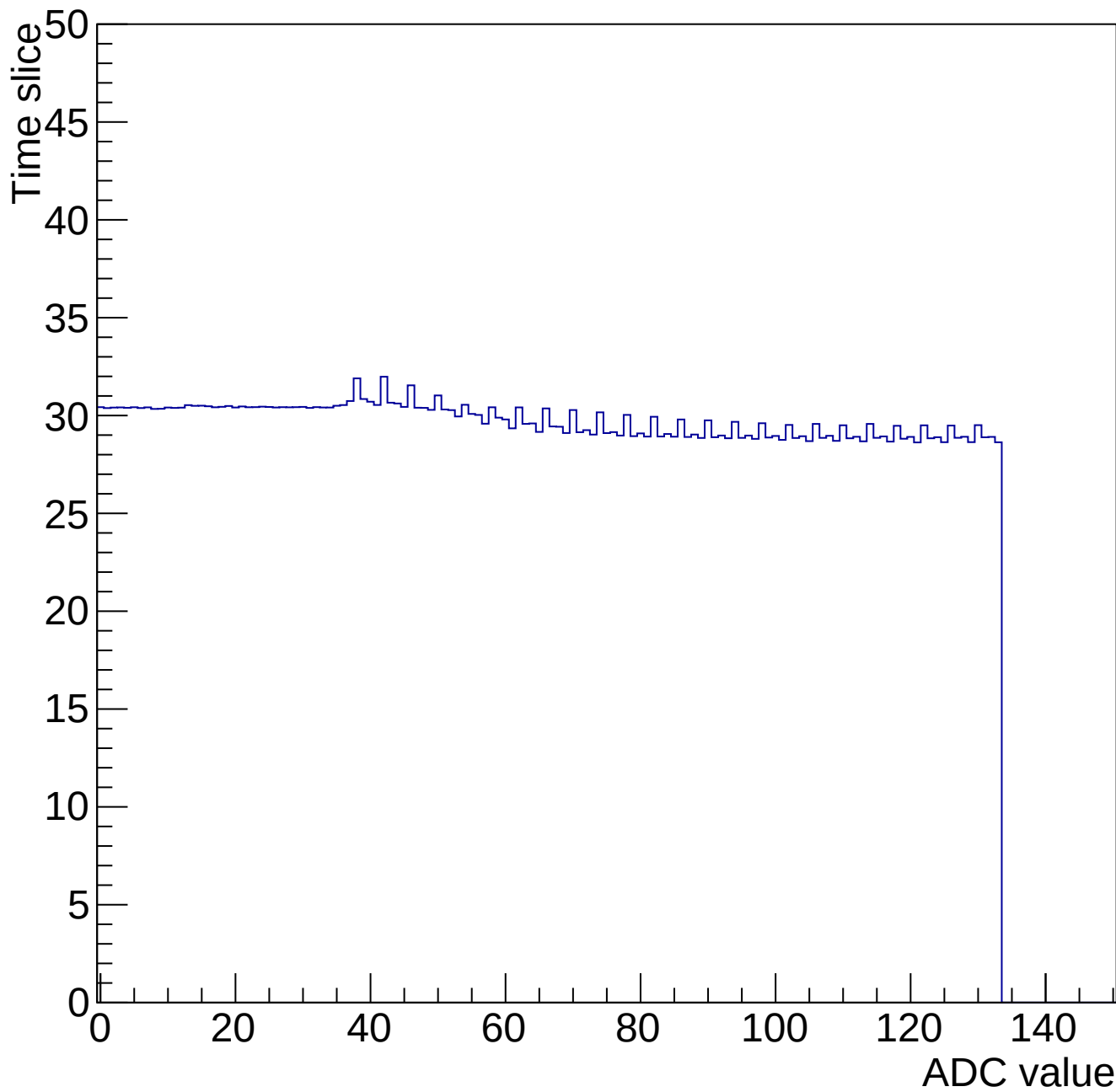
Time mcm 2003 chip 3 chan 4 34662-gain0-shaper6
