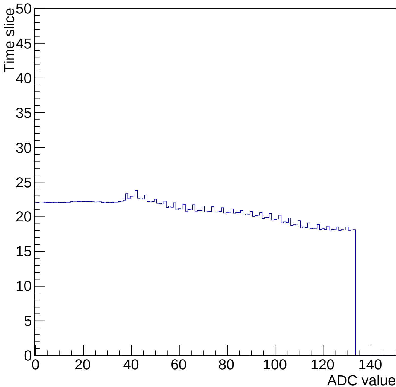
Time mcm 2004 chip 4 chan 2 34651-gain0-shaper0
