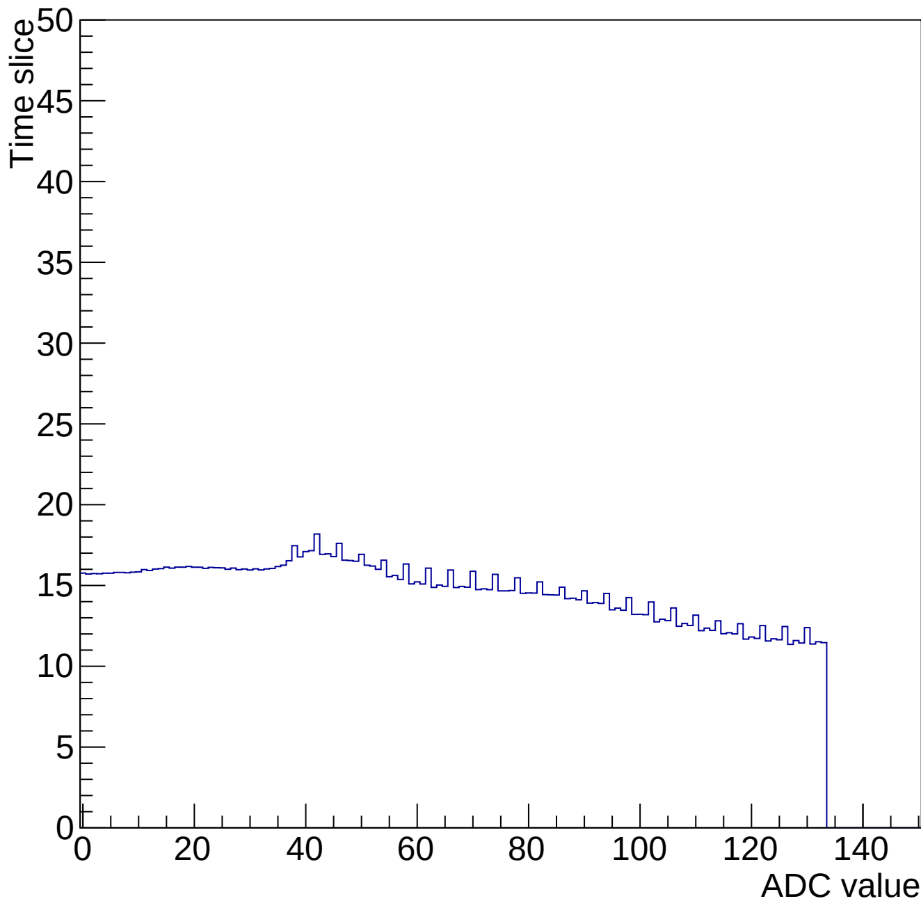
Time mcm 2004 chip 4 chan 8 34651-gain0-shaper0
