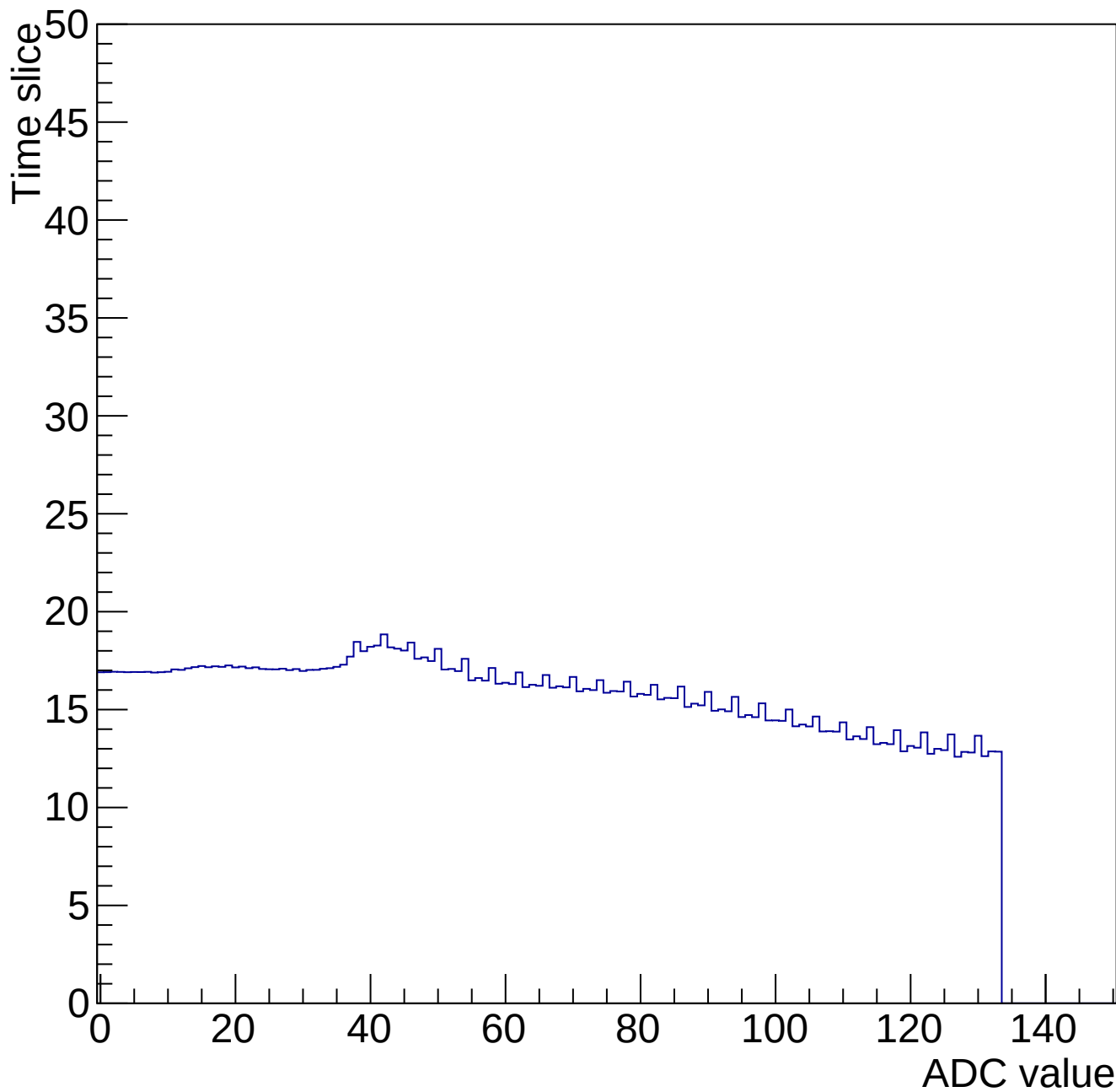
Time mcm 2004 chip 4 chan 5 34651-gain0-shaper0
