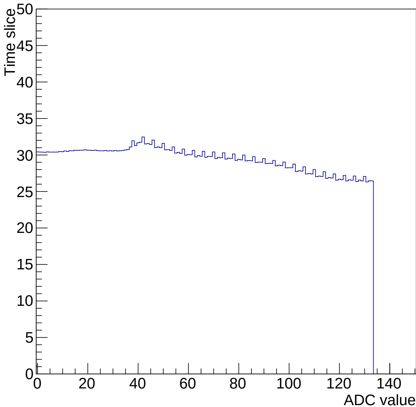
Time mcm 2004 chip 4 chan 7 34651-gain0-shaper0
