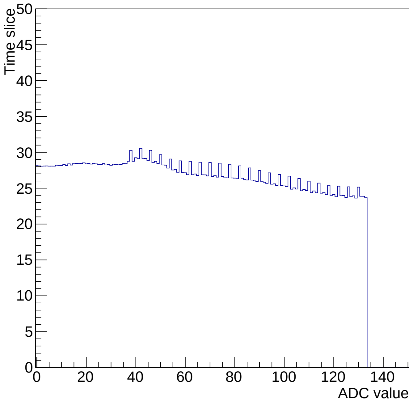
Time mcm 2005 chip 5 chan 0 34653-gain0-shaper0
