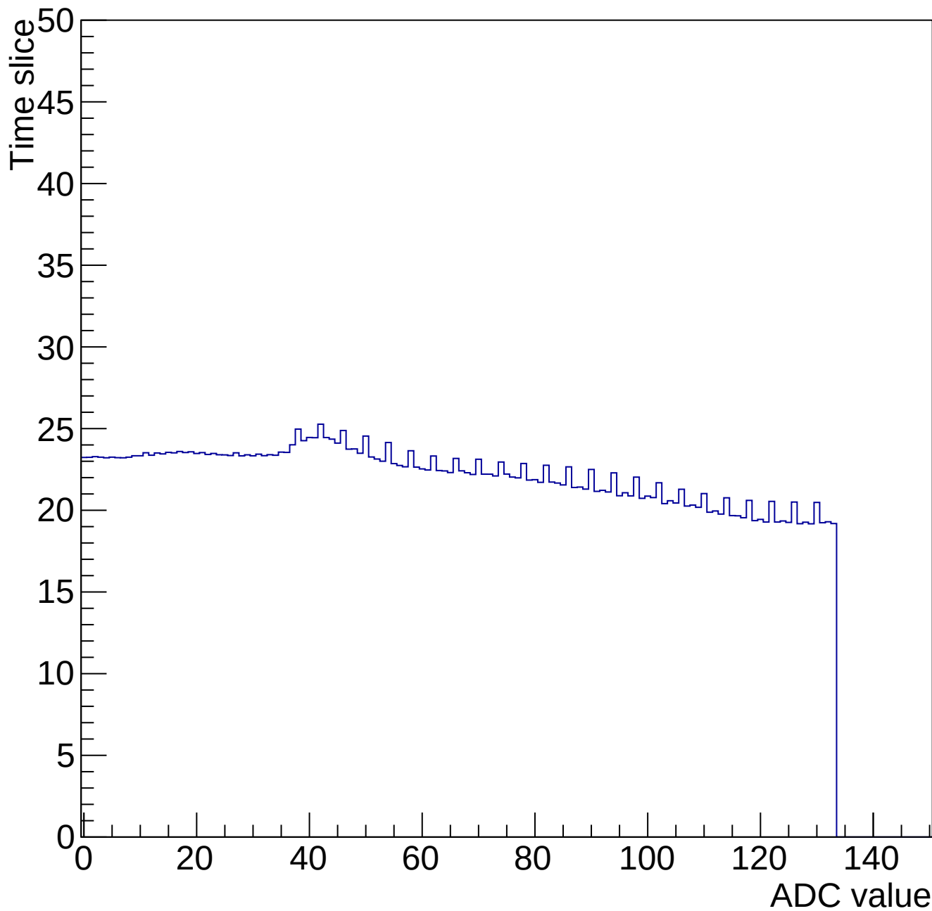
Time mcm 2005 chip 5 chan 8 34653-gain0-shaper0
