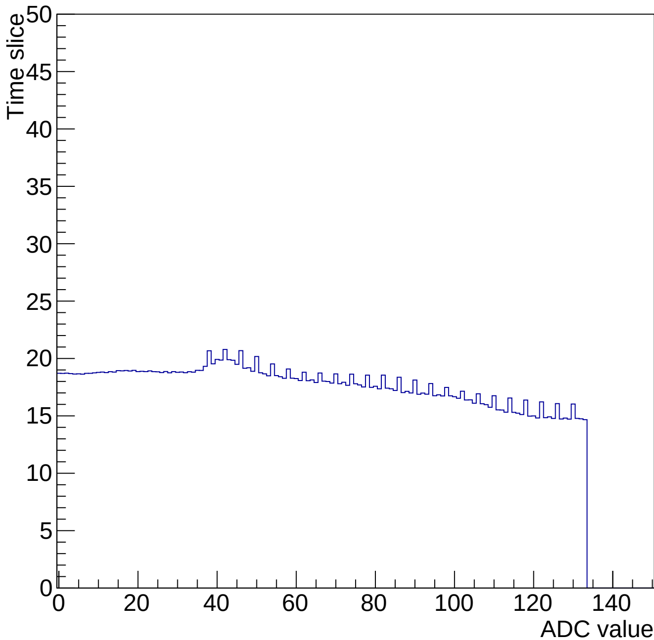
Time mcm 2005 chip 5 chan 14 34653-gain0-shaper0
