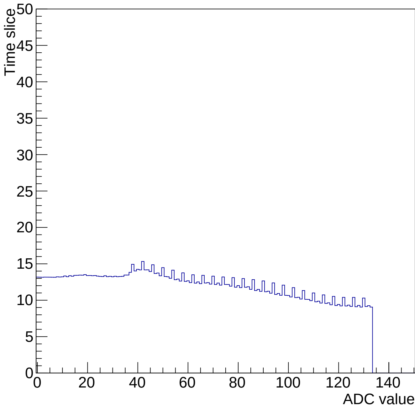
Time mcm 2005 chip 5 chan 4 34653-gain0-shaper0
