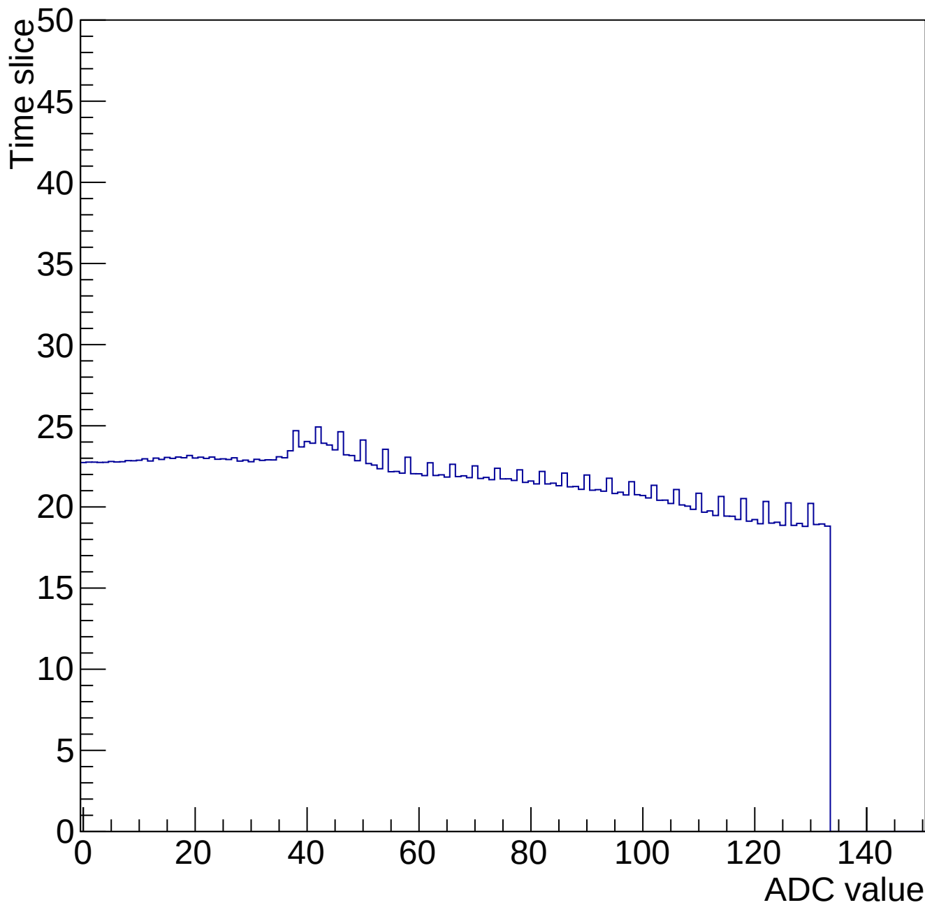
Time mcm 2005 chip 5 chan 5 34653-gain0-shaper0
