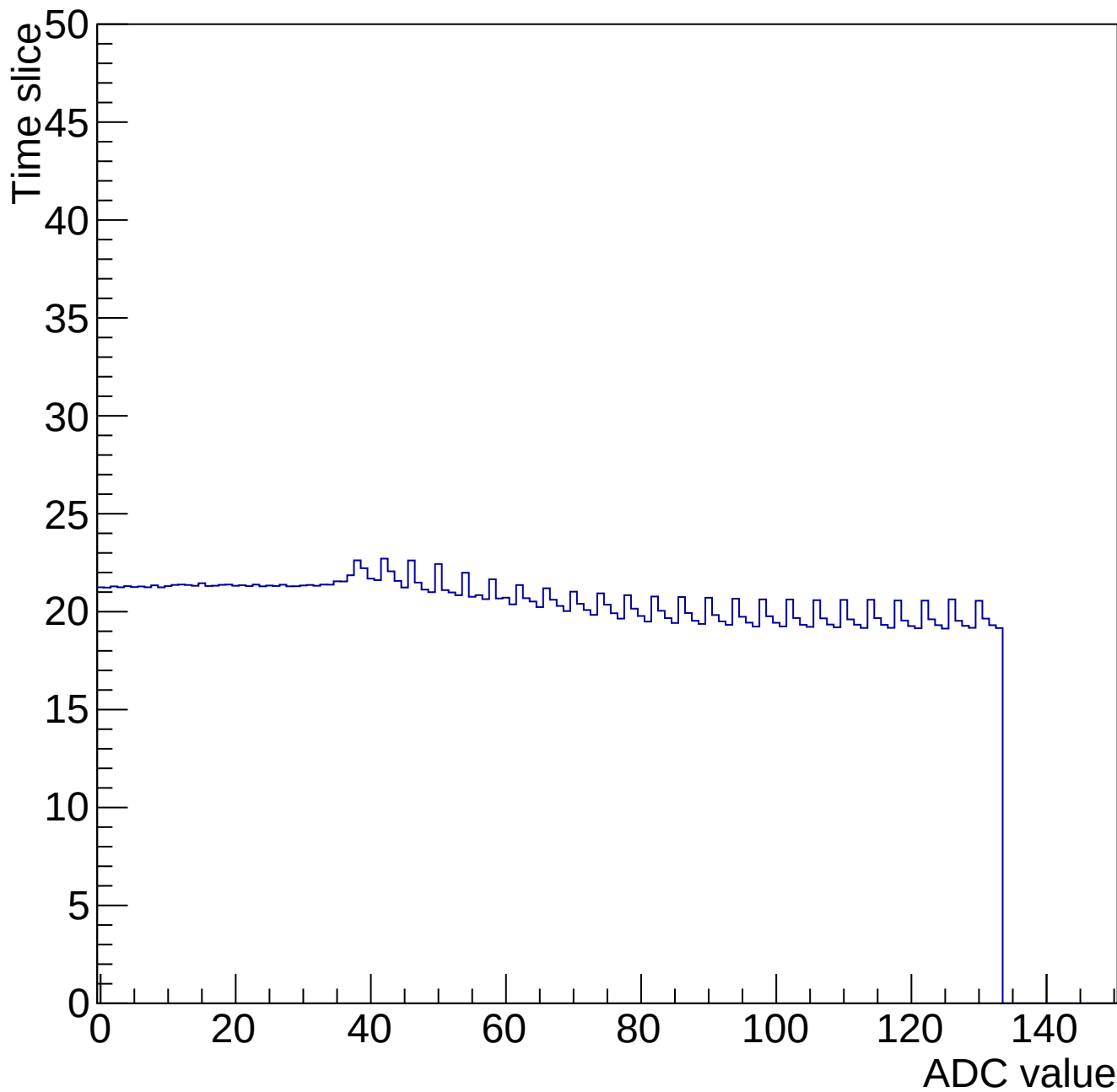
Time mcm 2005 chip 5 chan 8 34664-gain0-shaper6
