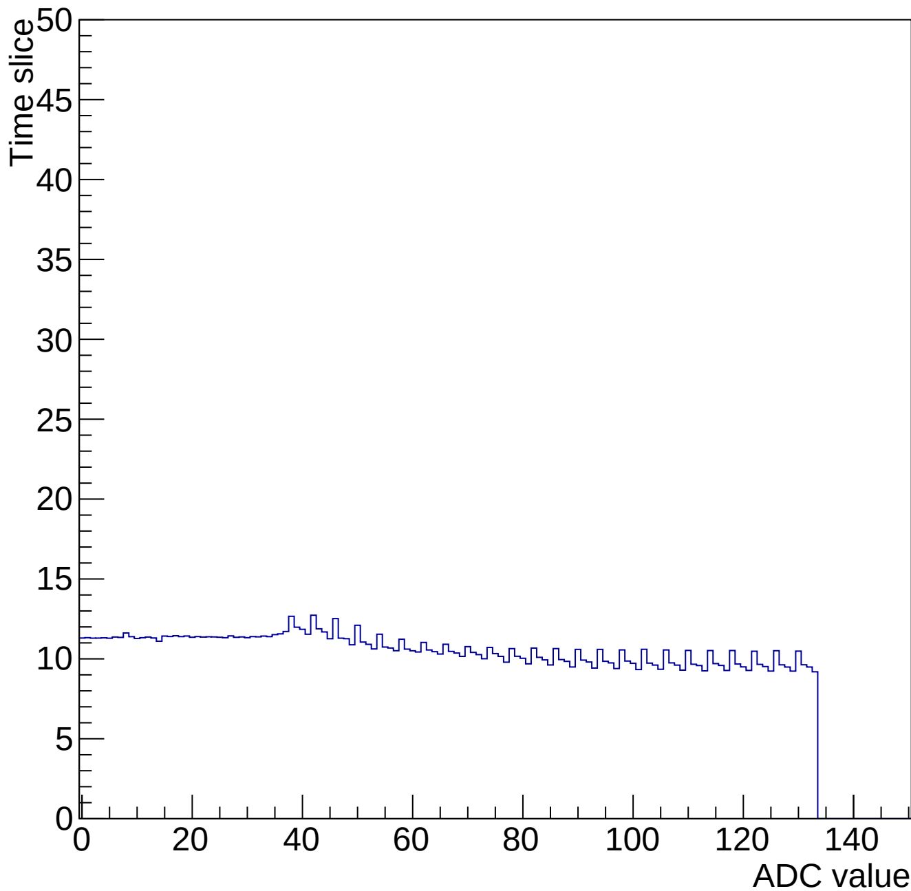
Time mcm 2005 chip 5 chan 13 34664-gain0-shaper6
