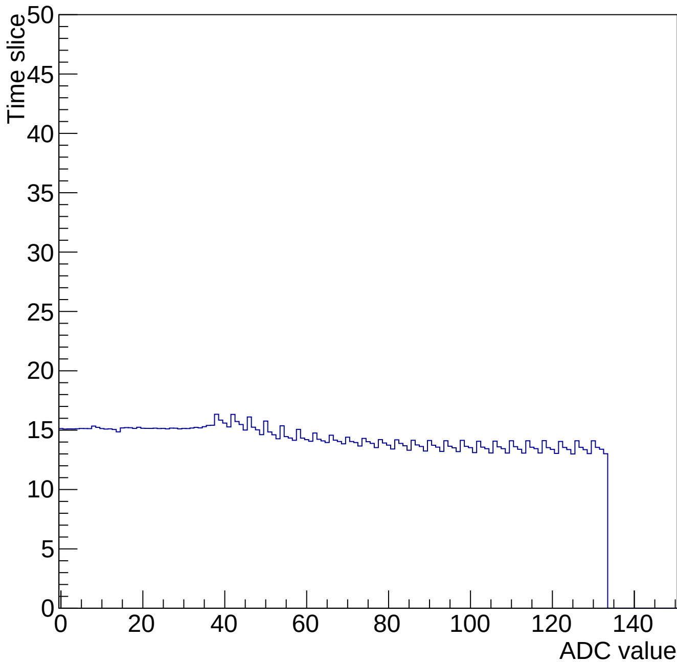
Time mcm 2005 chip 5 chan 9 34664-gain0-shaper6
