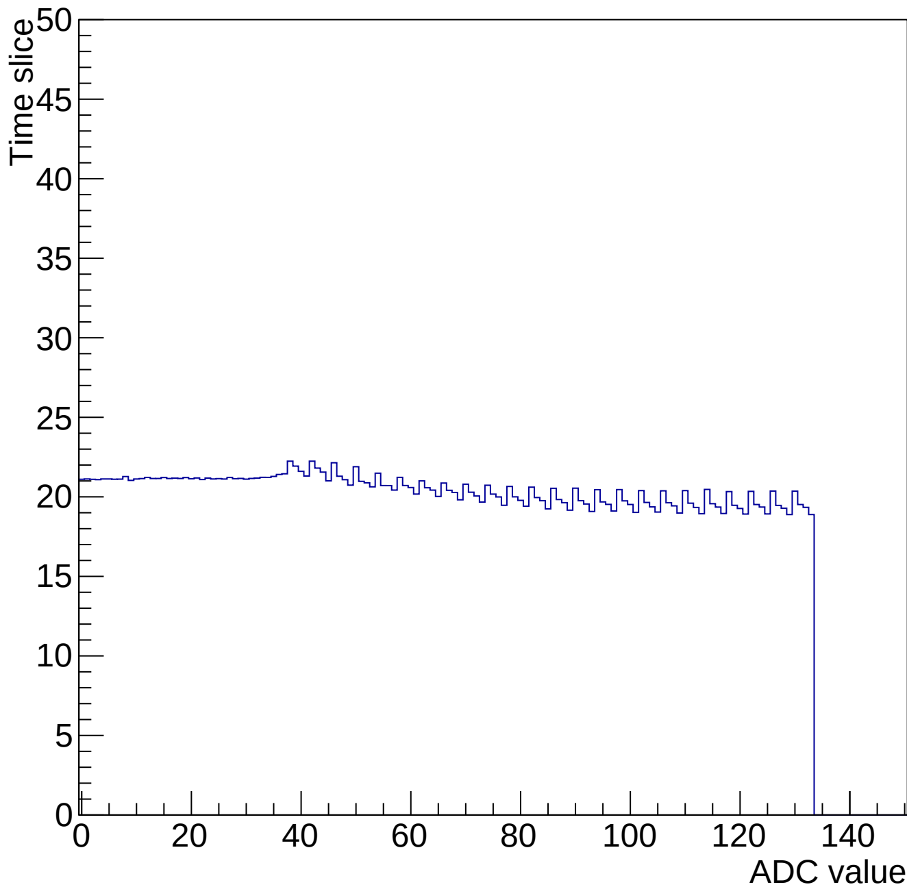
Time mcm 2005 chip 5 chan 2 34664-gain0-shaper6
