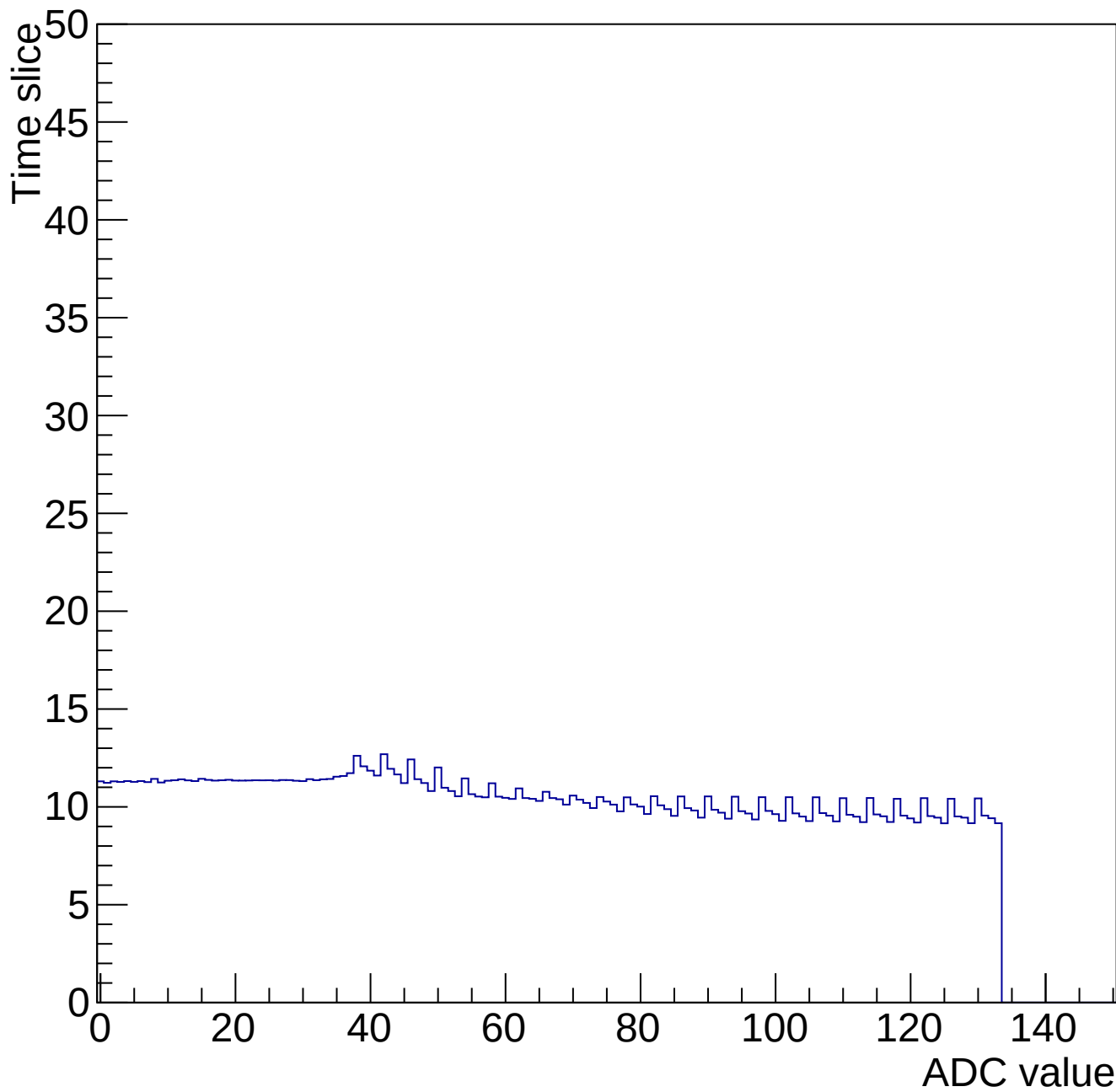
Time mcm 2005 chip 5 chan 14 34664-gain0-shaper6
