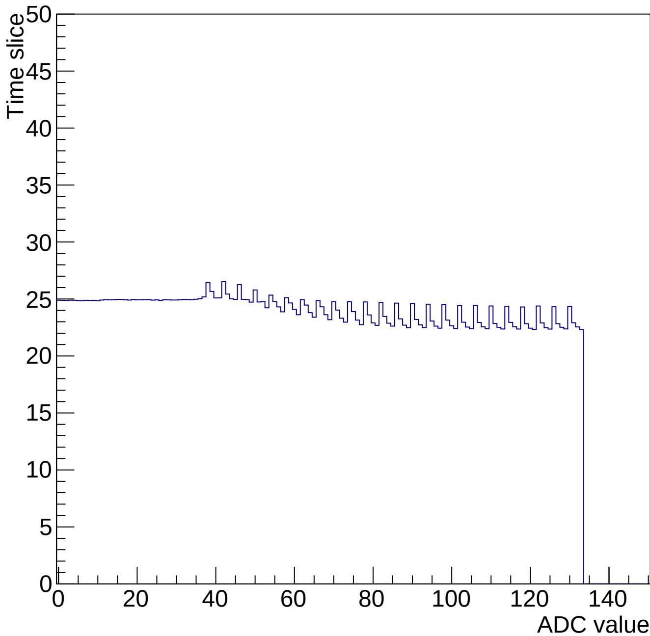
Time mcm 2005 chip 5 chan 0 34664-gain0-shaper6
