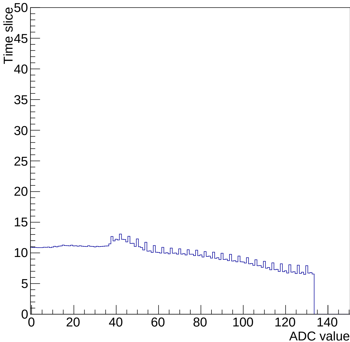
Time mcm 2006 chip 6 chan 4 34655-gain0-shaper0
