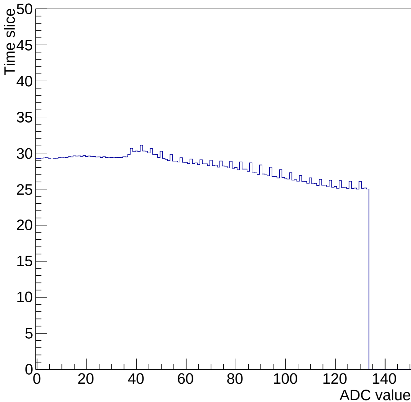
Time mcm 2006 chip 6 chan 5 34655-gain0-shaper0
