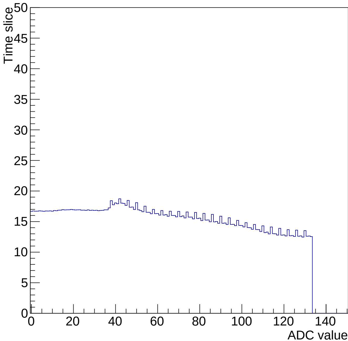
Time mcm 2006 chip 6 chan 14 34655-gain0-shaper0
