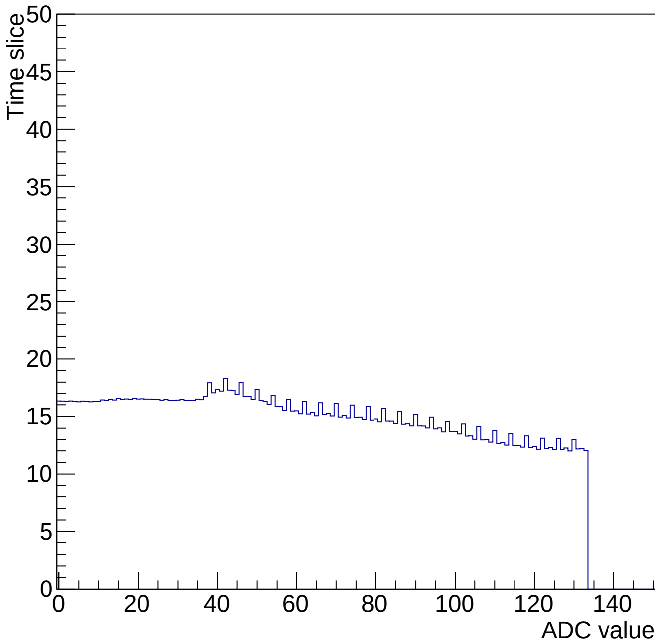
Time mcm 2006 chip 6 chan 3 34655-gain0-shaper0
