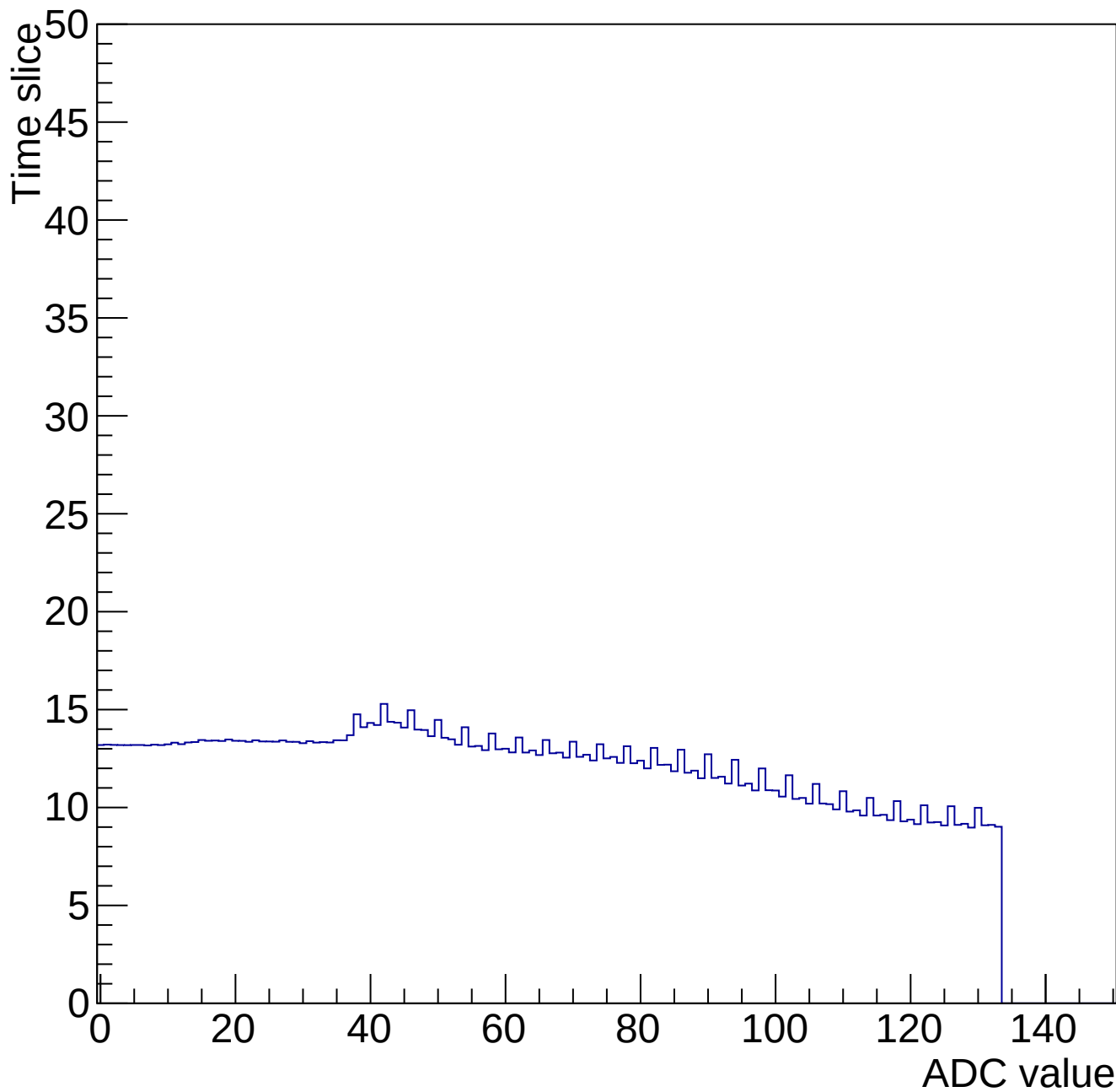
Time mcm 2006 chip 6 chan 6 34655-gain0-shaper0
