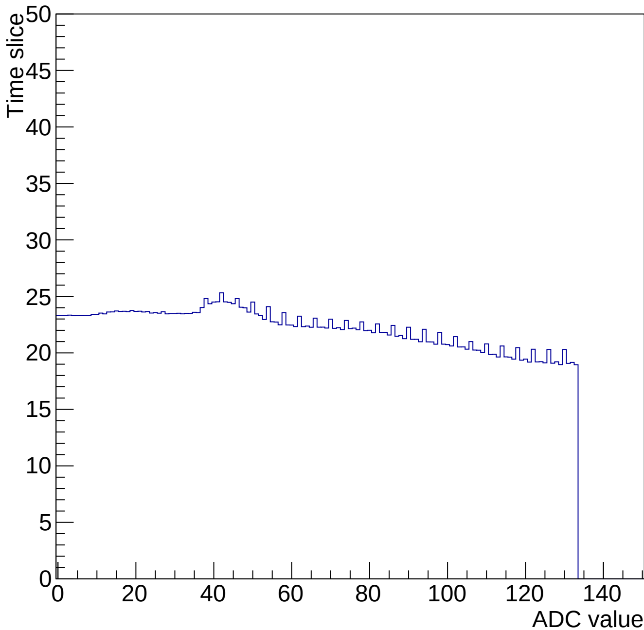
Time mcm 2006 chip 6 chan 13 34655-gain0-shaper0
