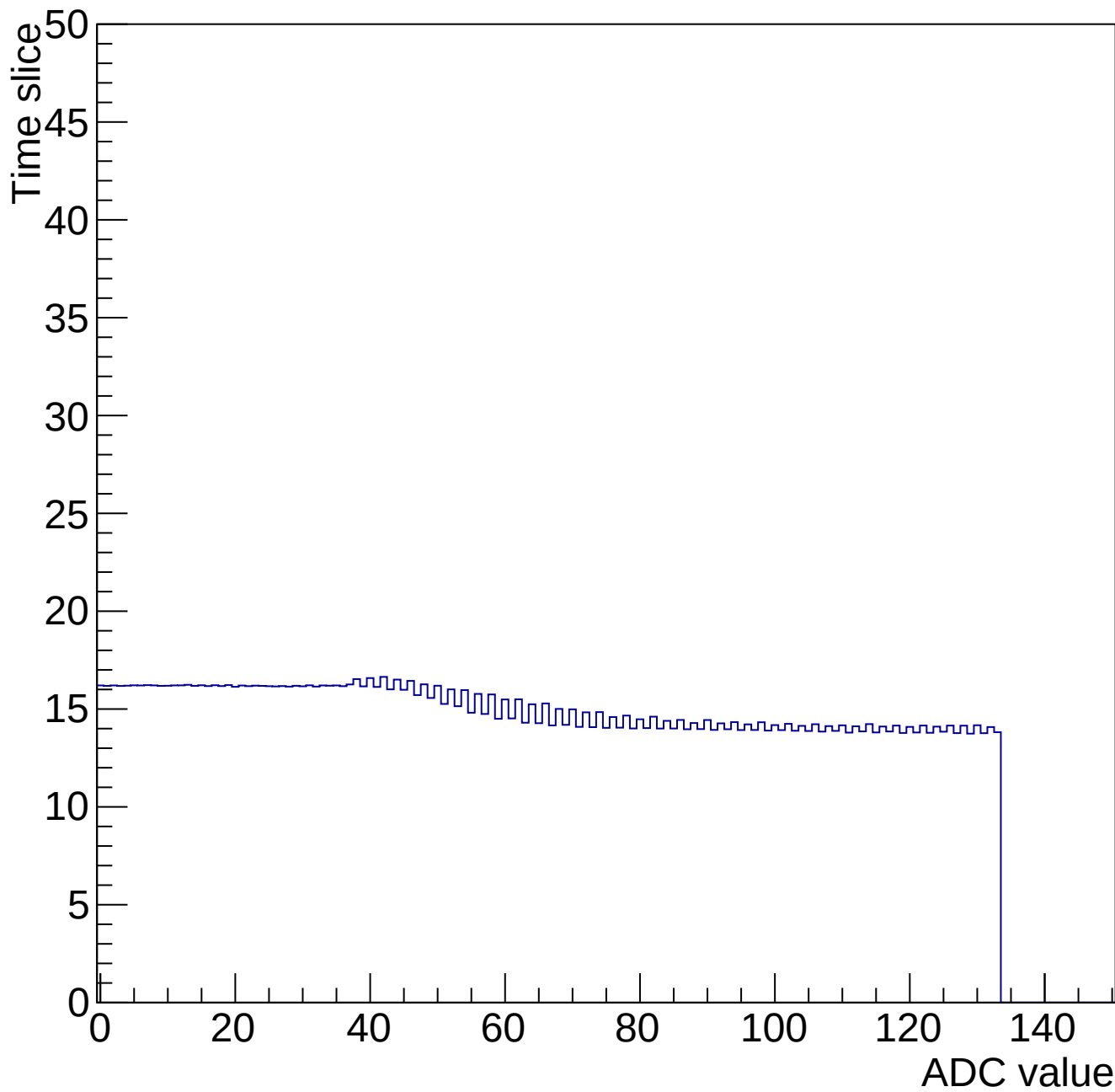
Time mcm 2006 chip 6 chan 2 34665-gain0-shaper6
