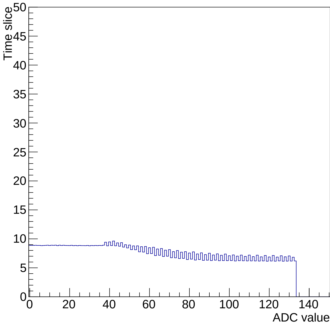
Time mcm 2006 chip 6 chan 8 34665-gain0-shaper6
