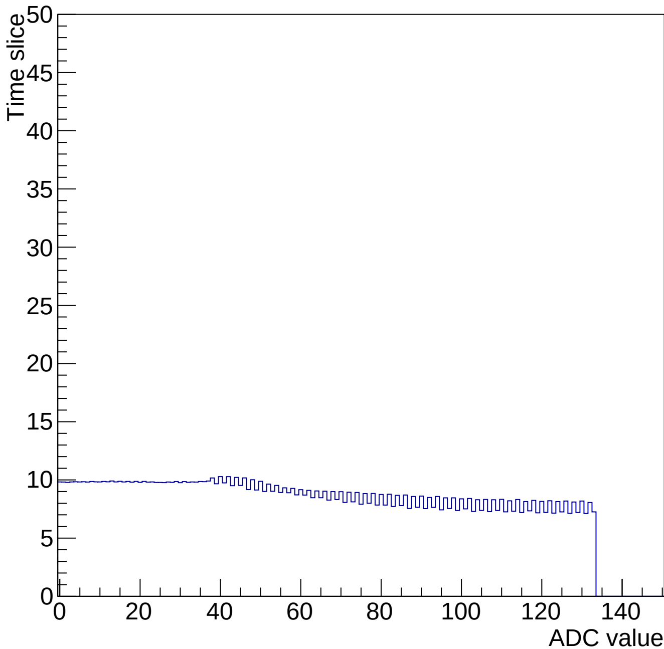
Time mcm 2006 chip 6 chan 6 34665-gain0-shaper6
