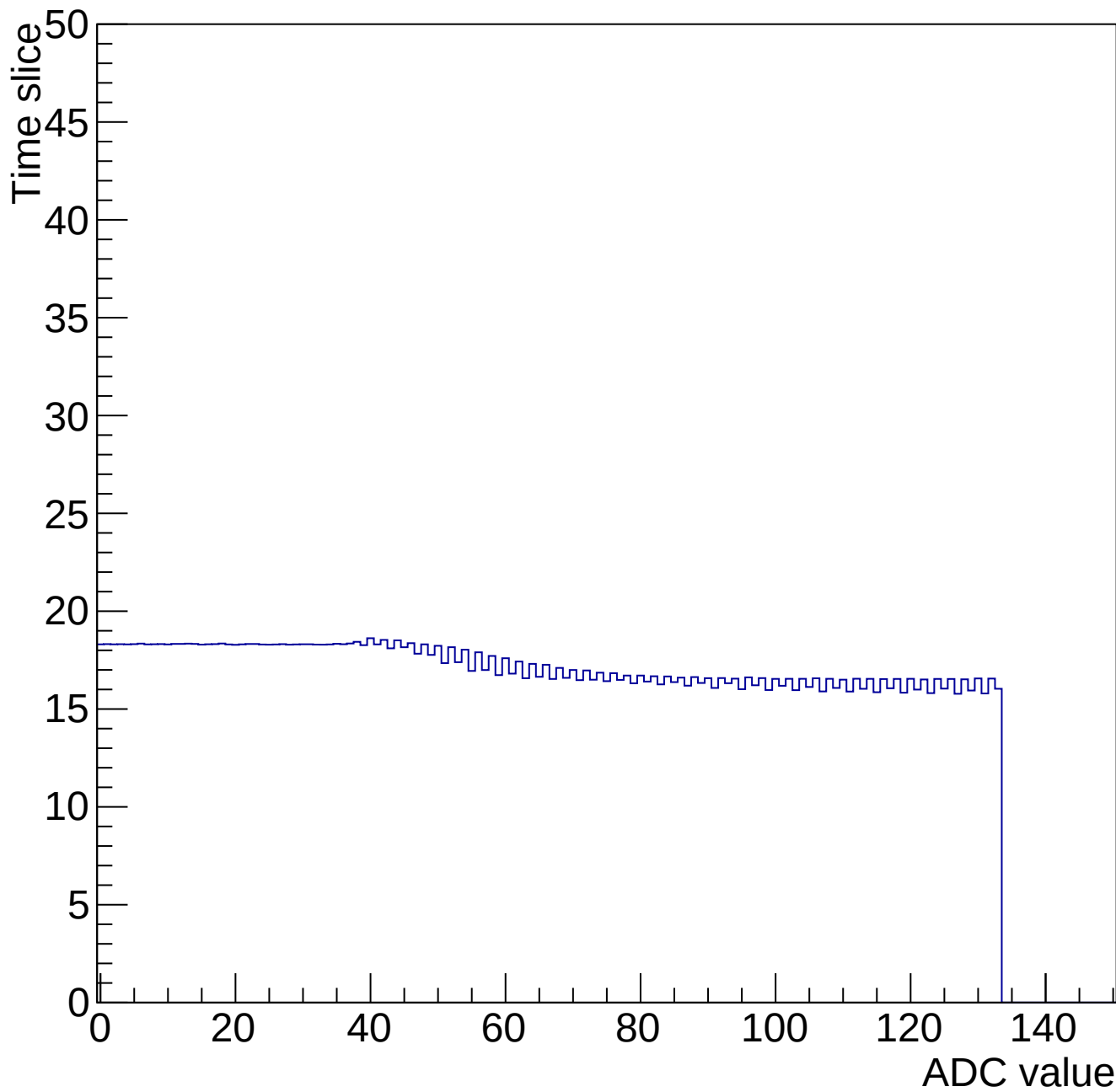
Time mcm 2006 chip 6 chan 13 34665-gain0-shaper6
