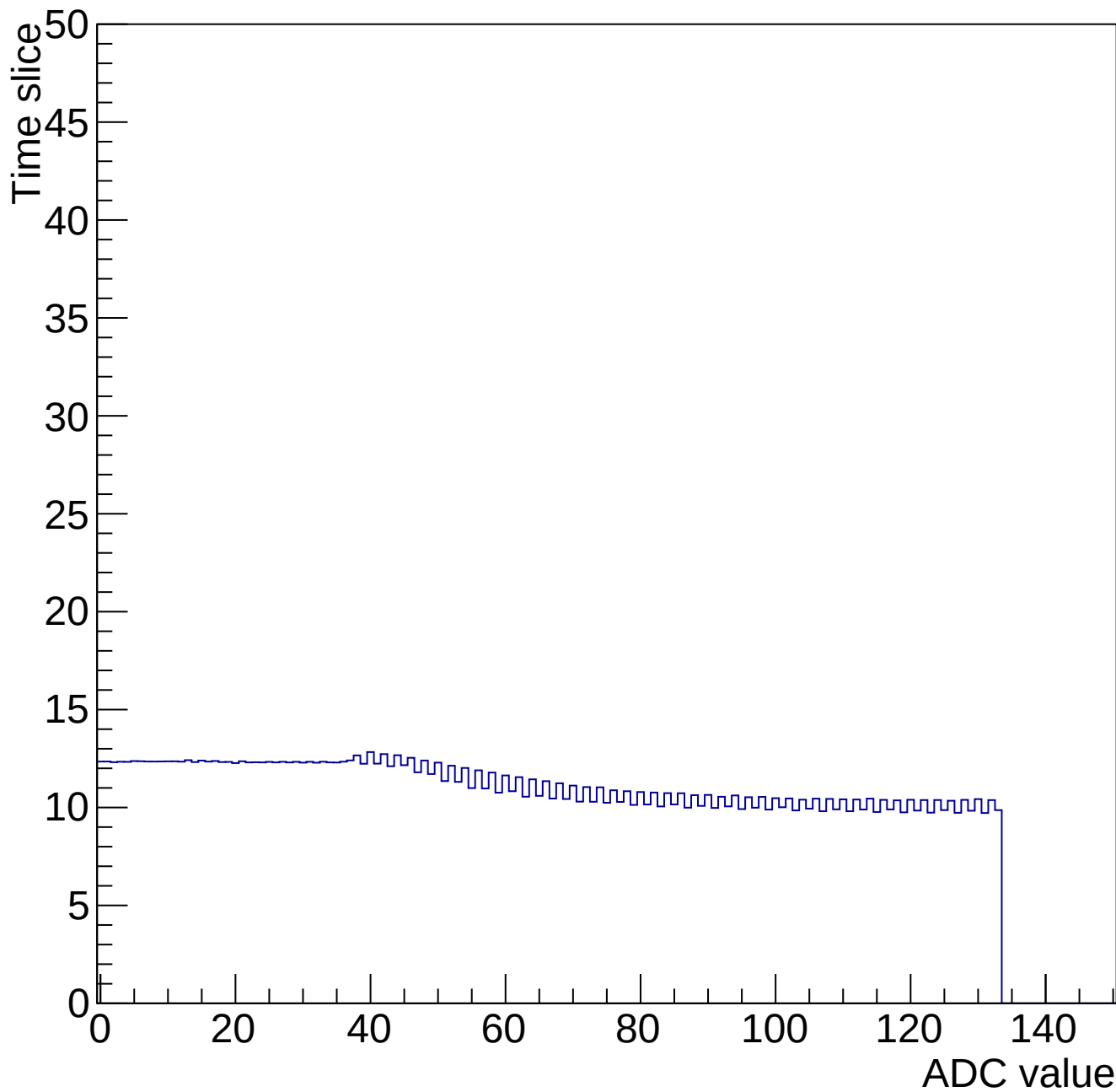
Time mcm 2006 chip 6 chan 3 34665-gain0-shaper6
