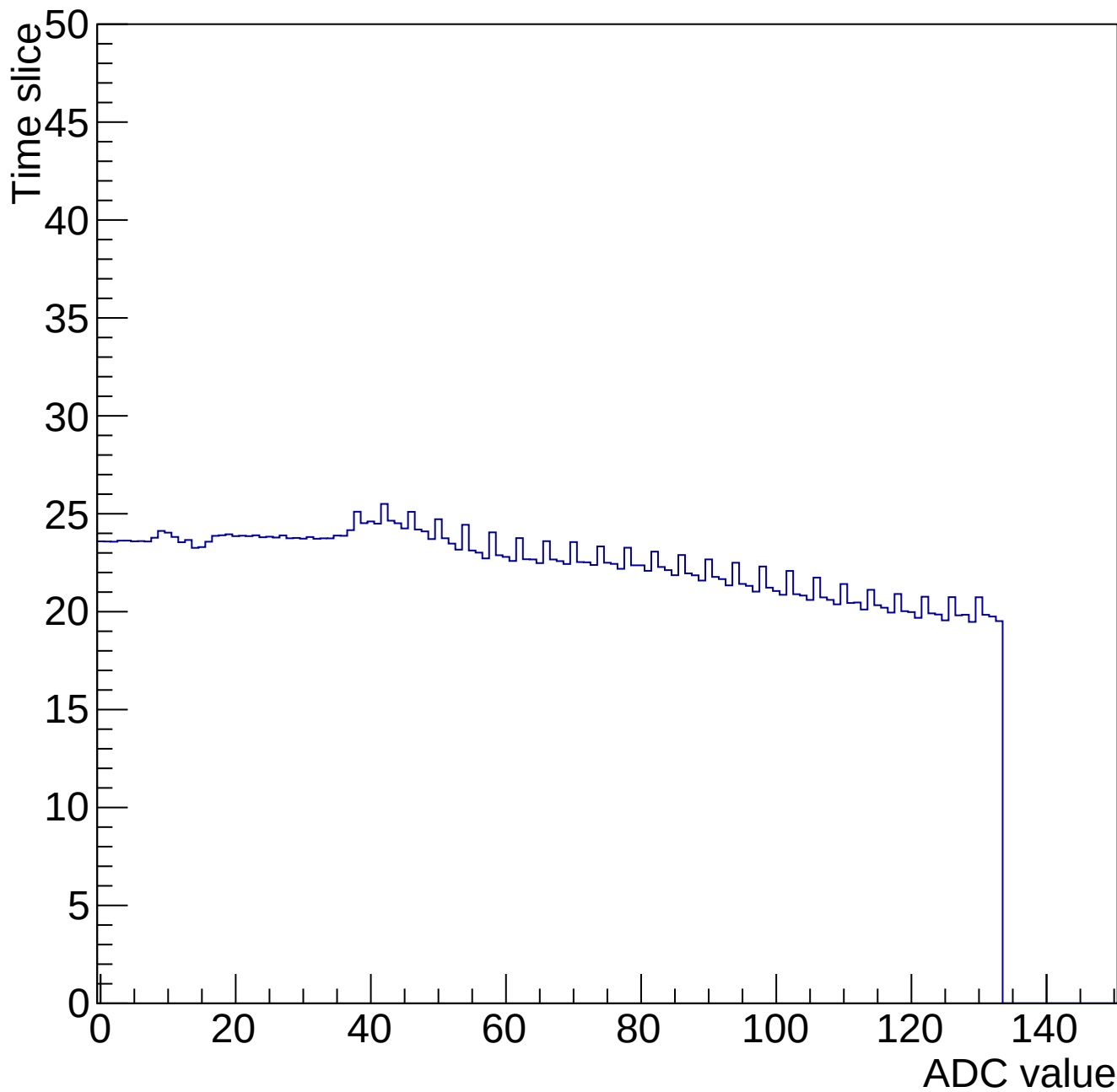
Time mcm 2007 chip 7 chan 3 34656-gain0-shaper0
