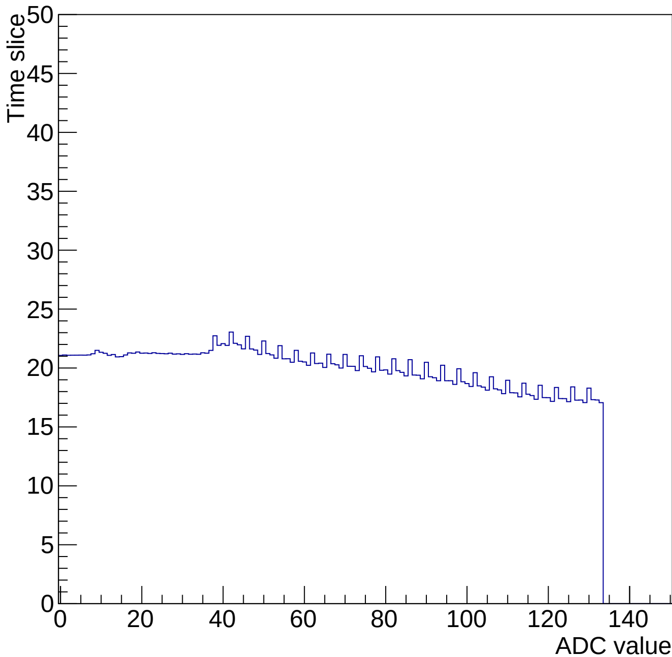
Time mcm 2007 chip 7 chan 7 34656-gain0-shaper0
