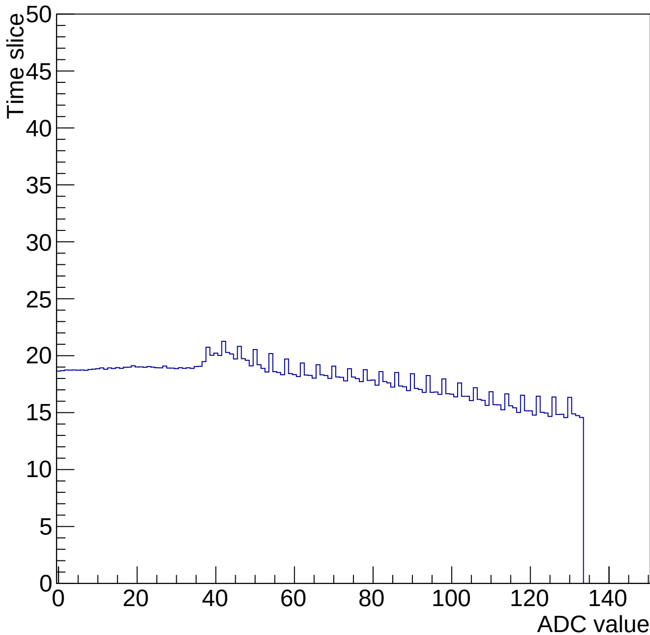
Time mcm 2007 chip 7 chan 4 34656-gain0-shaper0
