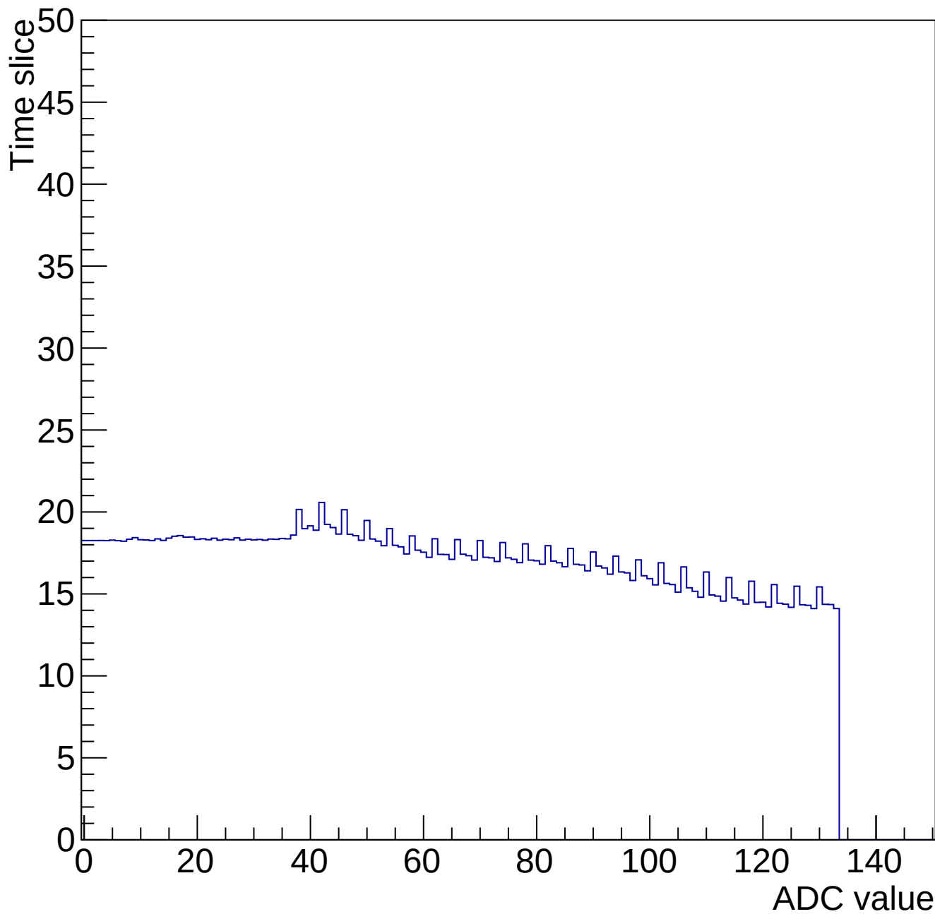
Time mcm 2007 chip 7 chan 15 34656-gain0-shaper0
