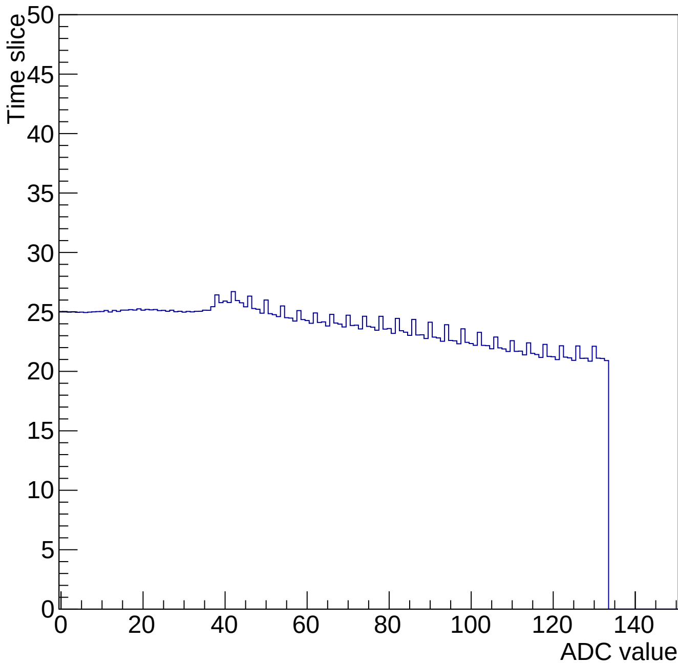
Time mcm 2007 chip 7 chan 6 34656-gain0-shaper0
