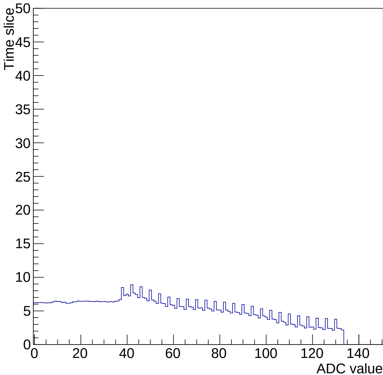
Time mcm 2007 chip 7 chan 0 34656-gain0-shaper0
