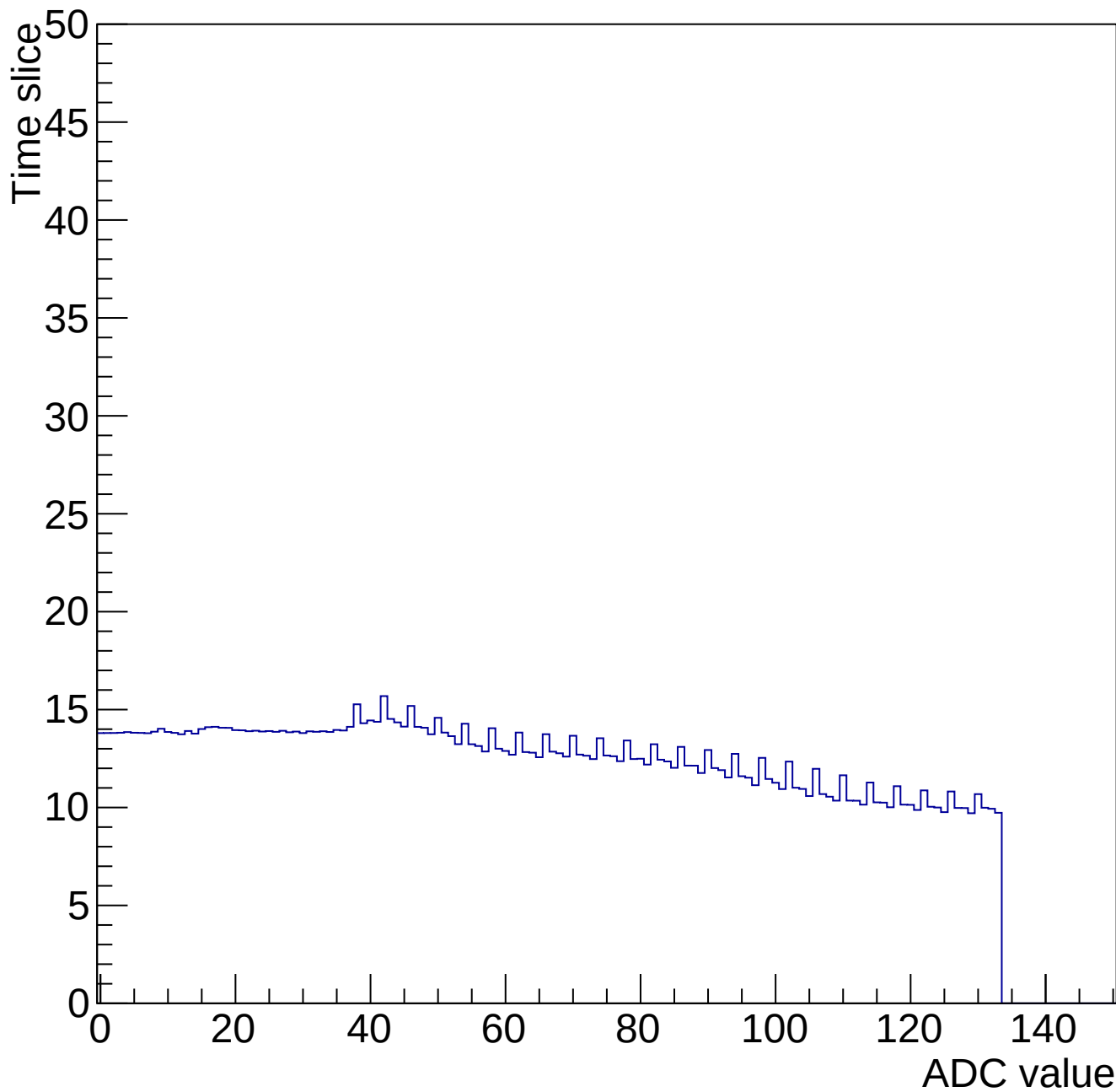
Time mcm 2007 chip 7 chan 12 34656-gain0-shaper0
