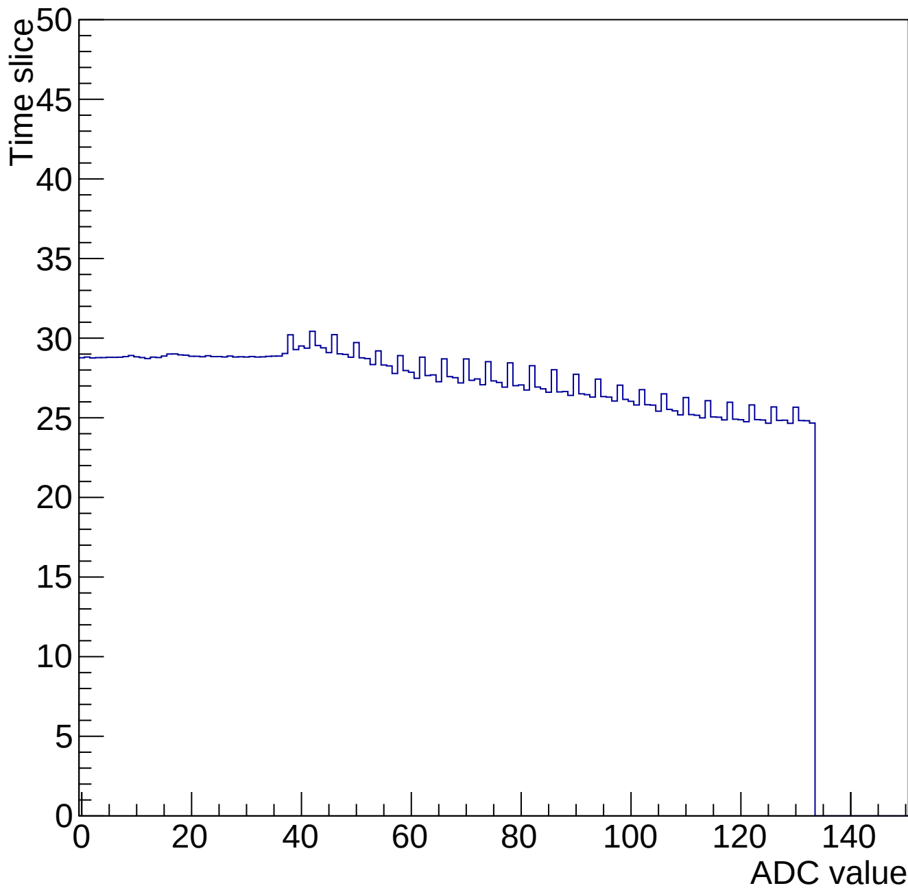
Time mcm 2007 chip 7 chan 14 34656-gain0-shaper0
