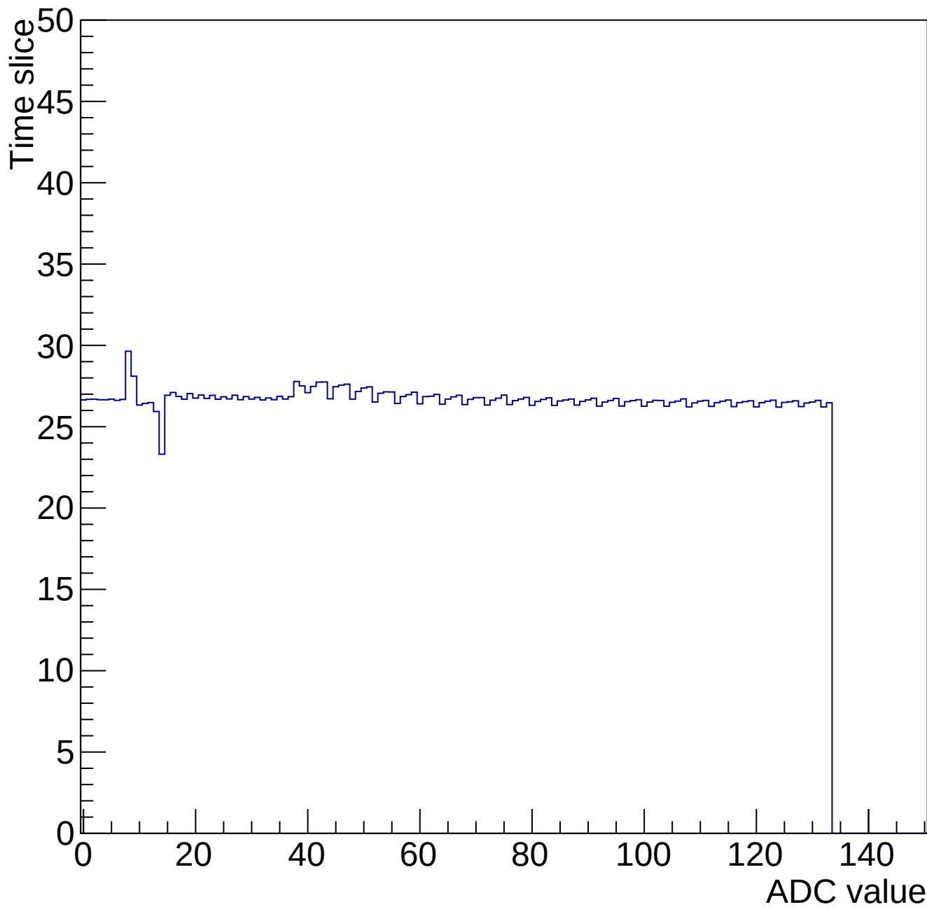
Time mcm 2000 chip 0 chan 1 34686-gain0-shaper6
