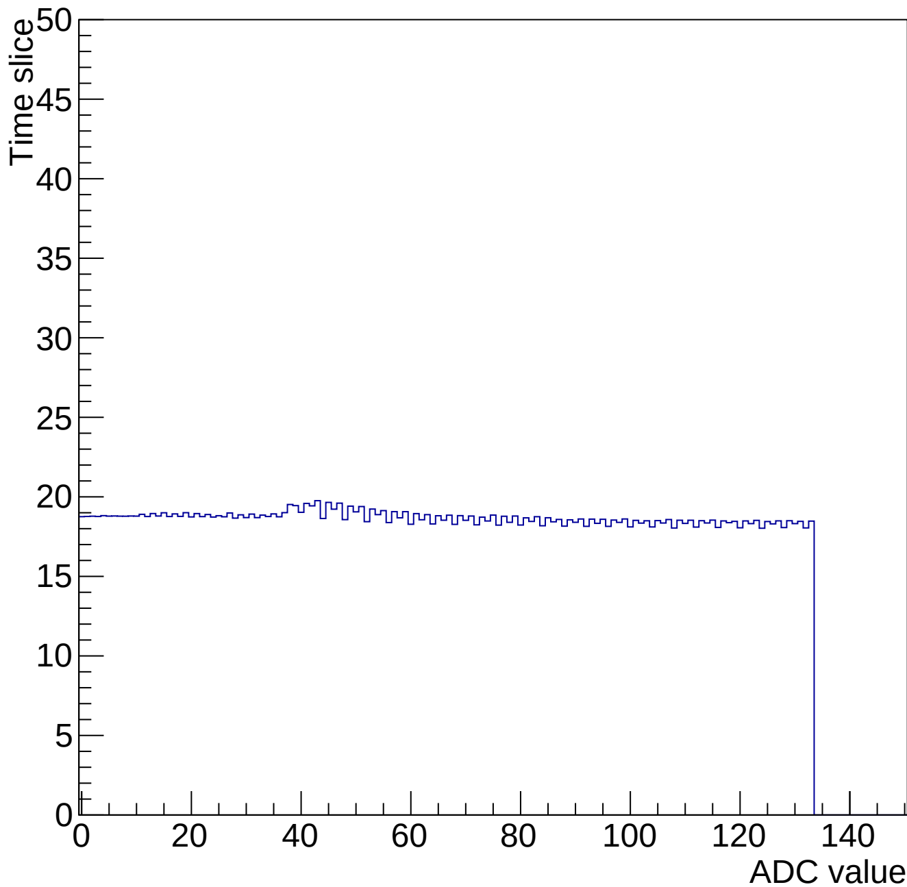
Time mcm 2000 chip 0 chan 3 34686-gain0-shaper6
