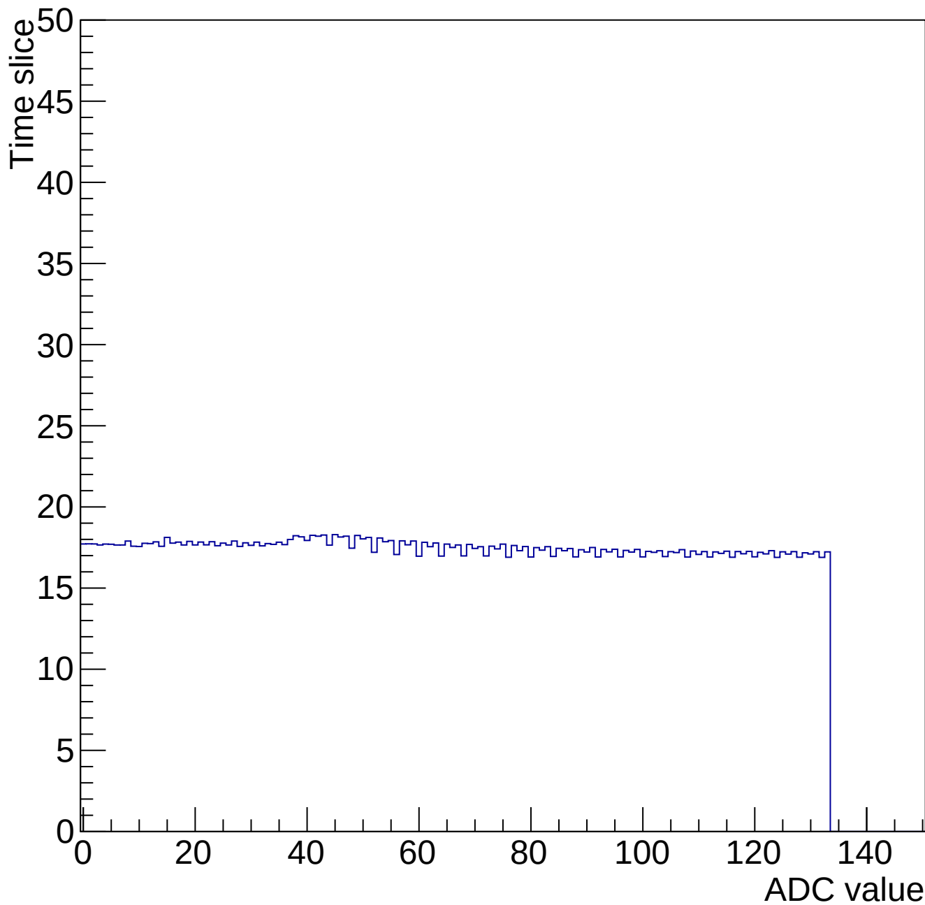
Time mcm 2000 chip 0 chan 15 34686-gain0-shaper6
