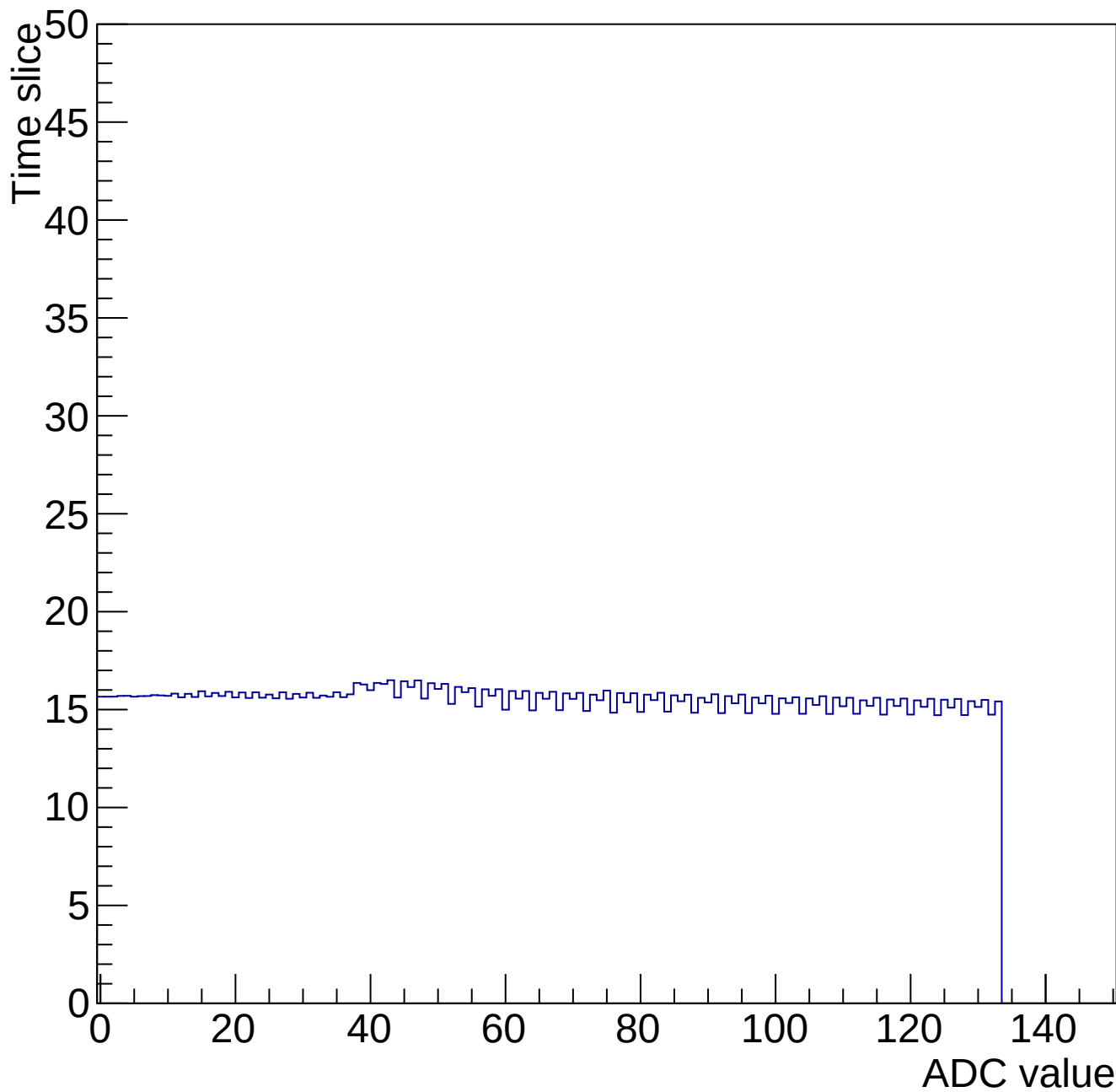
Time mcm 2000 chip 0 chan 10 34686-gain0-shaper6
