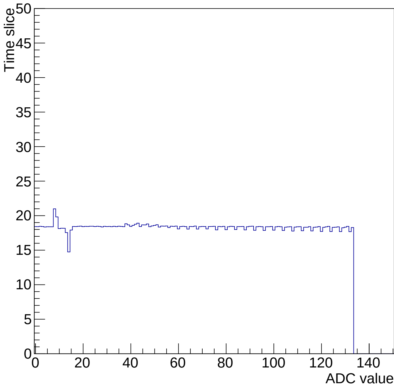
Time mcm 2000 chip 0 chan 2 34686-gain0-shaper6
