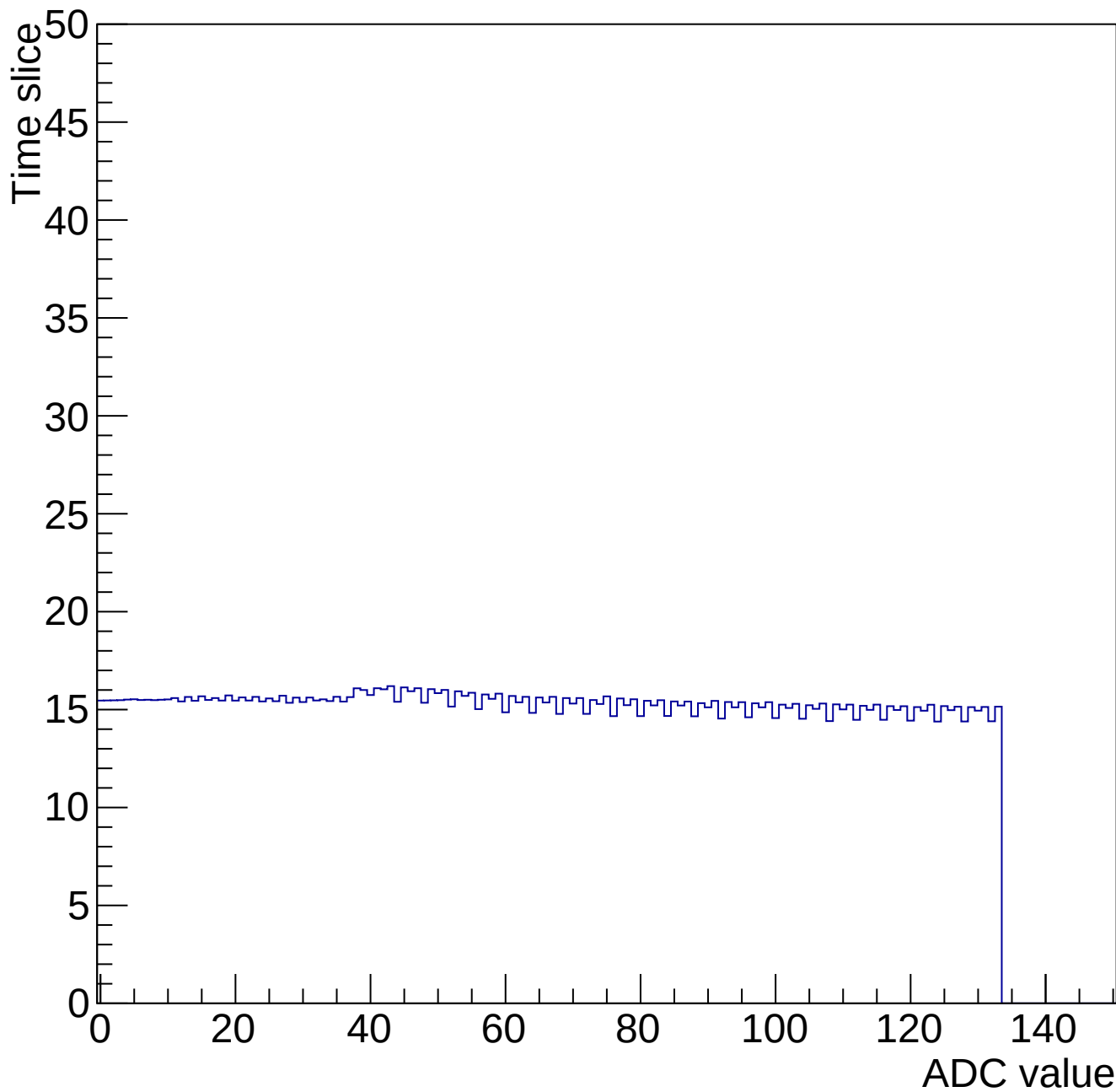
Time mcm 2000 chip 0 chan 9 34686-gain0-shaper6
