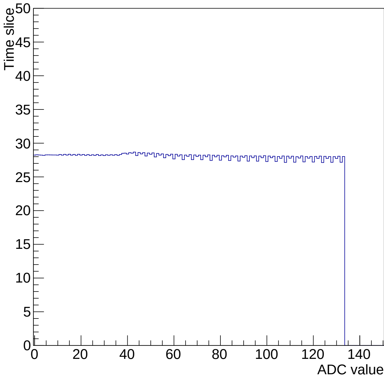
Time mcm 2000 chip 0 chan 5 34686-gain0-shaper6
