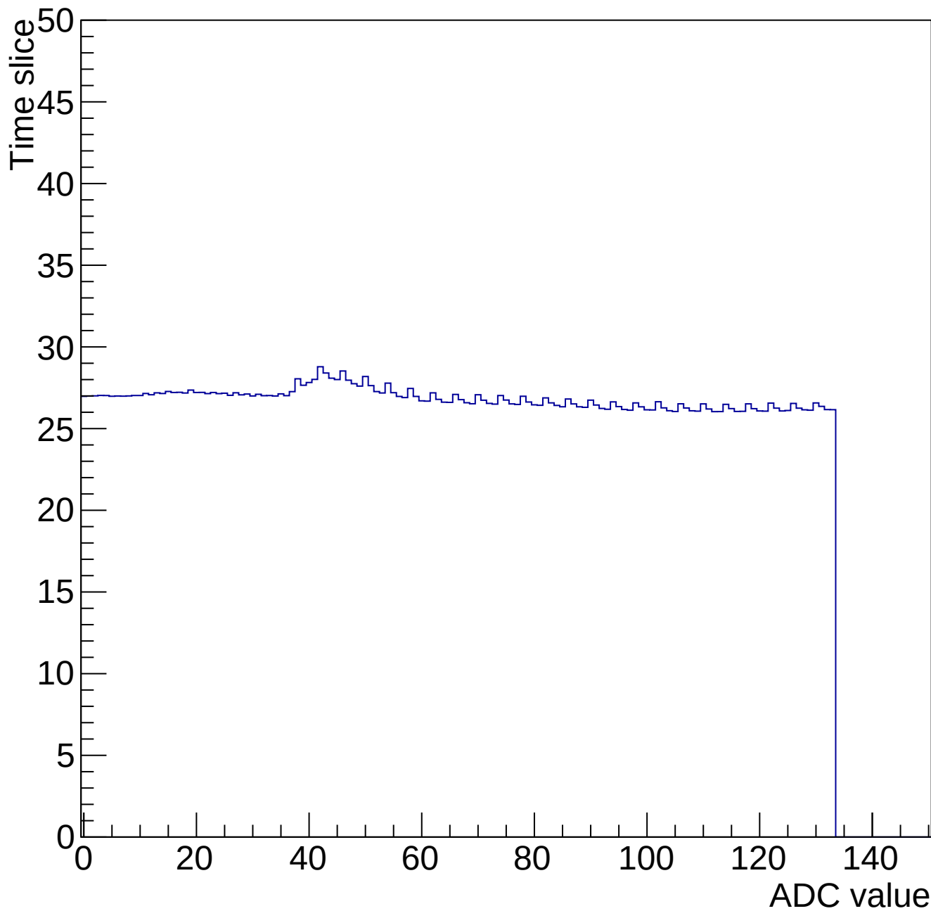
Time mcm 2000 chip 0 chan 7 34687-gain0-shaper0
