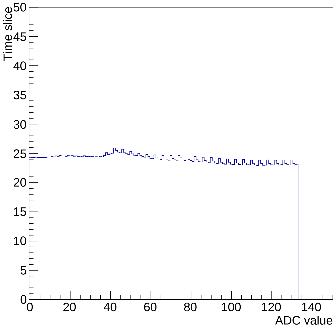
Time mcm 2000 chip 0 chan 4 34687-gain0-shaper0
