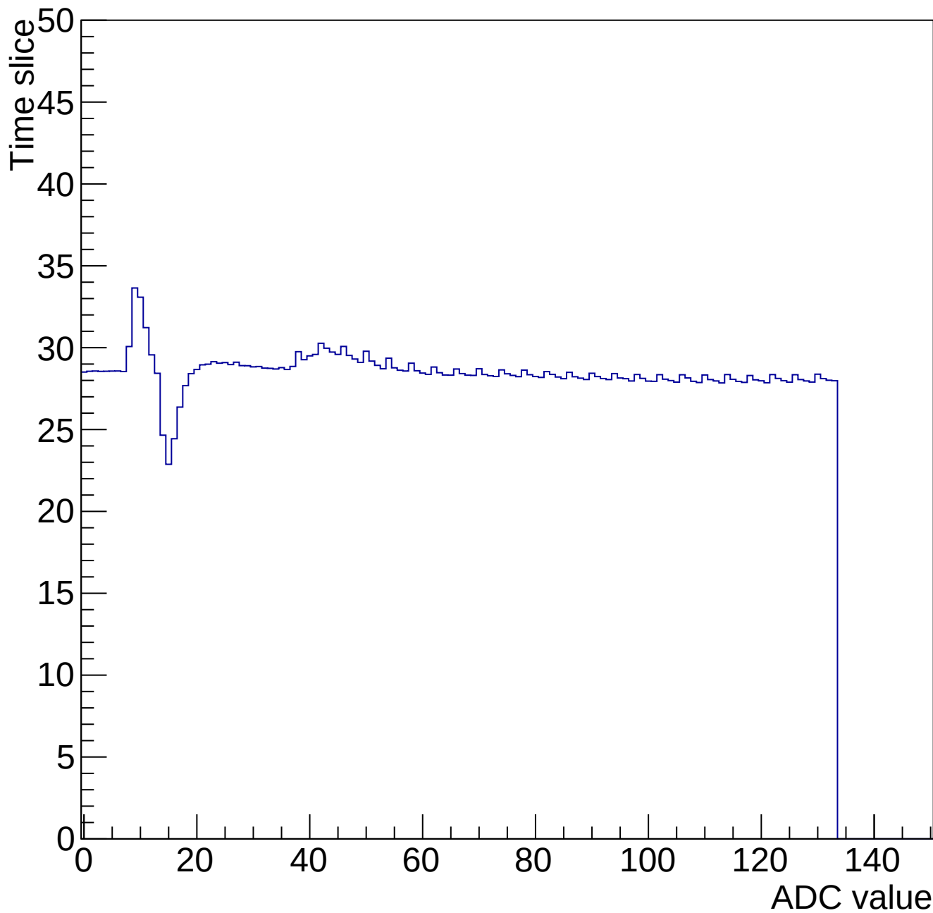
Time mcm 2000 chip 0 chan 1 34687-gain0-shaper0
