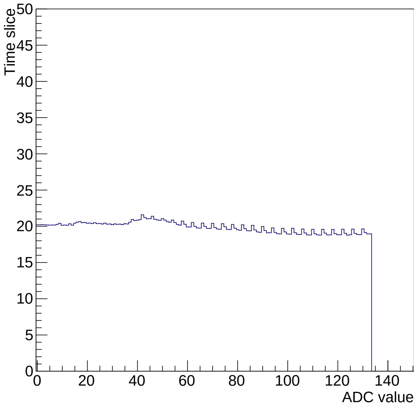
Time mcm 2000 chip 0 chan 15 34687-gain0-shaper0
