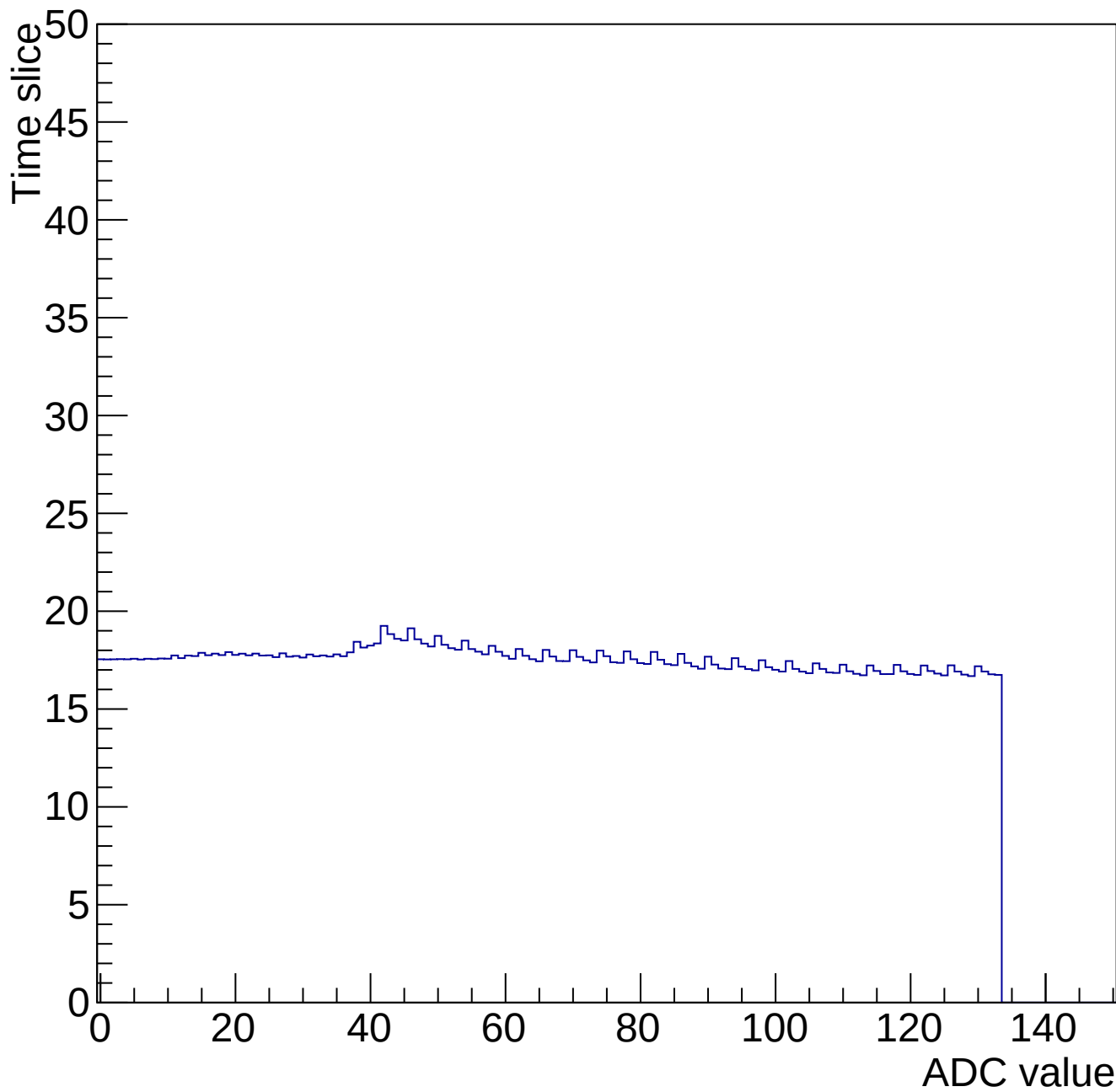
Time mcm 2000 chip 0 chan 9 34687-gain0-shaper0
