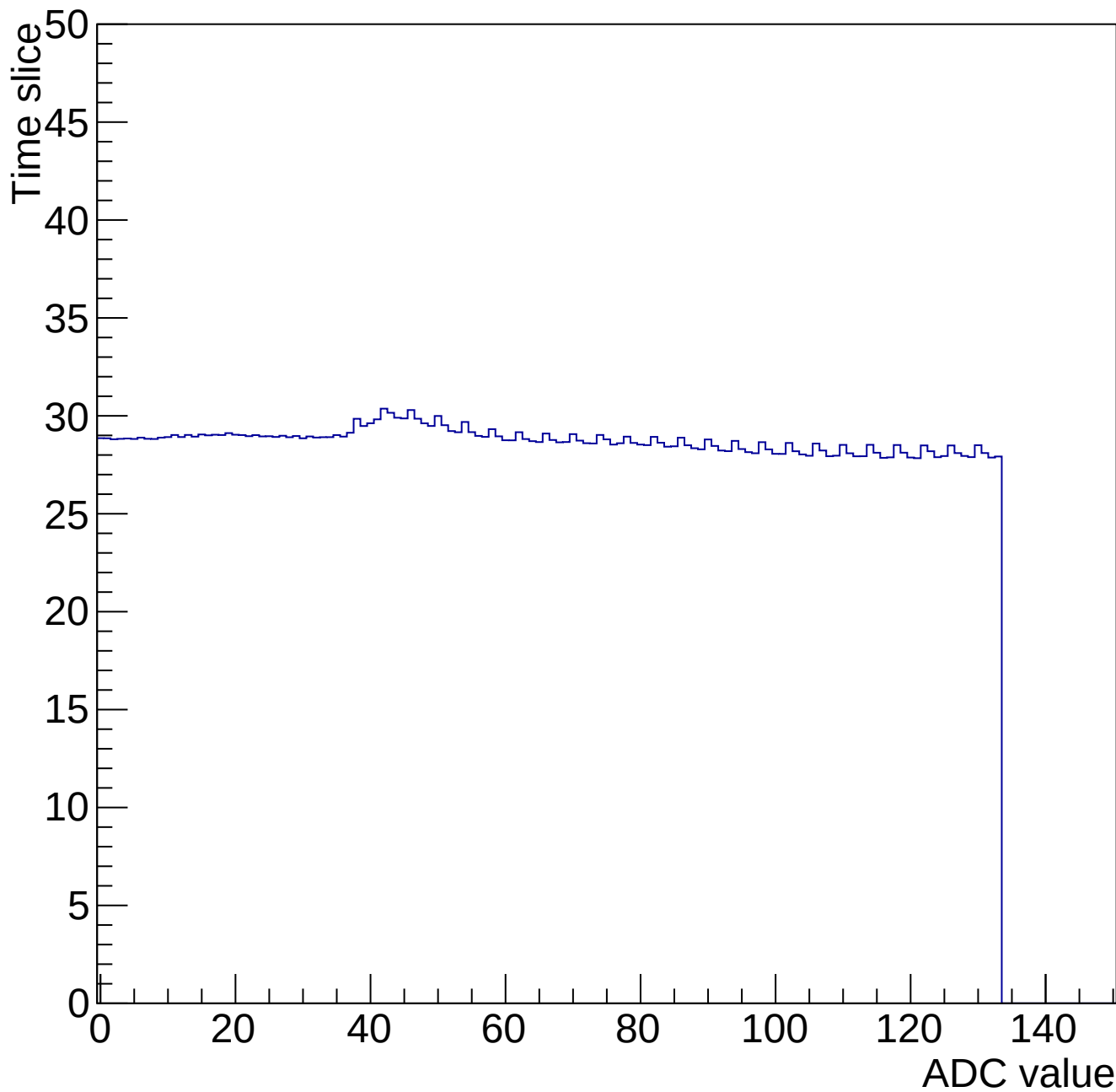
Time mcm 2000 chip 0 chan 12 34687-gain0-shaper0
