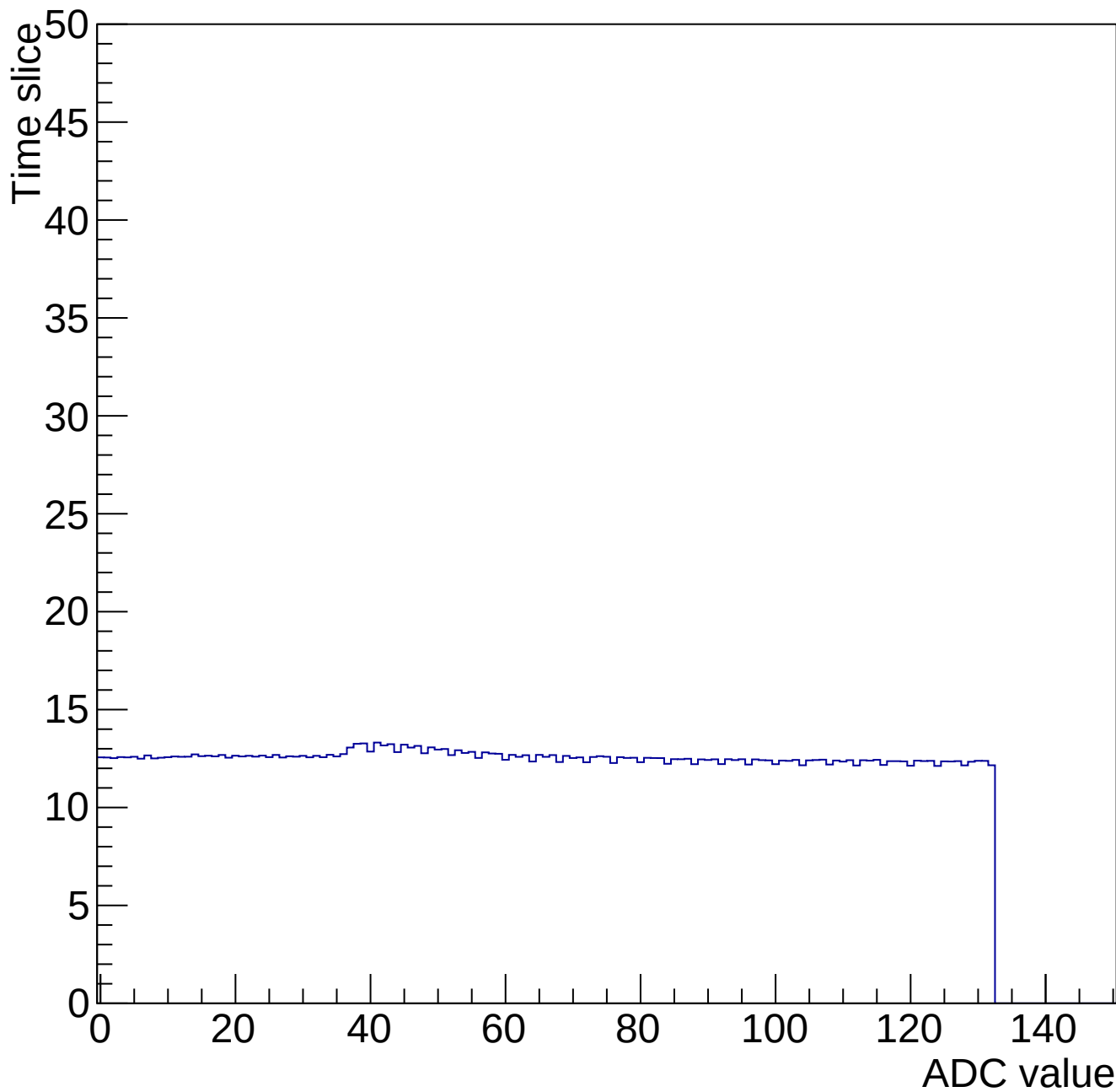
Time mcm 2001 chip 1 chan 1 34688-gain0-shaper0
