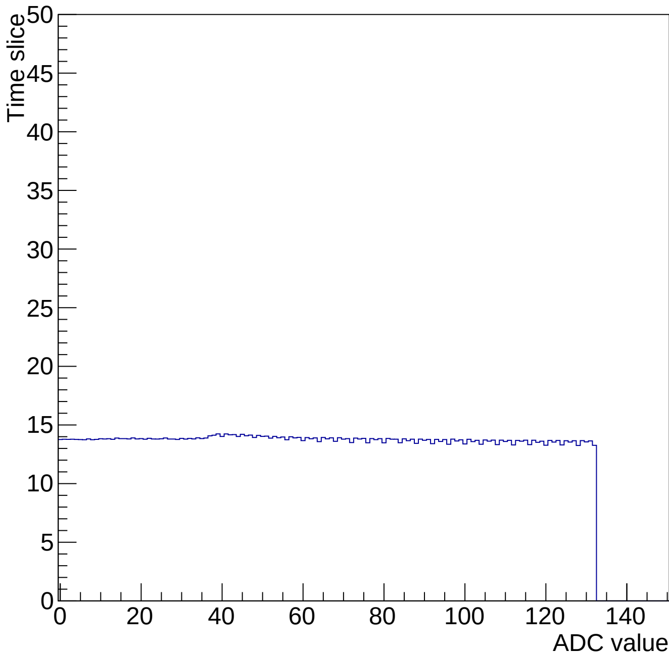
Time mcm 2001 chip 1 chan 2 34688-gain0-shaper0
