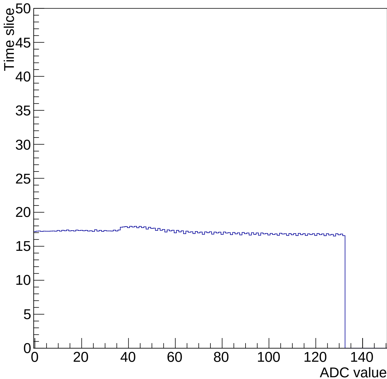
Time mcm 2001 chip 1 chan 9 34688-gain0-shaper0
