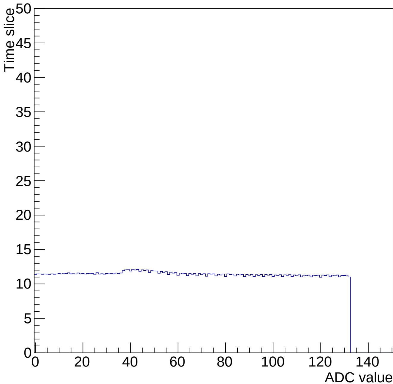
Time mcm 2001 chip 1 chan 7 34688-gain0-shaper0
