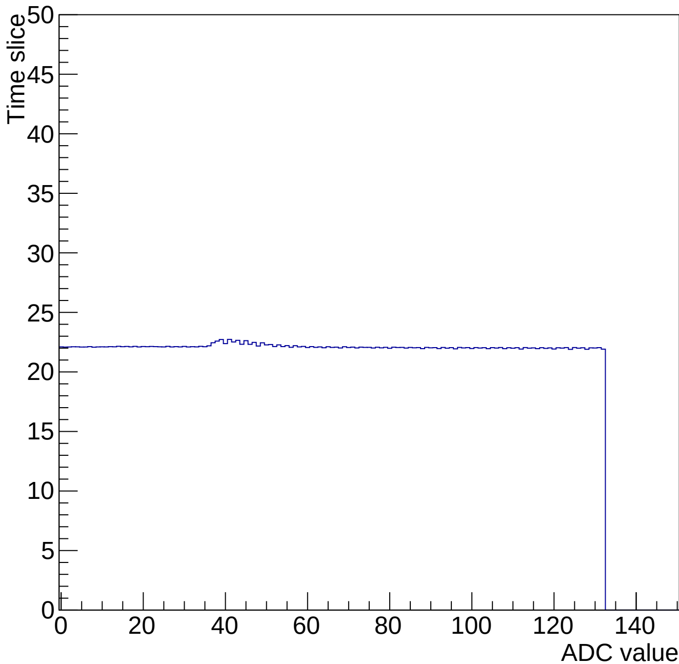
Time mcm 2001 chip 1 chan 3 34688-gain0-shaper0
