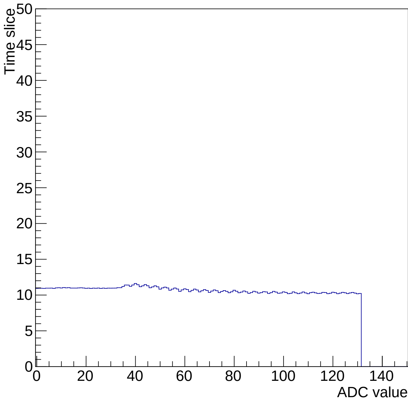
Time mcm 2002 chip 2 chan 12 34689-gain0-shaper0
