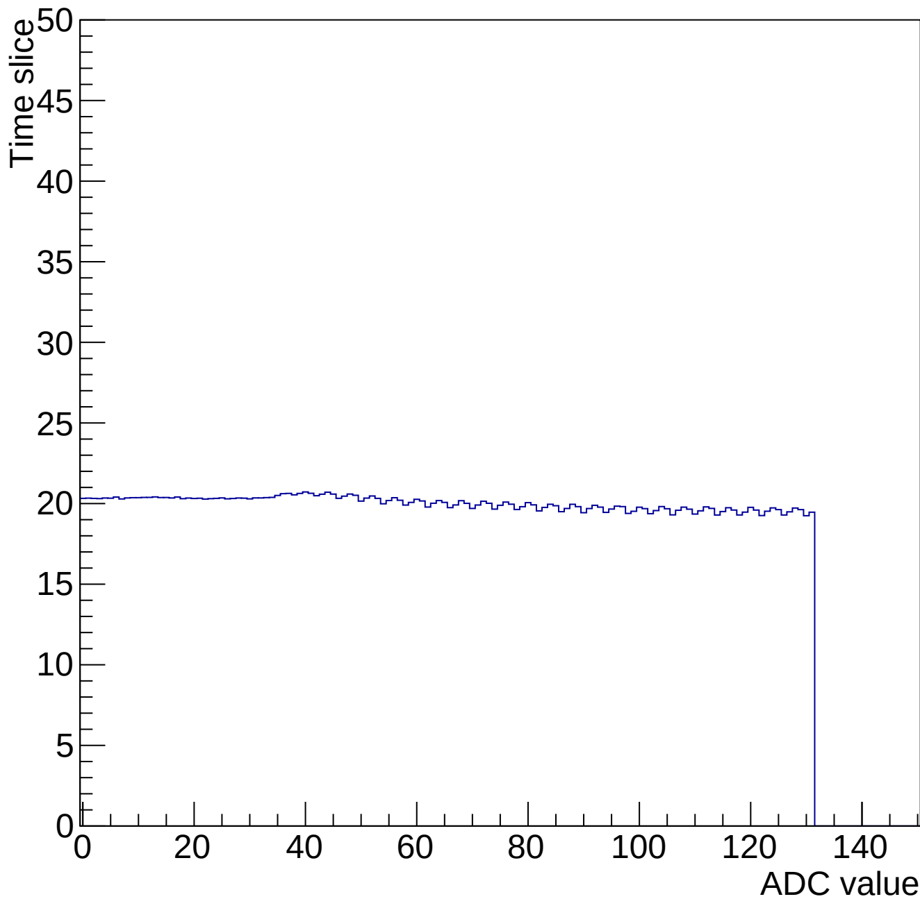
Time mcm 2002 chip 2 chan 10 34689-gain0-shaper0
