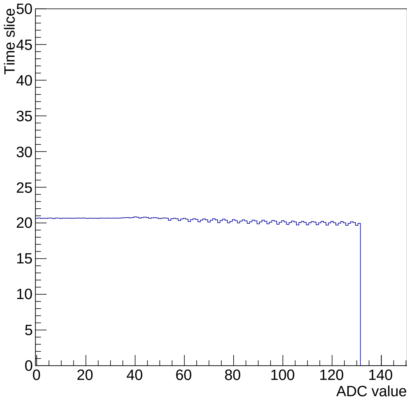
Time mcm 2002 chip 2 chan 11 34689-gain0-shaper0
