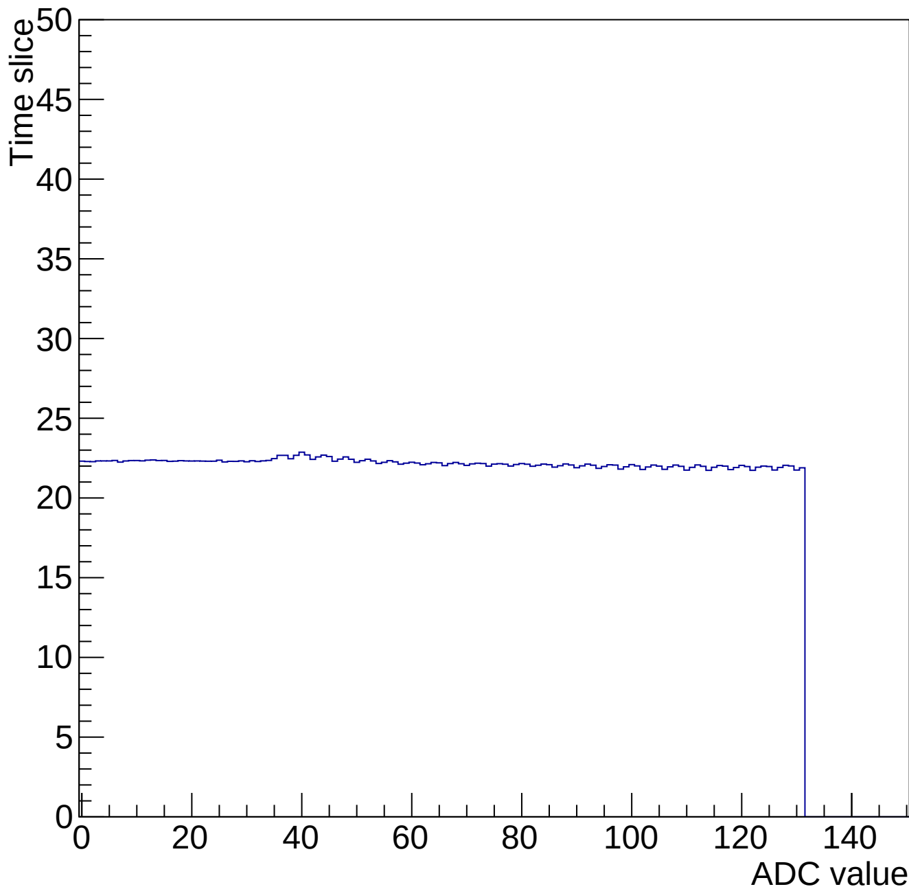
Time mcm 2002 chip 2 chan 5 34689-gain0-shaper0
