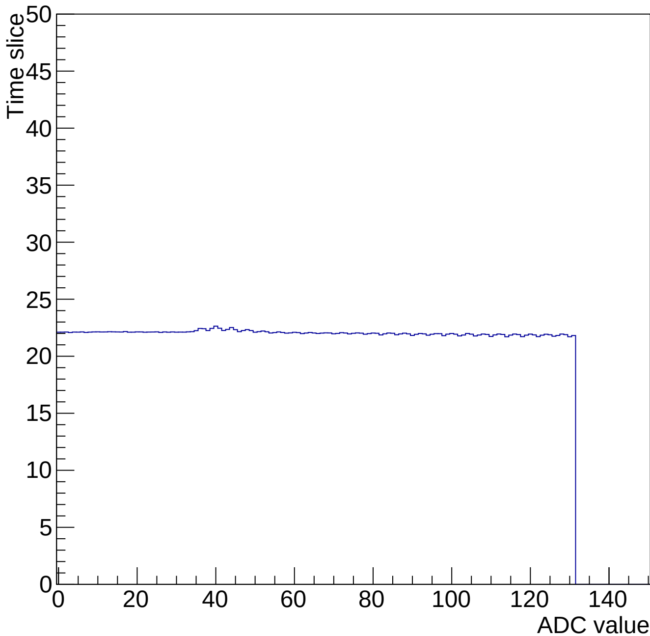
Time mcm 2002 chip 2 chan 7 34689-gain0-shaper0
