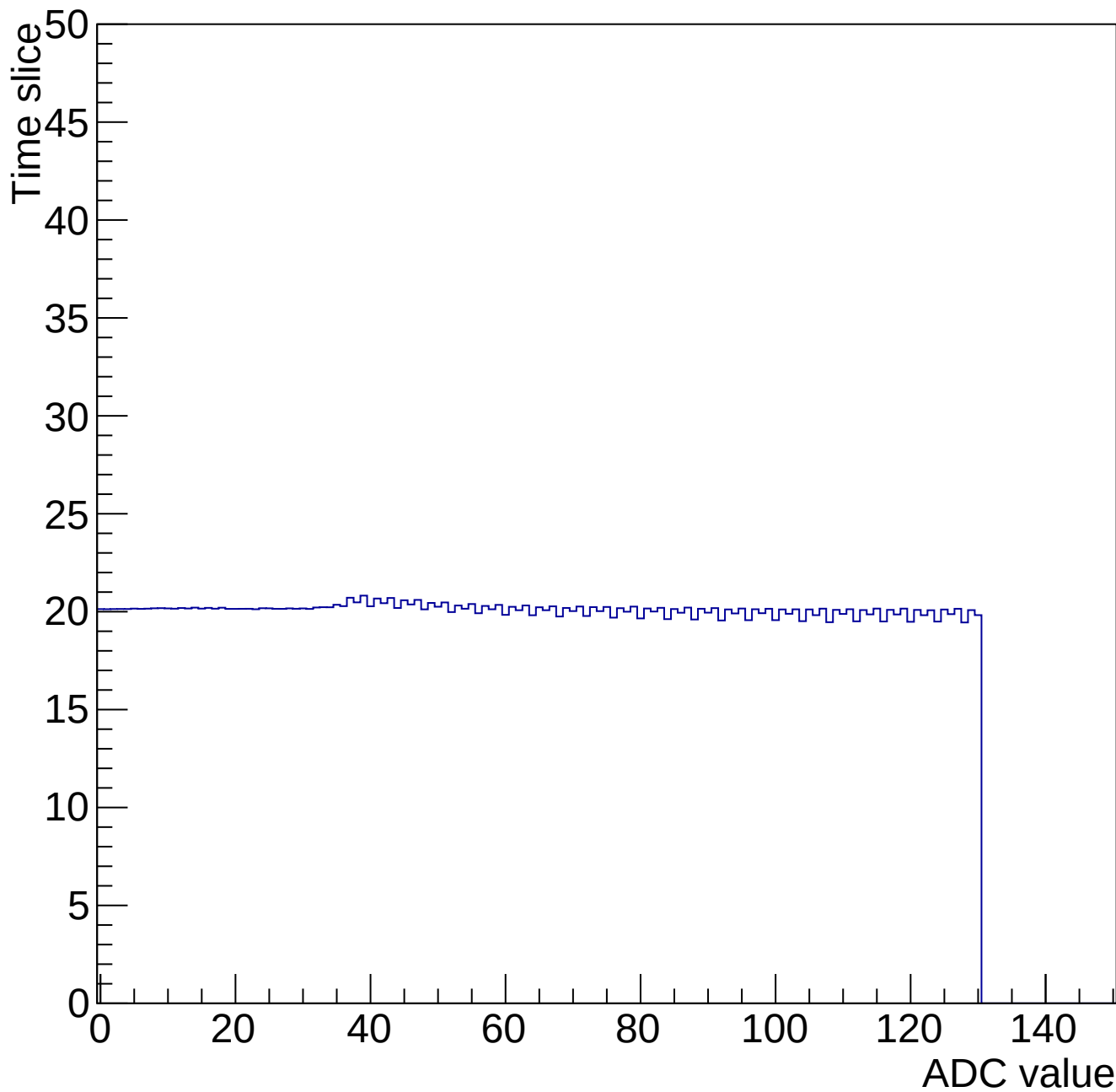
Time mcm 2003 chip 3 chan 5 34690-gain0-shaper0
