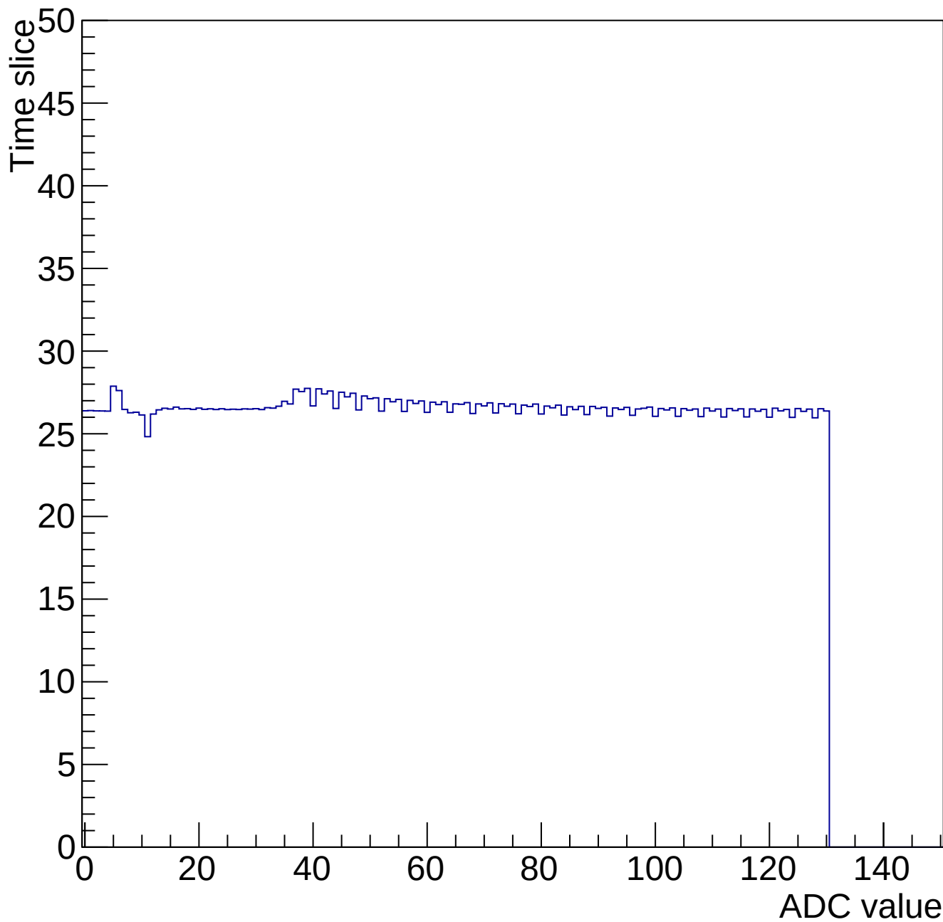
Time mcm 2003 chip 3 chan 0 34690-gain0-shaper0
