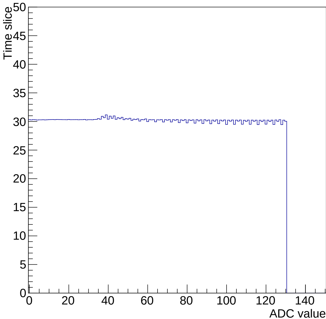
Time mcm 2003 chip 3 chan 4 34690-gain0-shaper0
