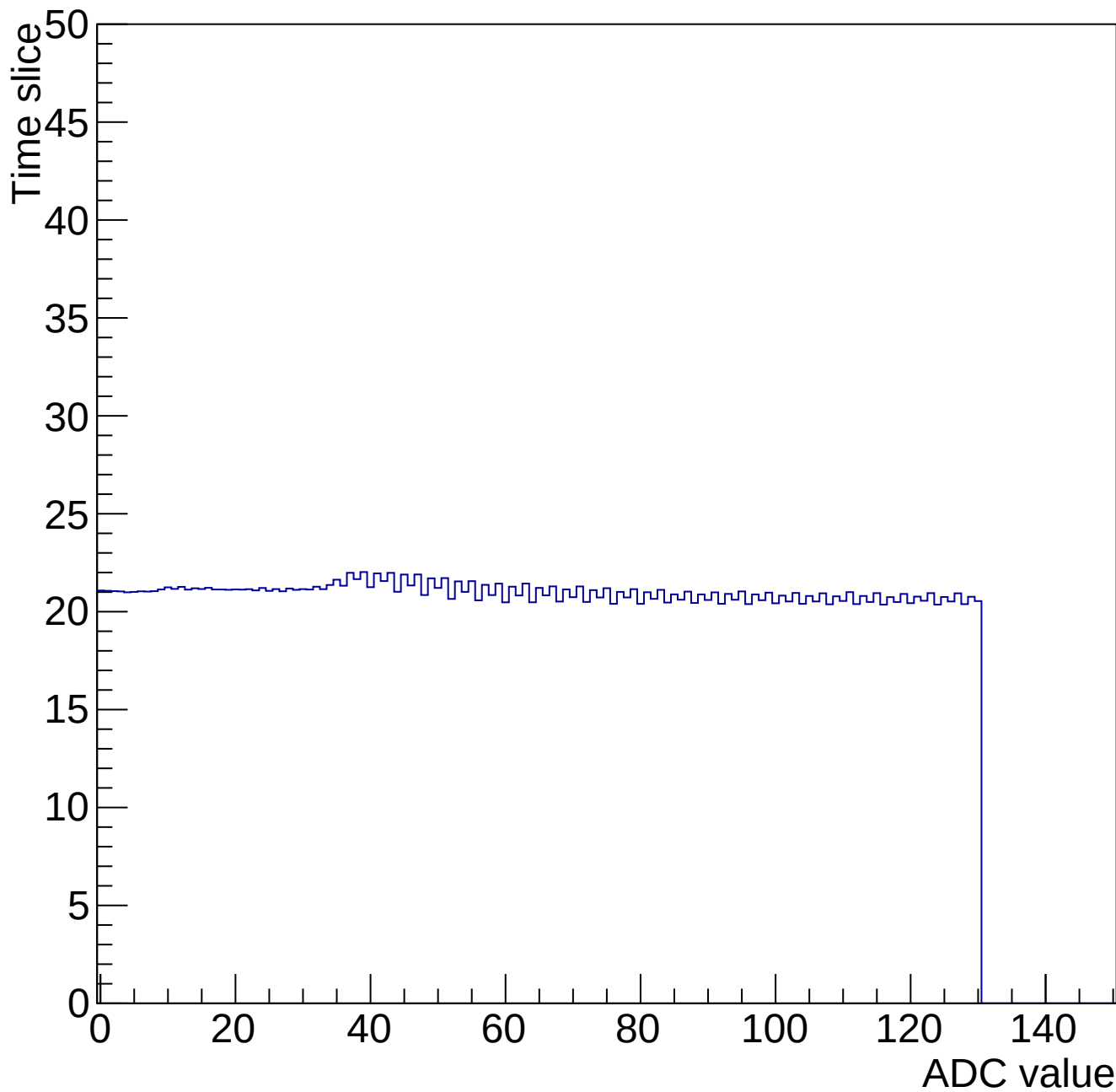
Time mcm 2003 chip 3 chan 9 34690-gain0-shaper0
