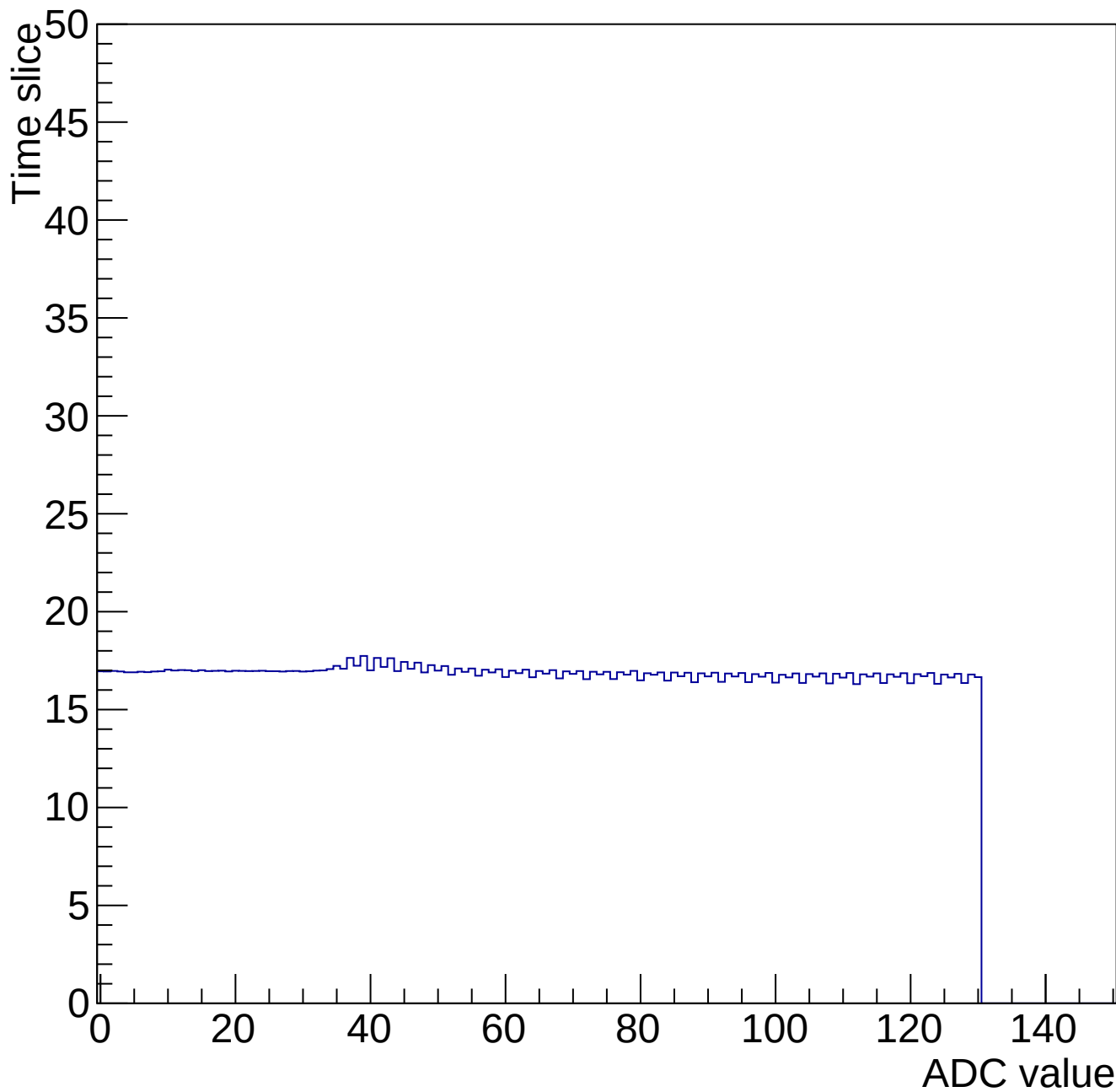
Time mcm 2003 chip 3 chan 6 34690-gain0-shaper0
