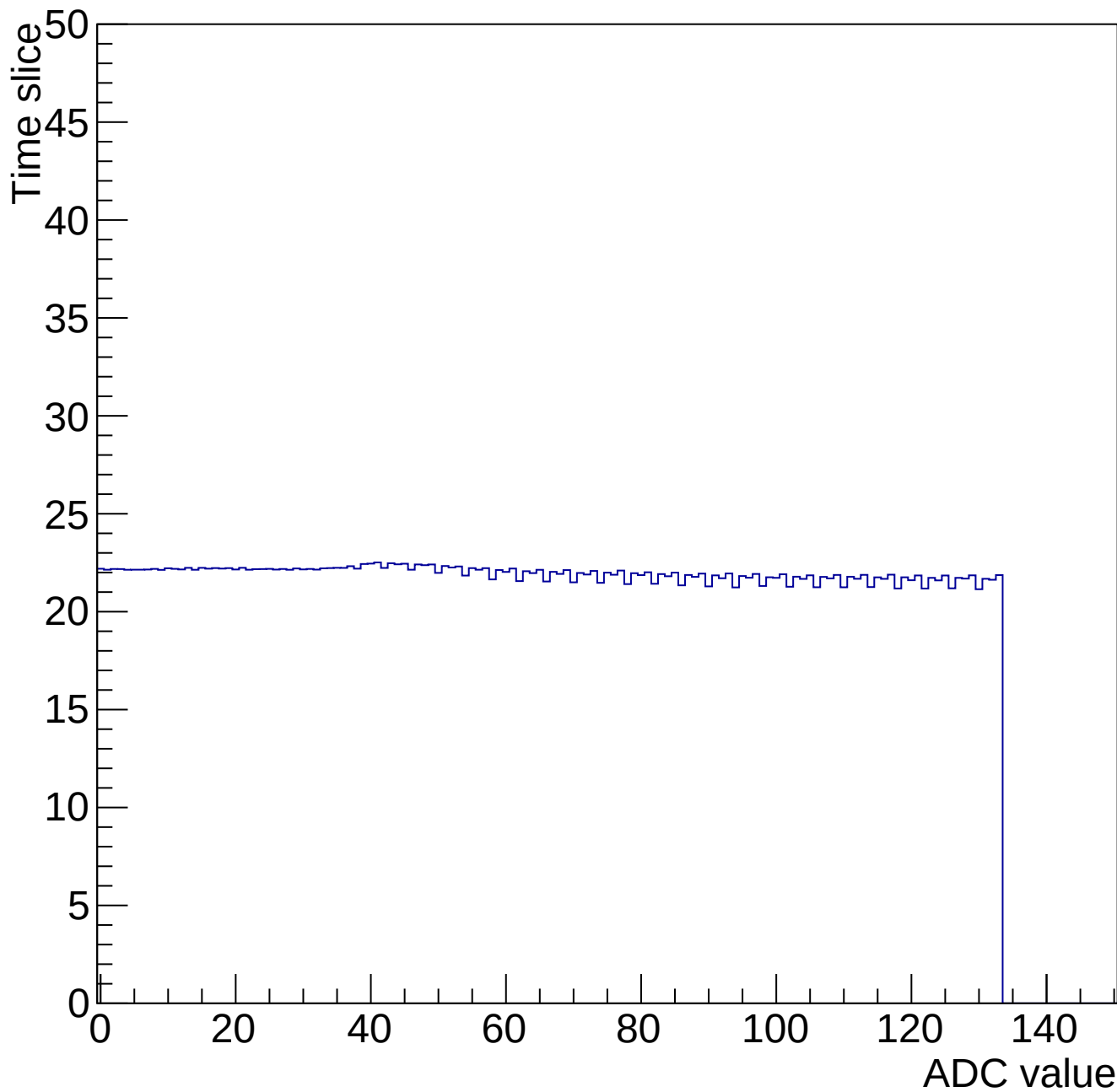
Time mcm 2004 chip 4 chan 11 34691-gain0-shaper0
