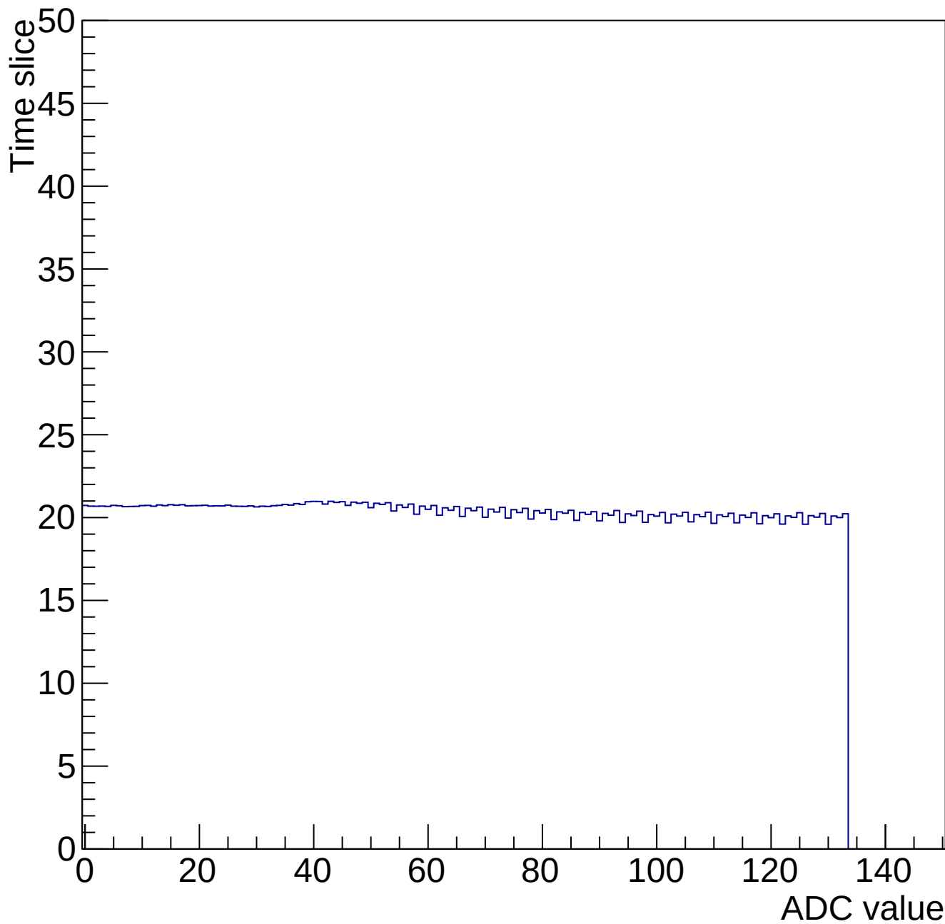
Time mcm 2004 chip 4 chan 3 34691-gain0-shaper0
