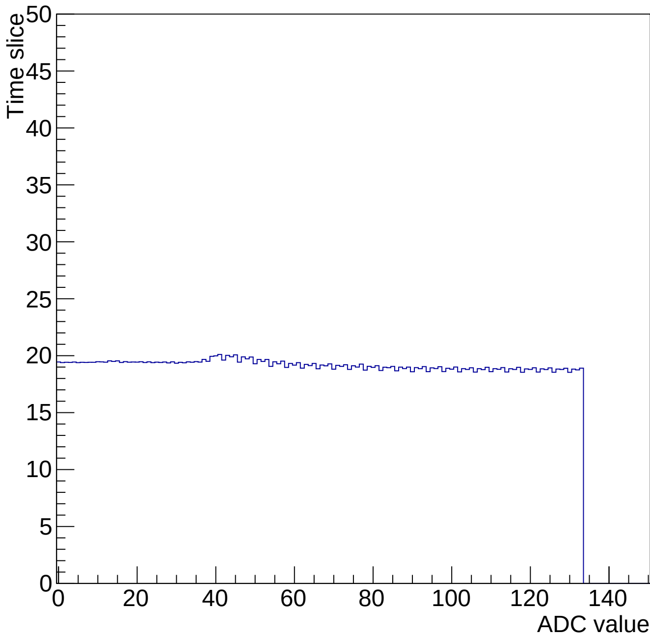
Time mcm 2004 chip 4 chan 10 34691-gain0-shaper0
