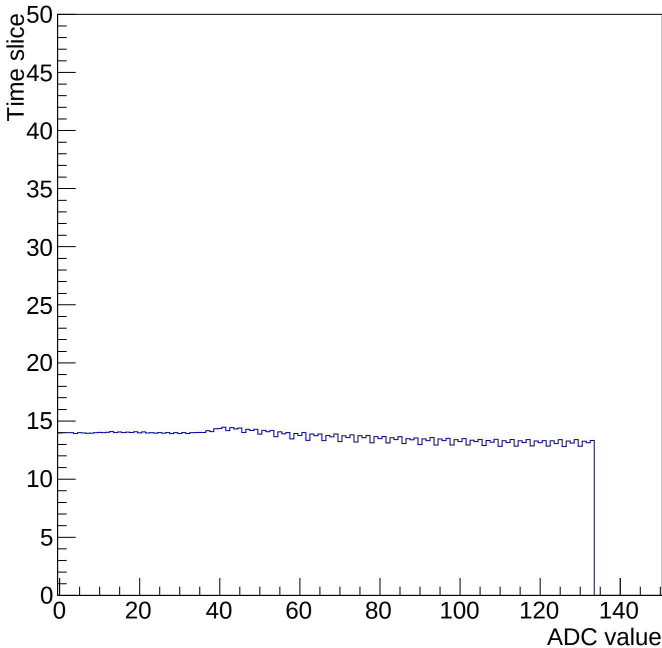
Time mcm 2004 chip 4 chan 8 34691-gain0-shaper0
