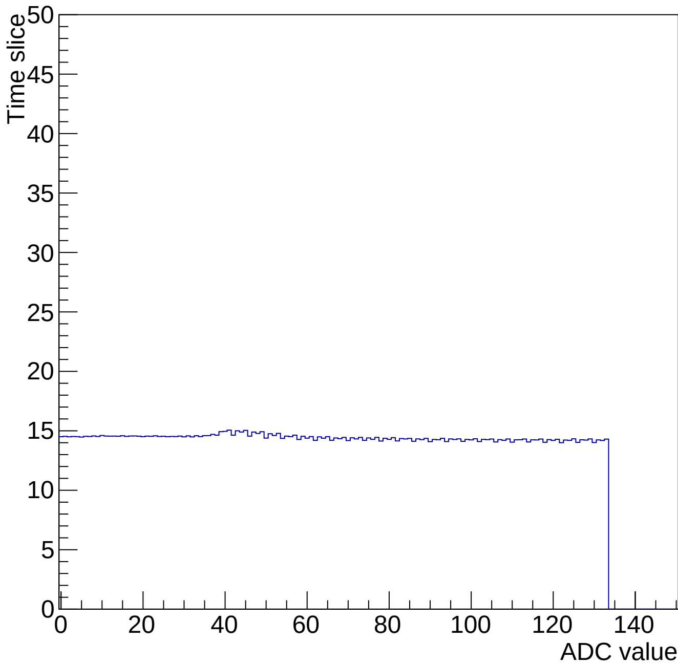
Time mcm 2004 chip 4 chan 13 34691-gain0-shaper0
