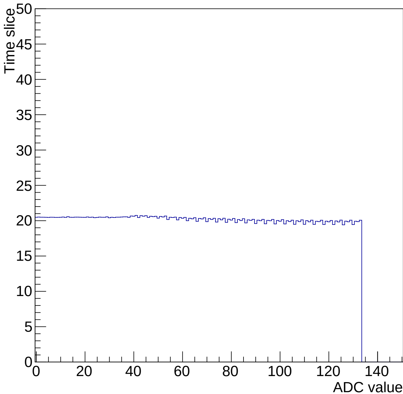
Time mcm 2004 chip 4 chan 12 34691-gain0-shaper0
