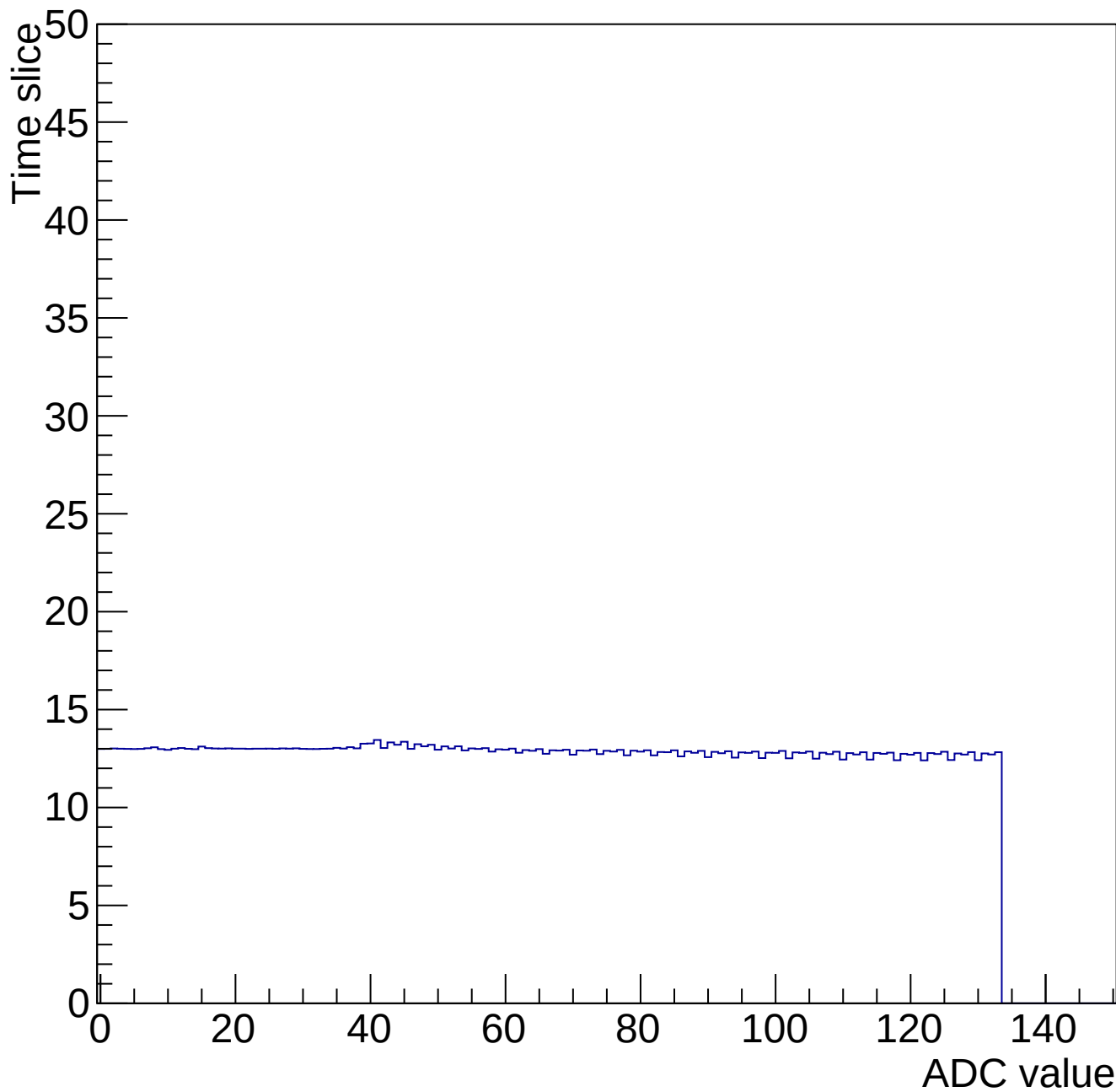
Time mcm 2004 chip 4 chan 15 34691-gain0-shaper0
