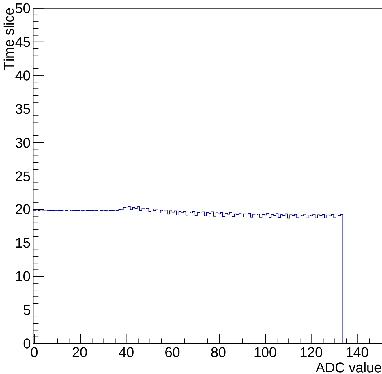
Time mcm 2004 chip 4 chan 4 34691-gain0-shaper0
