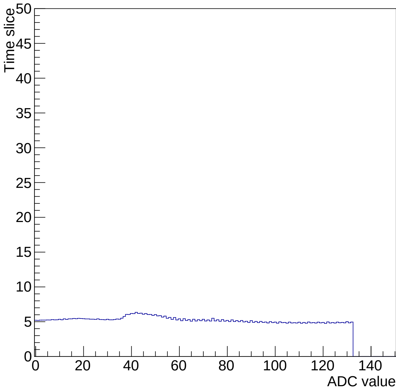
Time mcm 2005 chip 5 chan 12 34699-gain0-shaper0
