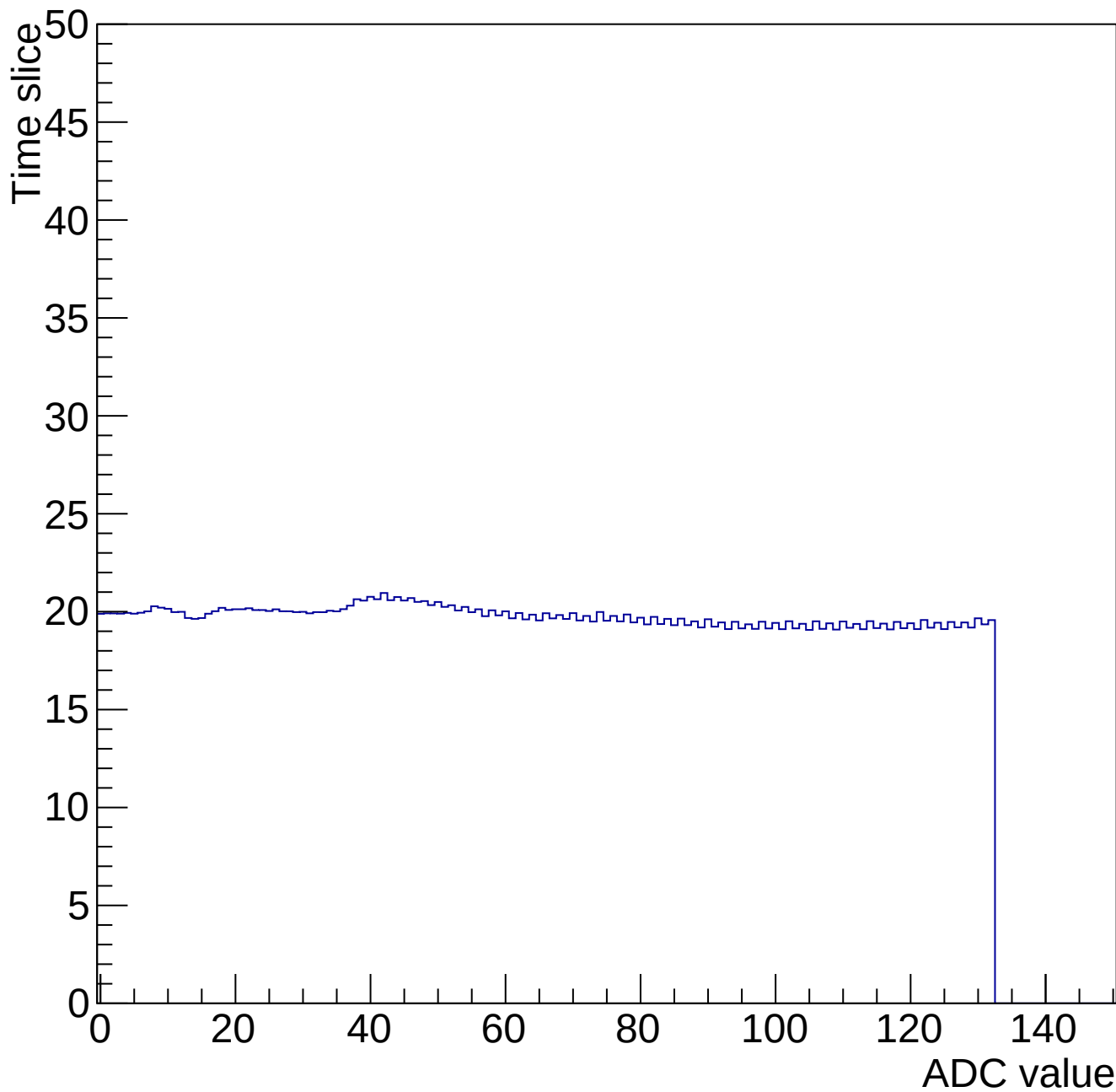
Time mcm 2005 chip 5 chan 9 34699-gain0-shaper0
