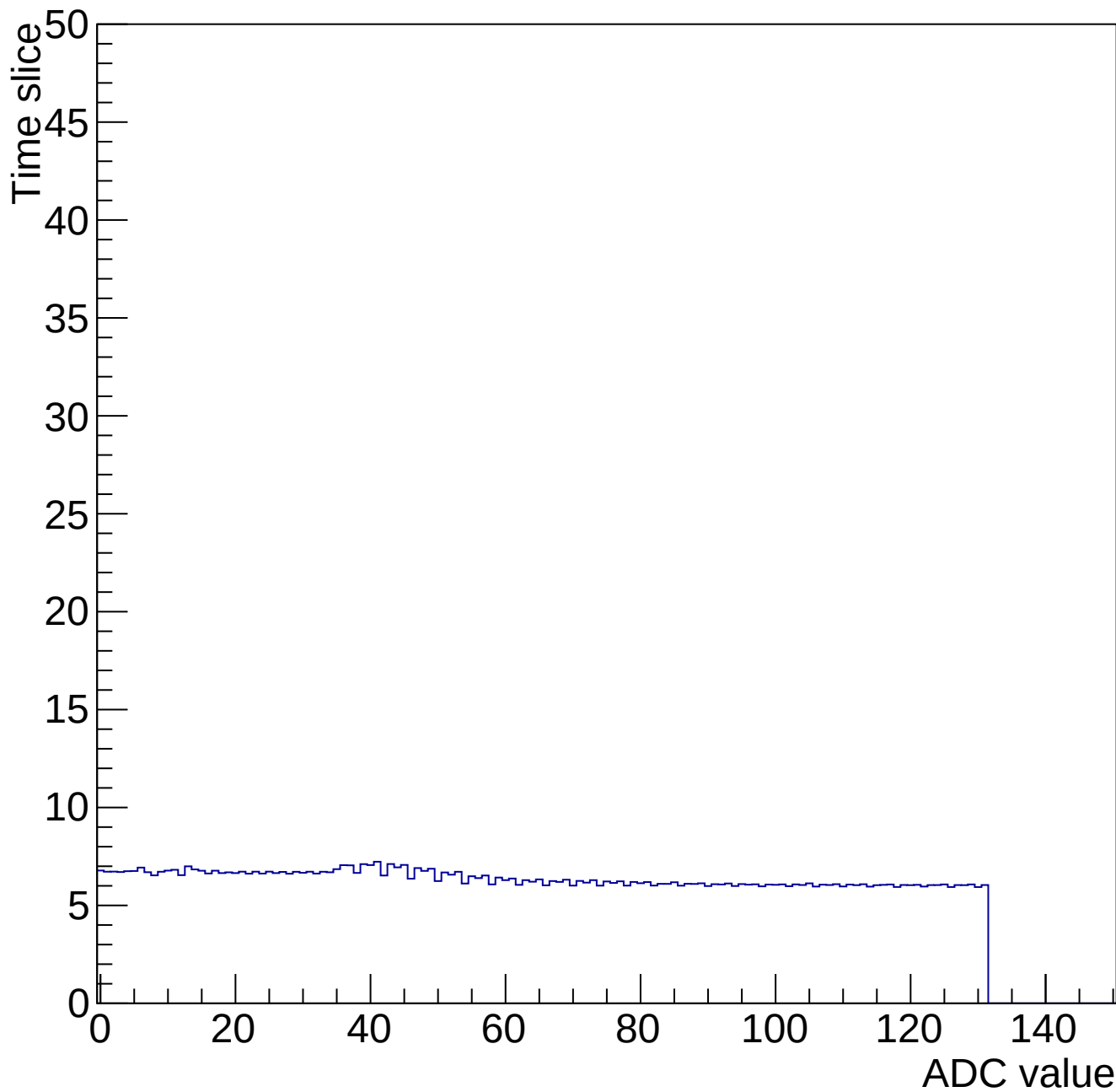
Time mcm 2006 chip 6 chan 15 34693-gain0-shaper0
