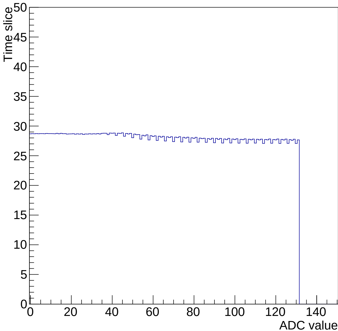
Time mcm 2006 chip 6 chan 5 34693-gain0-shaper0
