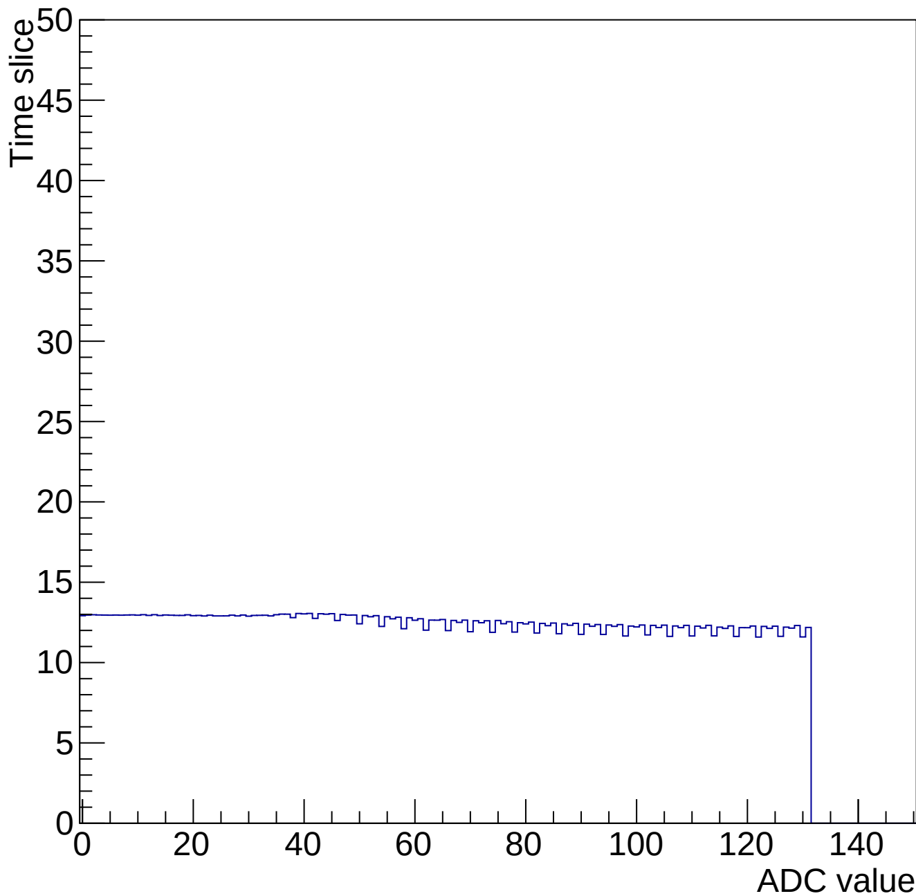
Time mcm 2006 chip 6 chan 10 34693-gain0-shaper0
