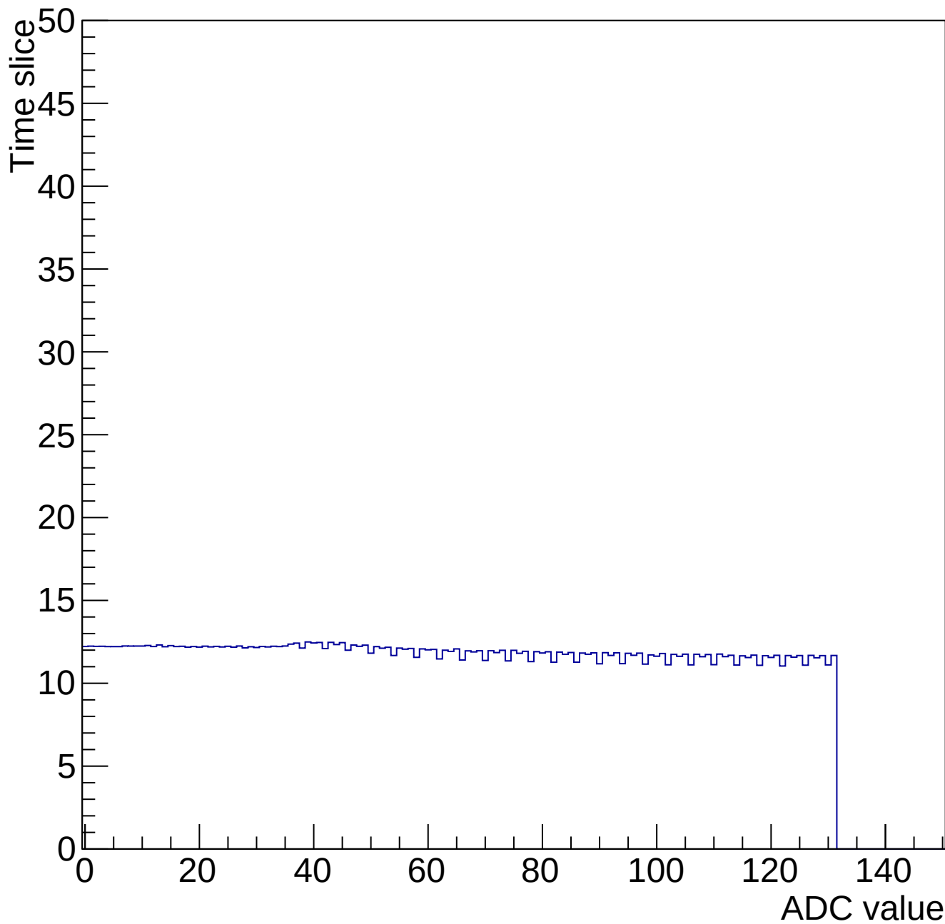
Time mcm 2006 chip 6 chan 3 34693-gain0-shaper0
