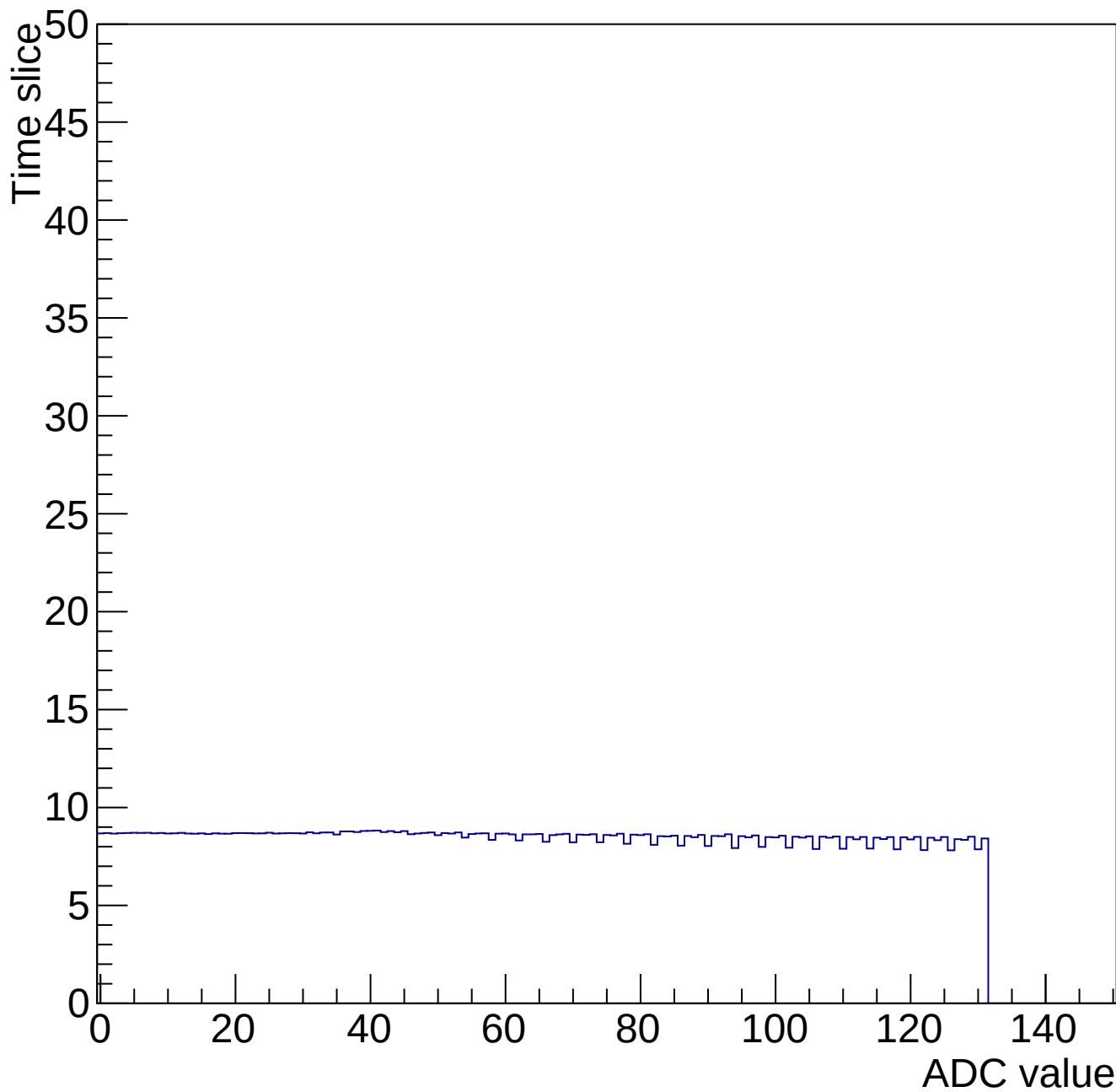
Time mcm 2006 chip 6 chan 7 34693-gain0-shaper0
