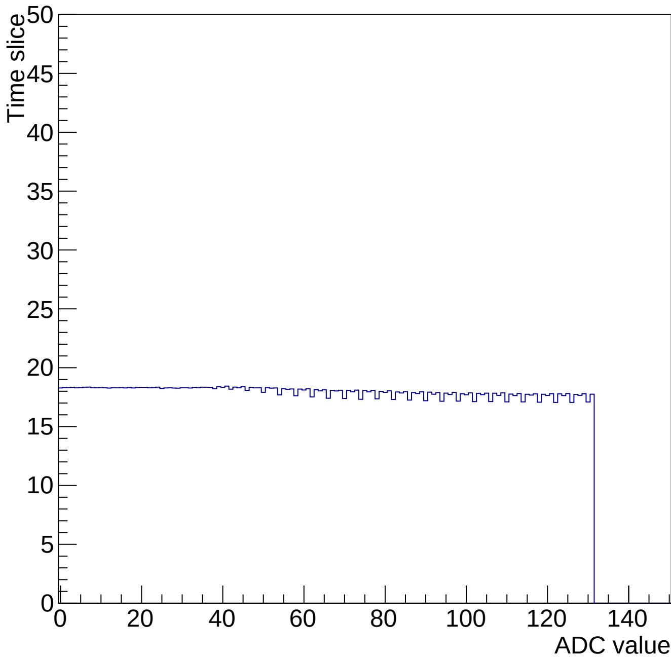
Time mcm 2006 chip 6 chan 13 34693-gain0-shaper0
