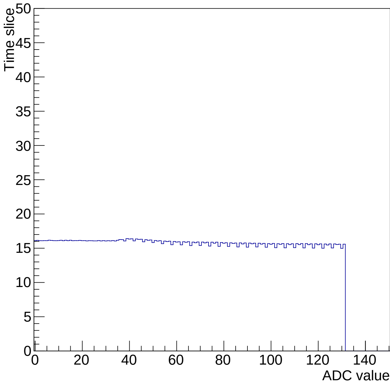
Time mcm 2006 chip 6 chan 2 34693-gain0-shaper0
