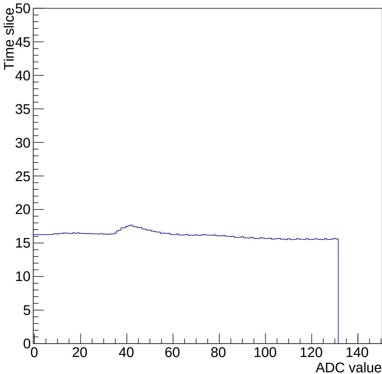
Time mcm 2006 chip 6 chan 3 34700-gain0-shaper0
