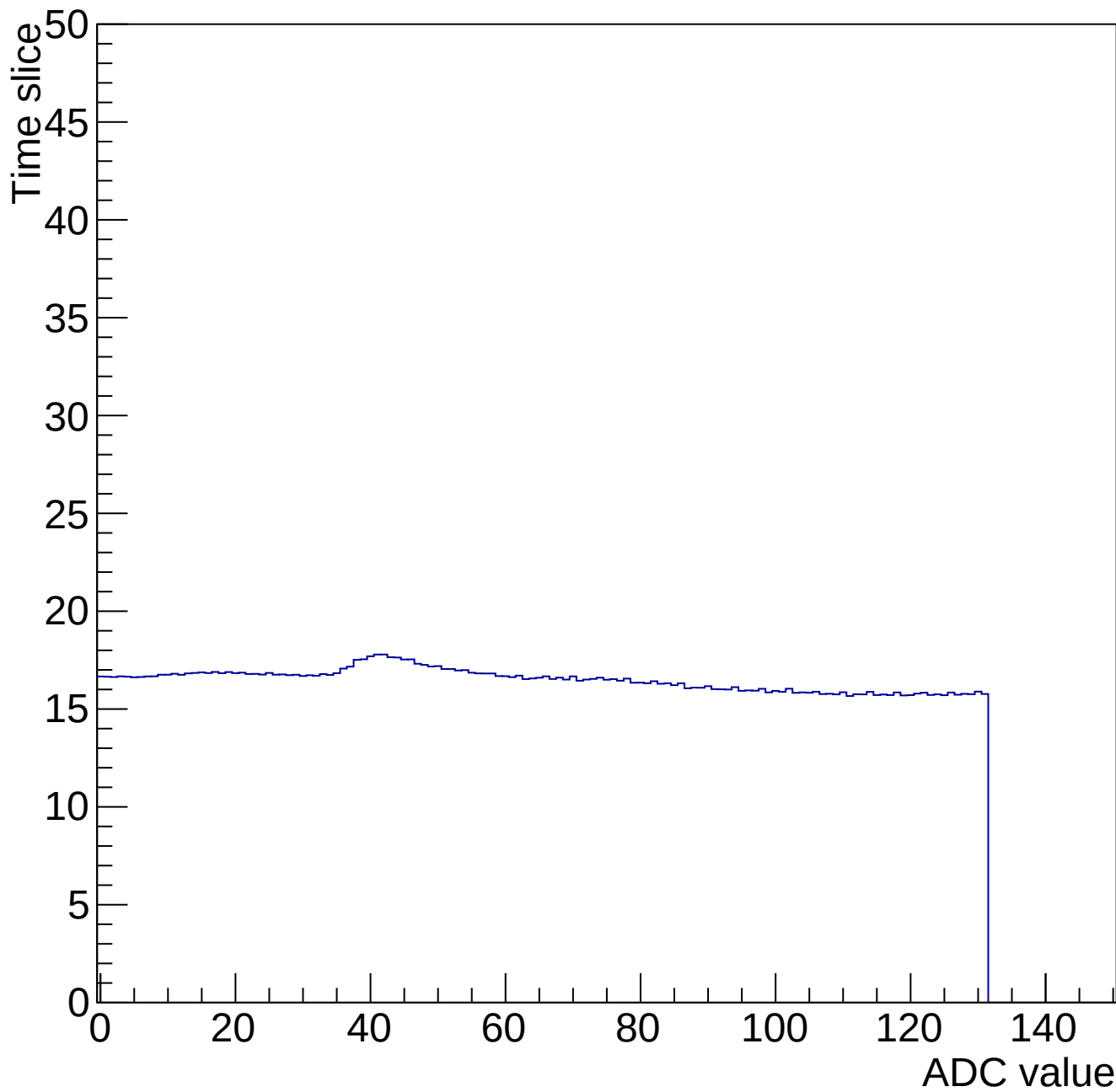
Time mcm 2006 chip 6 chan 10 34700-gain0-shaper0
