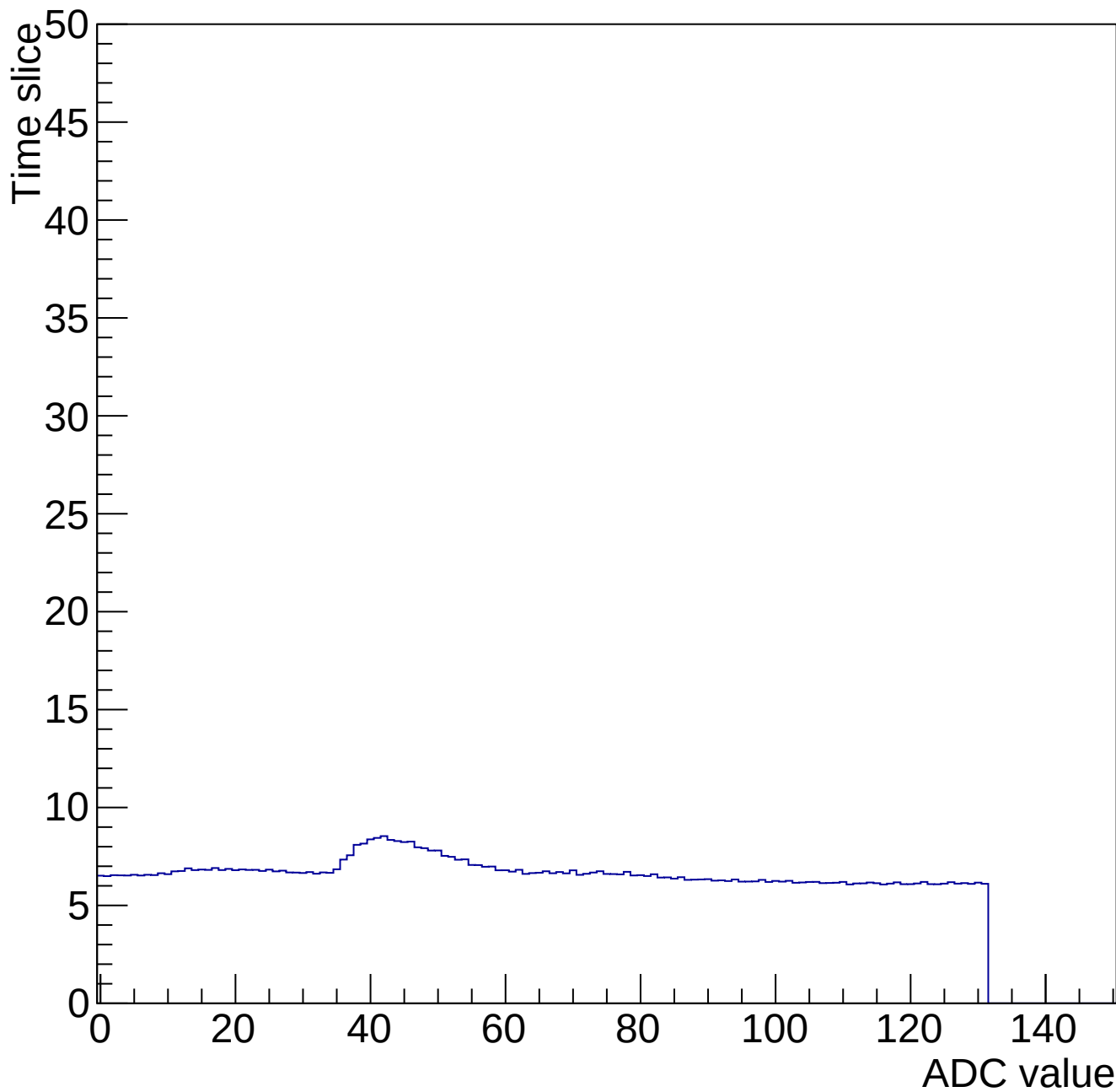
Time mcm 2006 chip 6 chan 8 34700-gain0-shaper0
