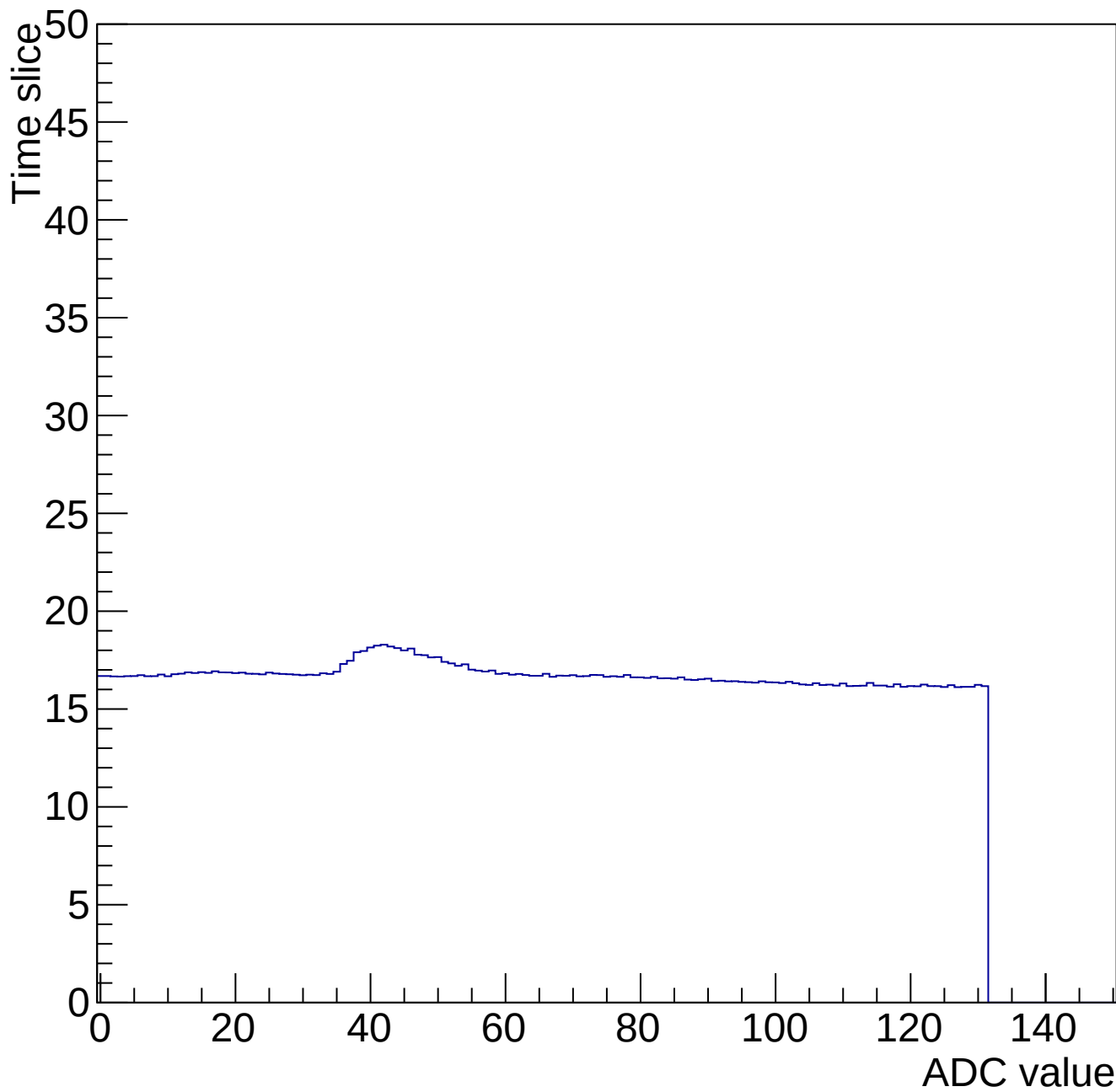
Time mcm 2006 chip 6 chan 14 34700-gain0-shaper0
