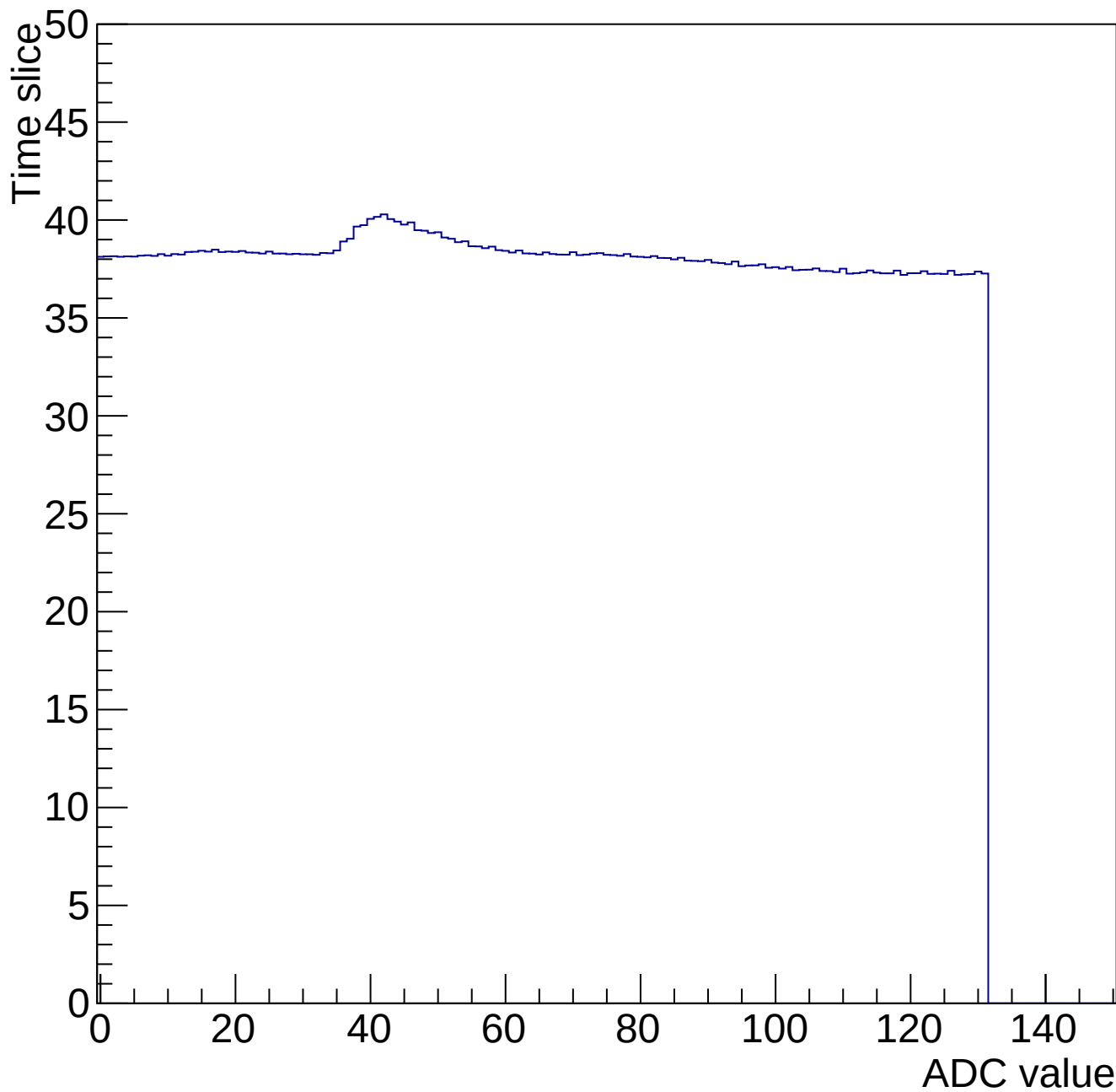
Time mcm 2006 chip 6 chan 0 34700-gain0-shaper0
