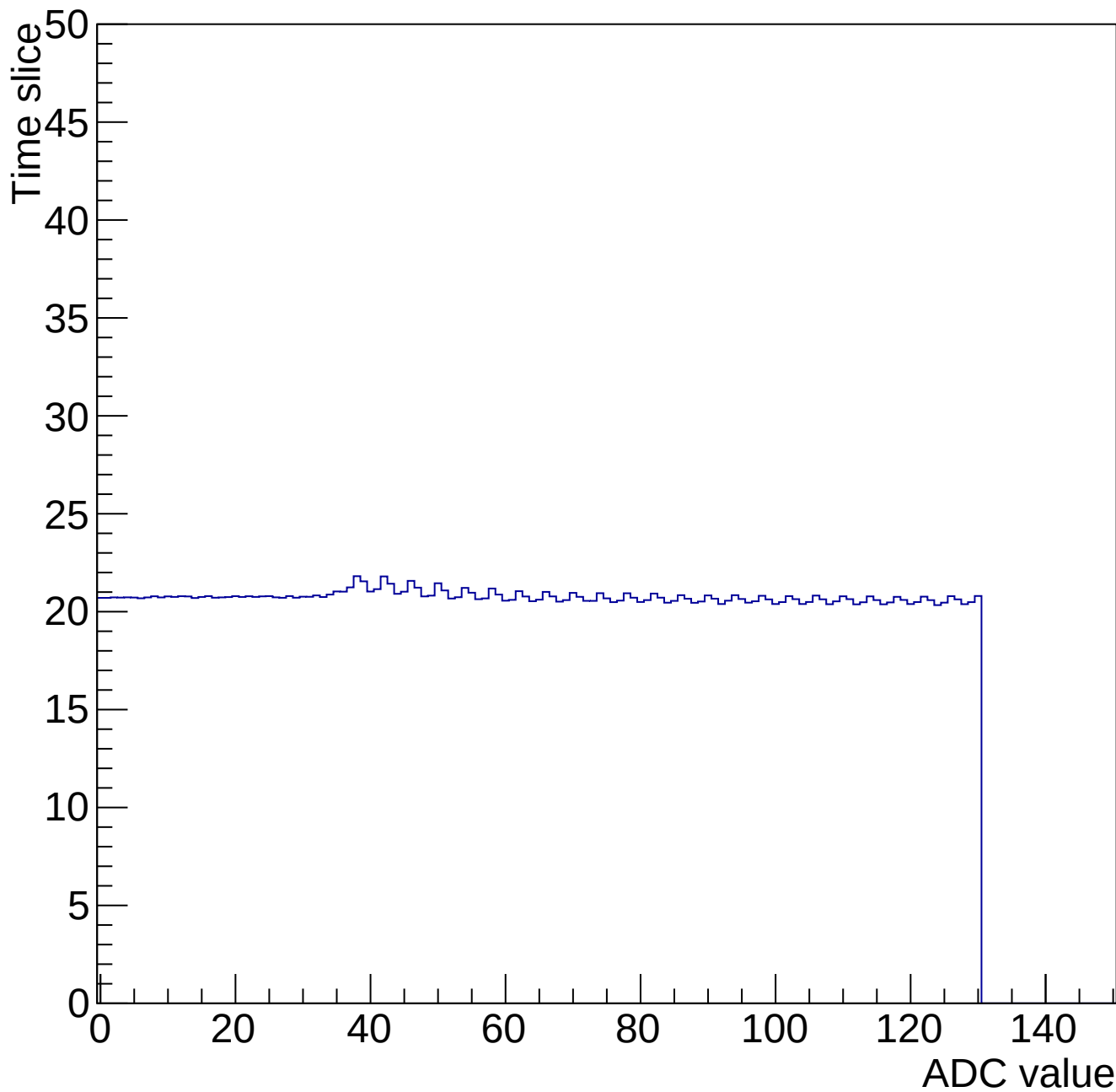
Time mcm 2007 chip 7 chan 13 34694-gain0-shaper6
