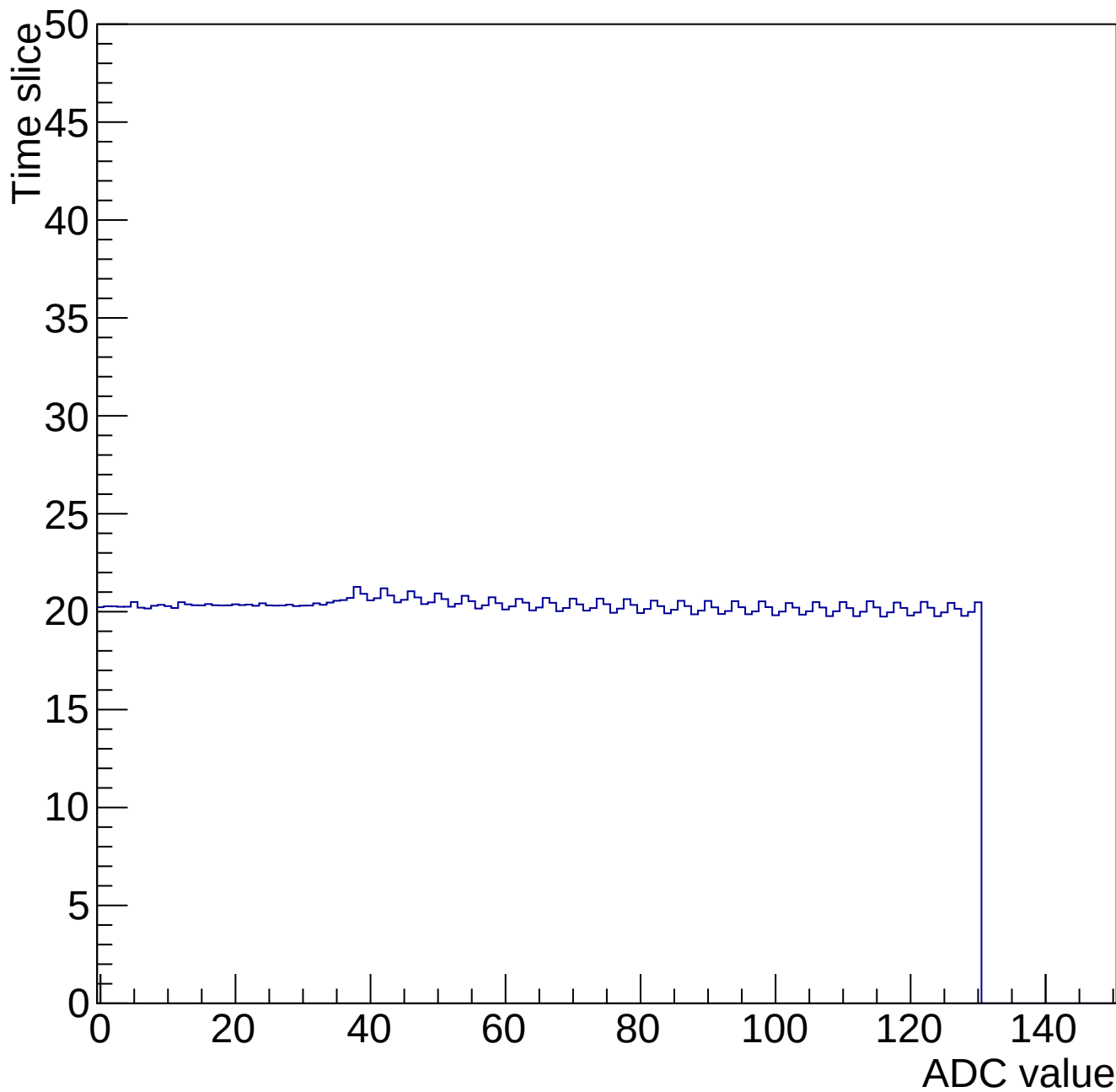
Time mcm 2007 chip 7 chan 10 34694-gain0-shaper6
