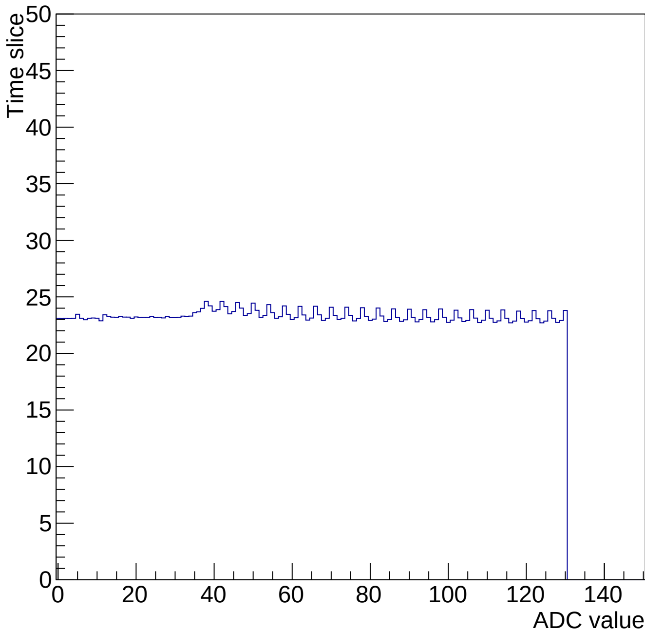
Time mcm 2007 chip 7 chan 3 34694-gain0-shaper6
