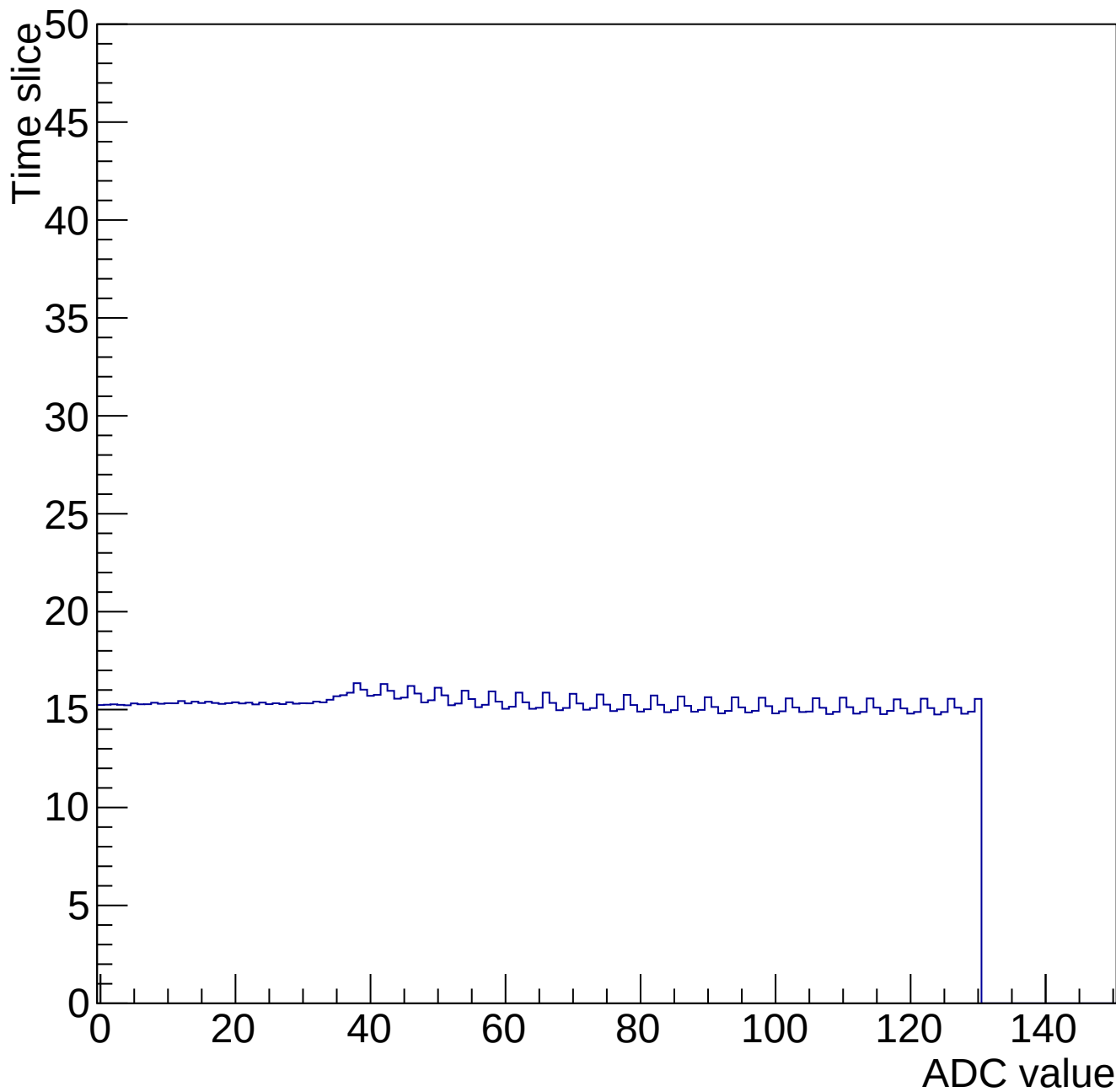
Time mcm 2007 chip 7 chan 9 34694-gain0-shaper6
