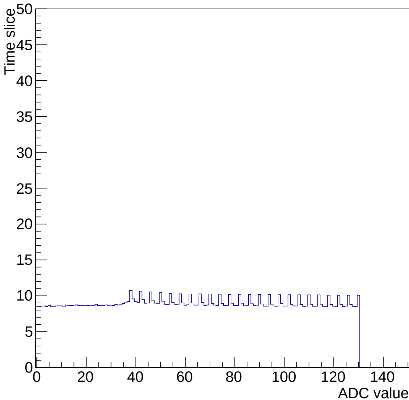
Time mcm 2007 chip 7 chan 0 34694-gain0-shaper6
