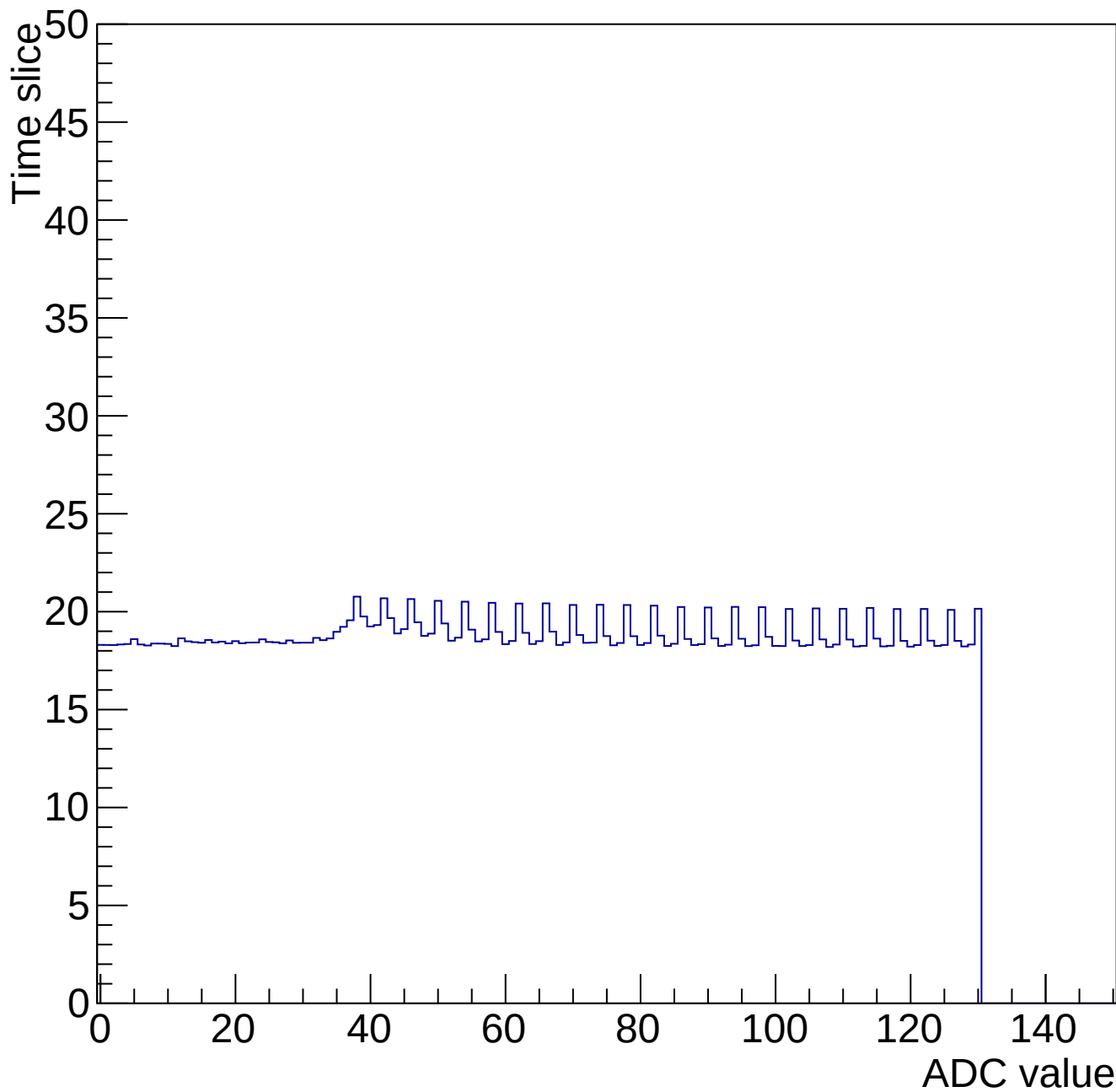
Time mcm 2007 chip 7 chan 8 34694-gain0-shaper6
