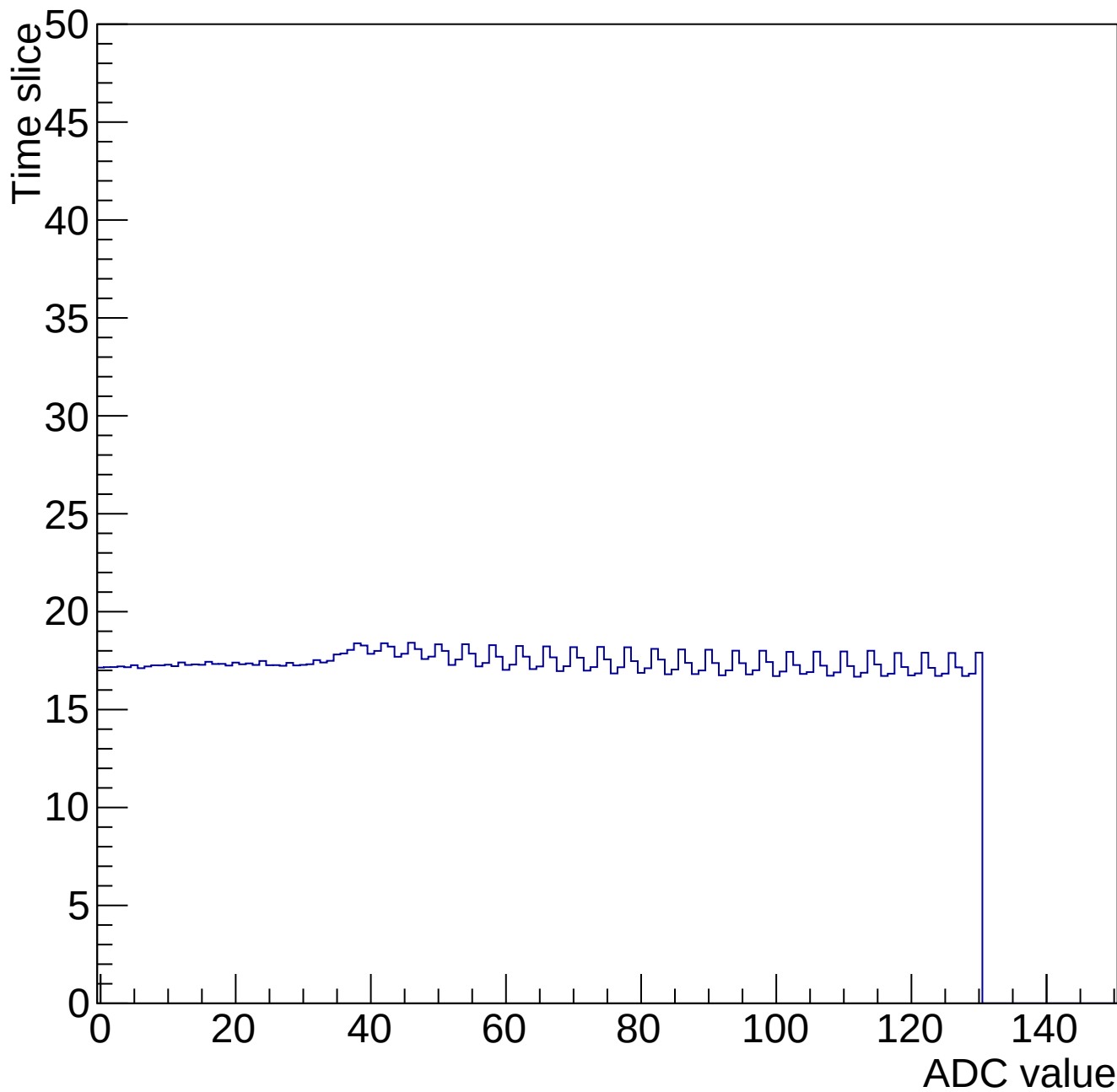
Time mcm 2007 chip 7 chan 4 34694-gain0-shaper6
