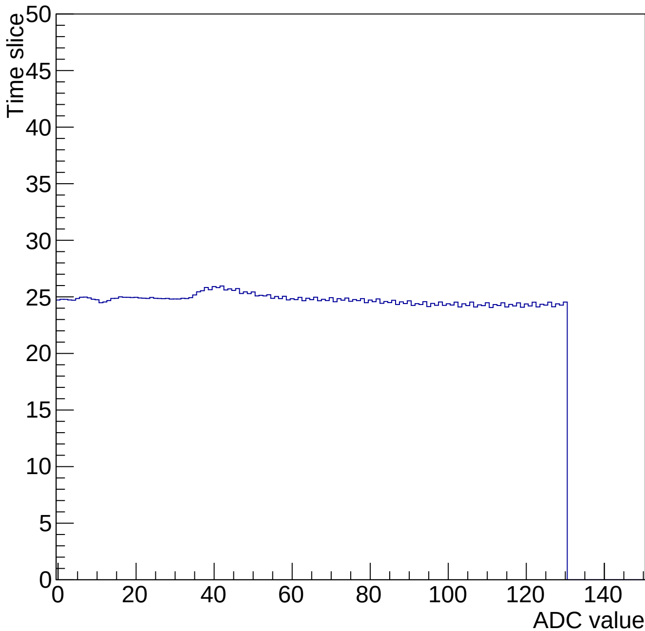
Time mcm 2007 chip 7 chan 1 34701-gain0-shaper0
