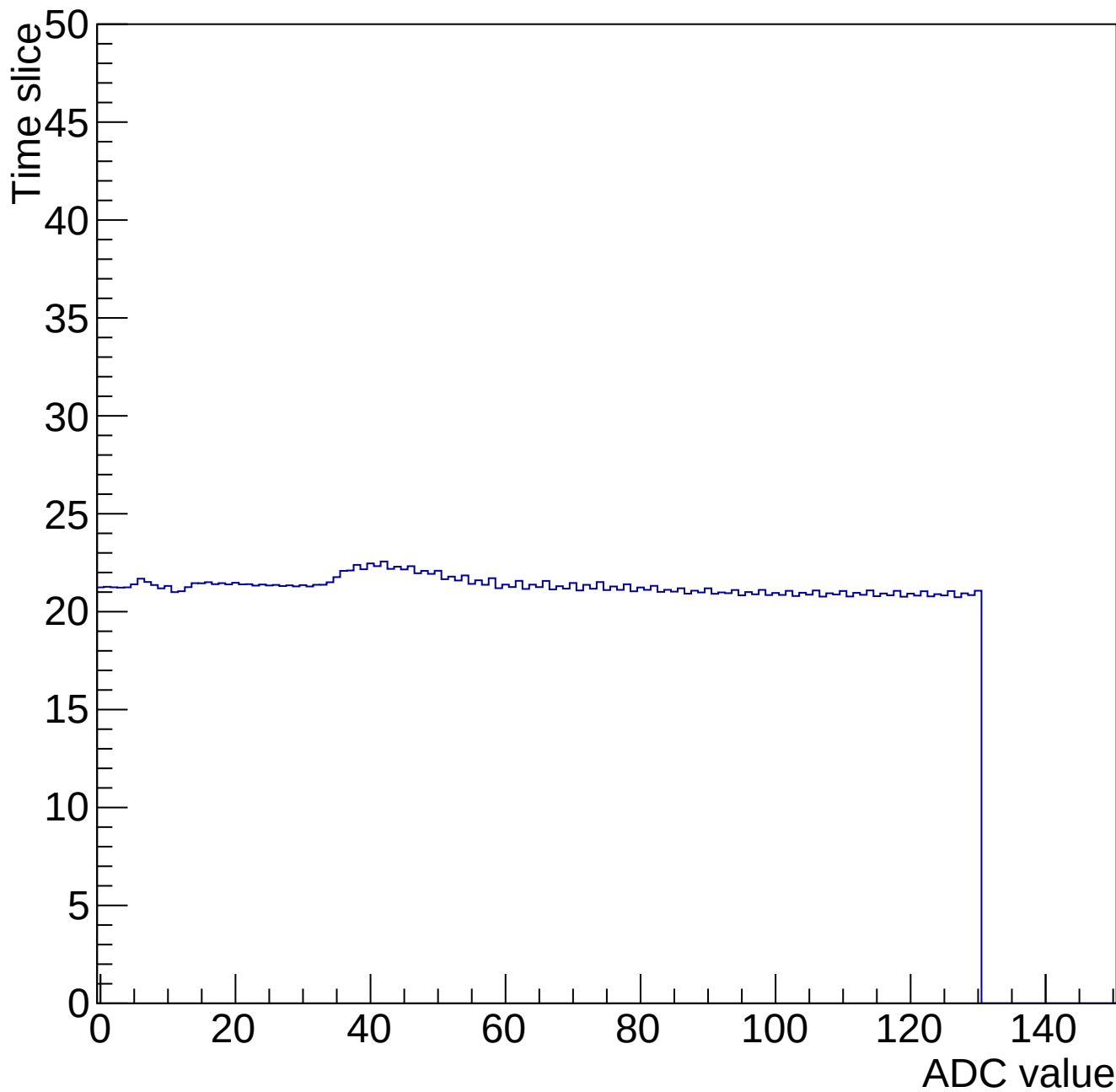
Time mcm 2007 chip 7 chan 7 34701-gain0-shaper0
