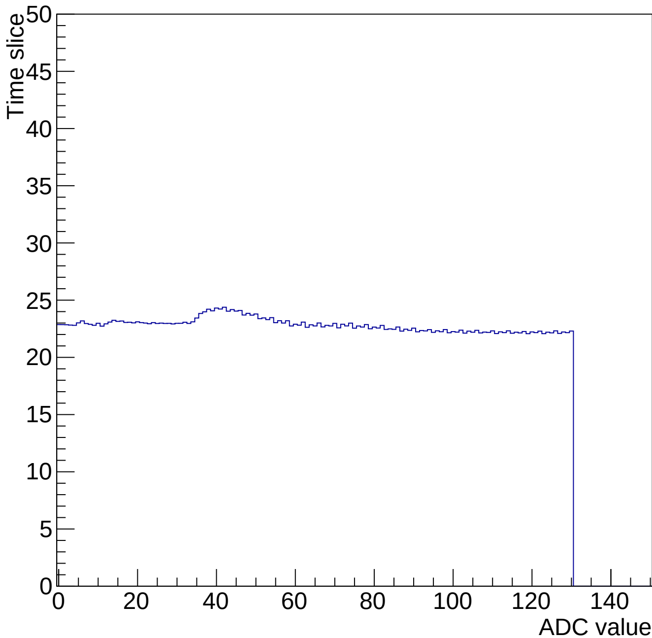
Time mcm 2007 chip 7 chan 10 34701-gain0-shaper0
