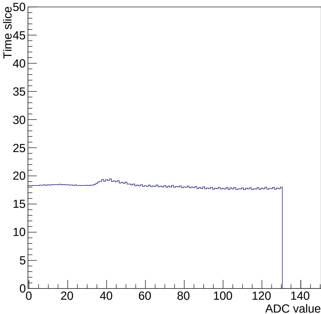
Time mcm 2007 chip 7 chan 9 34701-gain0-shaper0
