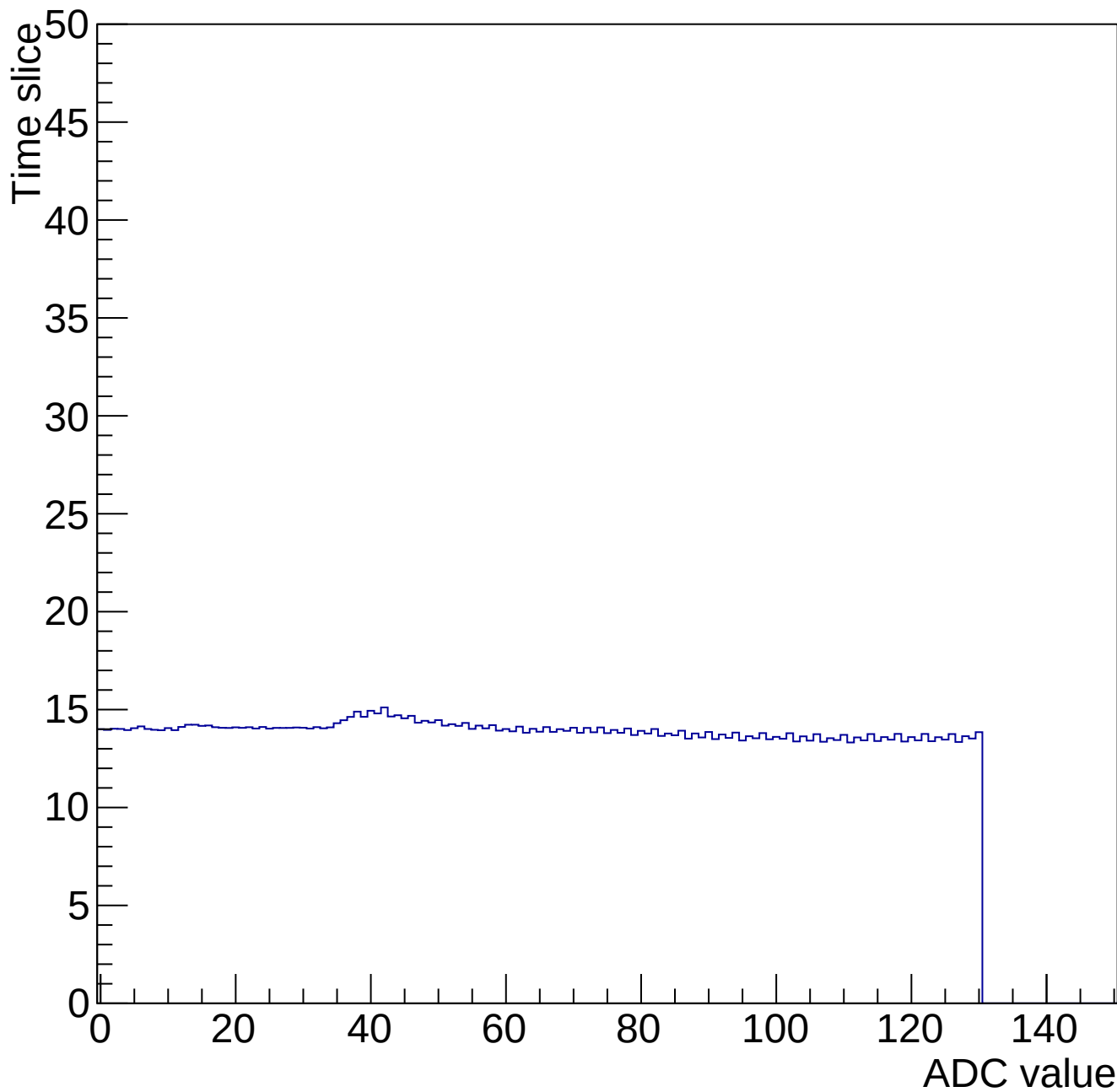
Time mcm 2007 chip 7 chan 12 34701-gain0-shaper0
