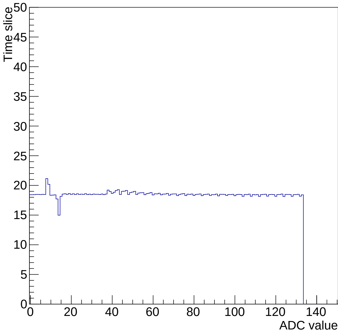
Time mcm 2000 chip 0 chan 2 34706-gain0-shaper6
