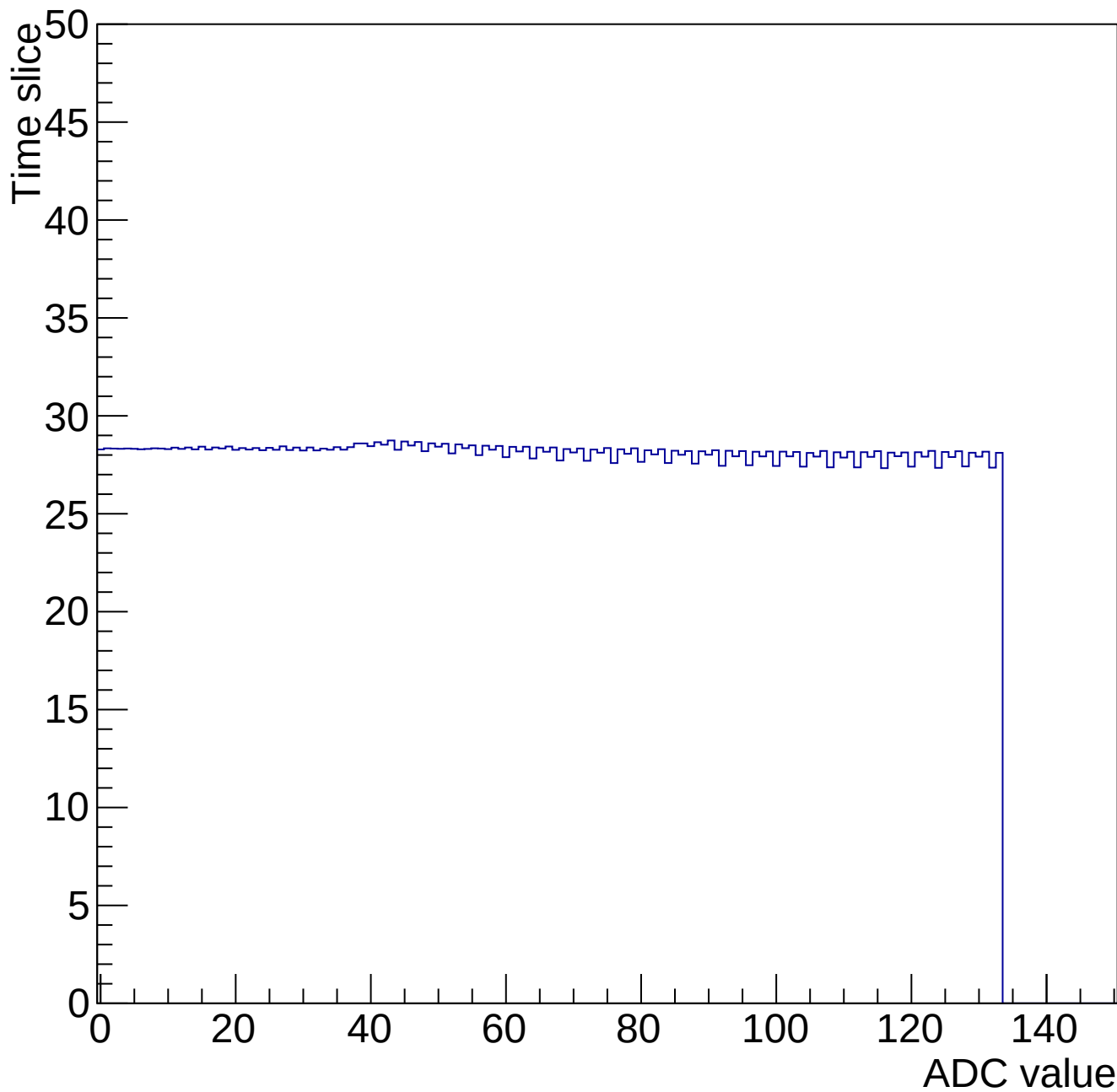
Time mcm 2000 chip 0 chan 5 34706-gain0-shaper6
