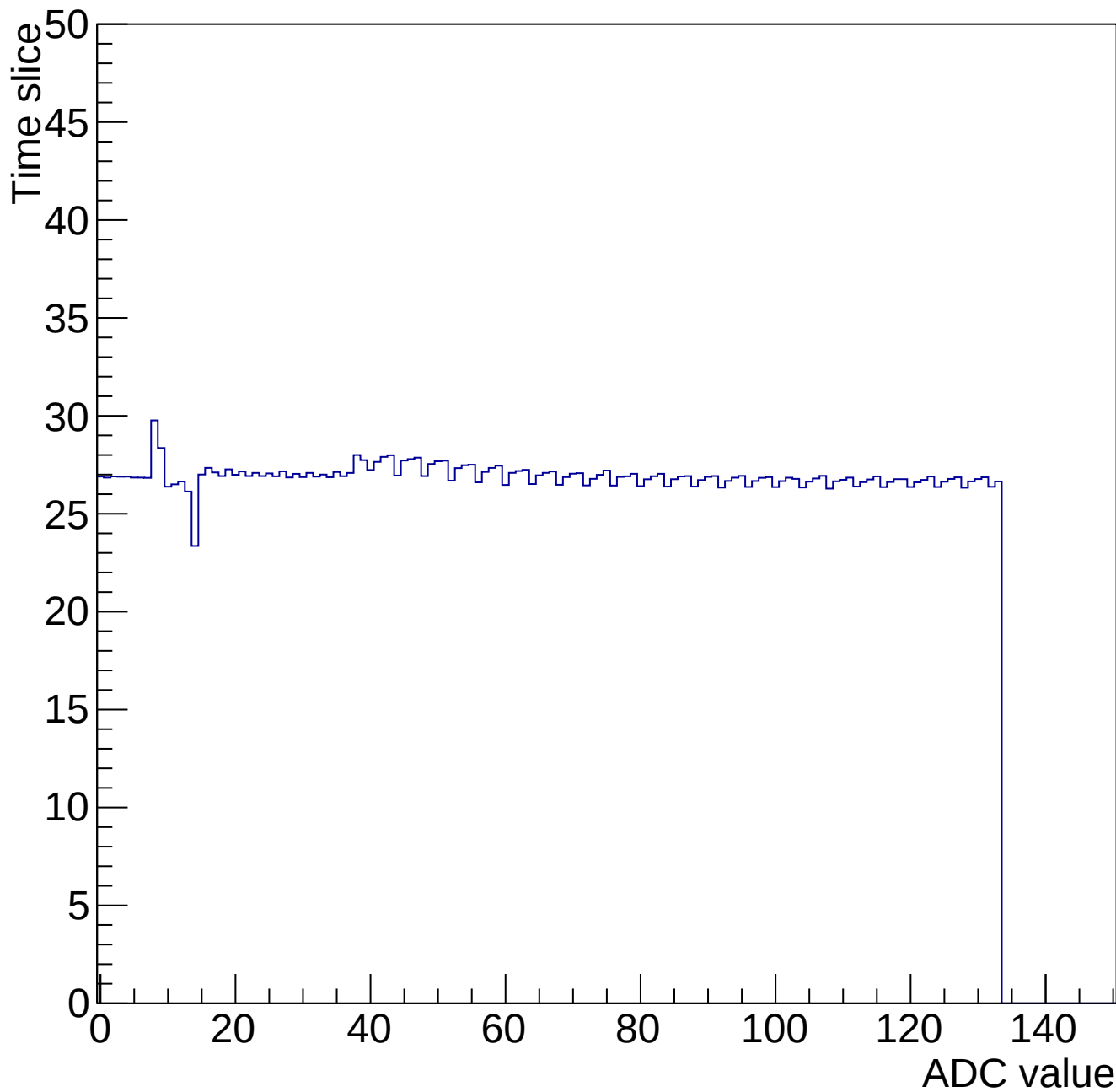
Time mcm 2000 chip 0 chan 1 34706-gain0-shaper6
