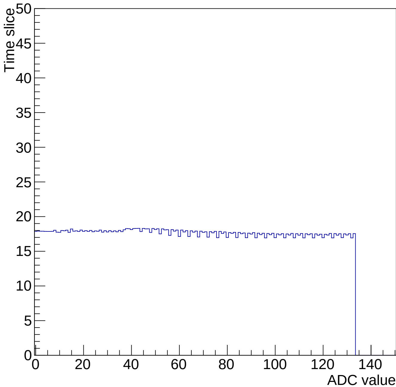
Time mcm 2000 chip 0 chan 15 34706-gain0-shaper6
