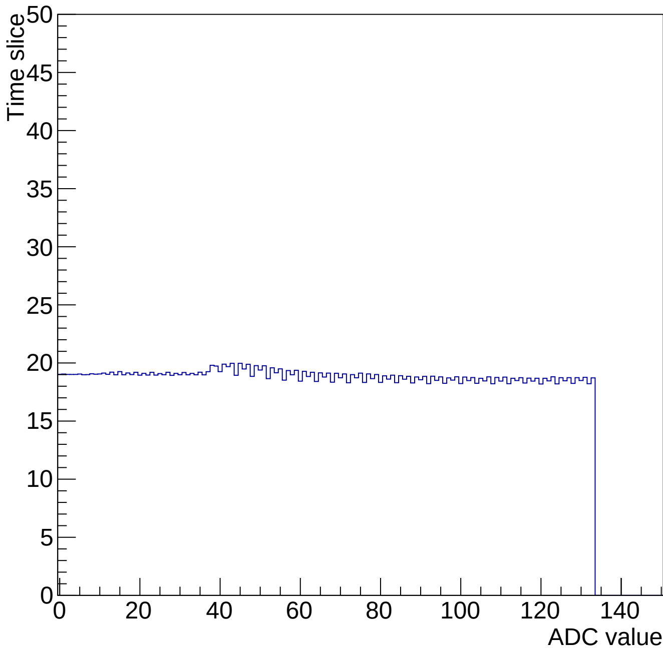
Time mcm 2000 chip 0 chan 3 34706-gain0-shaper6
