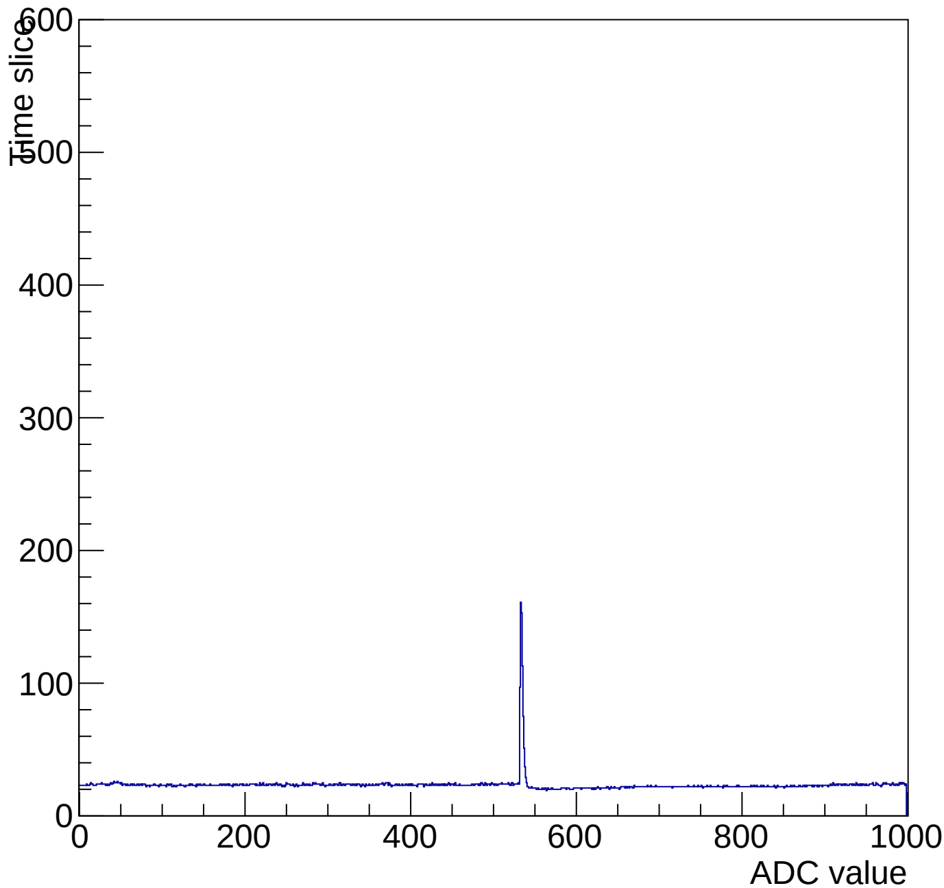
Evt 10 Time mcm 2000 chip 0 chan 4 pulser-10V-wire20
