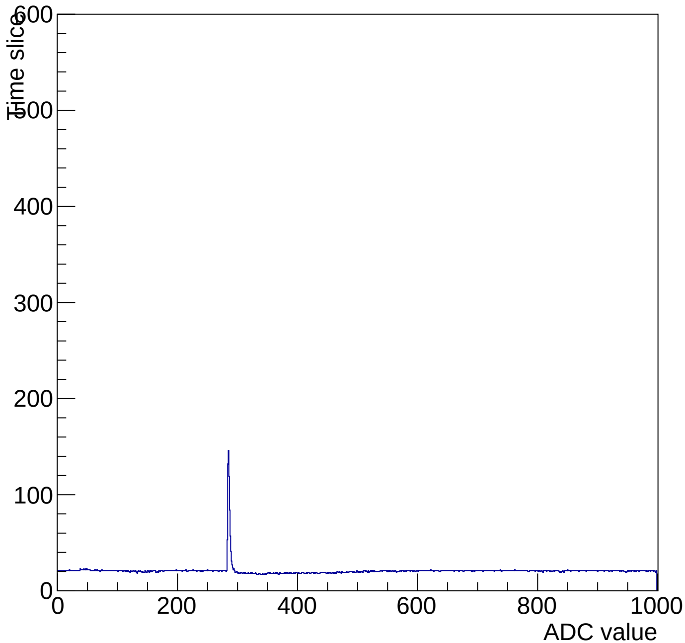
Evt 10 Time mcm 2000 chip 0 chan 11 pulser-10V-wire20
