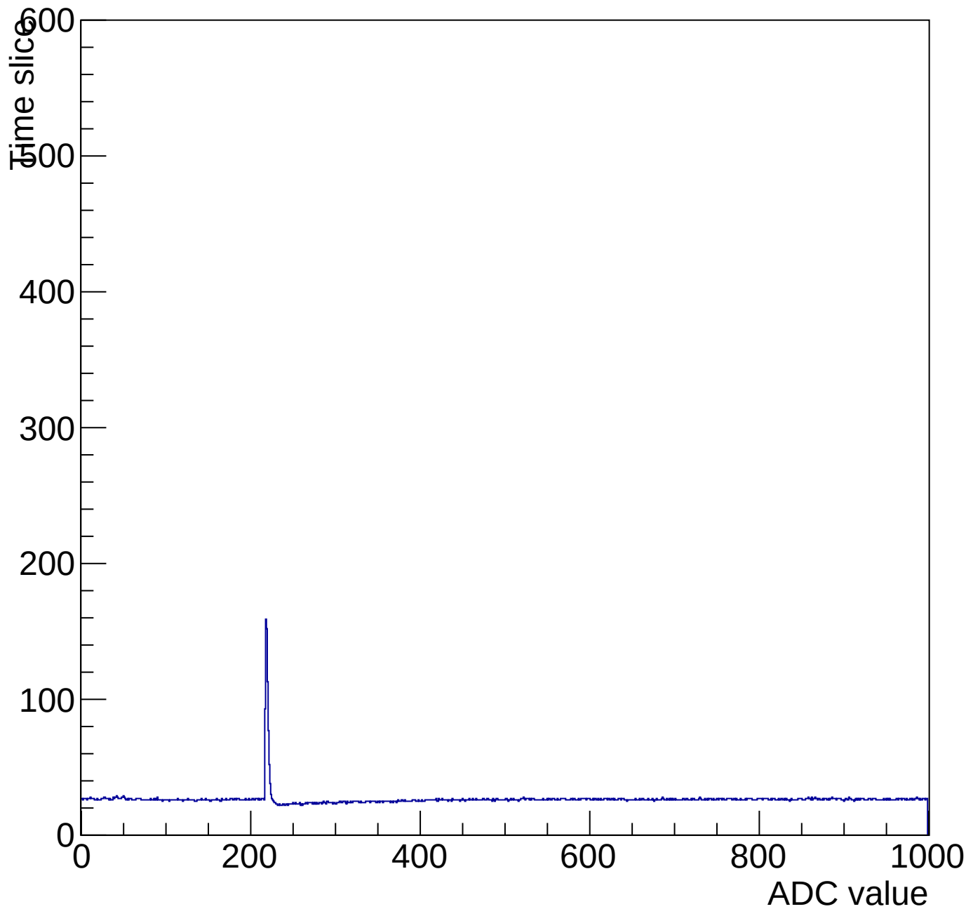
Evt 10 Time mcm 2000 chip 0 chan 7 pulser-10V-wire20
