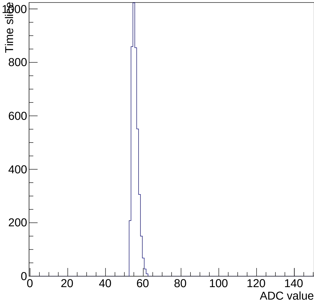
Evt 10 Time mcm 2001 chip 1 chan 1 pulser-10V-wire20-135
