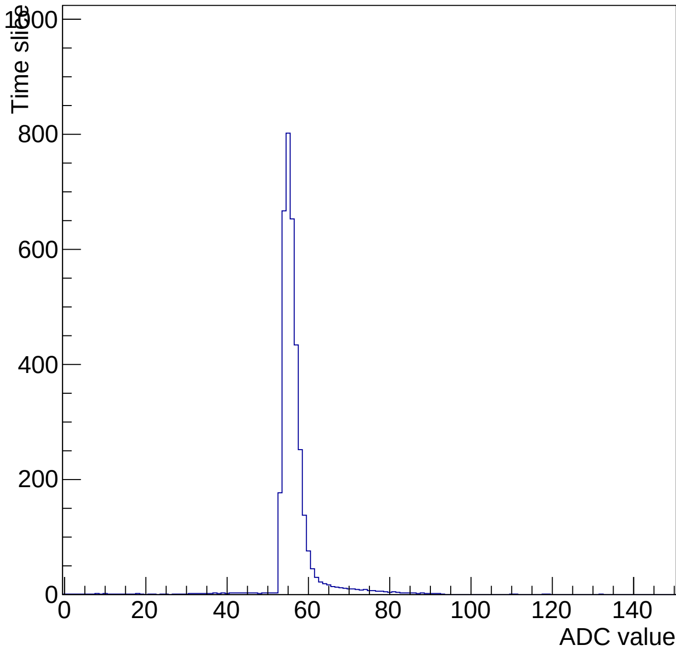
Evt 10 Time mcm 2001 chip 1 chan 13 pulser-10V-wire20-135
