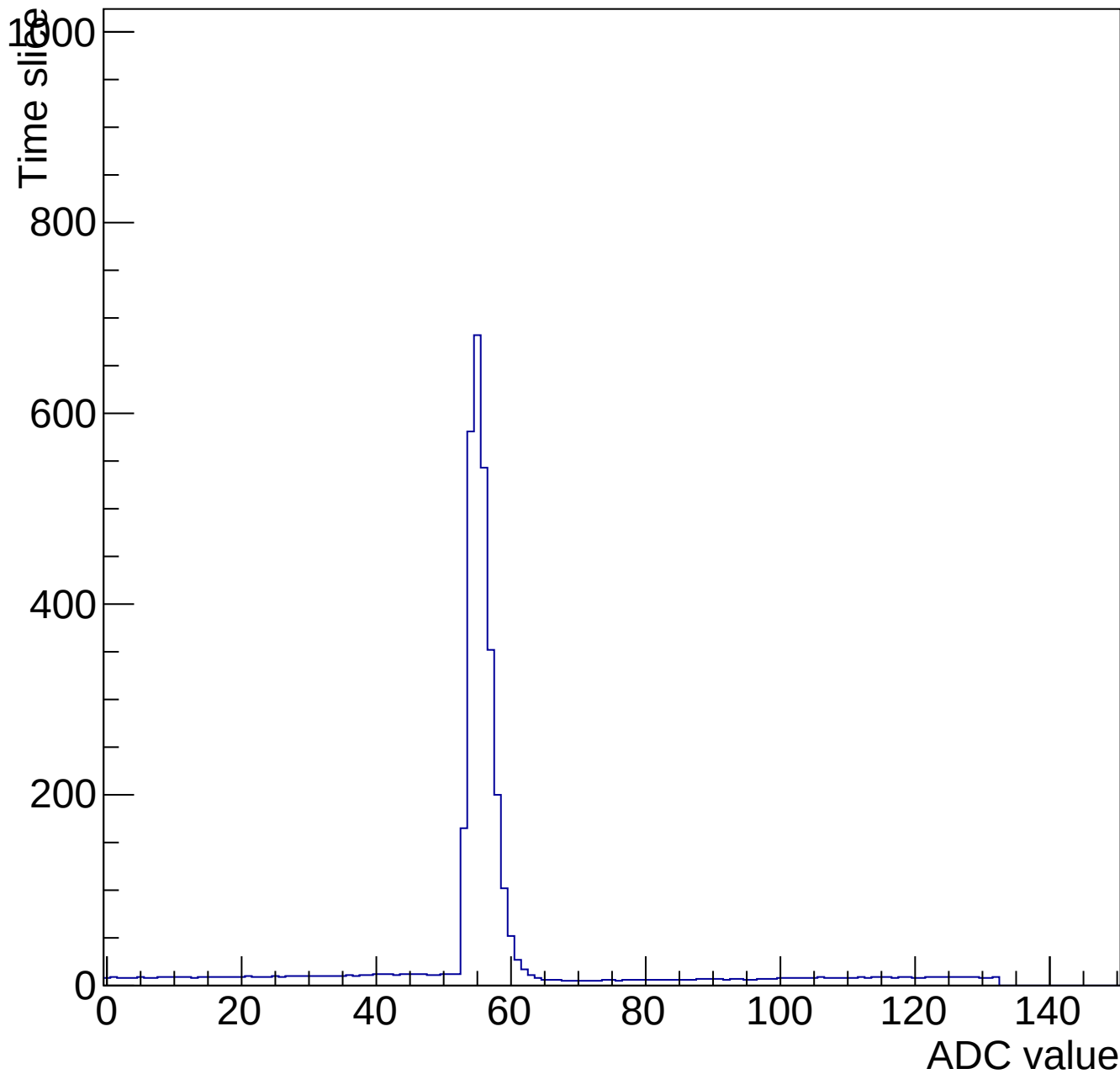
Evt 10 Time mcm 2001 chip 1 chan 10 pulser-10V-wire20-135
