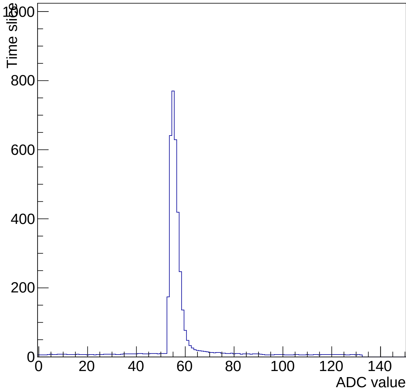
Evt 10 Time mcm 2001 chip 1 chan 15 pulser-10V-wire20-135
