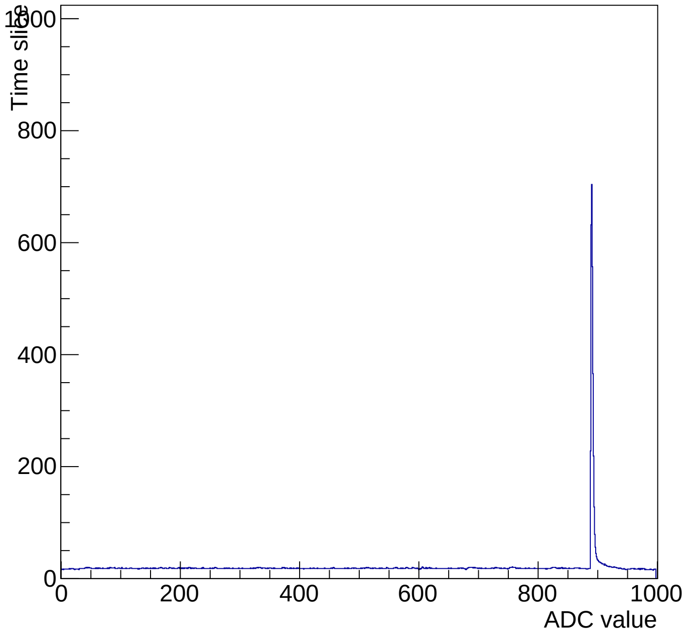
Evt 10 Time mcm 2001 chip 1 chan 5 pulser-6V-wire20
