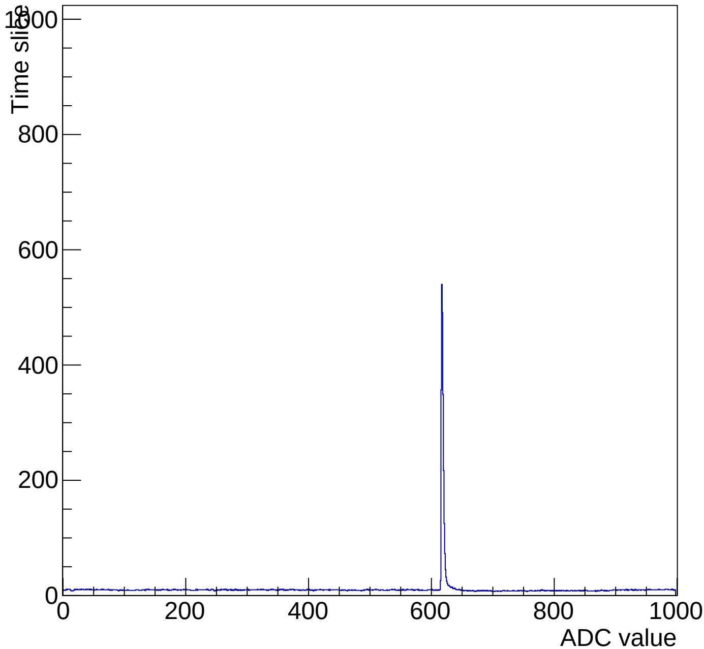
Evt 10 Time mcm 2001 chip 1 chan 14 pulser-6V-wire20
