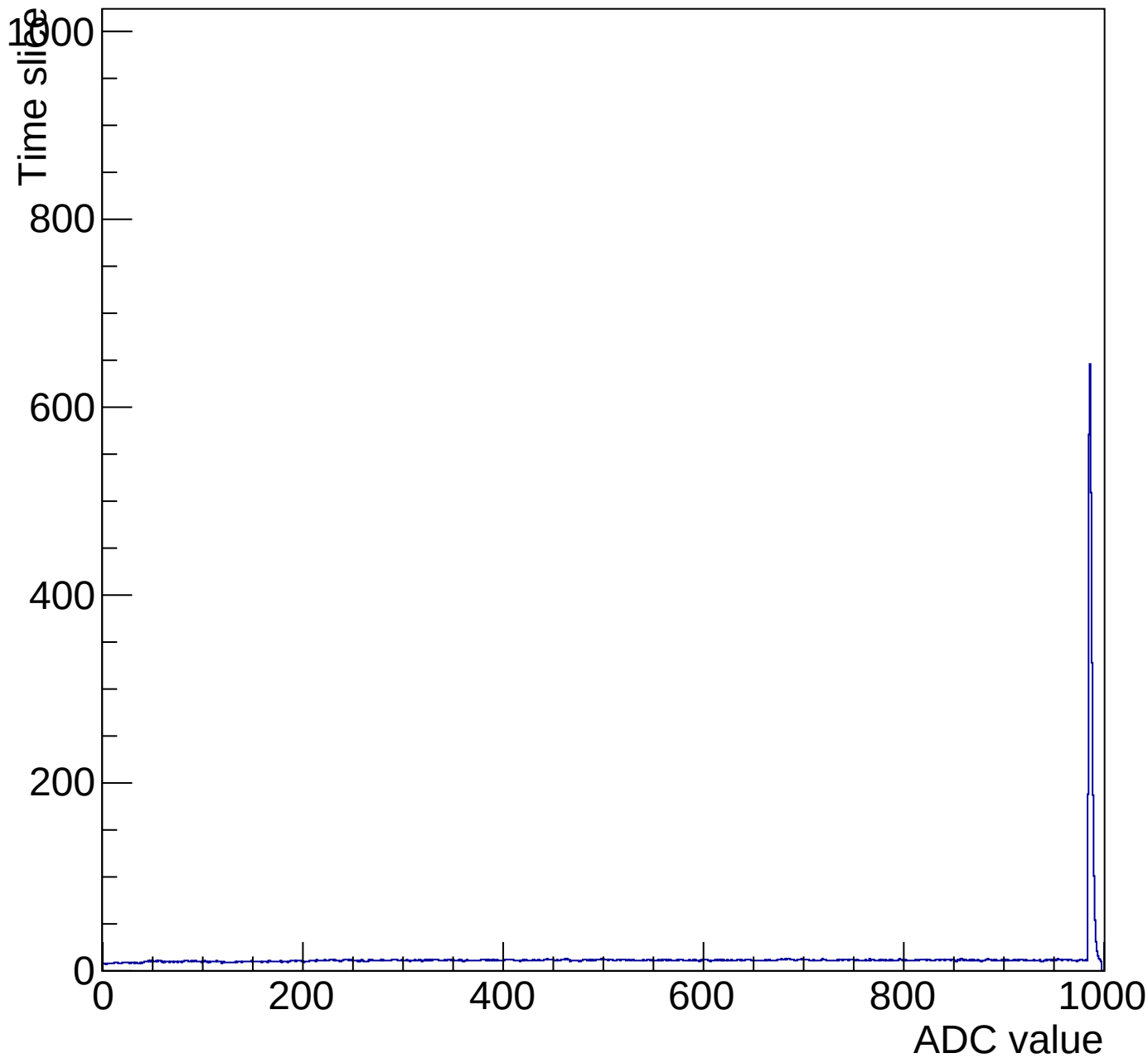
Evt 10 Time mcm 2001 chip 1 chan 7 pulser-6V-wire20
