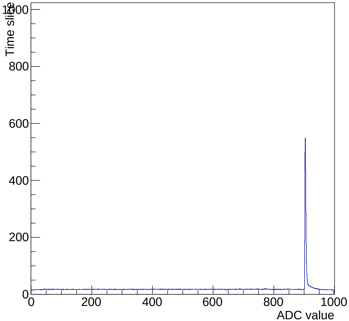
Evt 10 Time mcm 2001 chip 1 chan 8 pulser-6V-wire20
