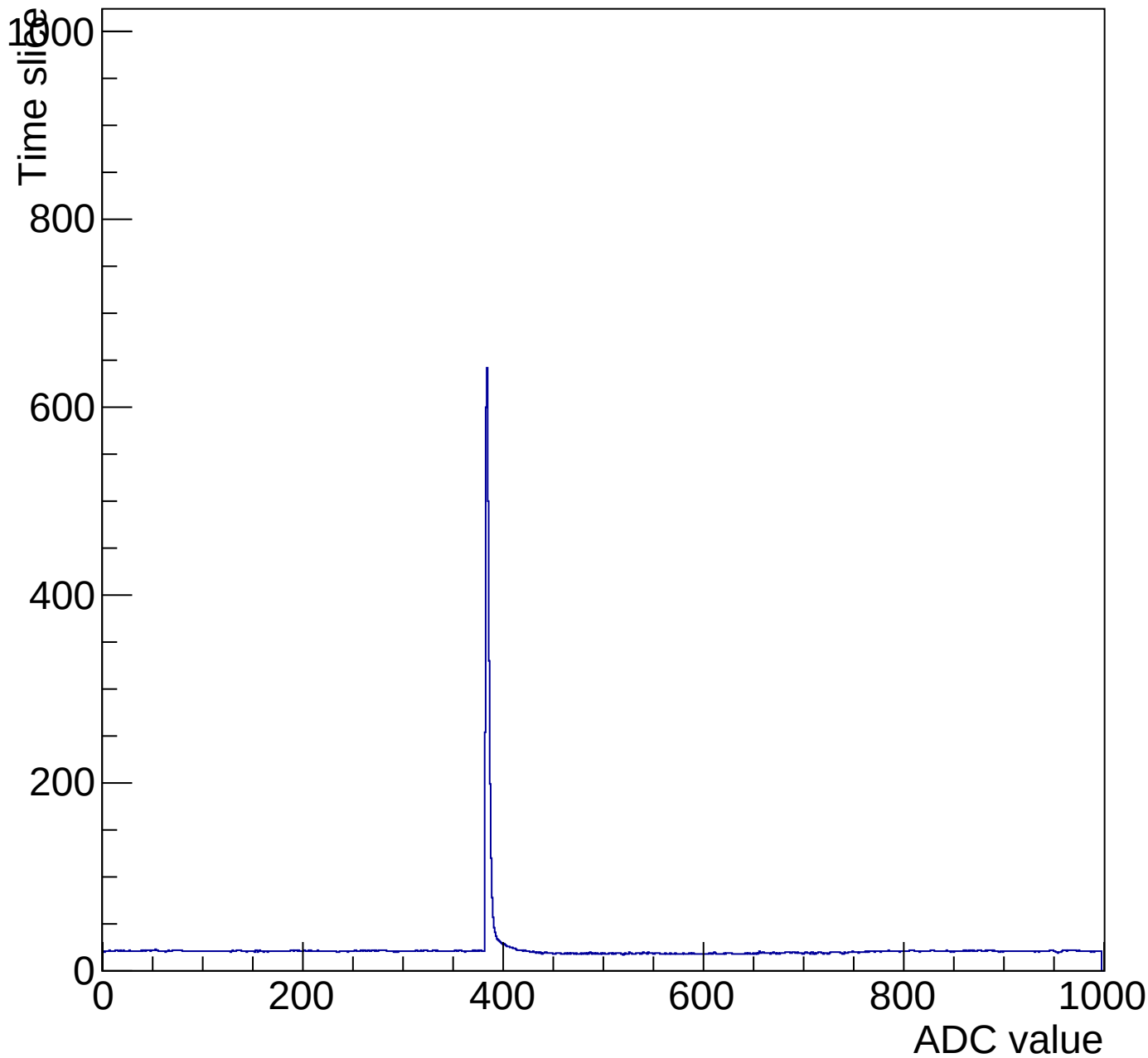
Evt 10 Time mcm 2001 chip 1 chan 11 pulser-6V-wire20
