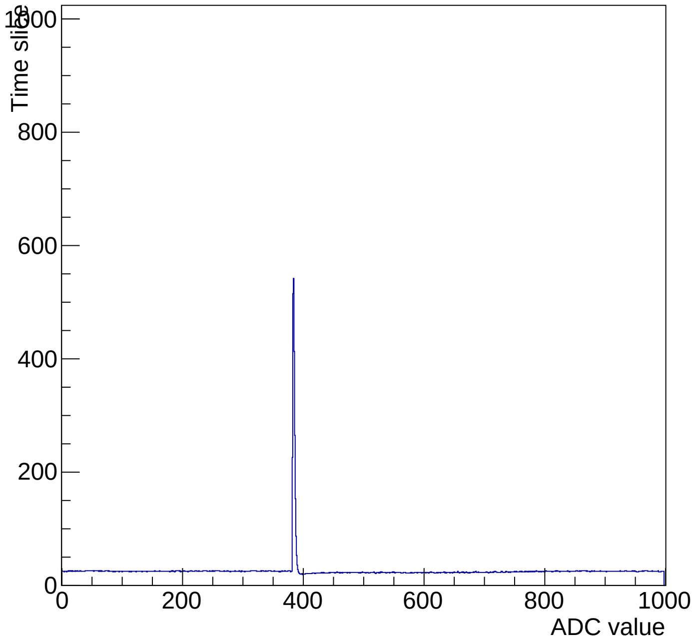
Evt 10 Time mcm 2001 chip 1 chan 10 pulser-6V-wire20
