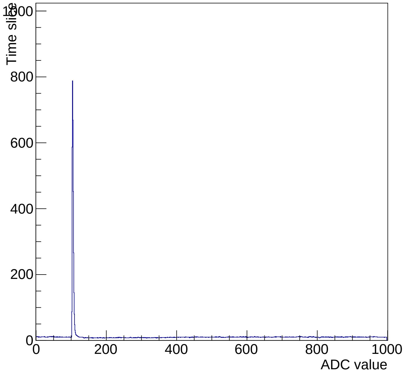
Evt 10 Time mcm 2001 chip 1 chan 1 pulser-6V-wire20
