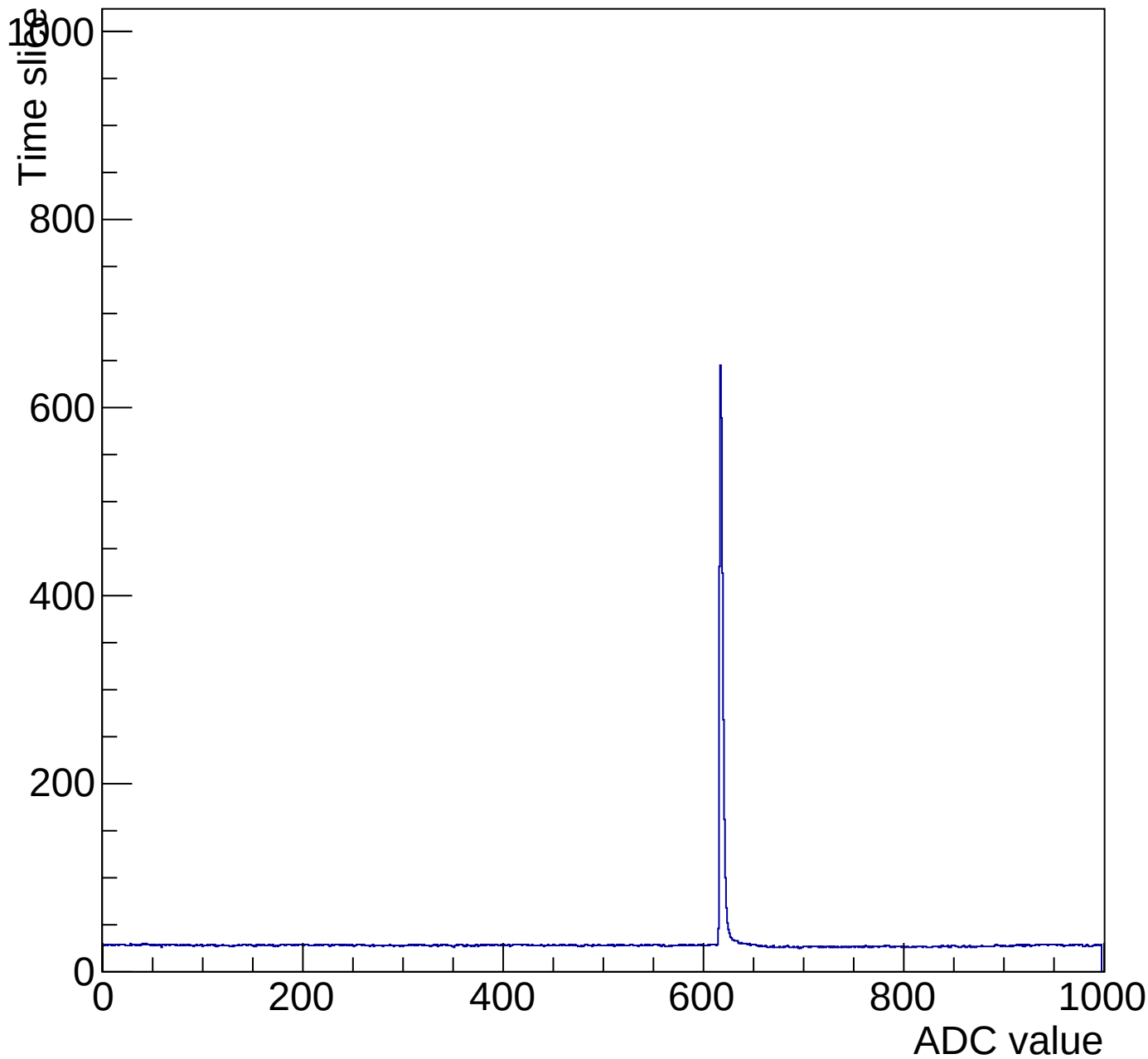
Evt 10 Time mcm 2001 chip 1 chan 15 pulser-6V-wire20
